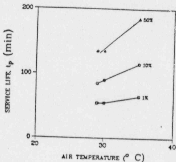
Fig. 21. Effect of air temperature on service lives at constant 24°C dewpoint for an MSA canister (2% TEDA, 5% KI,) at 64 L/min.
