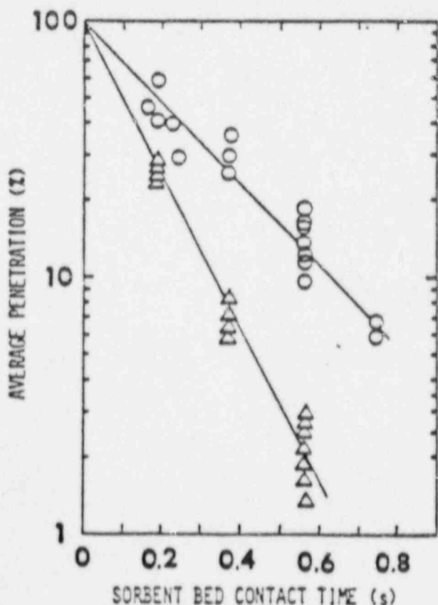
Fig. 9. Average instantaneous percent penetrations as logarithmic functions of bed contact times: O methyl radiiodide for a 5% KI 3 charcoal (GMR-I); Δ, methyl iodide and methyl radiiodide for a 5% TEDA charcoal (Scott).
