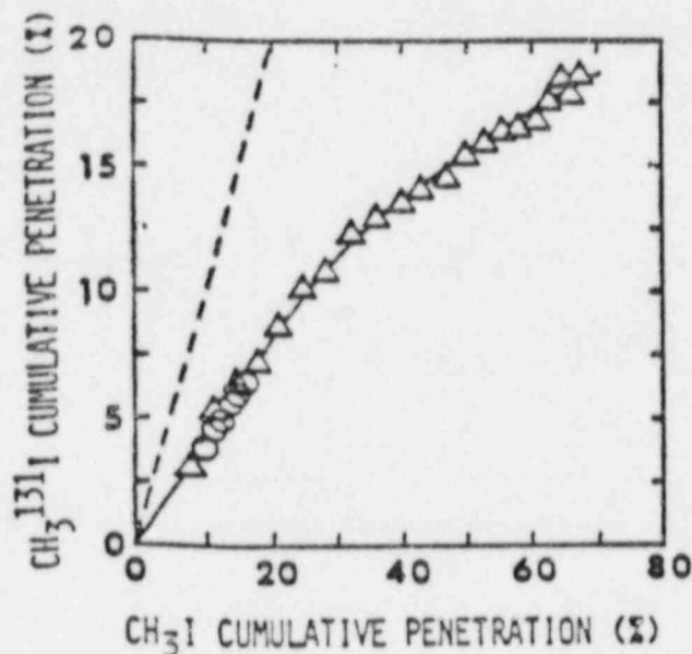
Fig. 6. Comparisons of cumulative percent penetrations of methyl radiiodide and methyl iodide for two 5% KI charcoals: \Delta GMR-I; \circ , GMR-I (TEDA).
