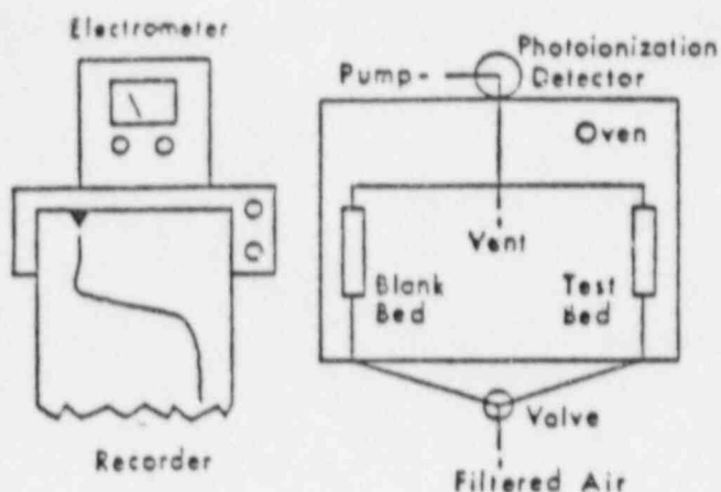
Fig. 23. The apparatus used for studies of TEDA desorption from charcoals.
