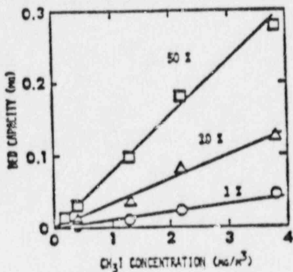
Fig. 10. Dynamic adsorption isotherms at three instantaneous penetration fractions for methyl iodide and MSA GMR-I (2% KI) charcoal.
