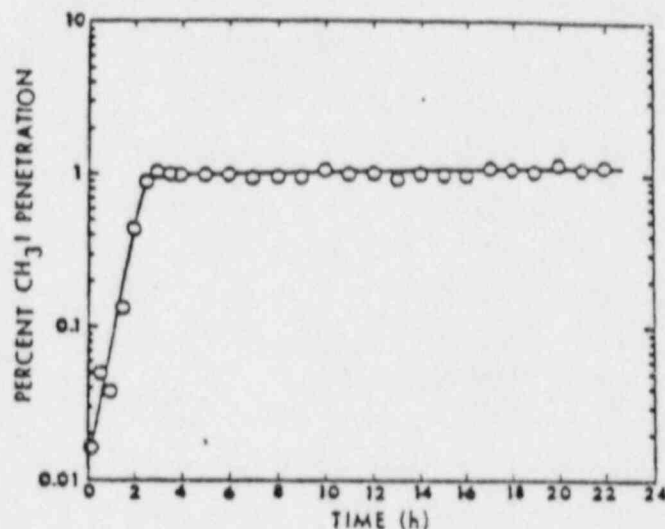
Fig. 13. Effect of exposure time on methyl iodide instantaneous penetration for a fresh Norton Type II cartridge tested at 90% RH, 32 L/min airflow, and 1.7 ppm (7.6 mg/m 3 ) methyl iodide.
