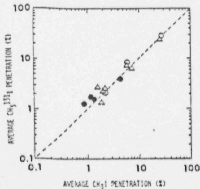
Fig. 7. Comparison of average percent penetrations of methyl radiiodide and methyl iodide for a 5% TEDA-impregnated charcoal (Scott 600252-75). Permeation tube generation: \circ , 97% RH and \Delta , 85% RH; aqueous solution generation: \Delta , 97% RH.
