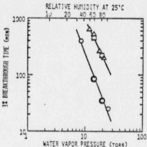
Fig. 15. Correlations of relative humidity and service life (1% breakthrough) for canisters (□, Scott and △, MSA) and a cartridge (○, Scott) containing 5% TEDA charcoals.
