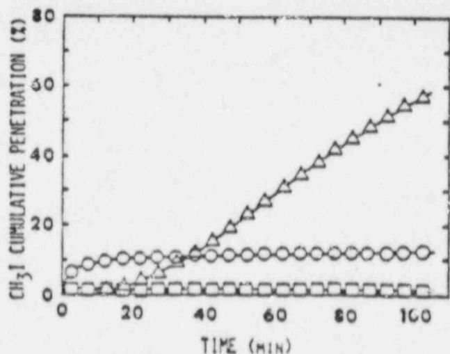
Fig. 4. Methyl iodide cumulative percent penetrations as functions of time for charcoals from three respirator canisters: □, Scott 600252-75 (5% TEDA); ○, MSA GMR-1 (5% KI, + 2% TEDA); Δ, MSA GMR-1 (5% KI).
