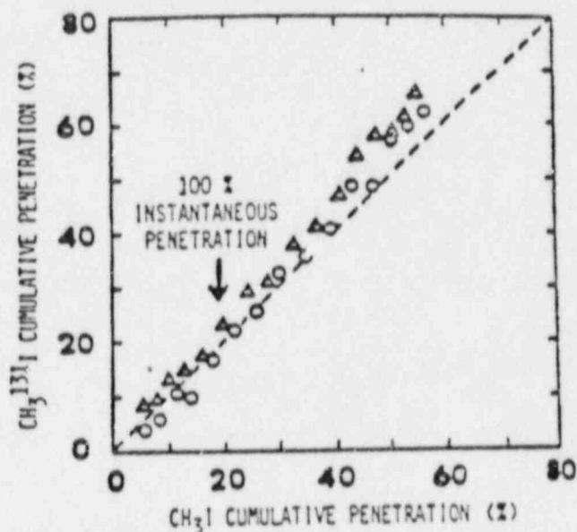
Fig. 8. Comparisons of cumulative percent penetrations of methyl radiiodide and methyl iodide for Whelanized charcoal (GMR-5) for two separate experiments ( \Delta and \circ ).
