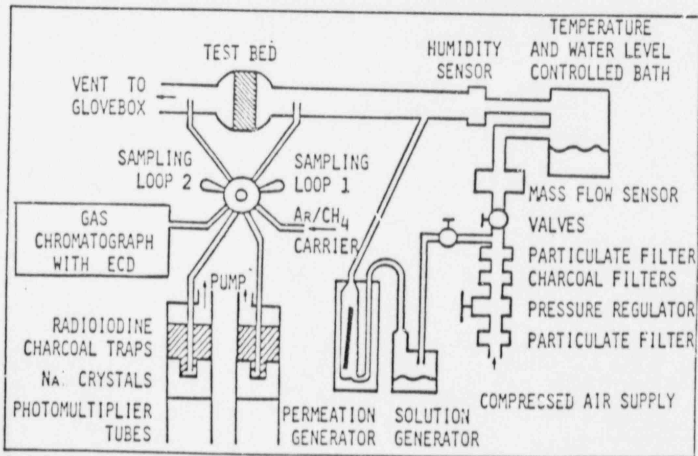
Fig. 2. Experimental apparatus for testing air-purifying respirator cartridges and canisters using radioiodine and normal iodine vapor species.
