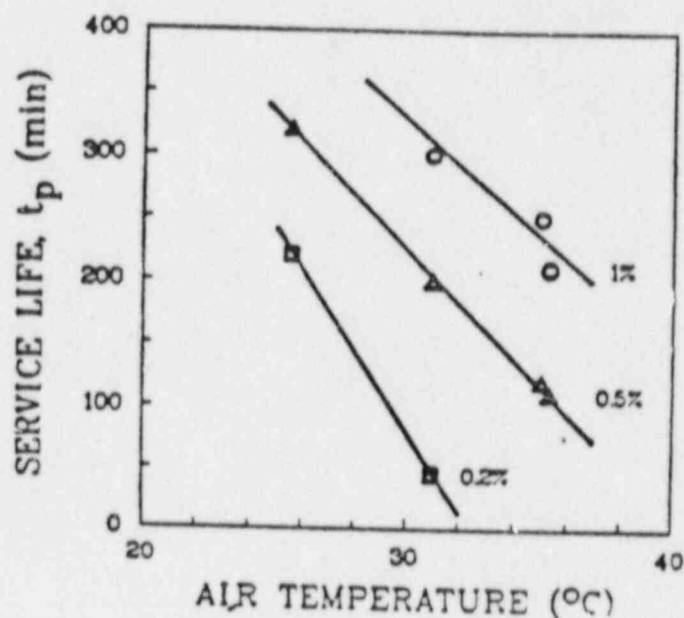
Fig. 20. Effect of air temperature on service lives at constant 50% RH for an MSA canister (2% TEDA, 5% KI 2 ) at 64 L/min.
