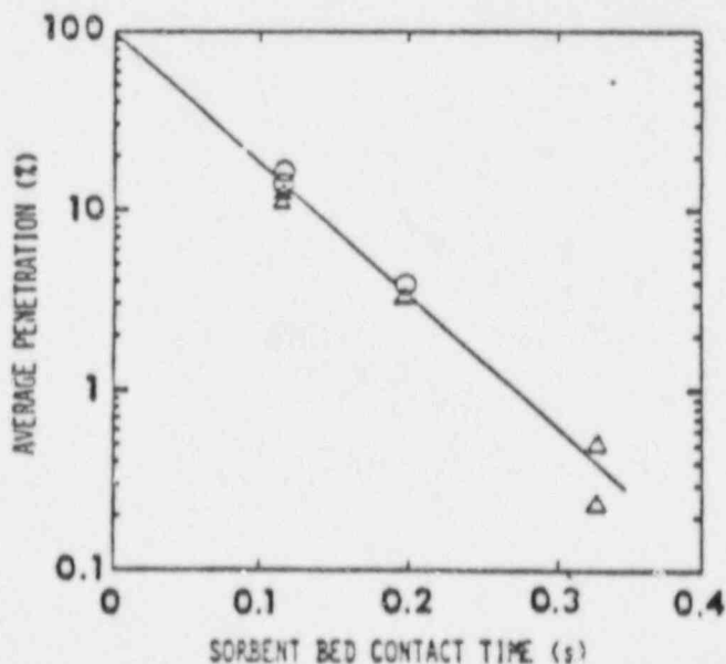
Fig. 11. Dependence of average instantaneous percent penetrations on bed contact times for canisters and cartridges containing 5% TEDA-impregnated charcoals: ○, methyl iodide; △, methyl radiiodide.
