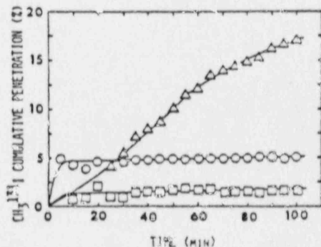
Fig. 5. Methyl radioiodide cumulative percent penetrations as functions of time for charcoals from three respirator canisters: □, Scott 600252-75 (5% TEDA); ○, MSA GMR-1 (5% KI, + 2% TEDA); Δ, MSA GMR-1 (5% KI).
