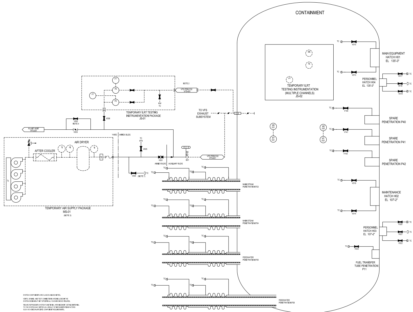
Figure 6.2.5-1 Simplified Containment Leak Rate Test System Piping and Instrumentation Diagram (REF) VUS 001
