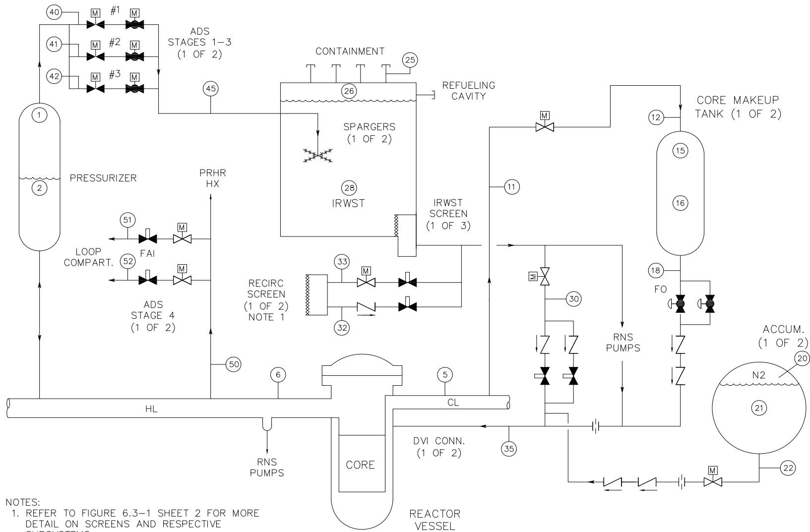
Inside Reactor Containment Figure 6.3-4 Passive Decay Heat Removal (REF) RCS & PXS
