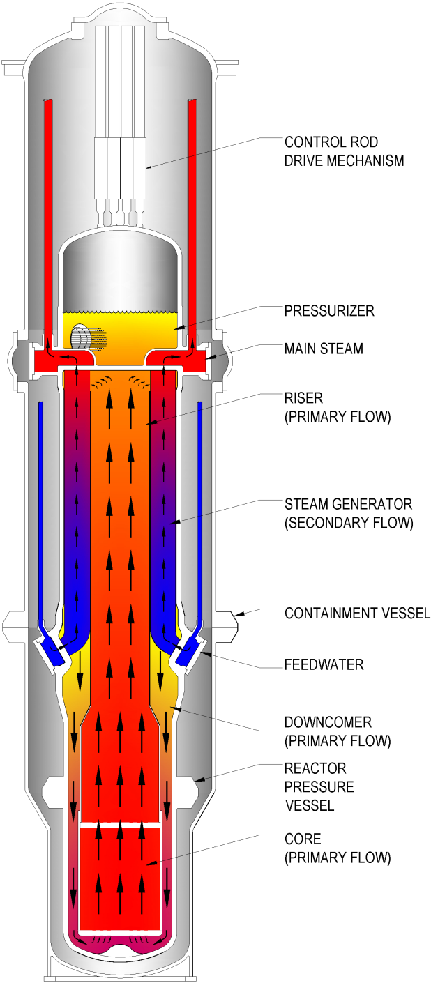
Figure 1.2-6: Cutaway View of NuScale Power Module
