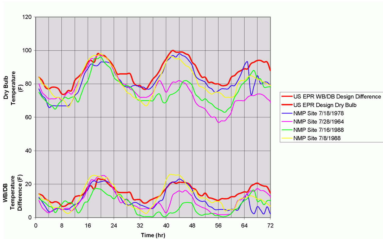
Figure 2.3-105—{Comparison of U.S. EPR Design and NMP3NPP Site Temperatures for Maximum Evaporation}
