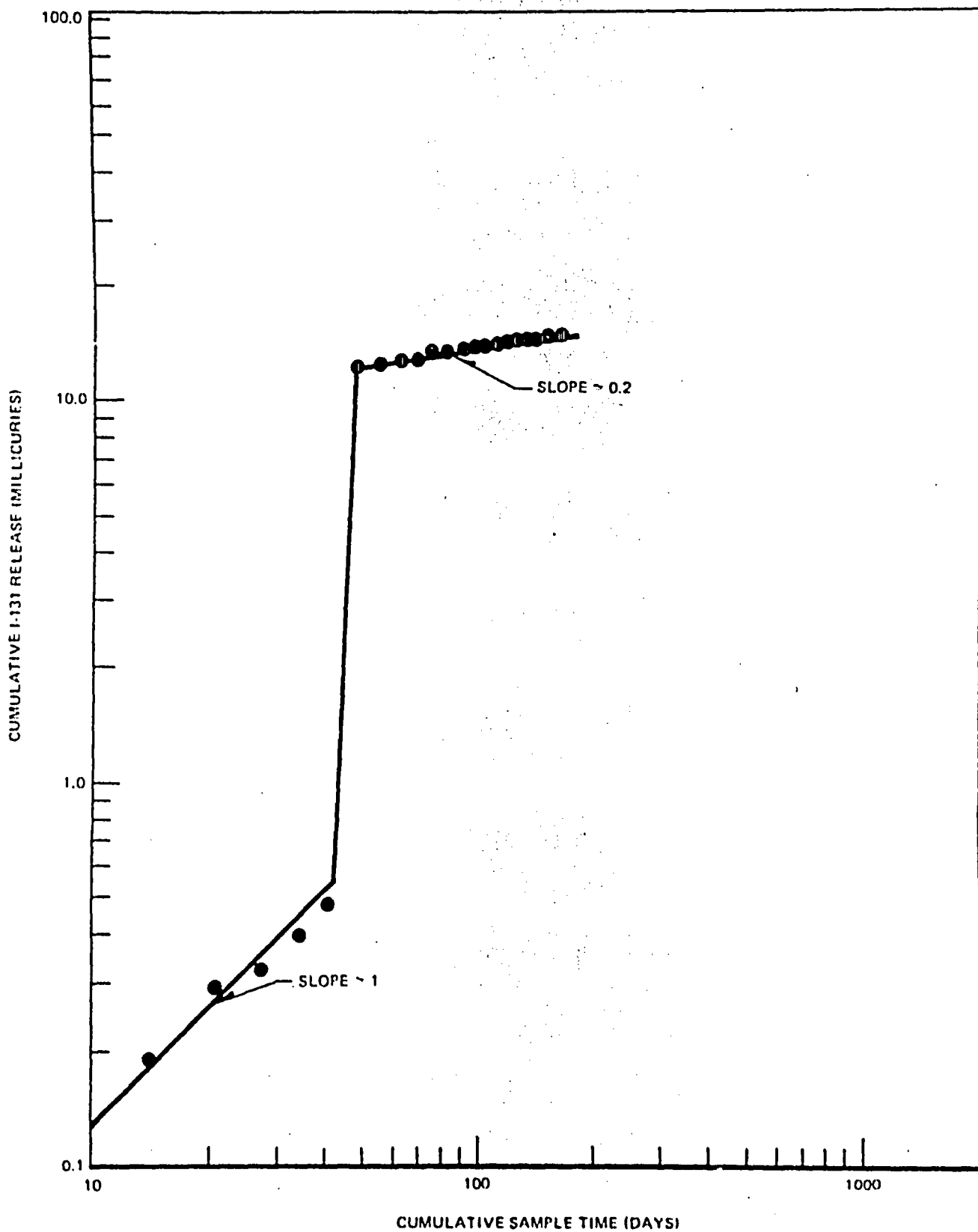
Figure 6-62. Cumulative Normalized I-131 Reactor Building Airborne Release at Oyster Creek (1976)
