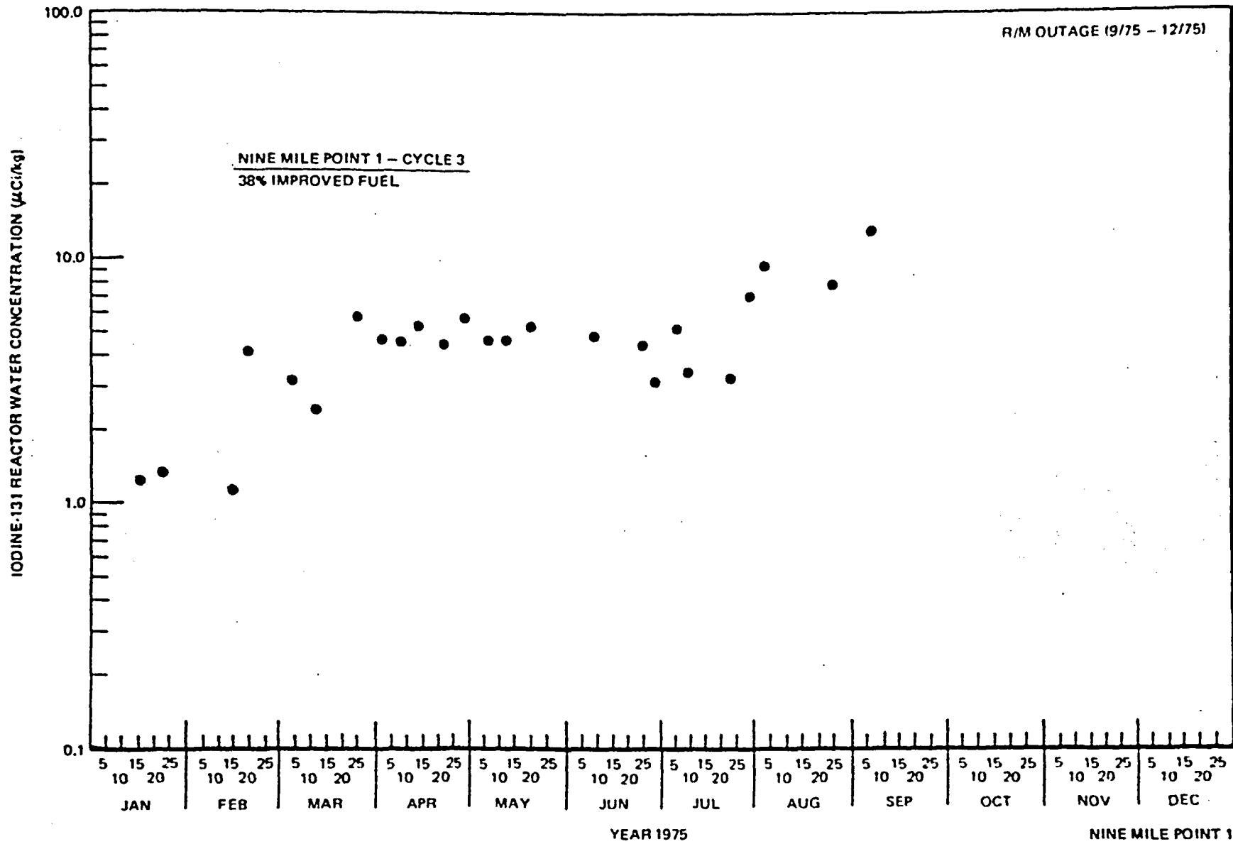
Figure 6-18. Iodine-131 Reactor Water Concentration at Nine Mile Point 1, 1975
