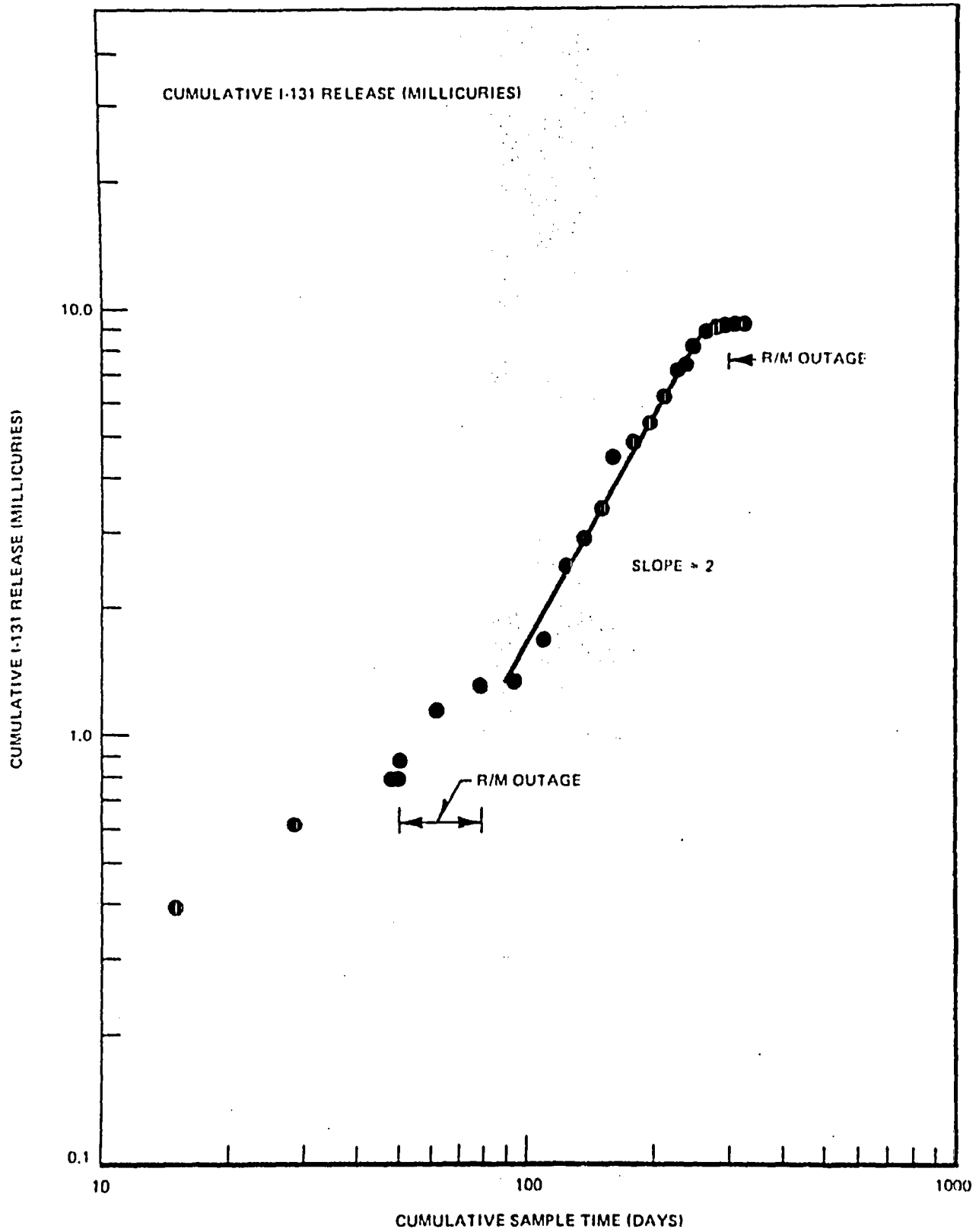
Figure 6-58. Cumulative Normalized I-131 Reactor Building Airborne Release at Monticello
