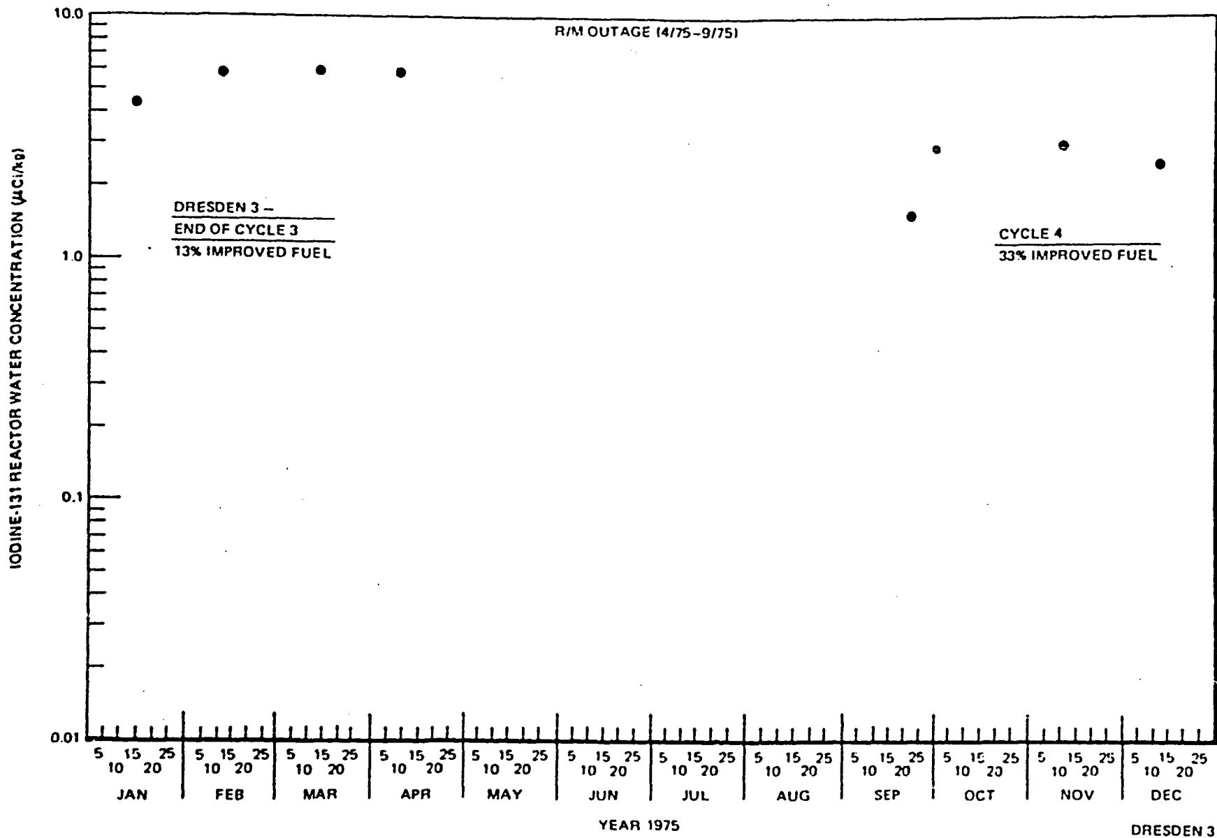
Figure 6-9. Iodine-131 Reactor Water Concentration at Dresden 3, 1975
