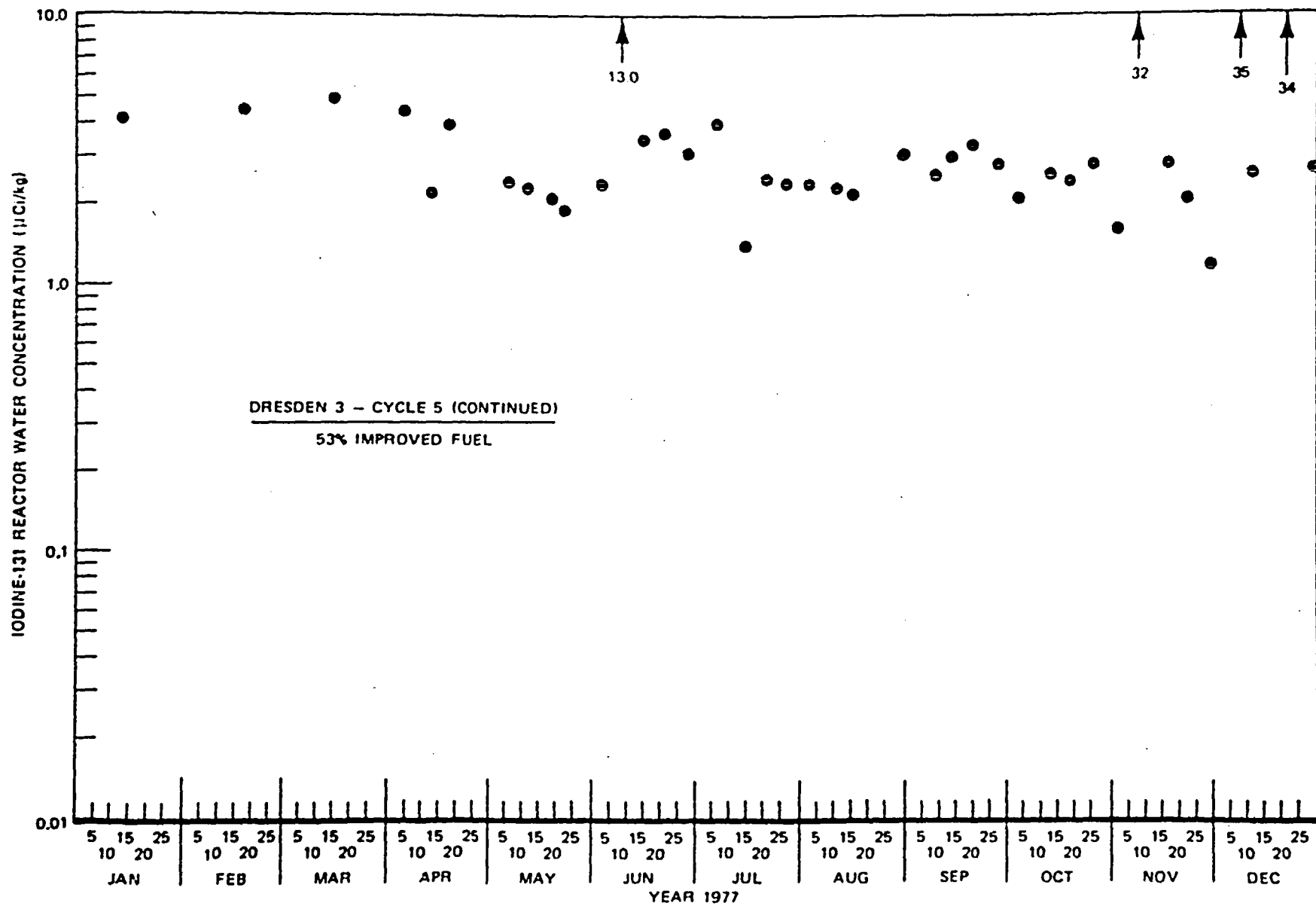
Figure 6-9b. Iodine-131 Reactor Water Concentration at Dresden 3, 1977
