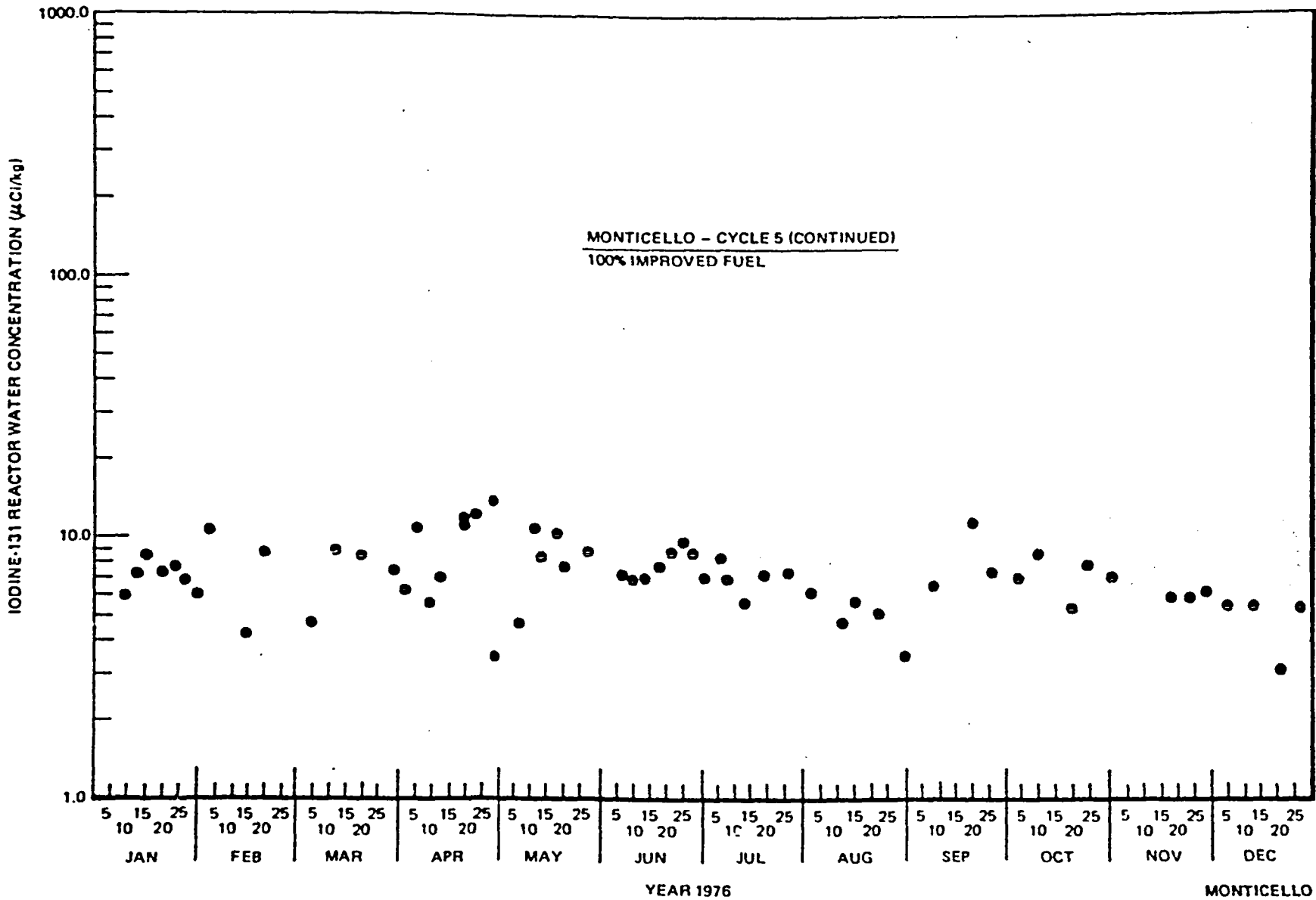
Figure 6-17. Iodine-131 Reactor Water Concentration at Monticello, 1976
