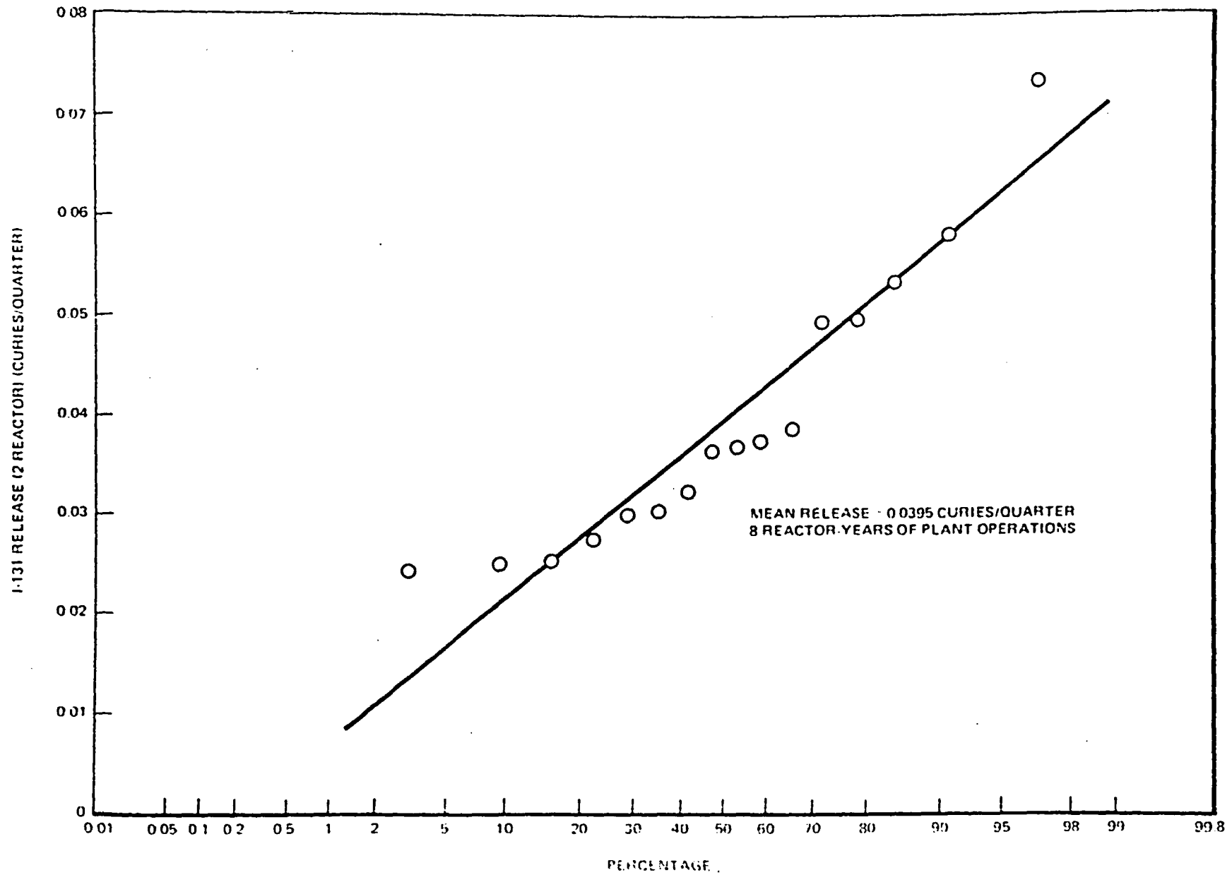
Figure 36. Accumulative Normal Probability Distribution of Calendar Quarter Reactor Ventilation Releases of I-131, Quad Cities 1-2 (July 1973 to June 1977)
