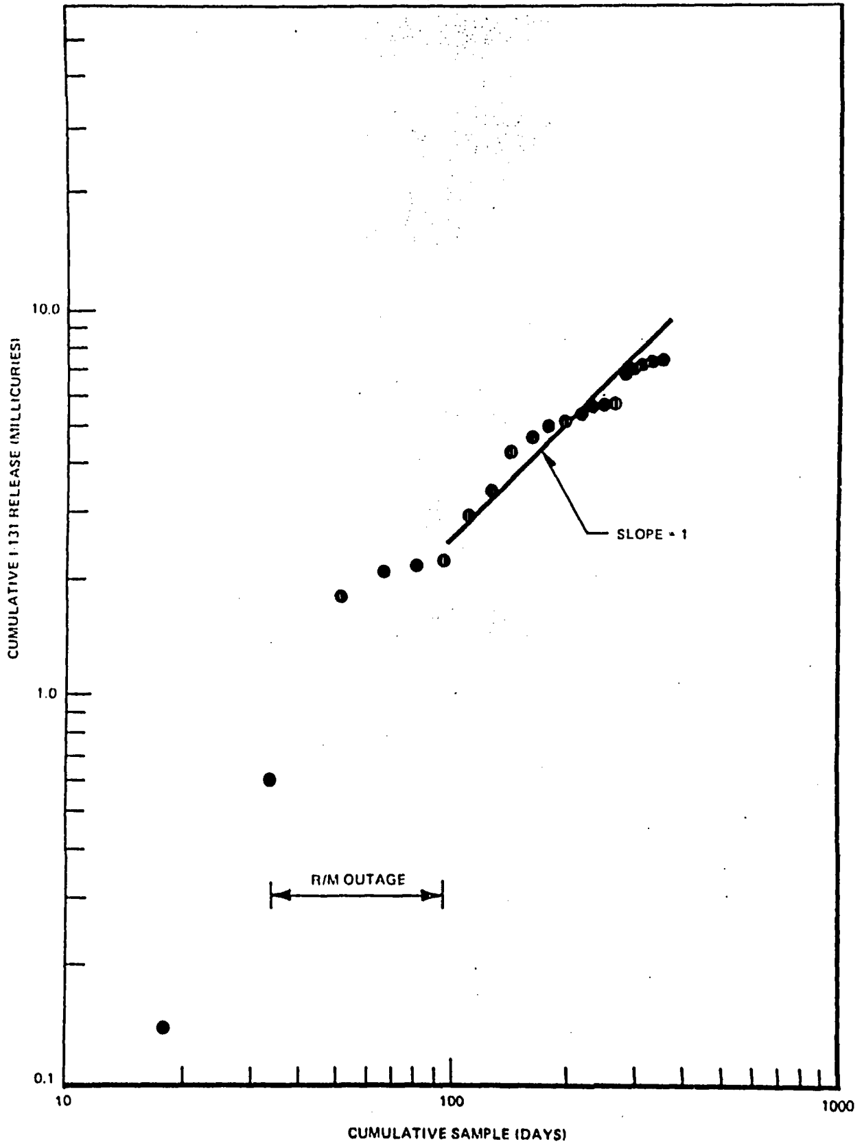
Figure 6-61. Cumulative Normalized I-131 Reactor Building Airborne Release at Oyster Creek (1975 - 1976)
