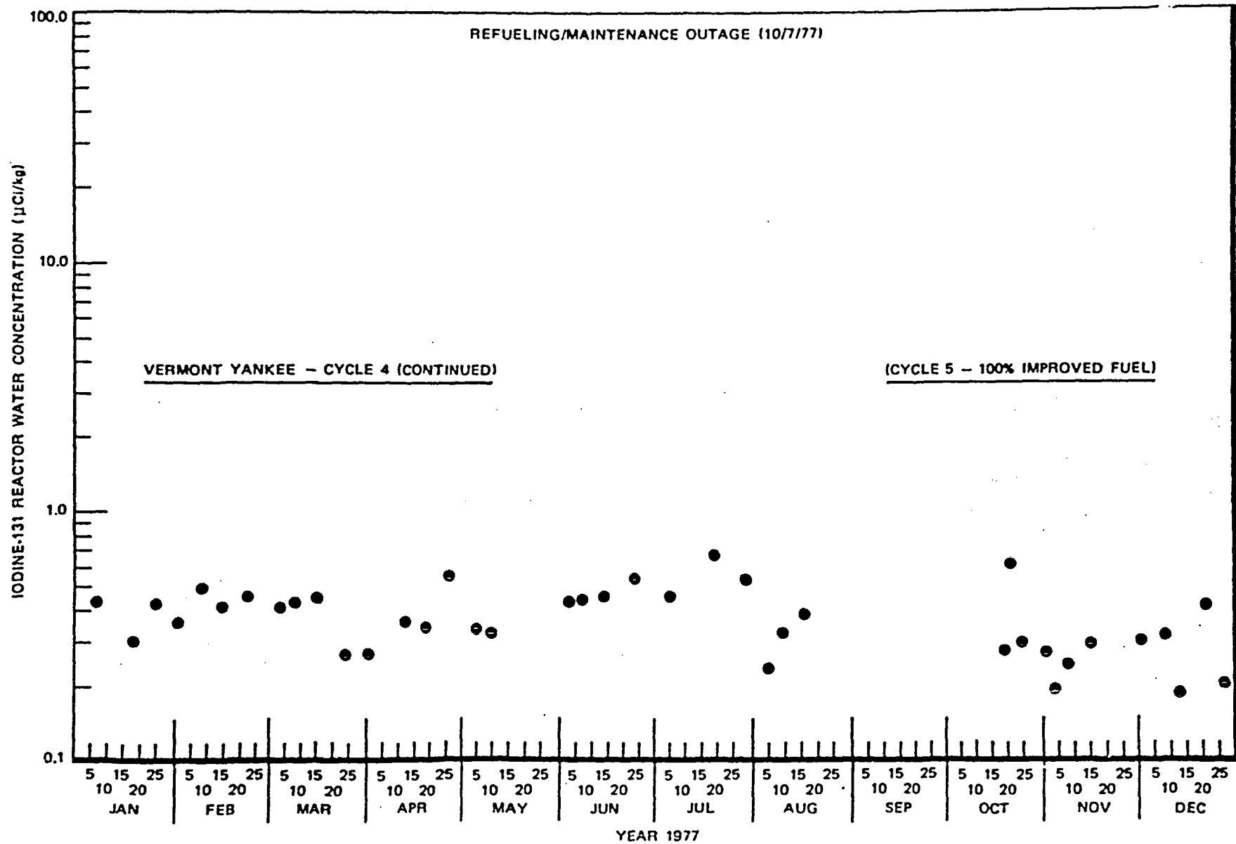
Figure 6-34a. Iodine-131 Reactor Water Concentration at Vermont Yankee, 1977
