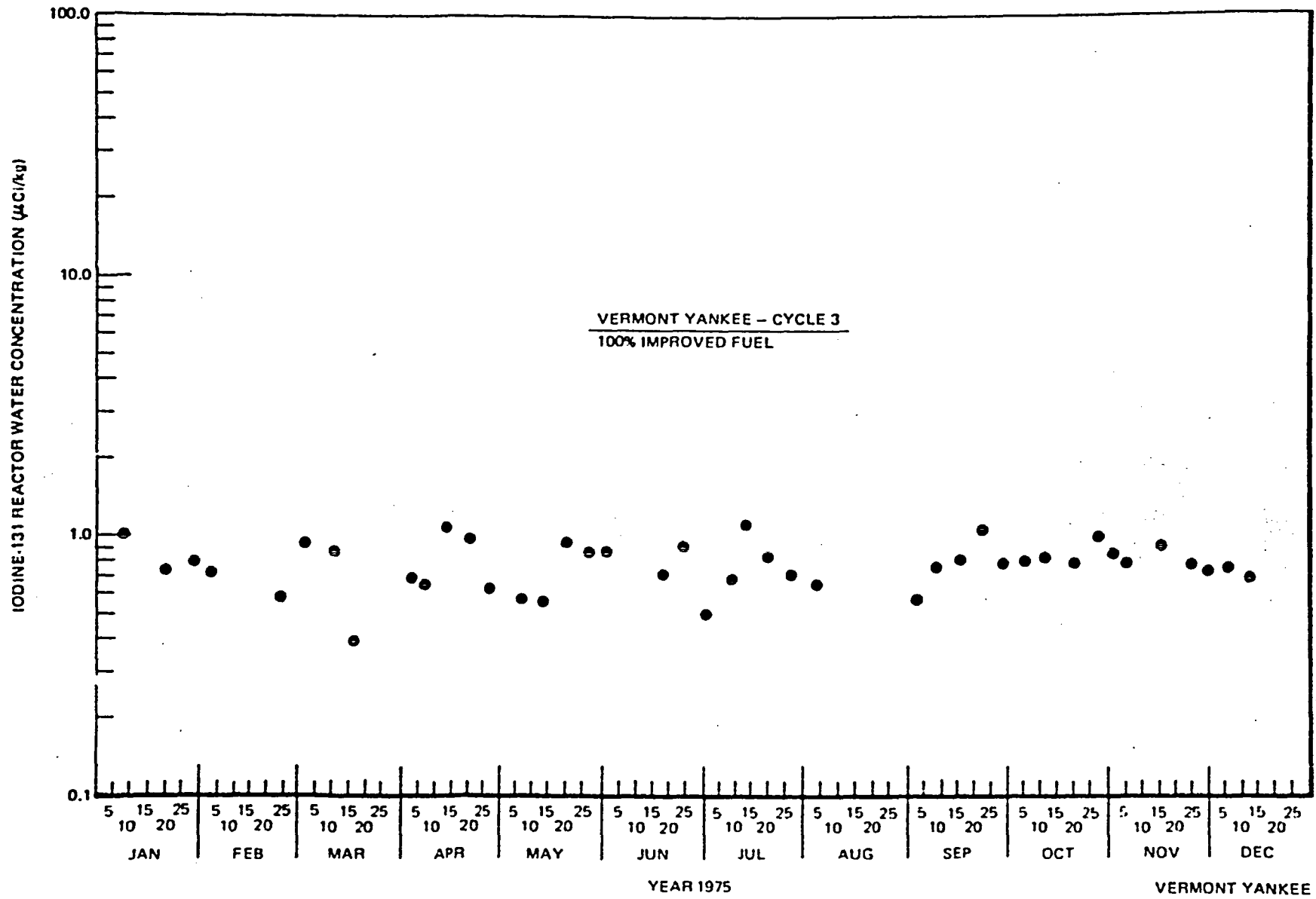
Figure 6-33. Iodine-131 Reactor Water Concentration at Vermont Yankee, 1975
