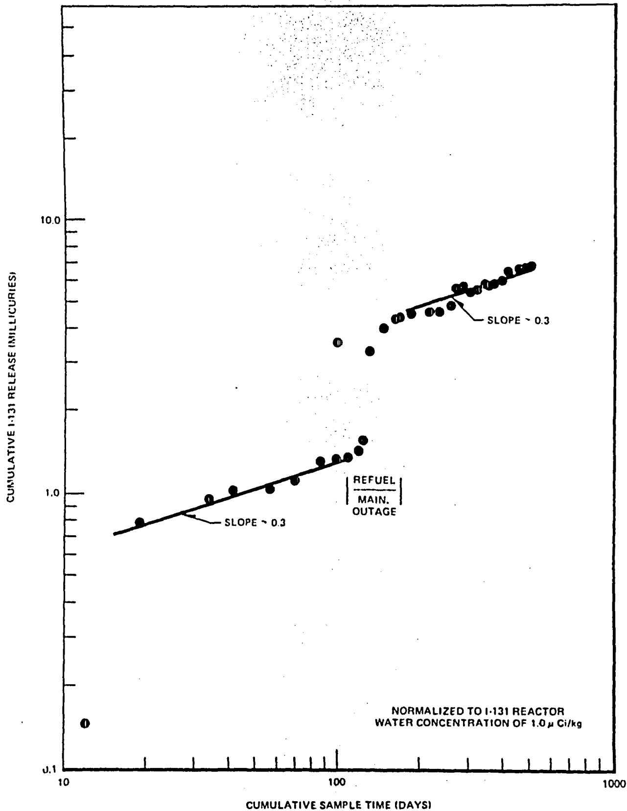
Figure 6-55. Cumulative Normalized I-131 Radwaste Building Airborne Release at Vermont Yankee
