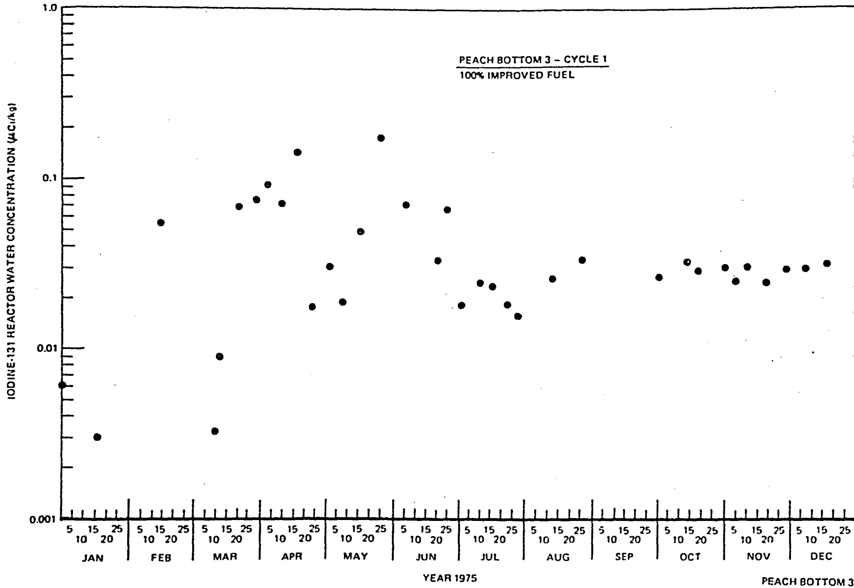
Figure 6-24. Iodine-131 Reactor Water Concentration at Peach Bottom 3, 1975
