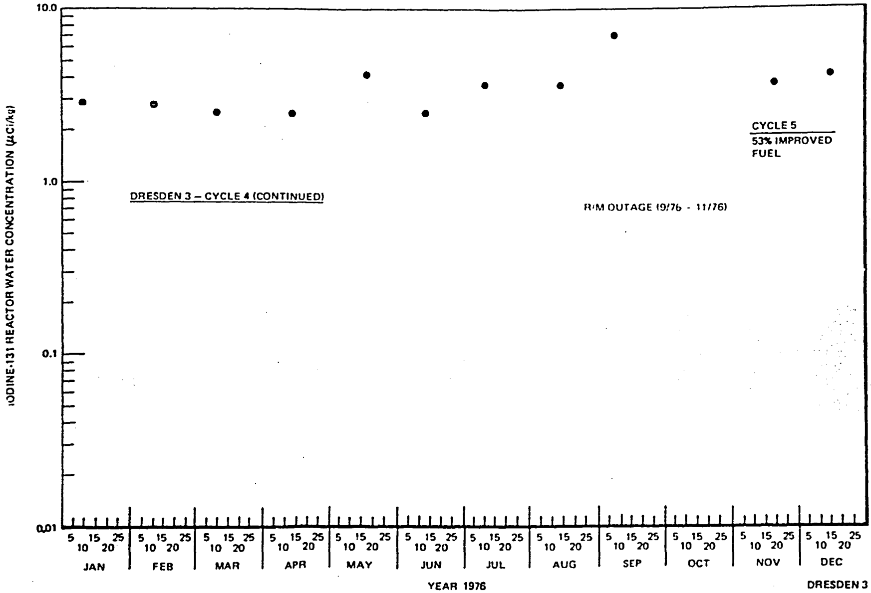
Figure 6-9a. Iodine-131 Reactor Water Concentration at Dresden 3, 1976
