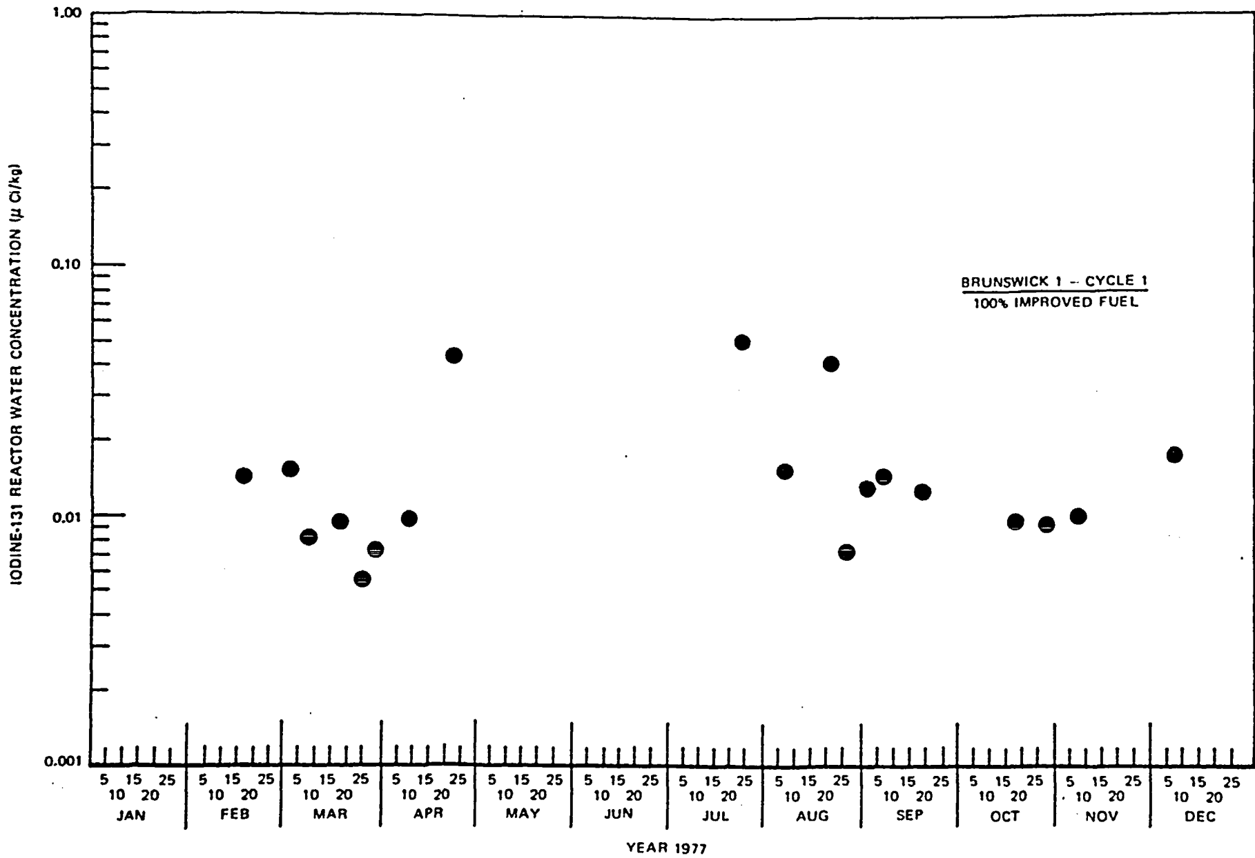
Figure 6-5. Iodine-131 Reactor Water Concentration at Brunswick 1, 1977
