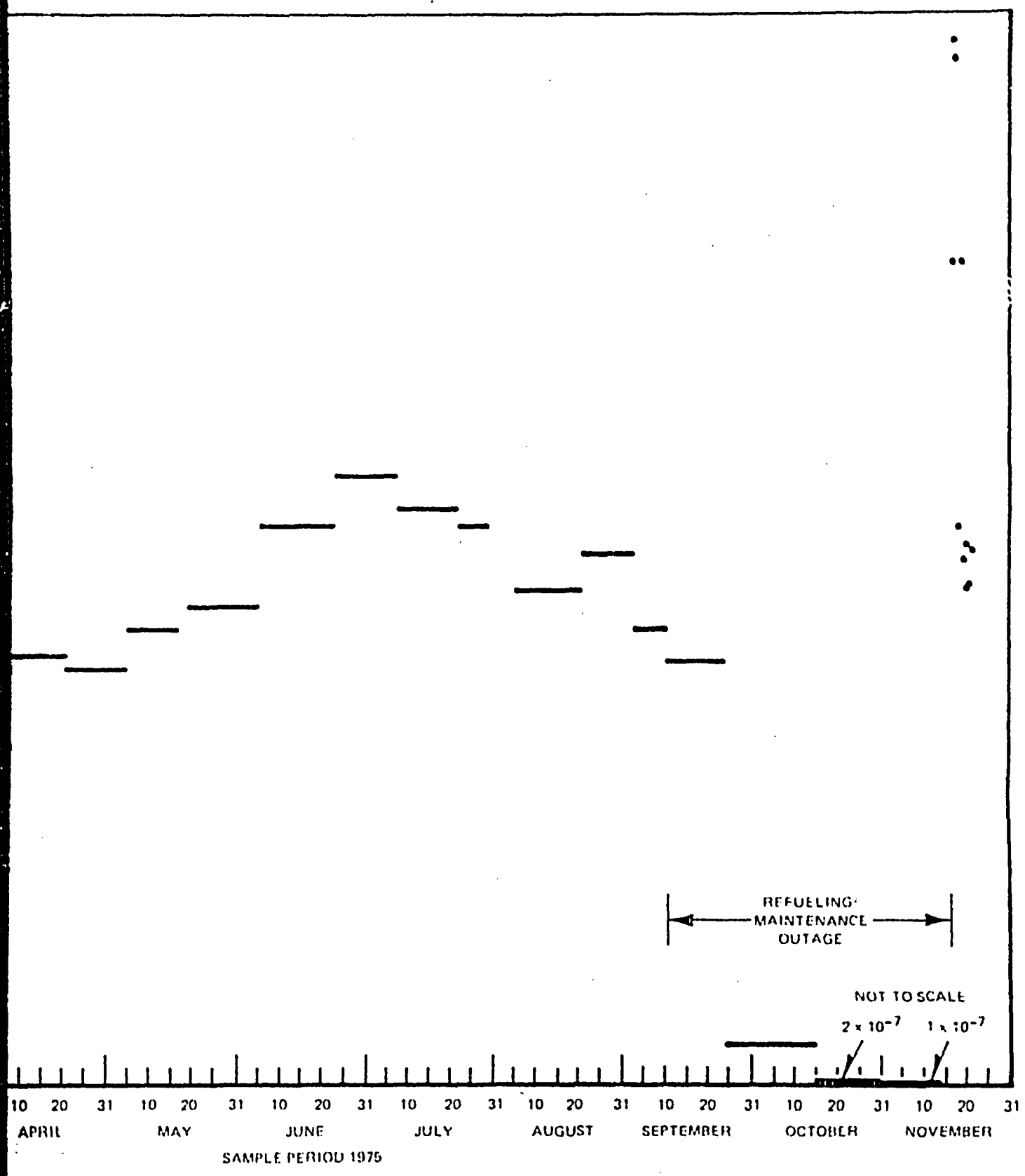
Figure 6-45. Normalized I-131 Release Rates, Radwaste Building Ventilation Exhaust at Monticello (1974 and 1975)
