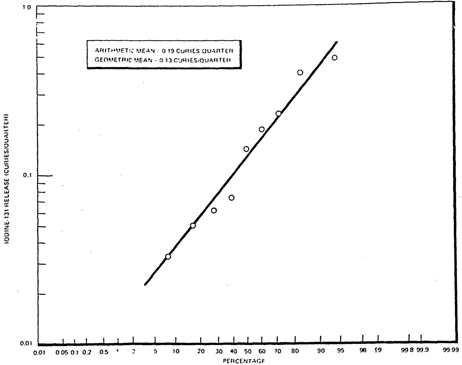
Figure 3-2 Accumulative Probability Distribution of Calendar Quarter I-131 Ventilation Releases, Pilgrim 1 (Reactor, Turbine and Radwaste Buildings, October 1974 to December 1976)
