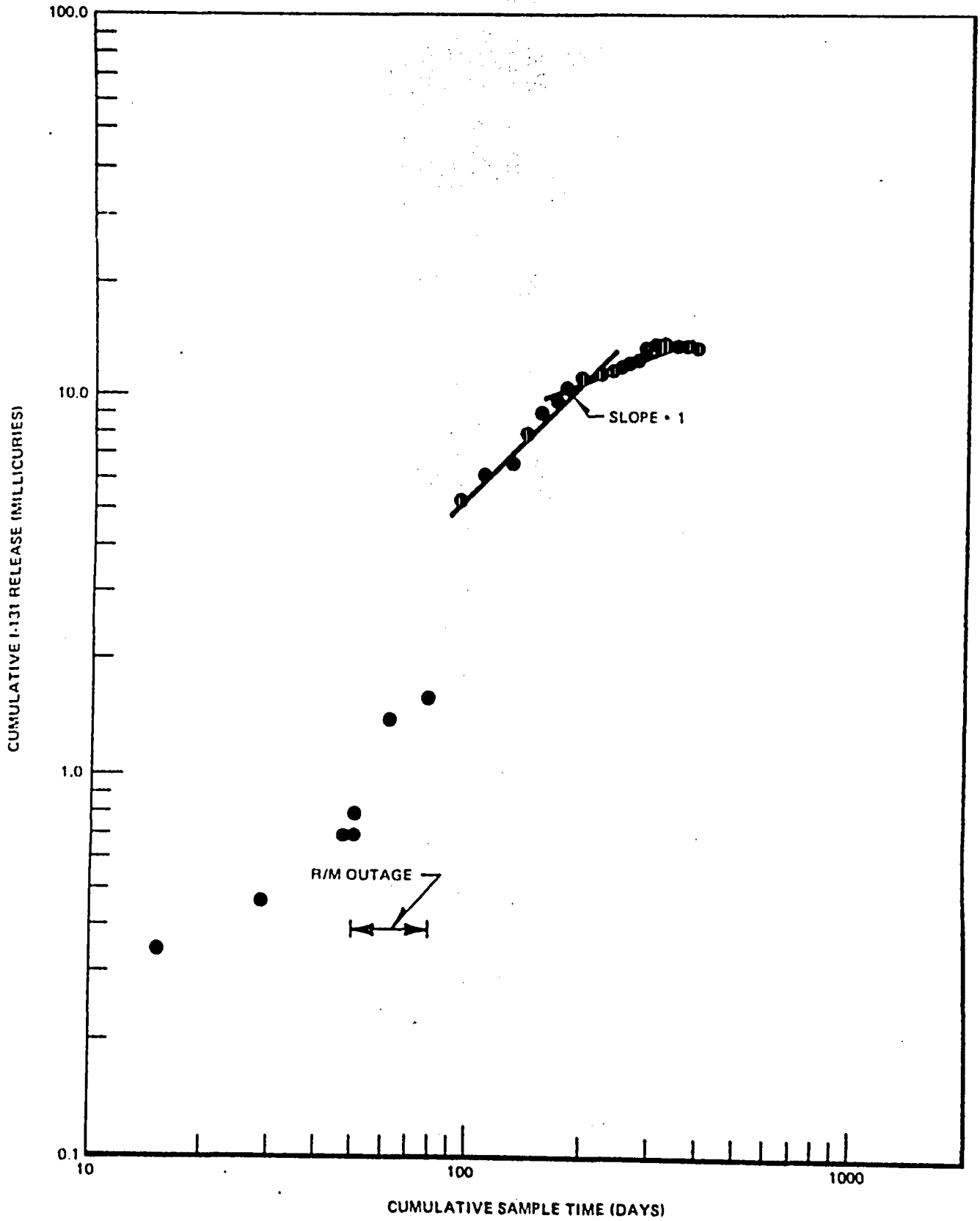
Figure 6-59. Cumulative Normalized I-131 Turbine Building Airborne Release at Monticello
