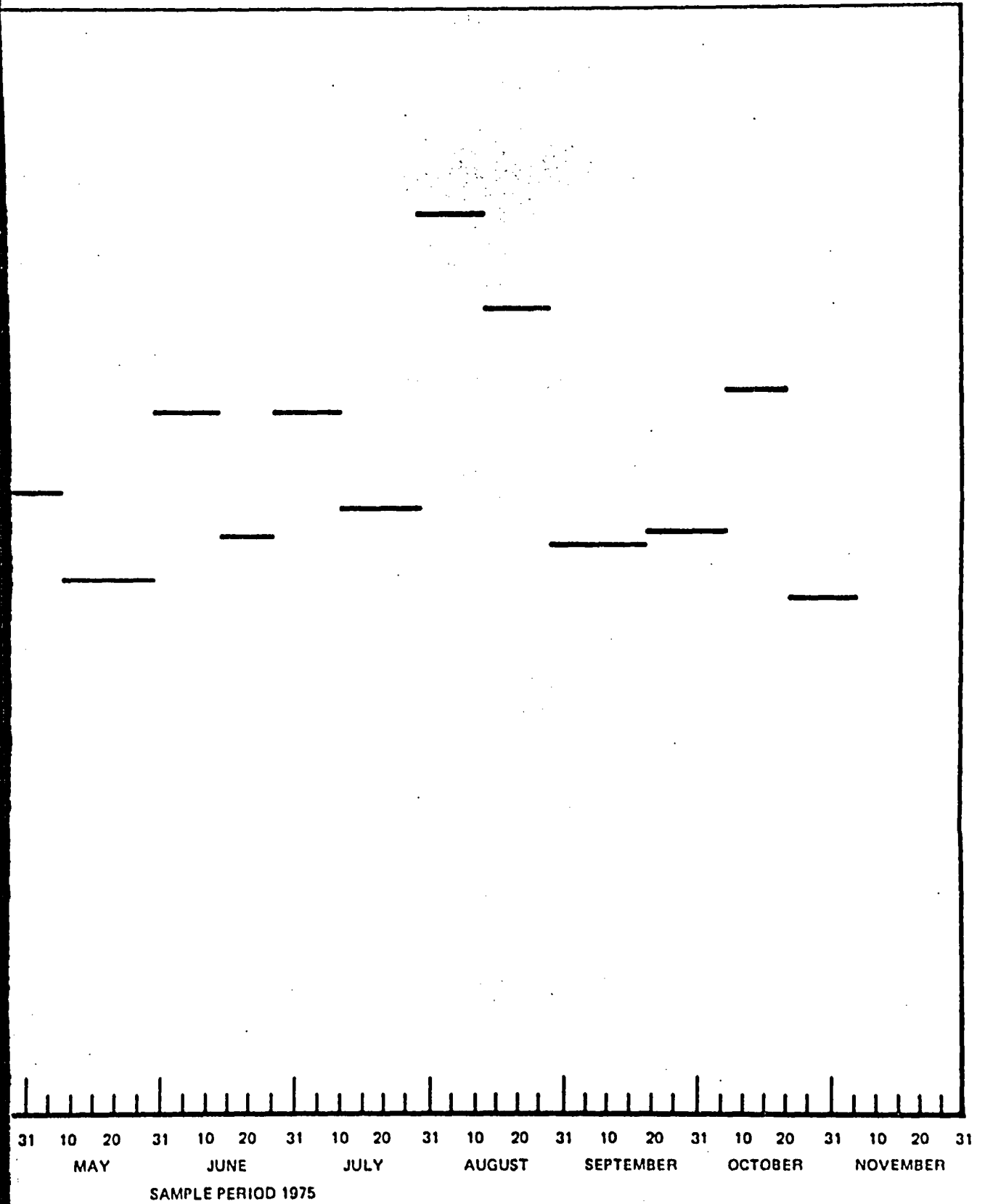
Figure 6-38. Normalized I-131 Release Rates, Reactor Building Ventilation Exhaust at Vermont Yankee (1974 and 1975)
