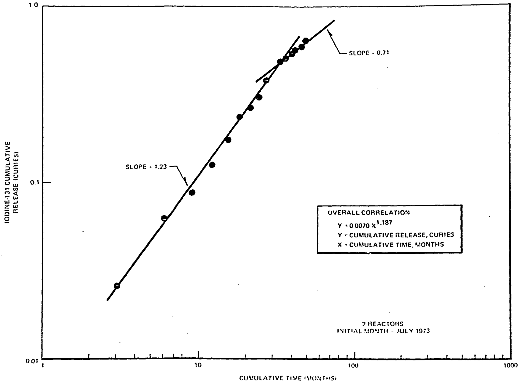
Figure 6.68. Trend Analysis of Quad Cities 1,2 Iodine-131 Airborne Releases of Reactor Building Ventilation Exhaust
