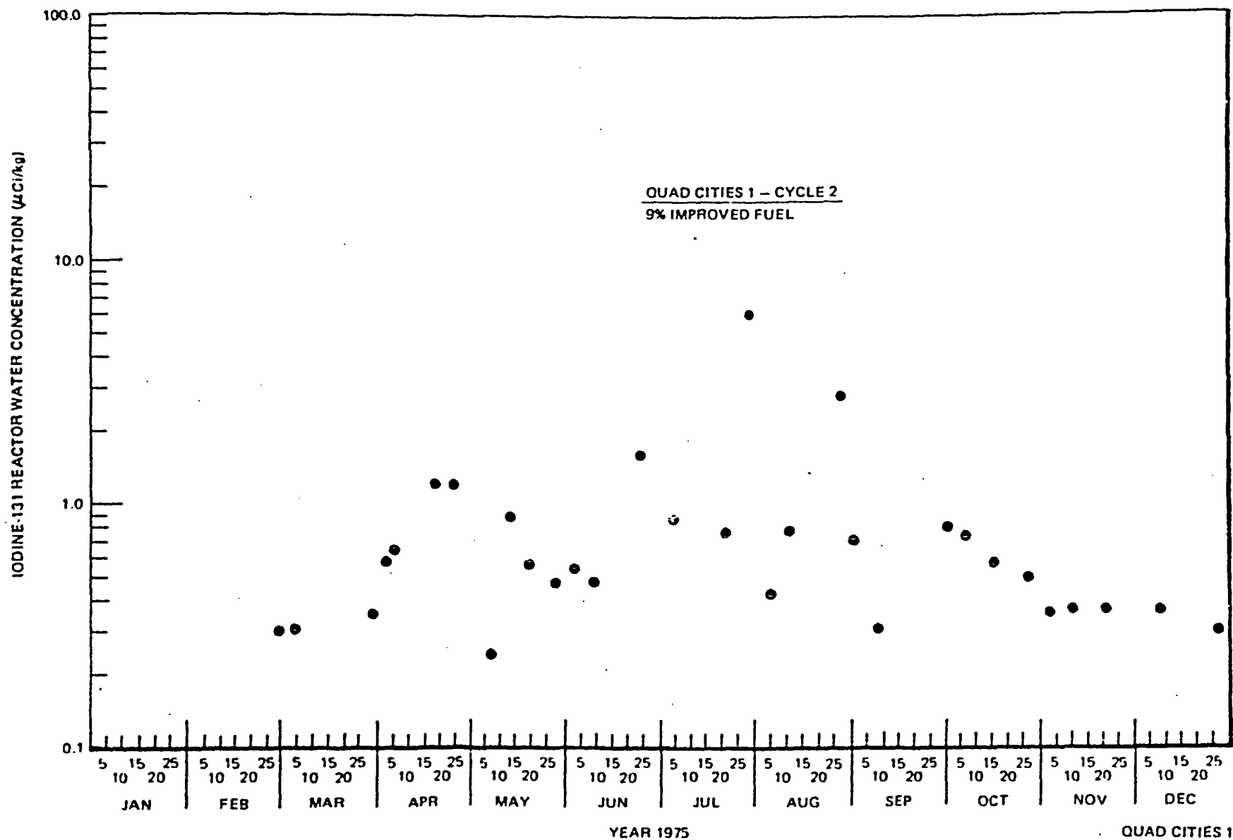
Figure 6-28. Iodine-131 Reactor Water Concentration at Quad Cities 1, 1975
