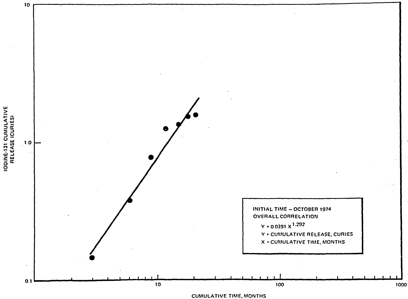
Figure 6.70. Trend Analysis of Pilgrim 1 Iodine-131 Airborne Releases from Reactor, Turbine and Radwaste Buildings
