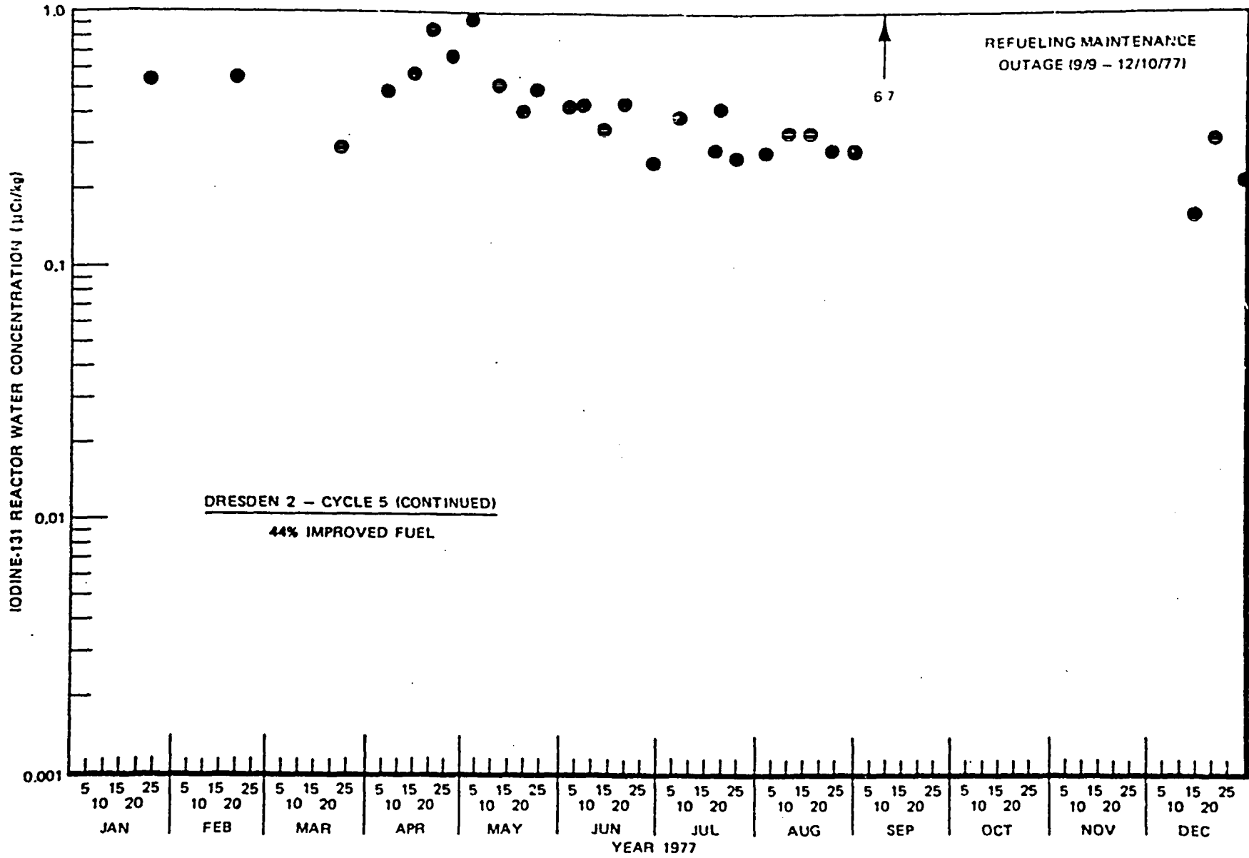
Figure 6-8b. Iodine-131 Reactor Water Concentration at Dresden 2, 1977
