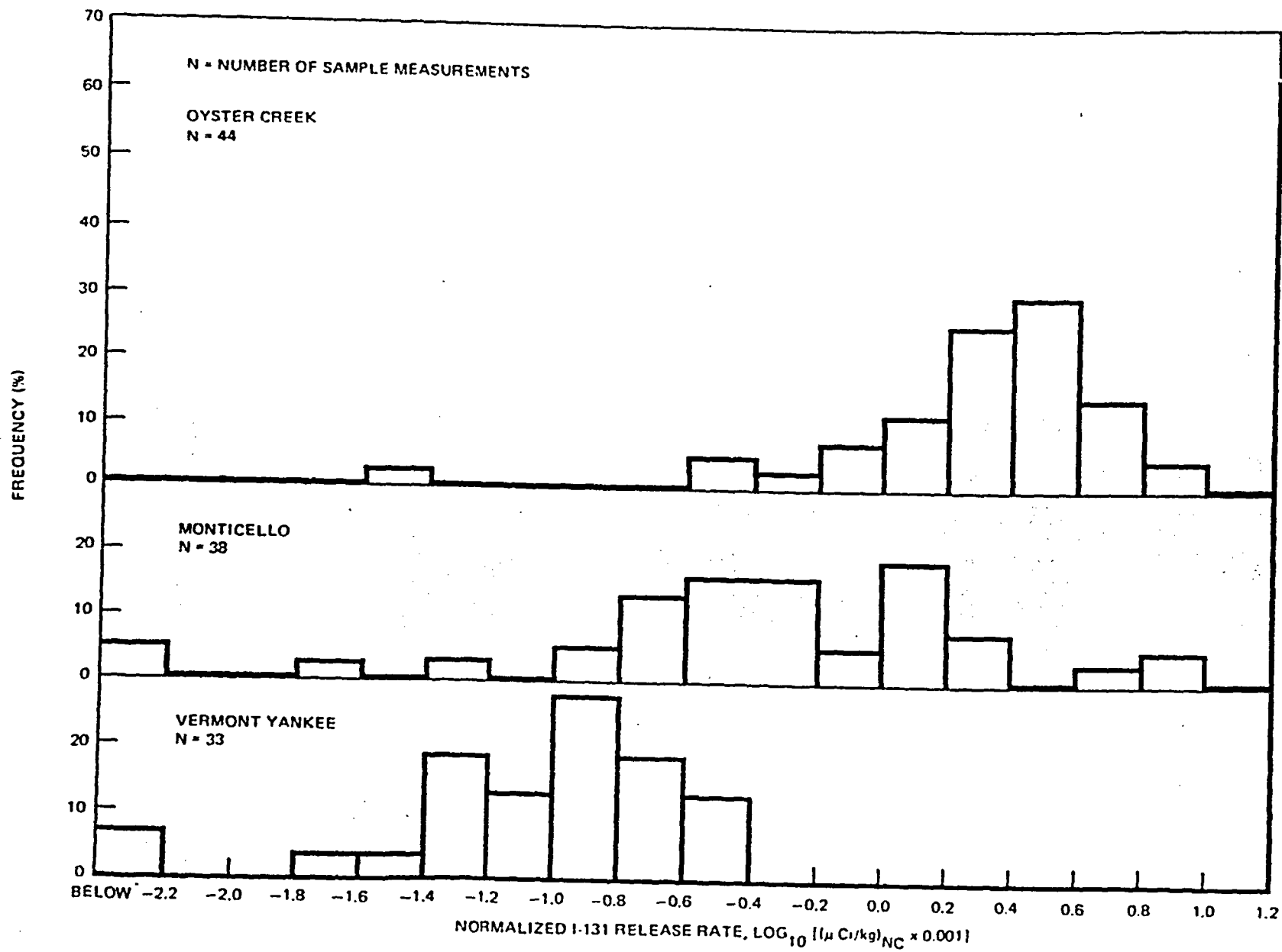
Figure 6-53. Frequency Polygons of Normalized I-131 Turbine Building Airborne Release Rates Adjusted to I-131 Carryover of 1 Percent
