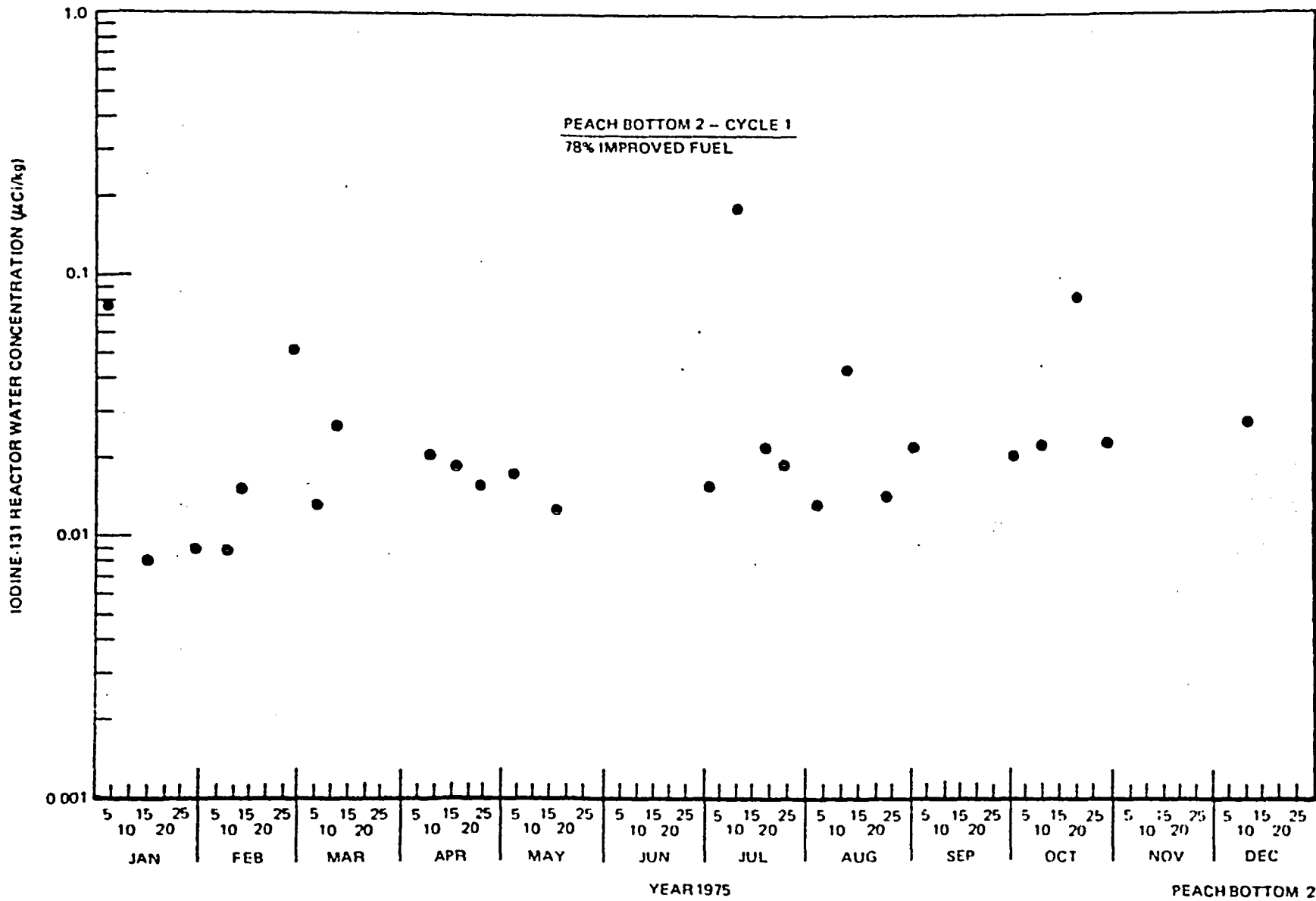
Figure 6-22. Iodine-131 Reactor Water Concentration at Peach Bottom 2, 1975
