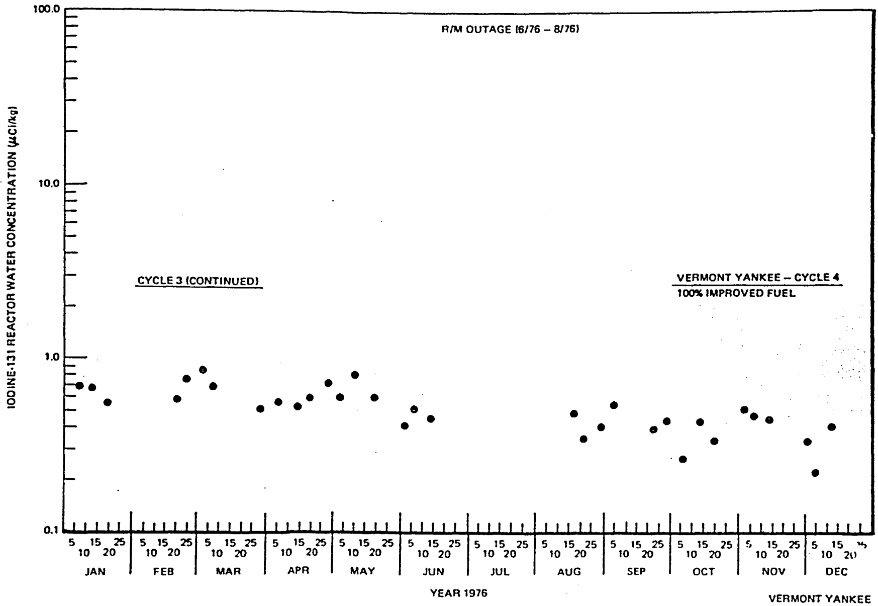
Figure 6-34. Iodine-131 Reactor Water Concentration at Vermont Yankee, 1976
