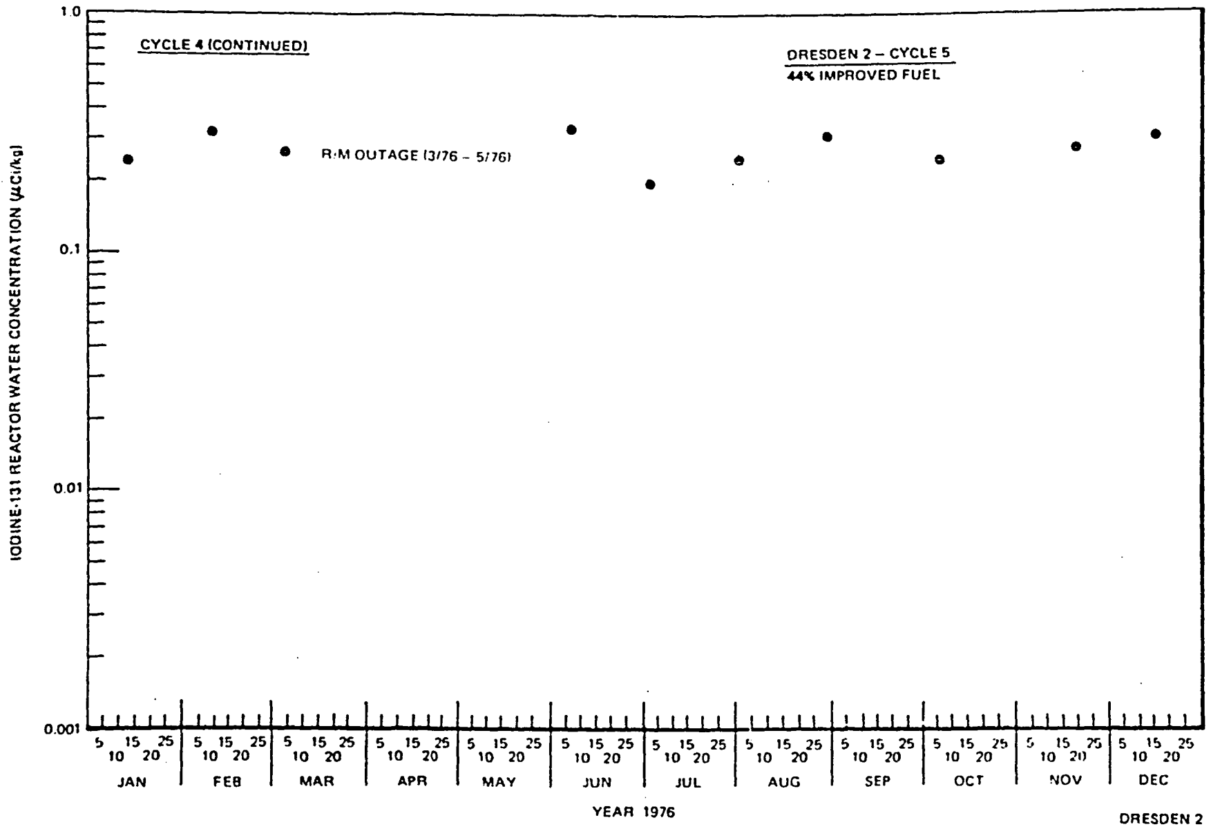
Figure 6-8a. Iodine-131 Reactor Water Concentration at Dresden 2, 1976
