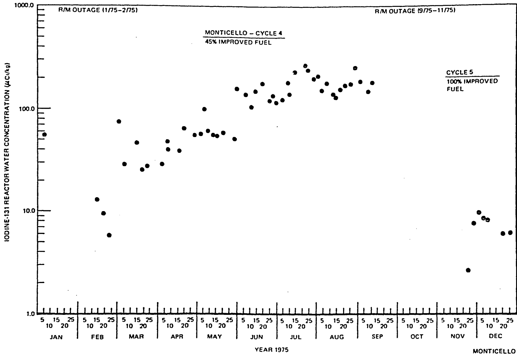
Figure 6-16. Iodine-131 Reactor Water Concentration at Monticello, 1975
