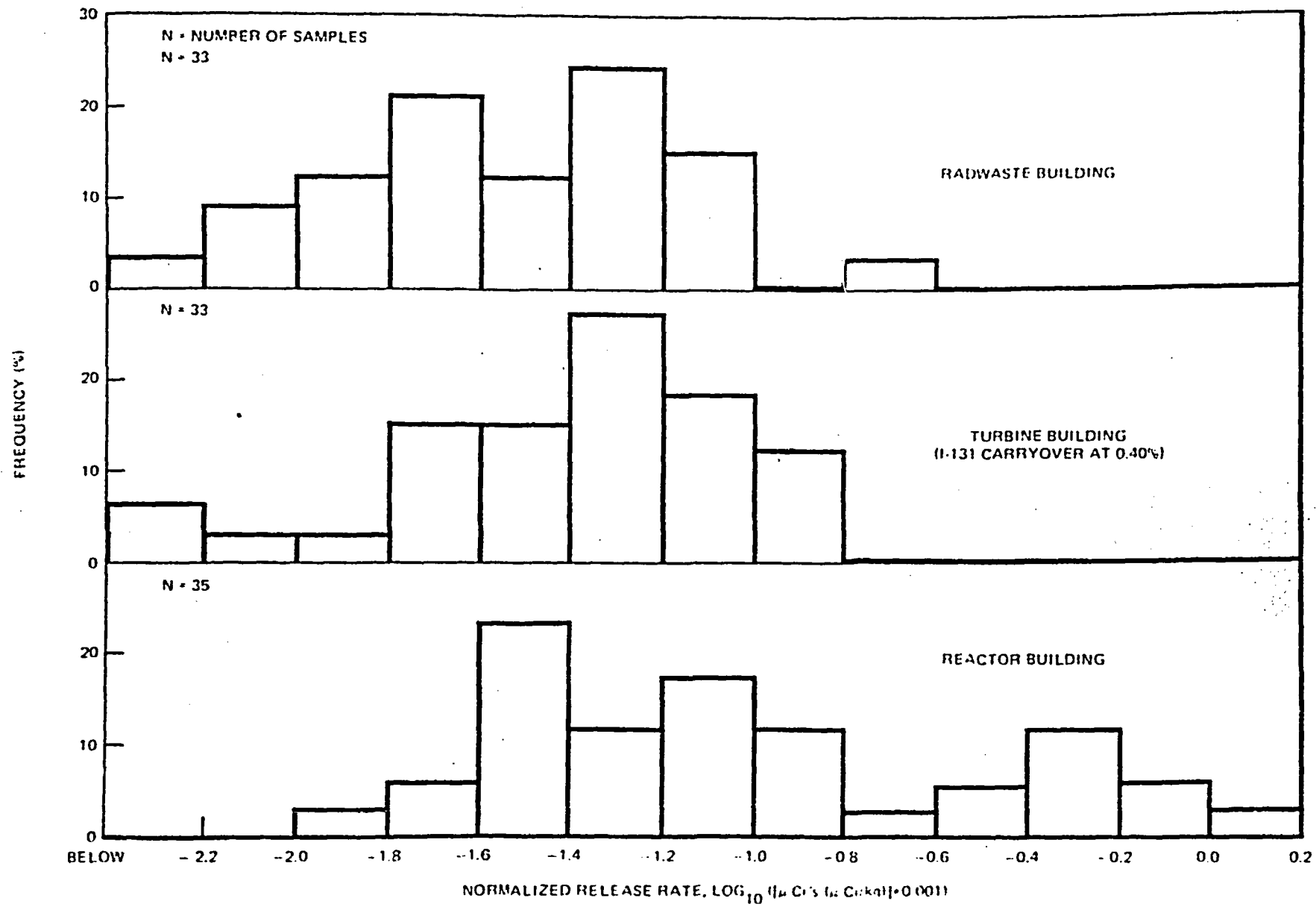
Figure 6-50. Frequency Polygons of Normalized I-131 Airborne Release Rates From Reactor, Turbine and Radwaste Buildings at Vermont Yankee
