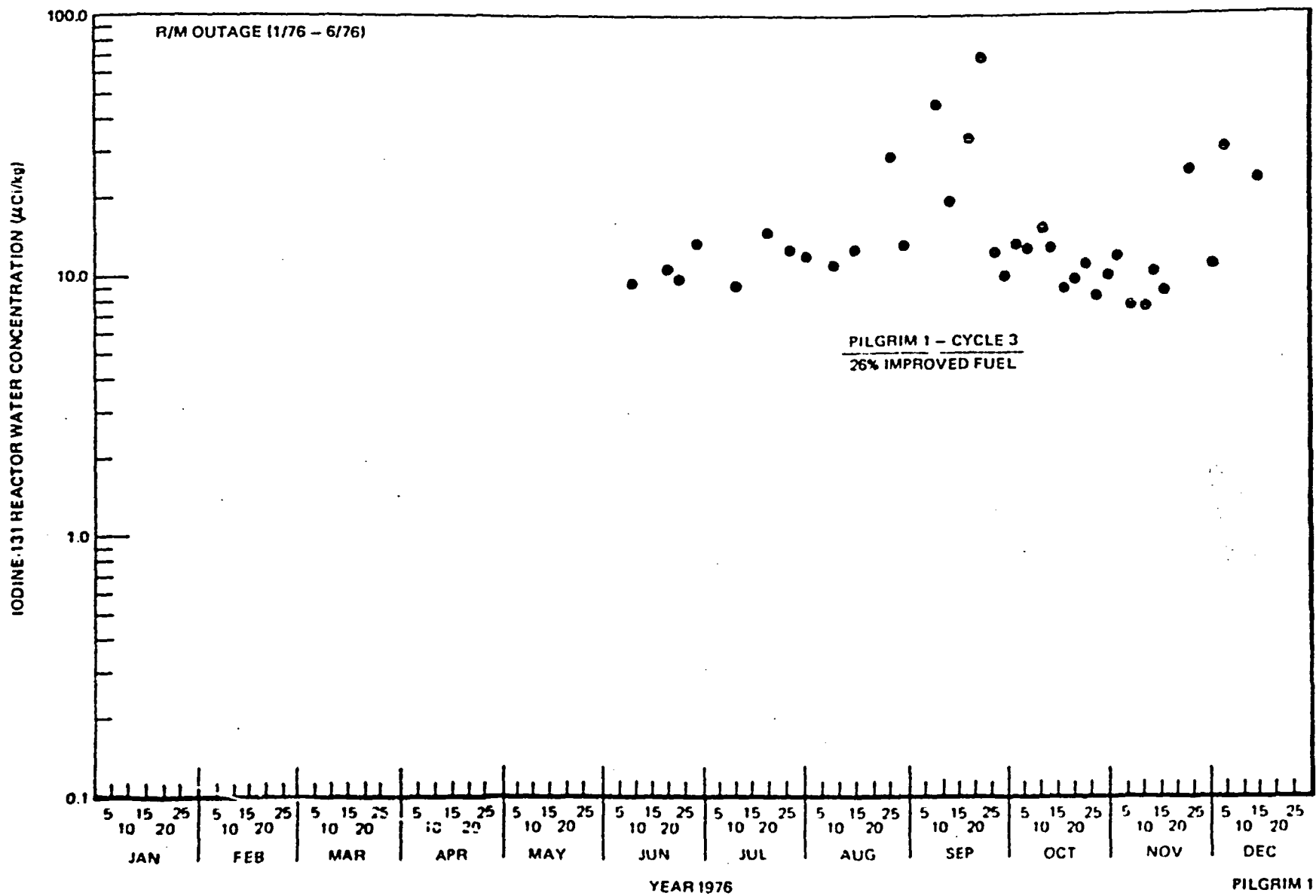
Figure 6-27. Iodine-131 Reactor Water Concentration at Pilgrim 1, 1976
