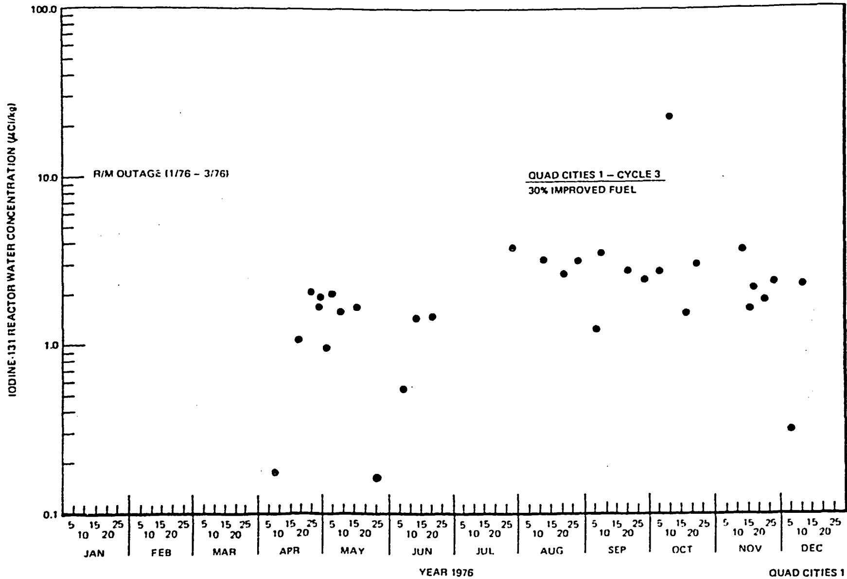
Figure 6-29. Iodine-131 Reactor Water Concentration at Quad Cities 1, 1976
