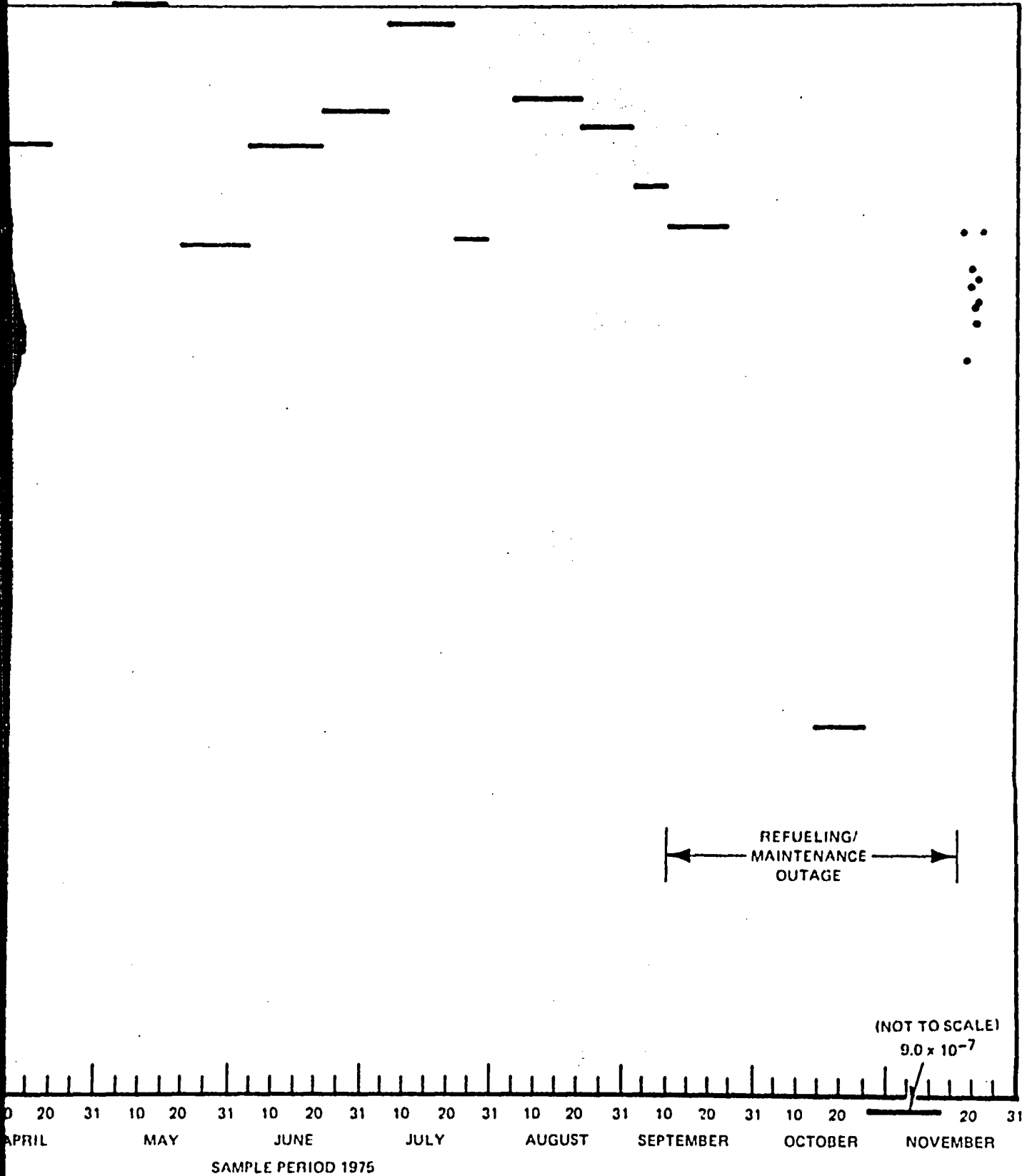
Figure 6-39. Normalized I-131 Release Rates, Reactor Building Ventilation Exhaust at Monticello (1974 and 1975)
