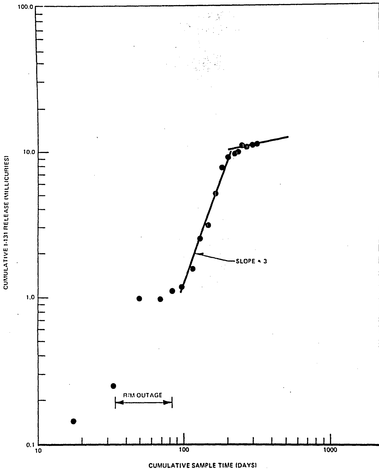
Figure 6-65. Cumulative Normalized I-131 Radwaste Building Airborne Release at Oyster Creek (1975 - 1976)
