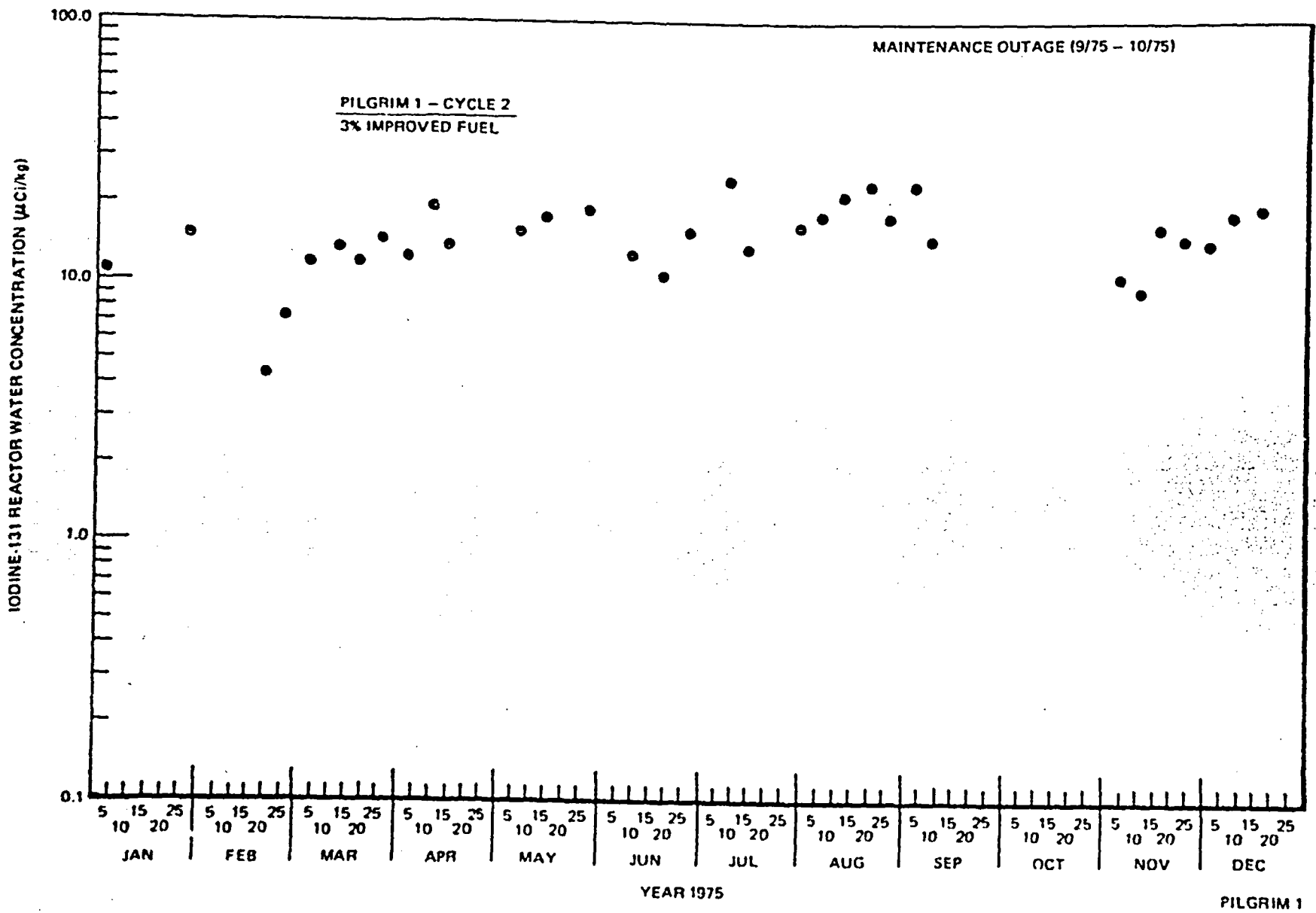
Figure 6-26. Iodine-131 Reactor Water Concentration at Pilgrim 1, 1975
