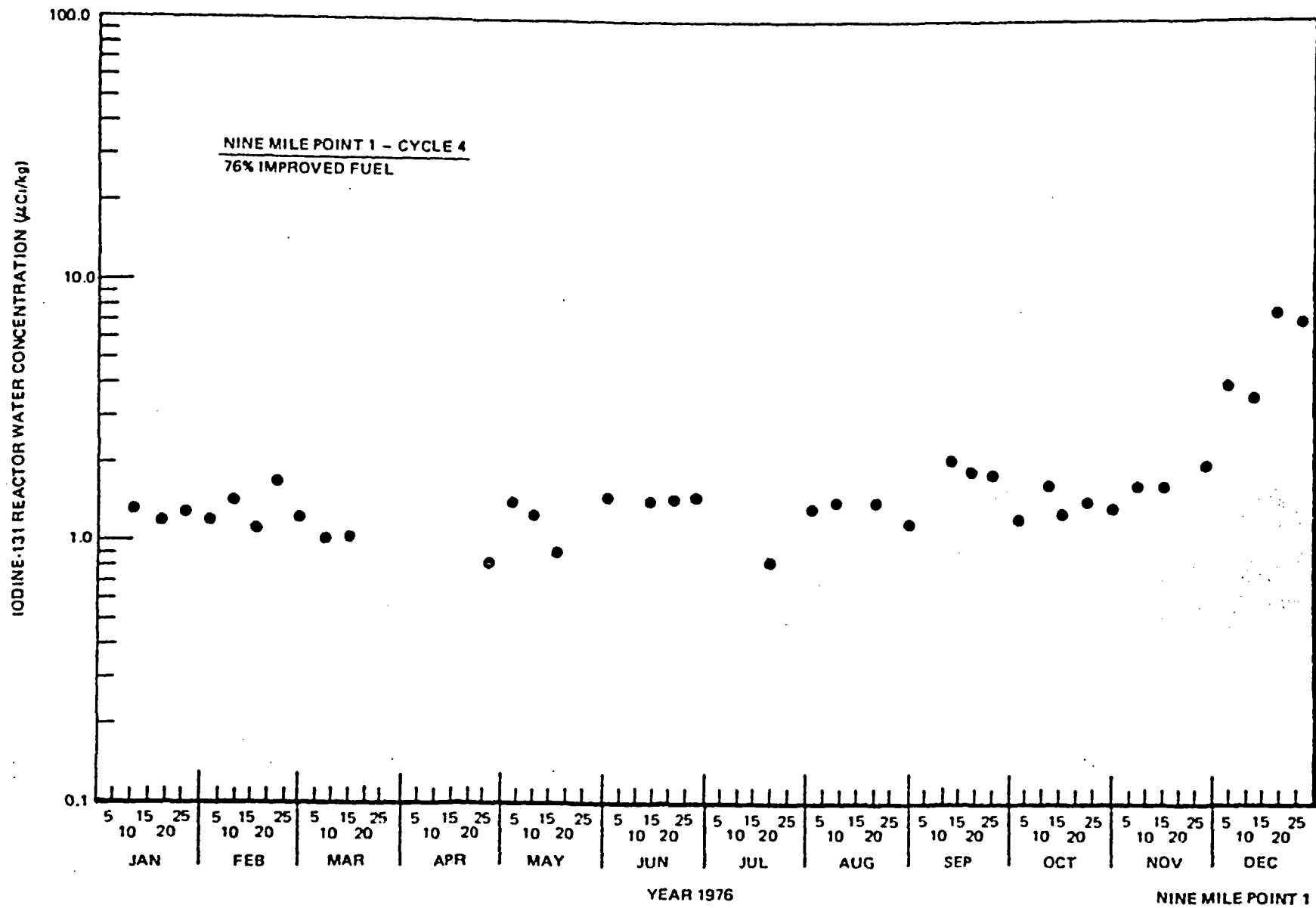
Figure 6-19. Iodine-131 Reactor Water Concentration at Nine Mile Point 1, 1976
