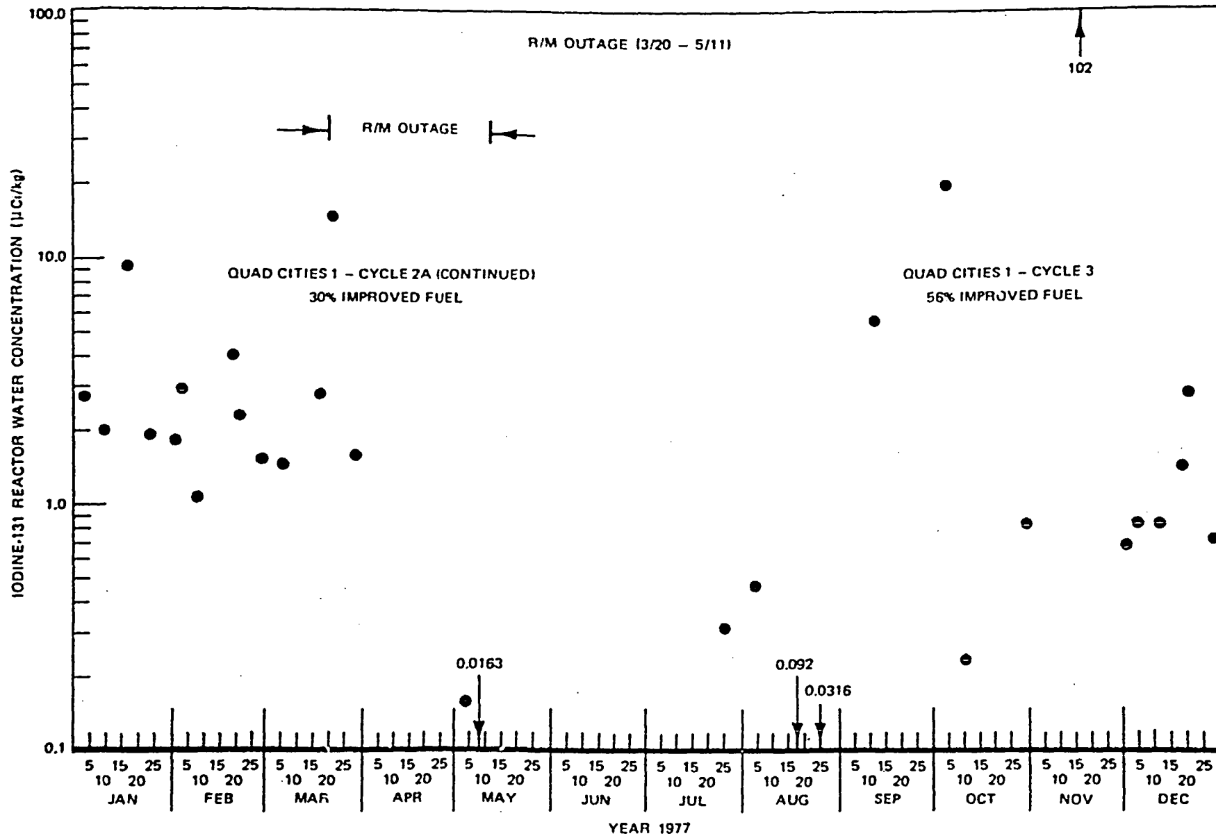
Figure 6-29a. Iodine-131 Reactor Water Concentration at Quad Cities 1, 1977
