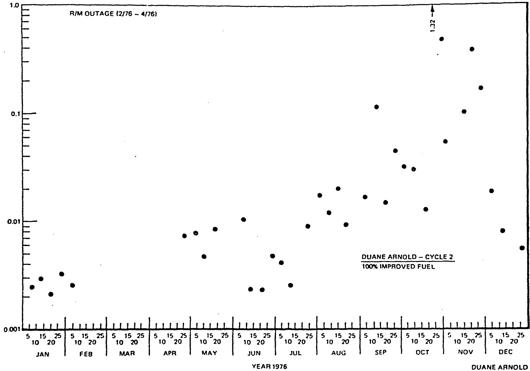
Figure 6-10a. Iodine-131 Reactor Water Concentration at Duane Arnold, 1976
