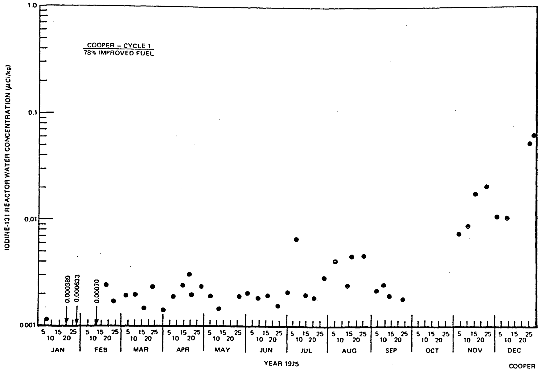
Figure 6-7. Iodine-131 Reactor Water Concentration at Cooper, 1975
