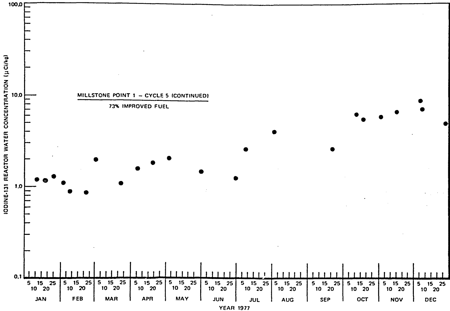
Figure 6-14a. Iodine-131 Reactor Water Concentration at Millstone Point 1, 1977
