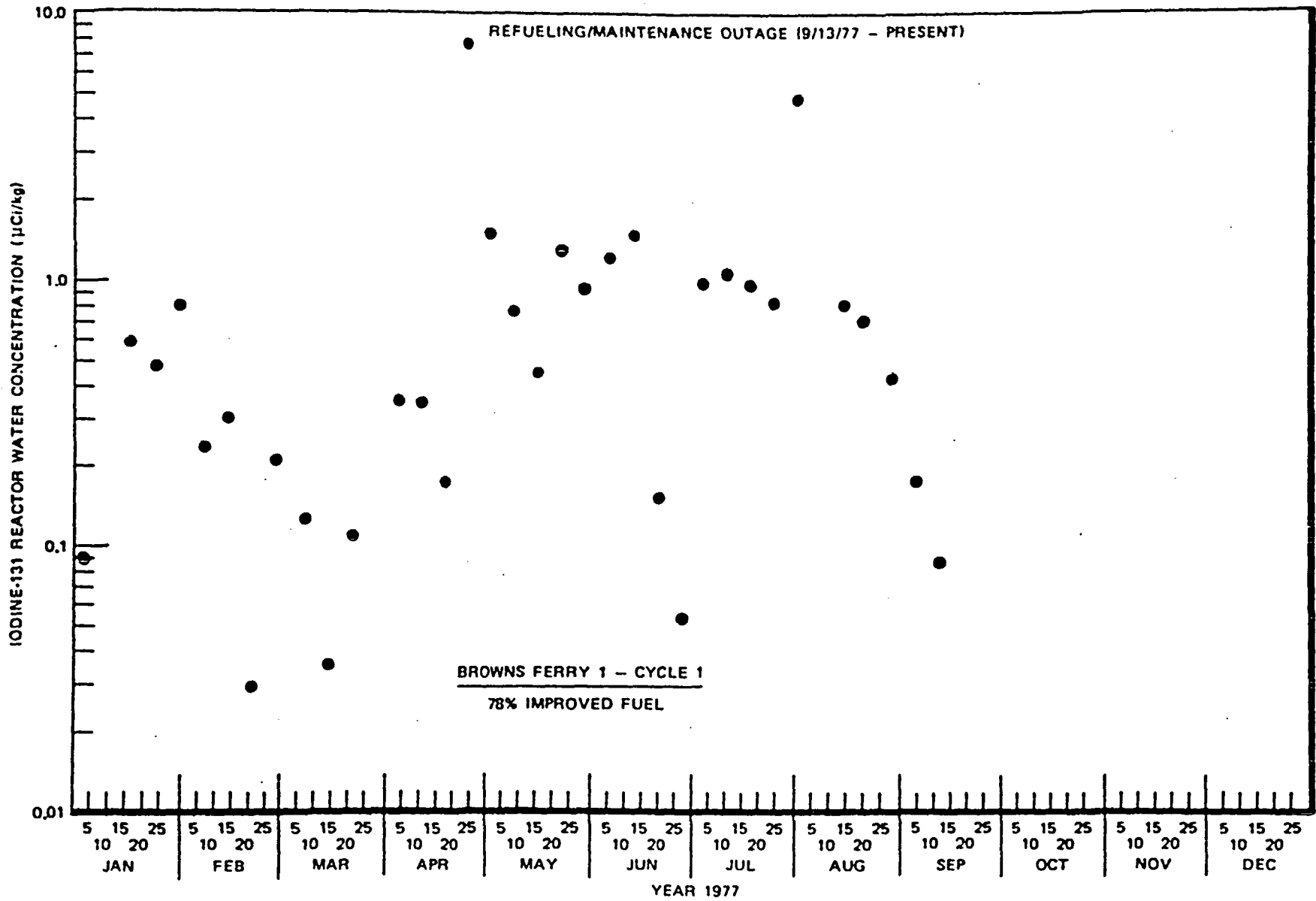
Figure 6-2. Iodine-131 Reactor Water Concentration at Browns Ferry 1, 1977
