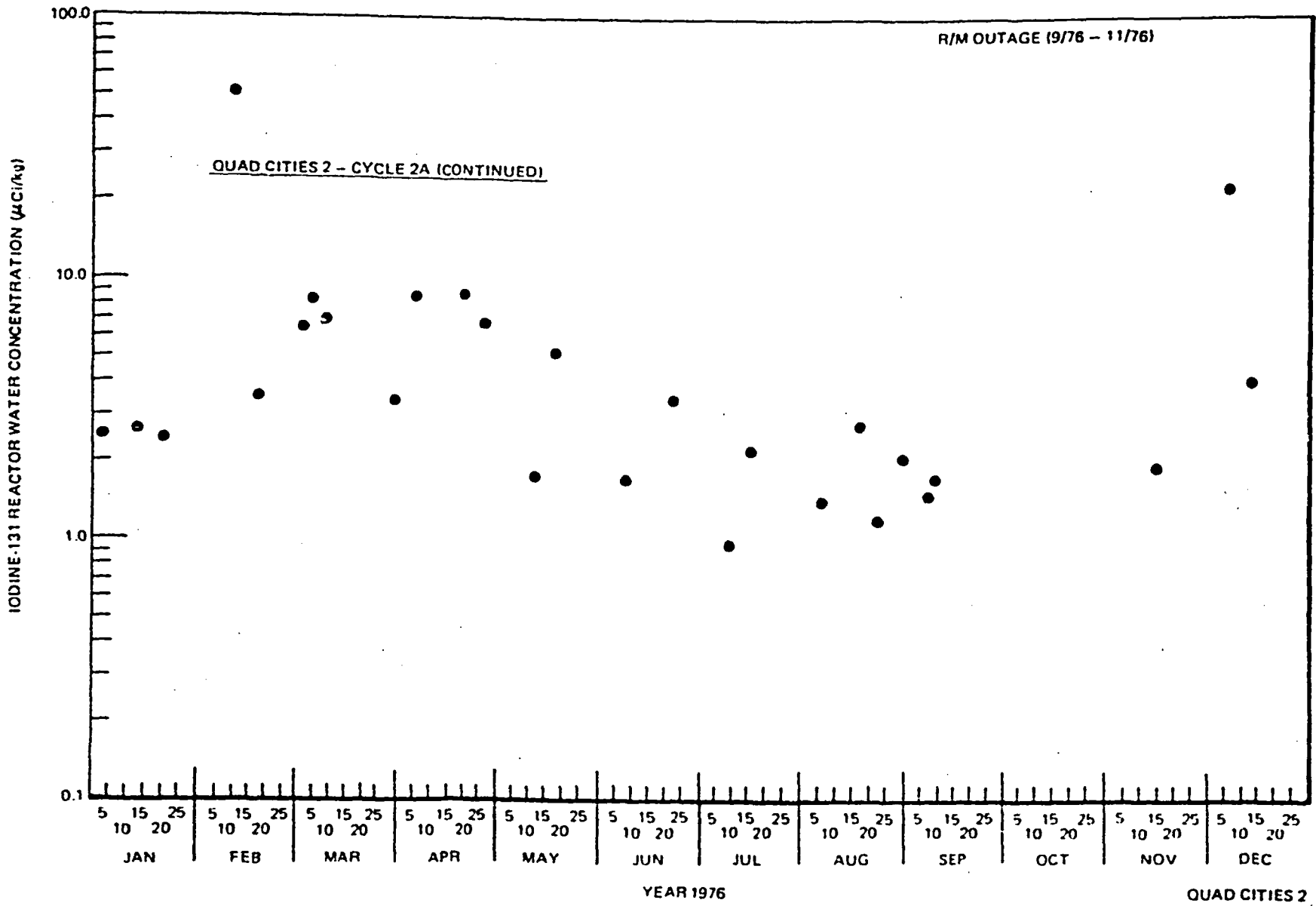
Figure 6-31. Iodine-131 Reactor Water Concentration at Quad Cities 2, 1976
