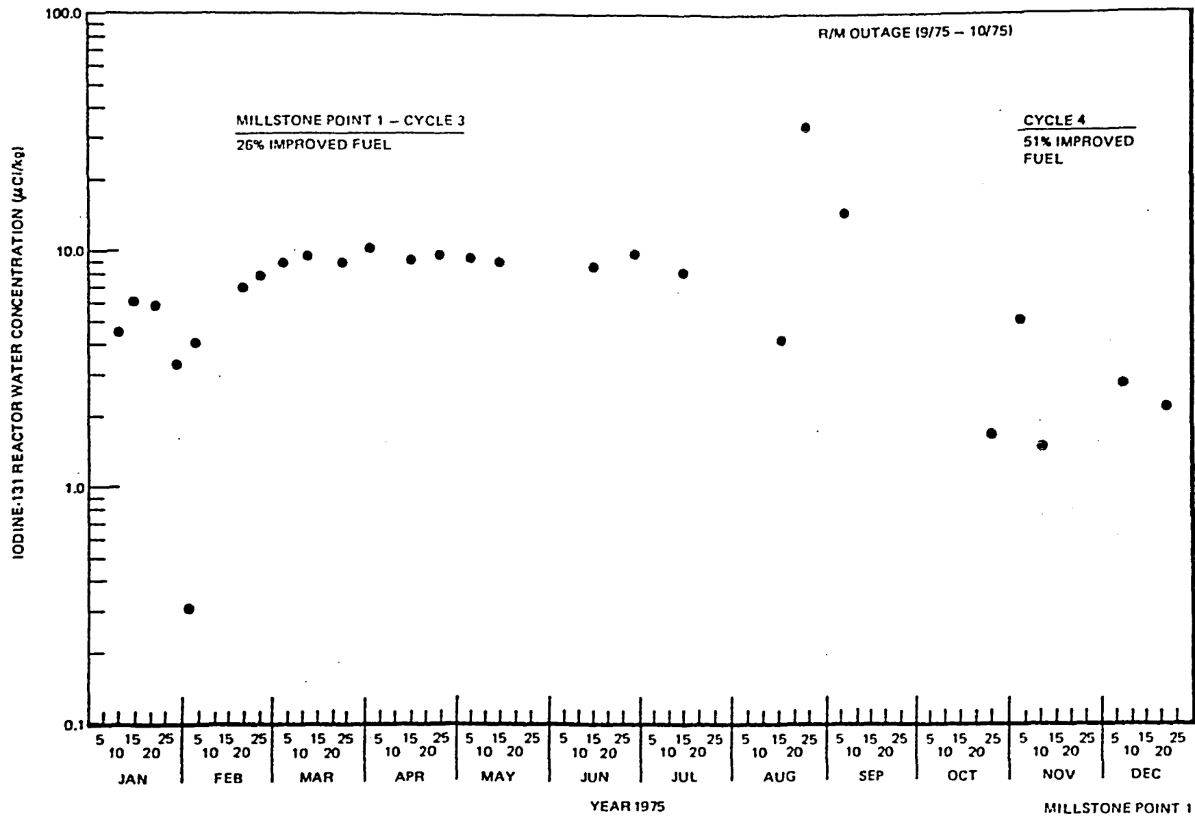
Figure 6-13. Iodine-131 Reactor Water Concentration at Millstone Point 1, 1975
