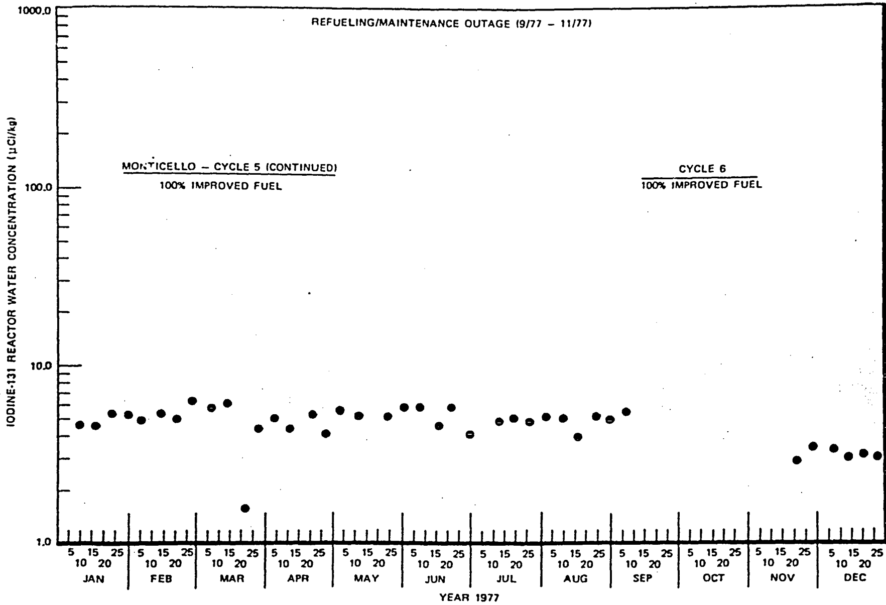
Figure 6-17a. Iodine-131 Reactor Water Concentration at Monticello, 1977
