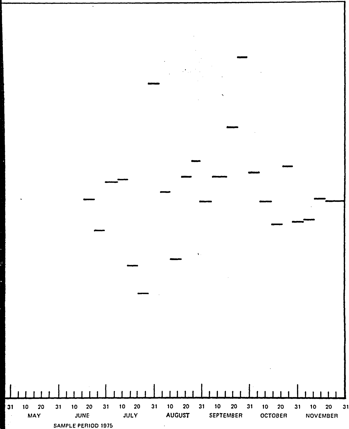
Figure 6-46. Normalized I-131 Release Rates, Radwaste Building Ventilation Exhaust at Oyster Creek (1975 and 1976)
