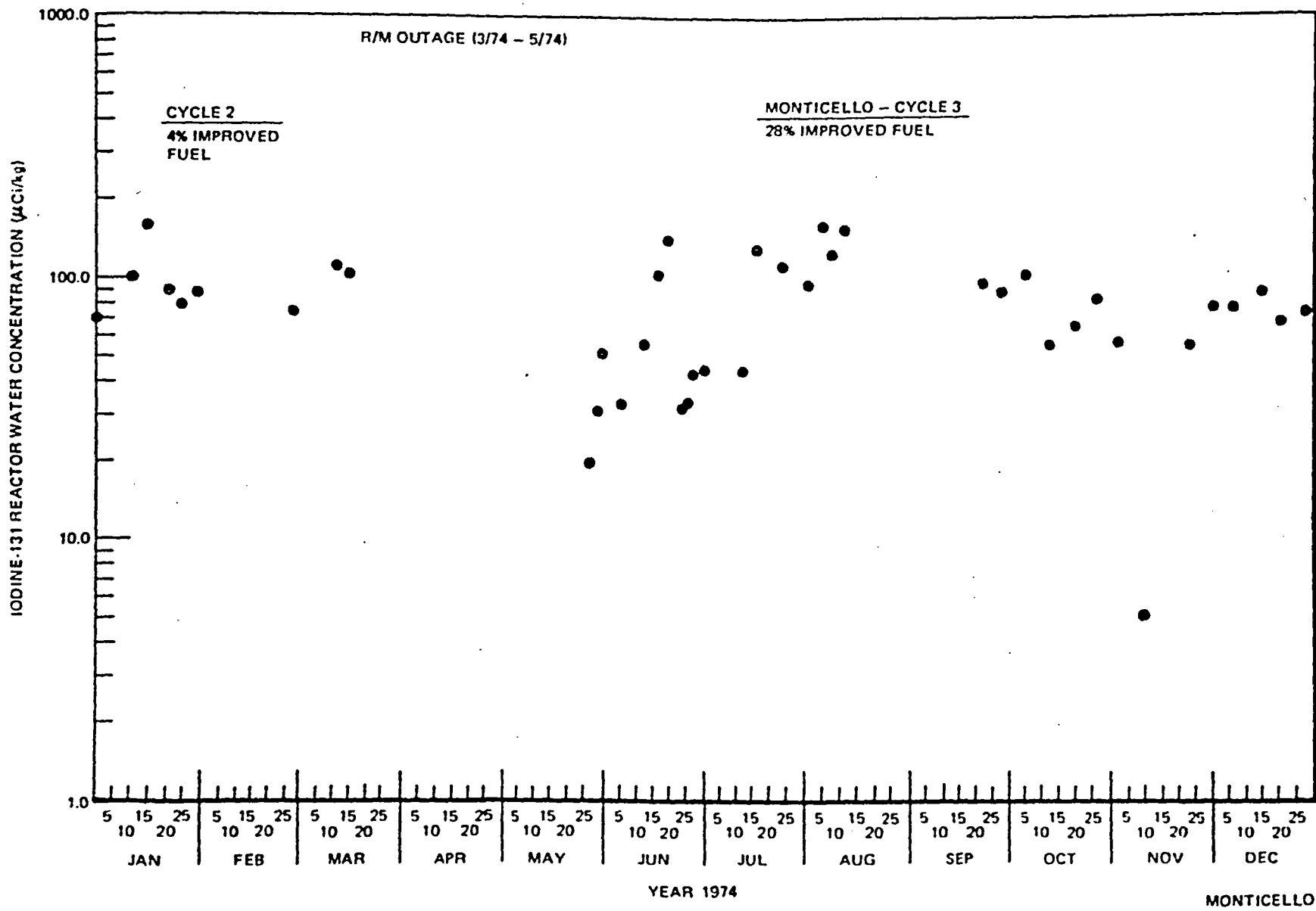
Figure 6-15. Iodine-131 Reactor Water Concentration at Monticello, 1974
