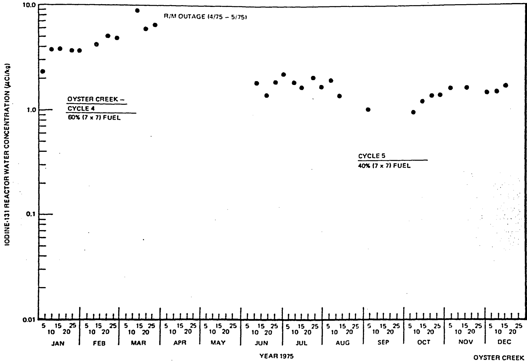
Figure 6-20. Iodine-131 Reactor Water Concentration at Oyster Creek, 1975
