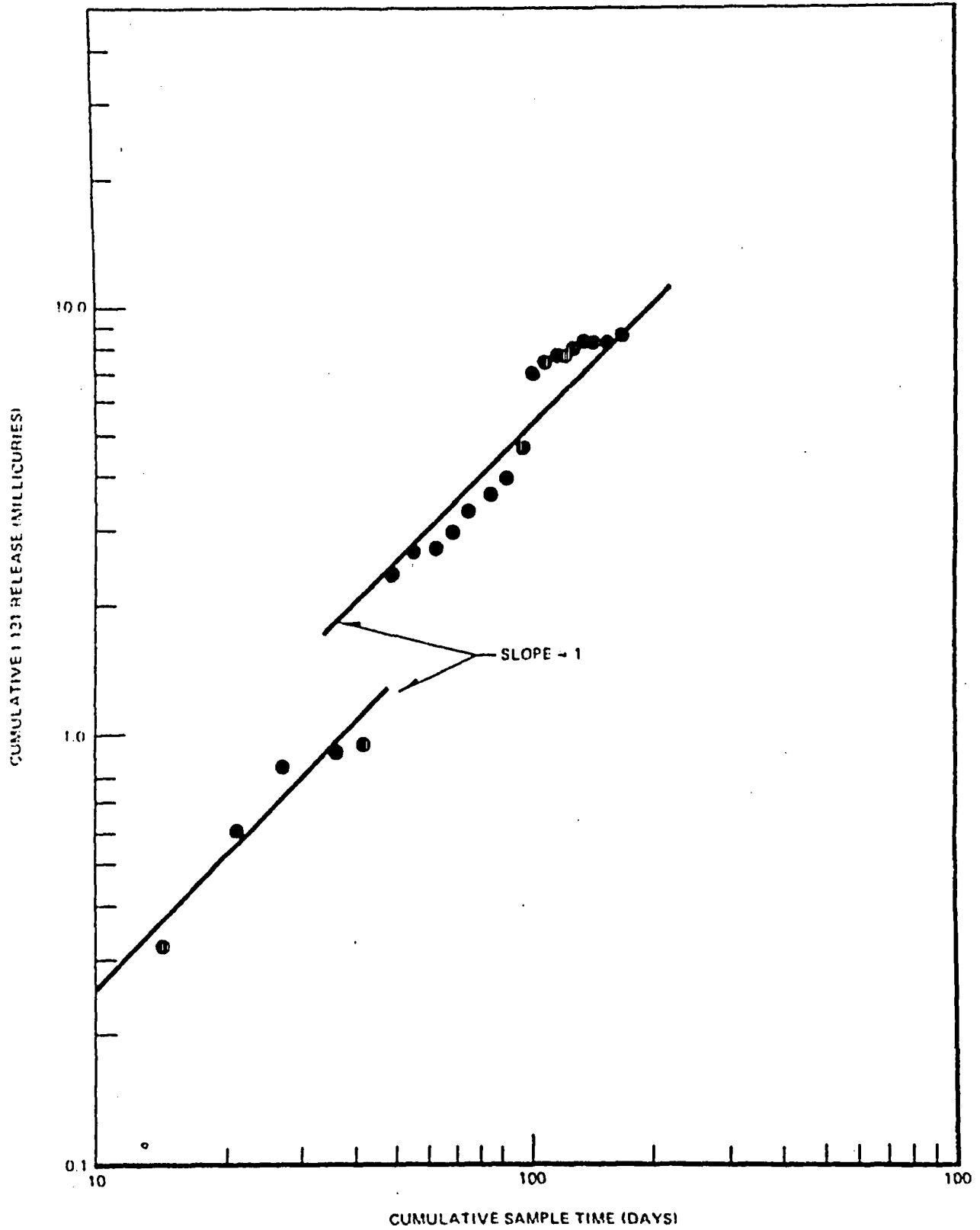
Figure 6-66. Cumulative Normalized I-131 Radwaste Building Airborne Release at Oyster Creek (1976)
