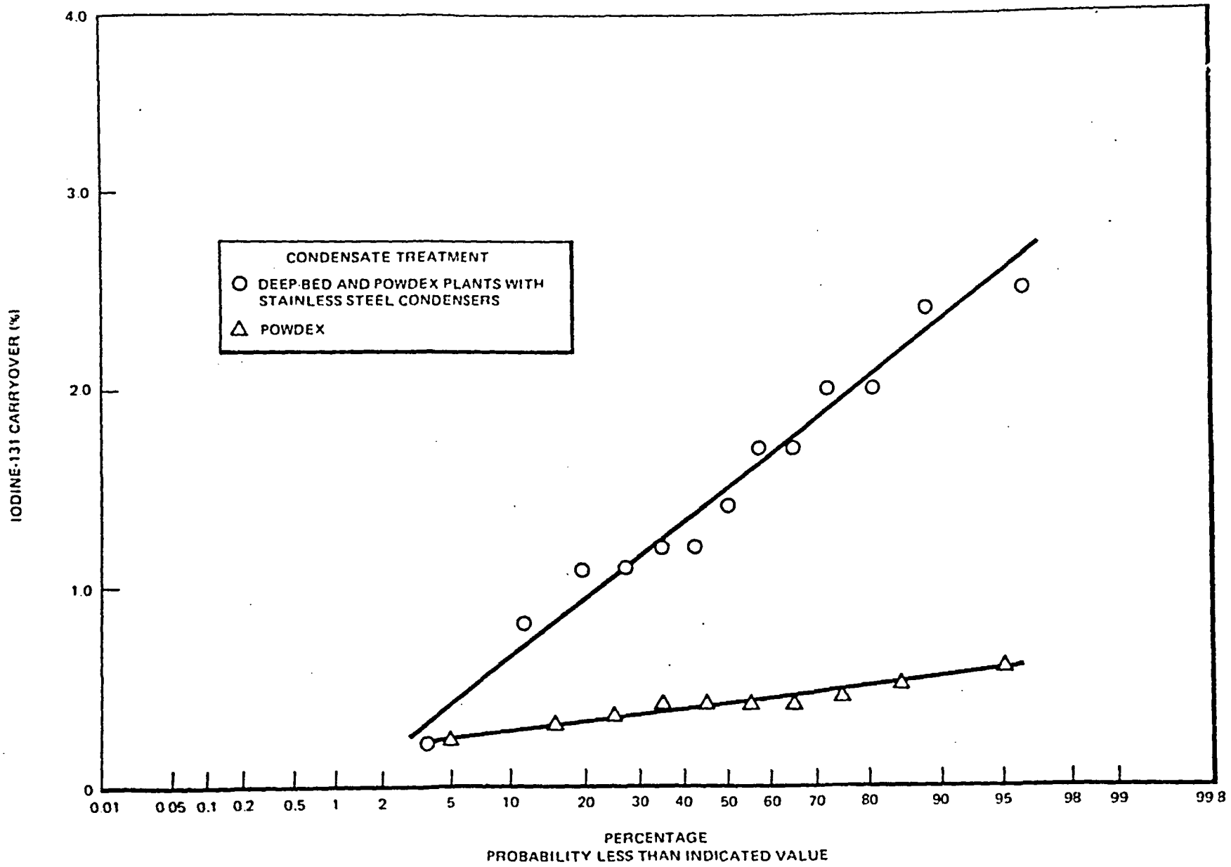
Figure 6-1. Normal Probability Distribution of Iodine-131 Carryover in BWR's
