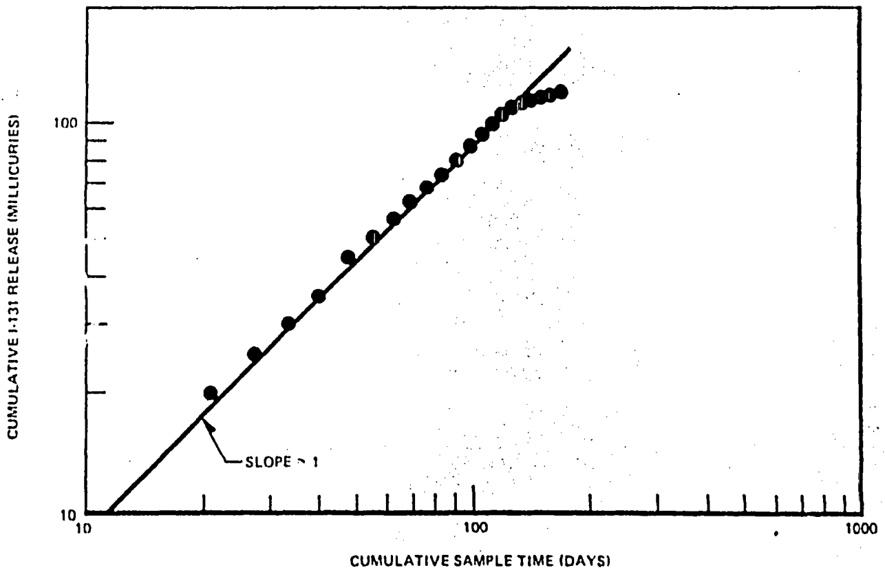
Figure 6-64. Cumulative Normalized I-131 Turbine Building Airborne Release at Oyster Creek (1976)
