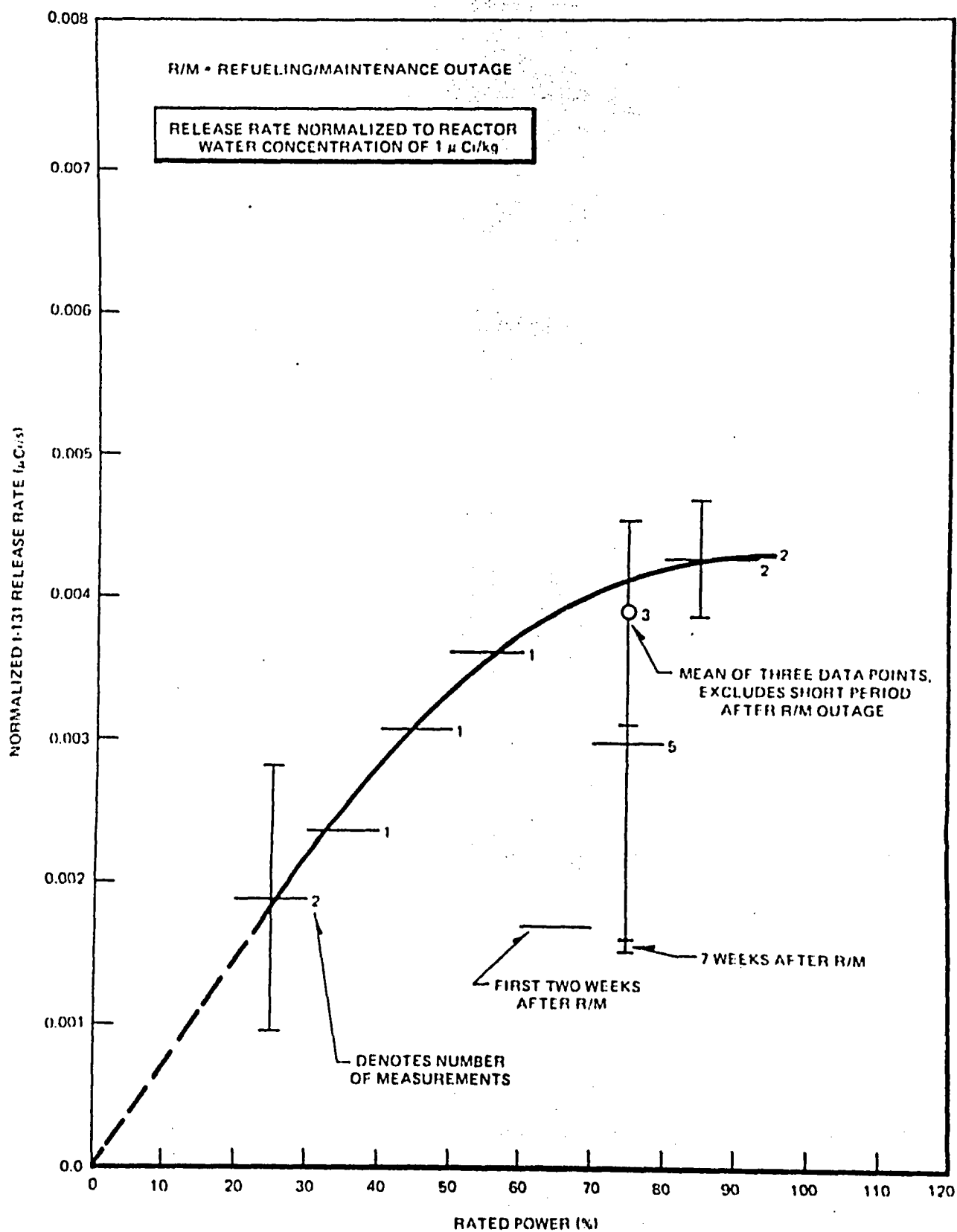
Figure 6-54. Normalized I-131 Turbine Building Airborne Release Rates and Reactor Power at Oyster Creek
