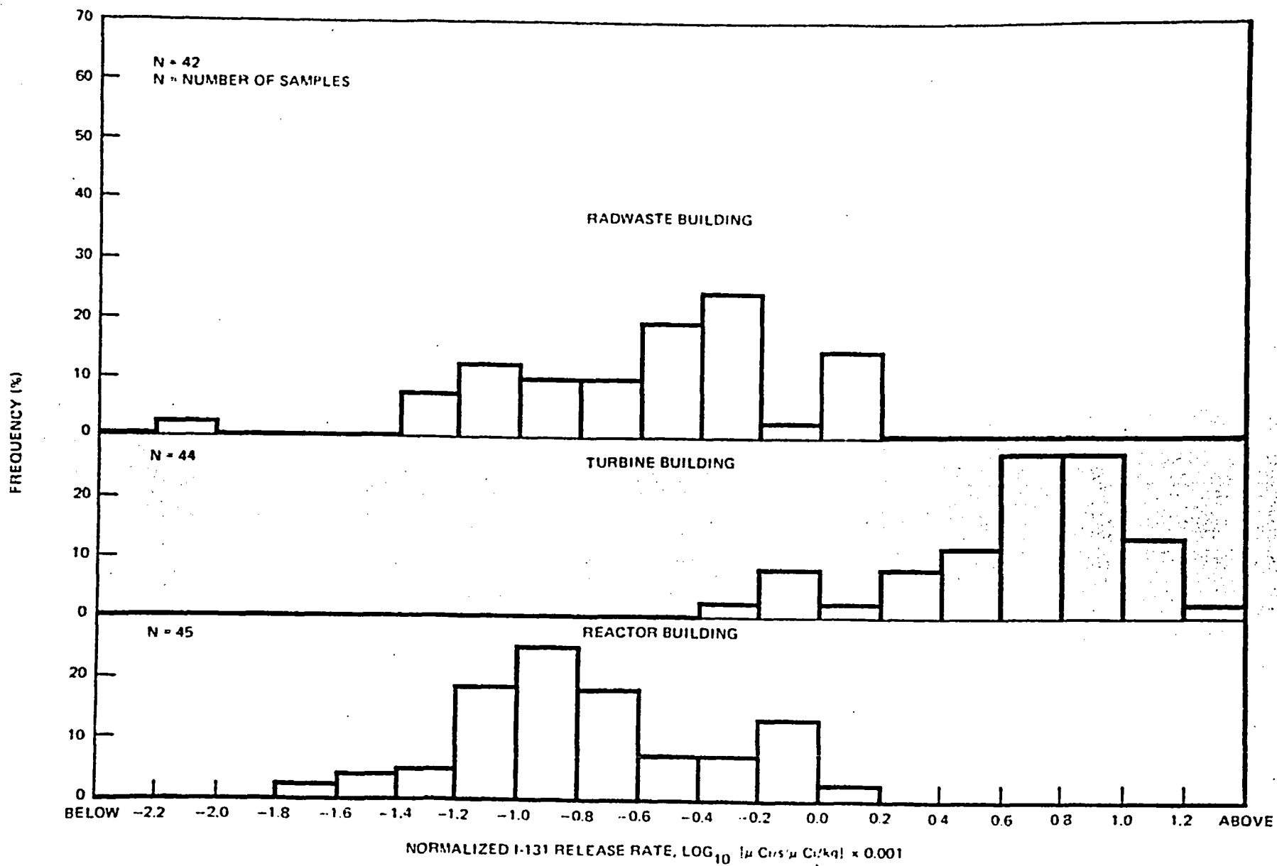
Figure 6-52. Frequency Polygons of Normalized I-131 Airborne Release Rates From Reactor, Turbine and Radwaste Buildings at Oyster Creek
