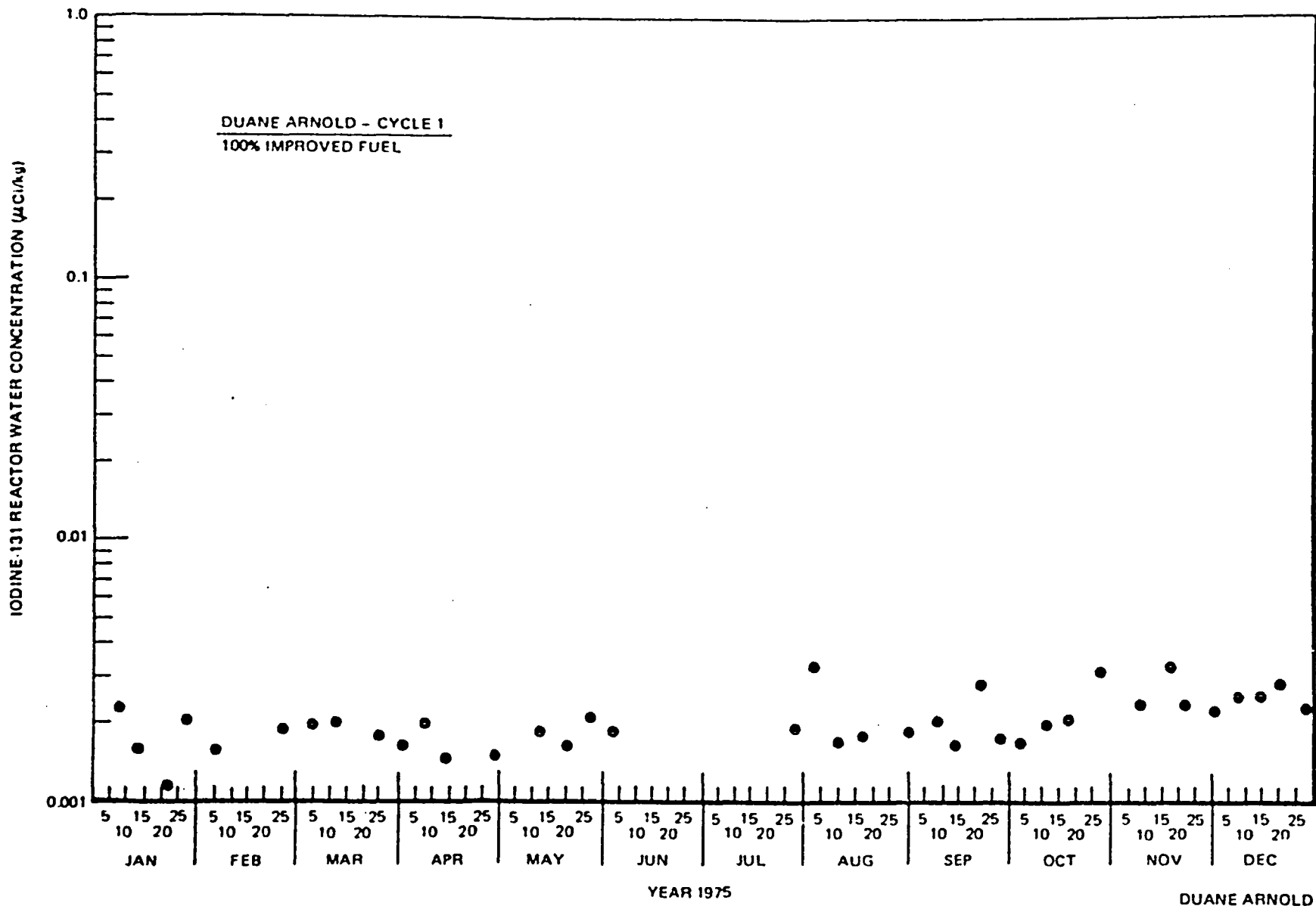
Figure 6-10. Iodine-131 Reactor Water Concentration at Duane Arnold, 1975
