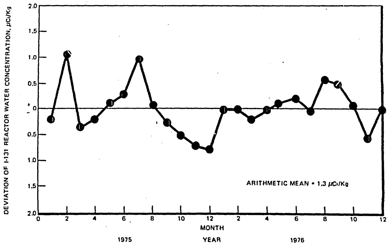
Figure 6-36. Variation of Median I-131 Reactor Water Concentration in Domestic BWR's for 1975 and 1976
