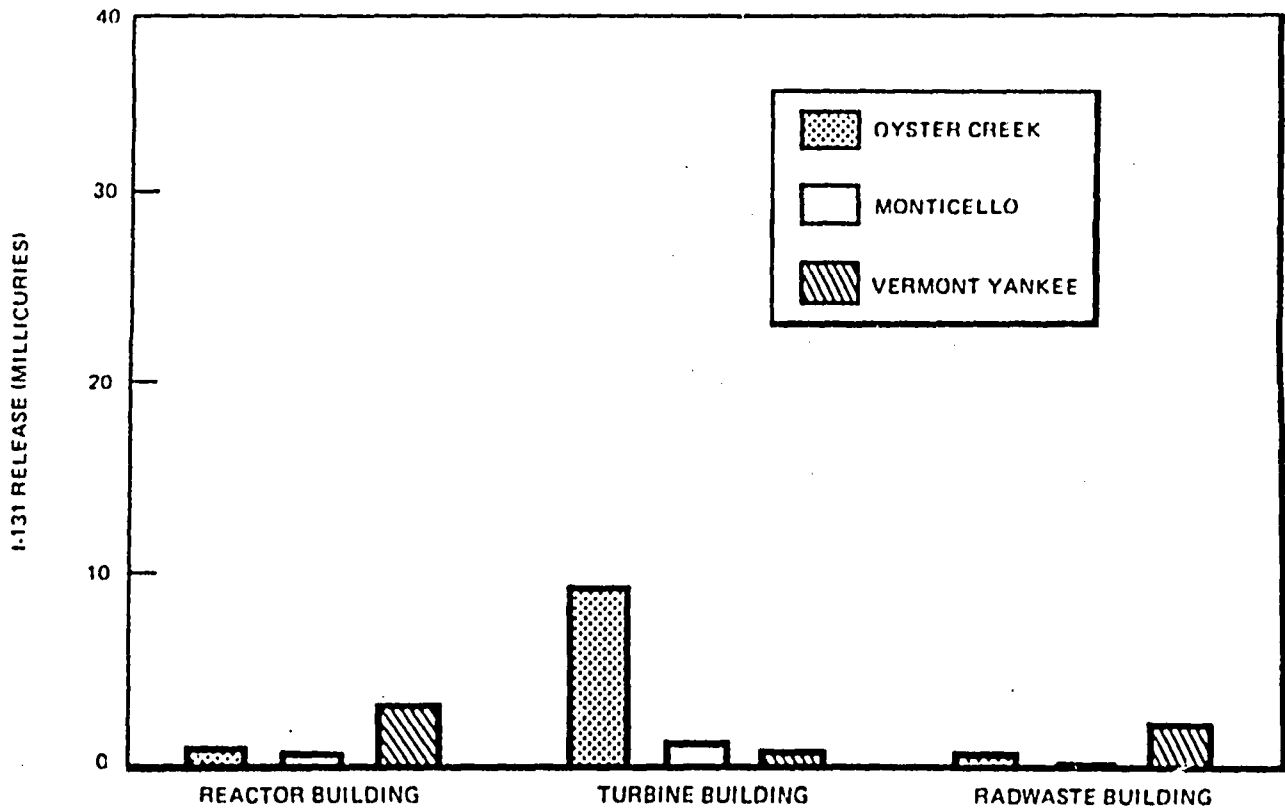
Figure 6-49. Bar Graph of Normalized I-131 Airborne Releases at Three BWRs for One Refueling/Maintenance Outage
