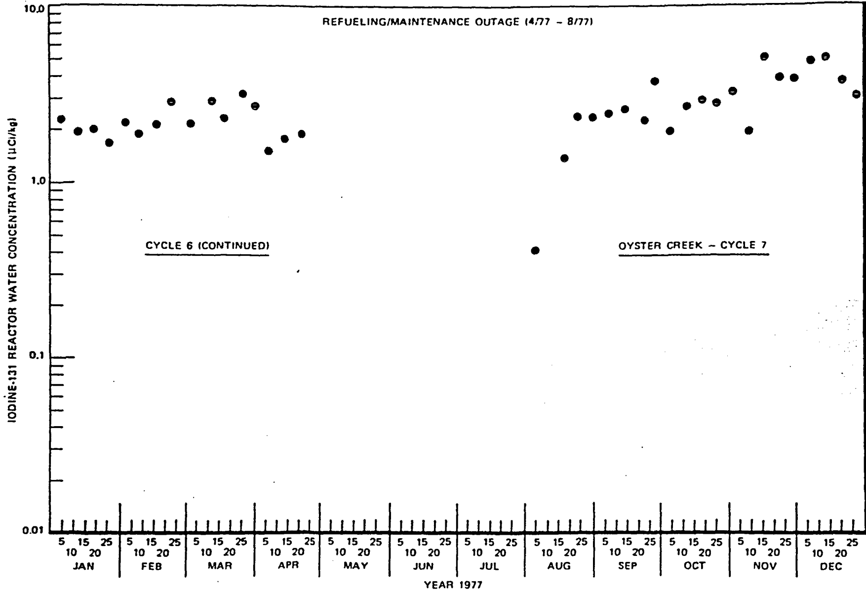
Figure 6-21a. Iodine-131 Reactor Water Concentration at Oyster Creek, 1977
