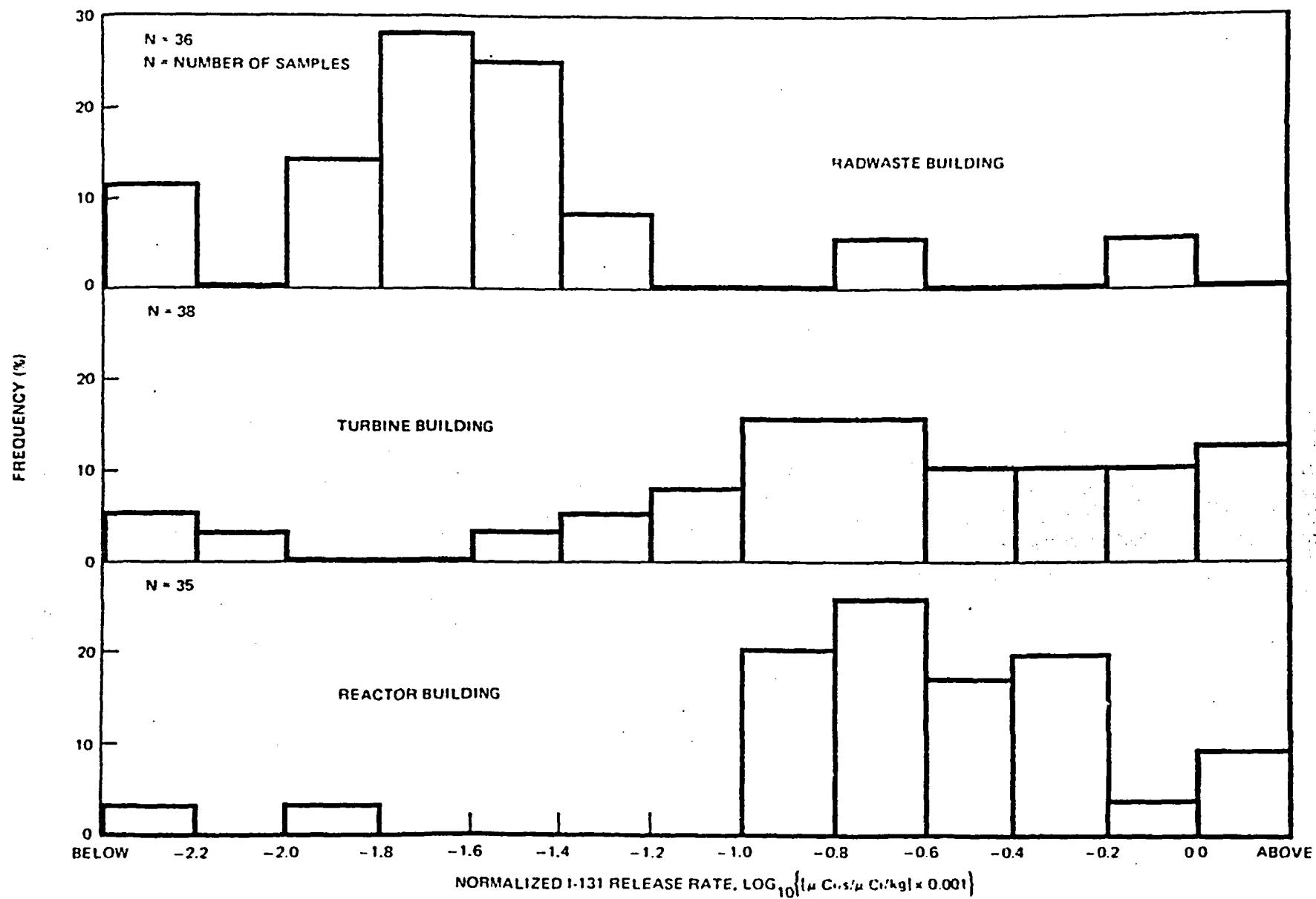
Figure 6-51. Frequency Polygons of Normalized I-131 Airborne Release Rates from Reactor, Turbine and Radwaste Buildings at Monticello
