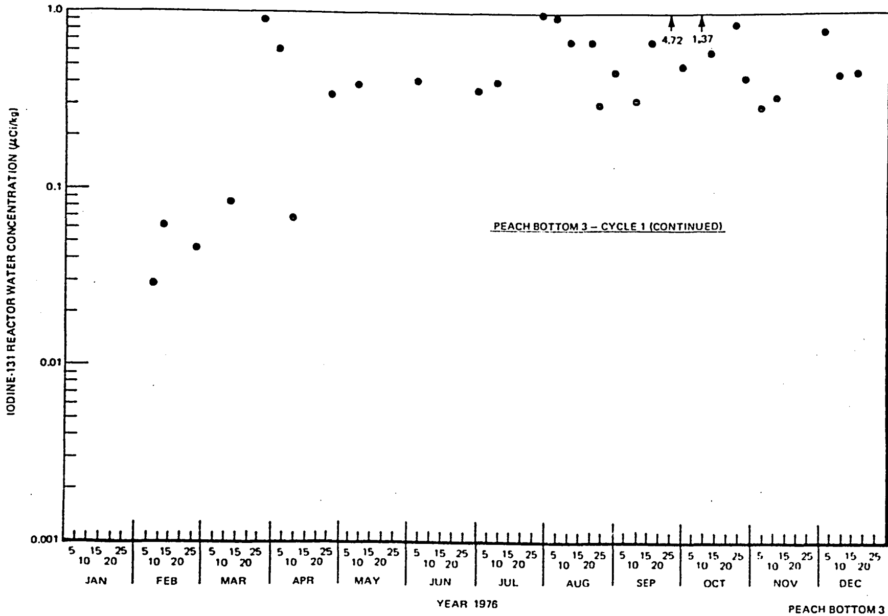
Figure 6-25. Iodine-131 Reactor Water Concentration at Peach Bottom 3, 1976
