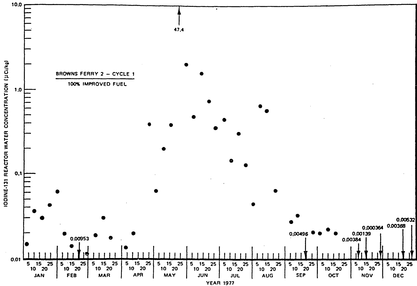
Figure 6-3. Iodine-131 Reactor Water Concentration at Browns Ferry 2, 1977
