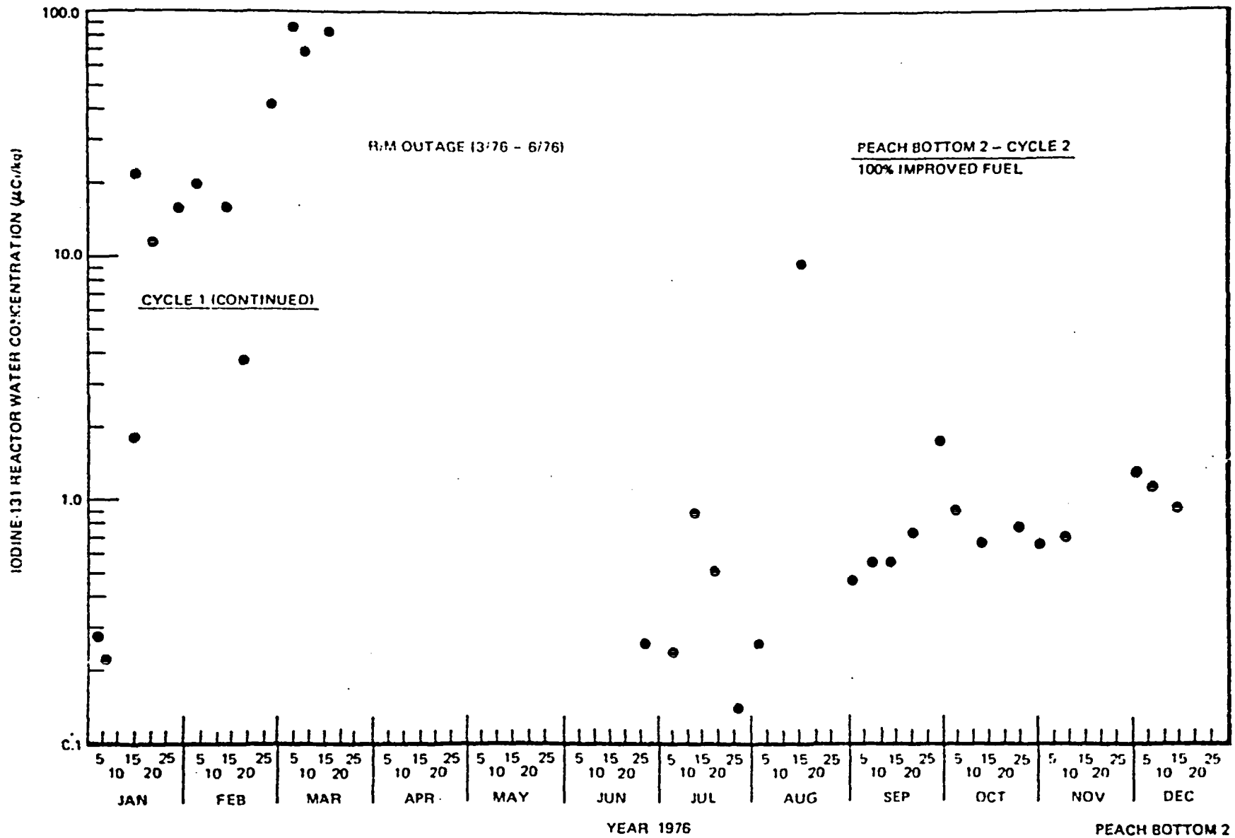
Figure 6-23. Iodine-131 Reactor Water Concentration at Peach Bottom 2, 1976
