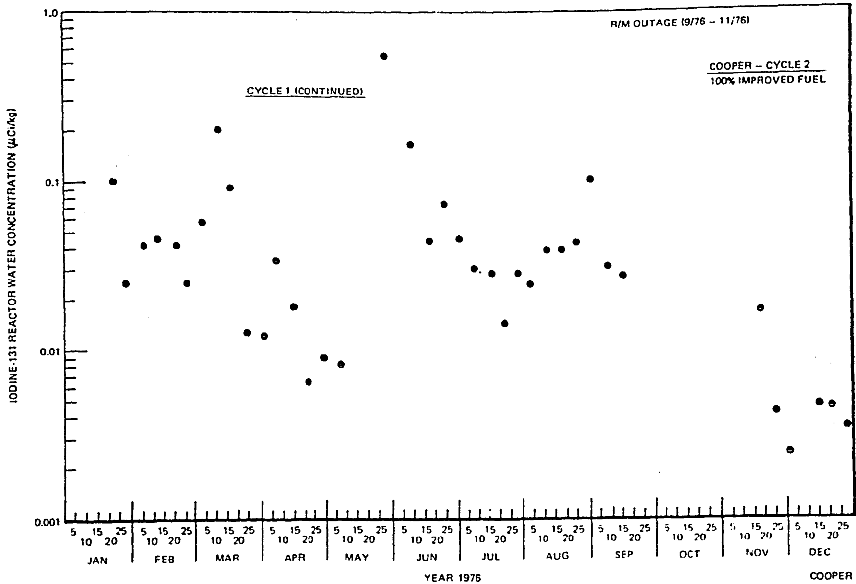
Figure 6-7a. Iodine-131 Reactor Water Concentration at Cooper, 1976
