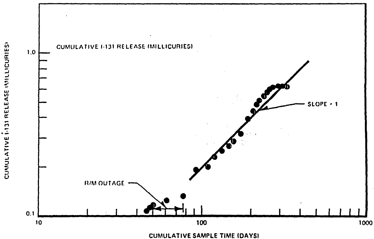
Figure 6-60. Cumulative Normalized I-131 Radwaste Building Airborne Release at Monticello
