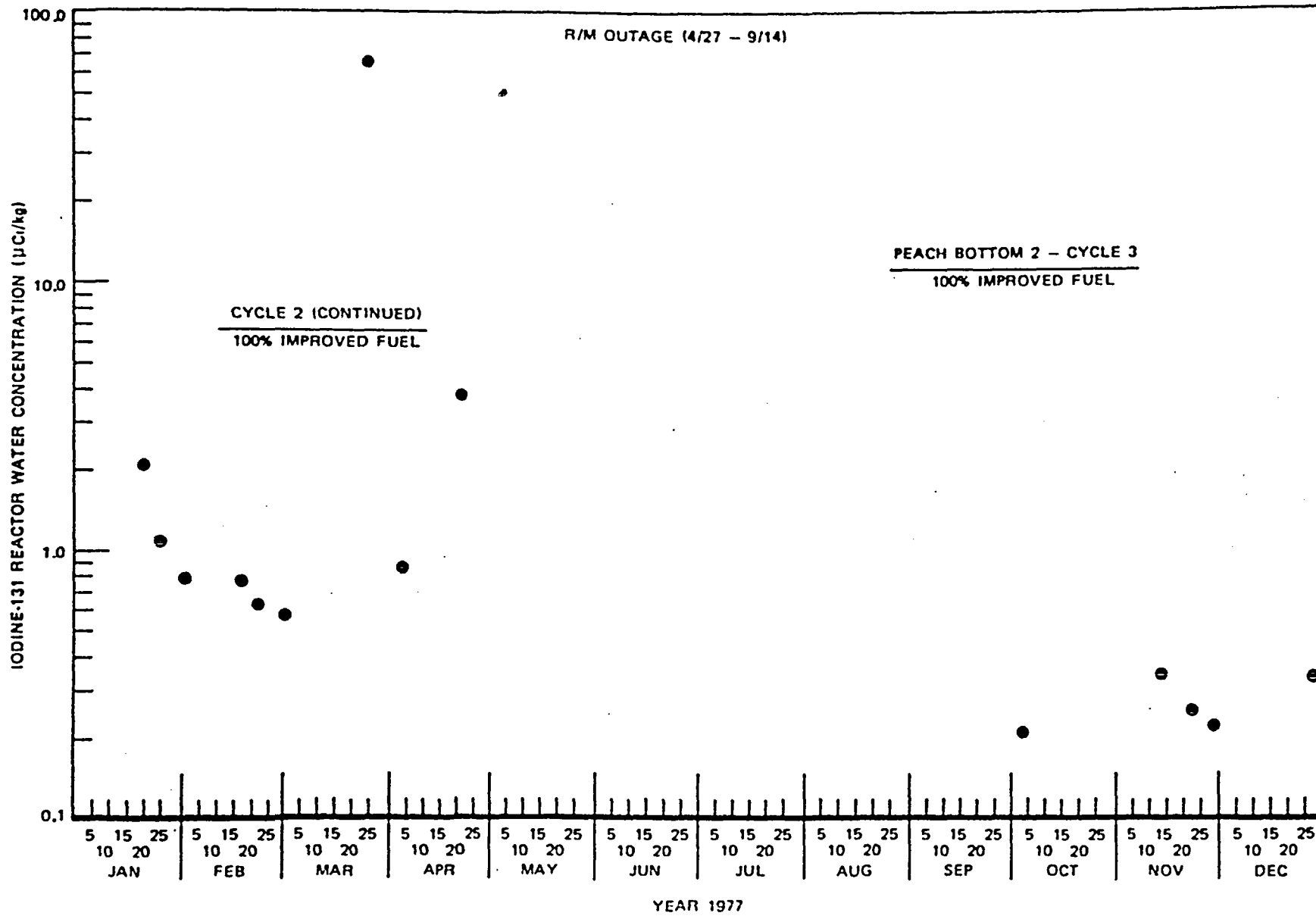
Figure 6-23a. Iodine-131 Reactor Water Concentration at Peach Bottom 2, 1977
