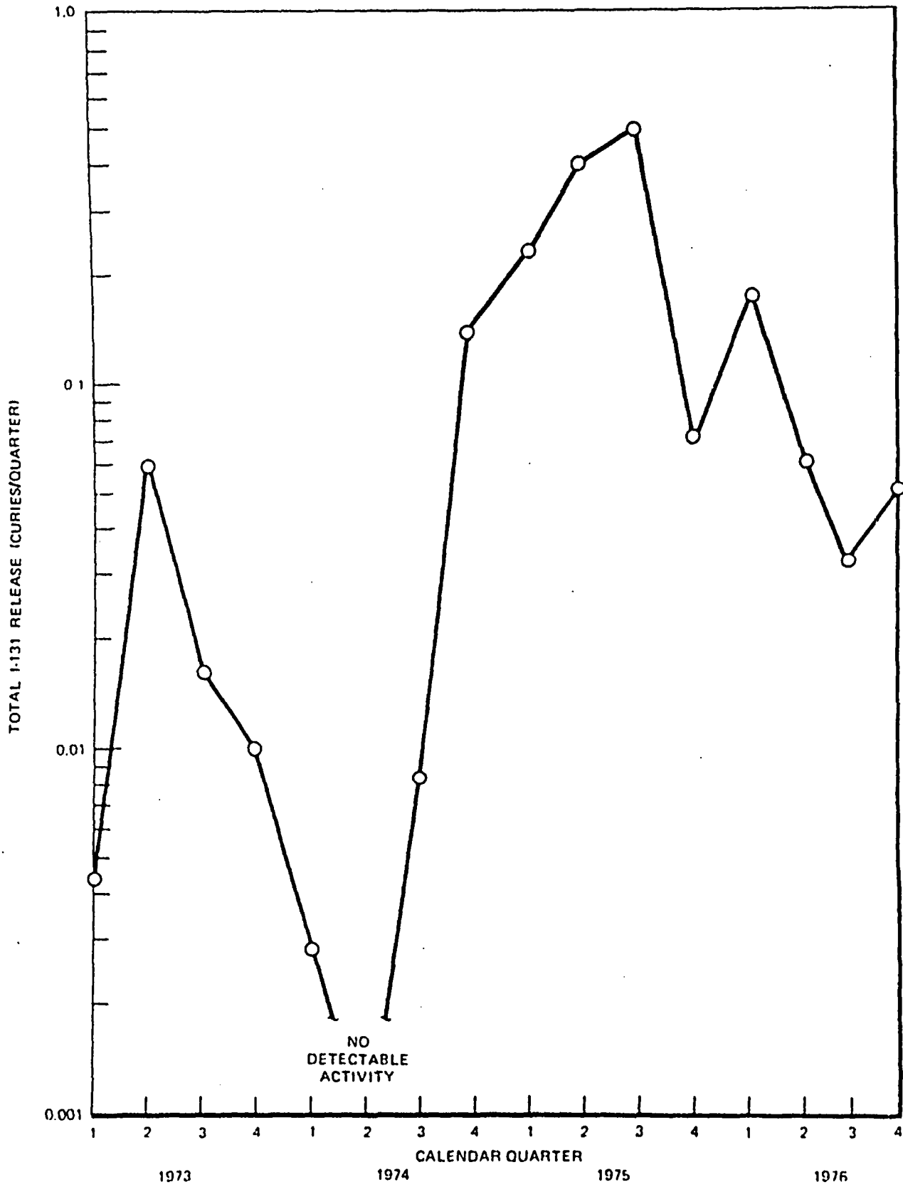
Figure 3-1. Calendar Quarterly Total Plant Ventilation Releases of I-131 versus Time, Pilgrim 1 (Reactor, Turbine and Radwaste Buildings)
