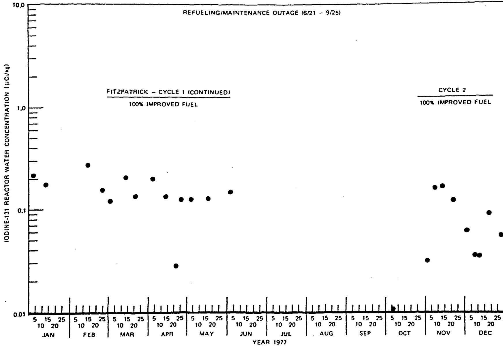
Figure 6-11. Iodine-131 Reactor Water Concentration at Fitzpatrick, 1977
