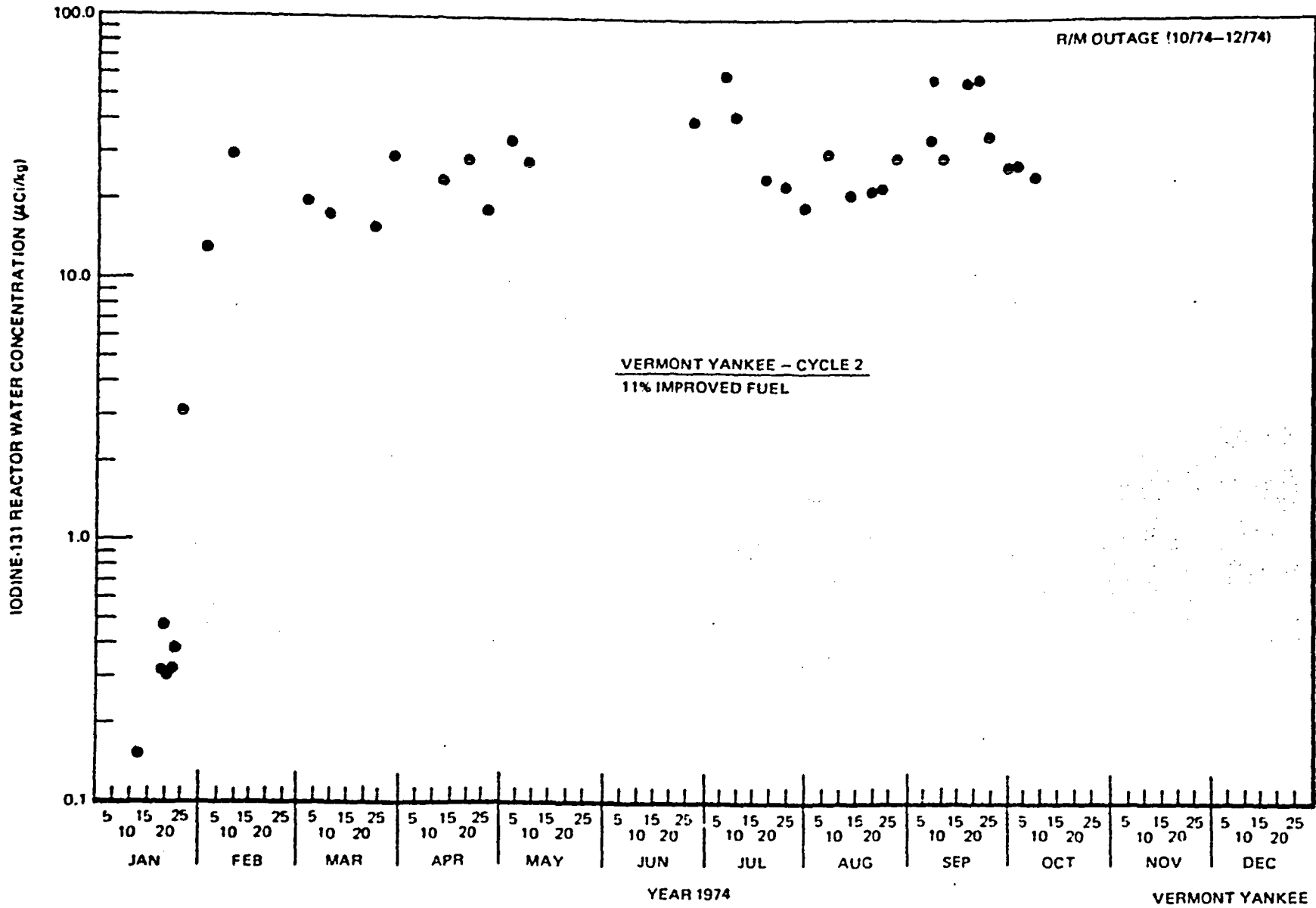
Figure 6-32. Iodine-131 Reactor Water Concentration at Vermont Yankee, 1974
