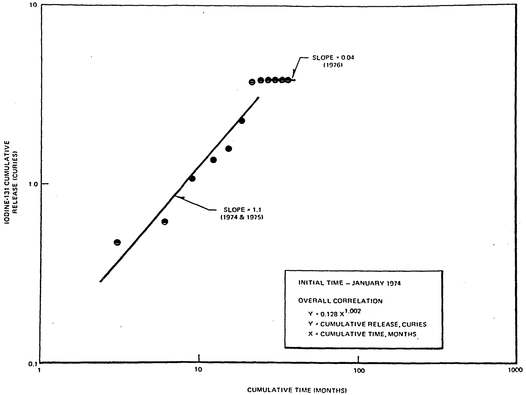
Figure 6-69. Trend Analysis of Monticello Iodine-131 Airborne Releases from Reactor, Turbine and Radwaste Buildings
