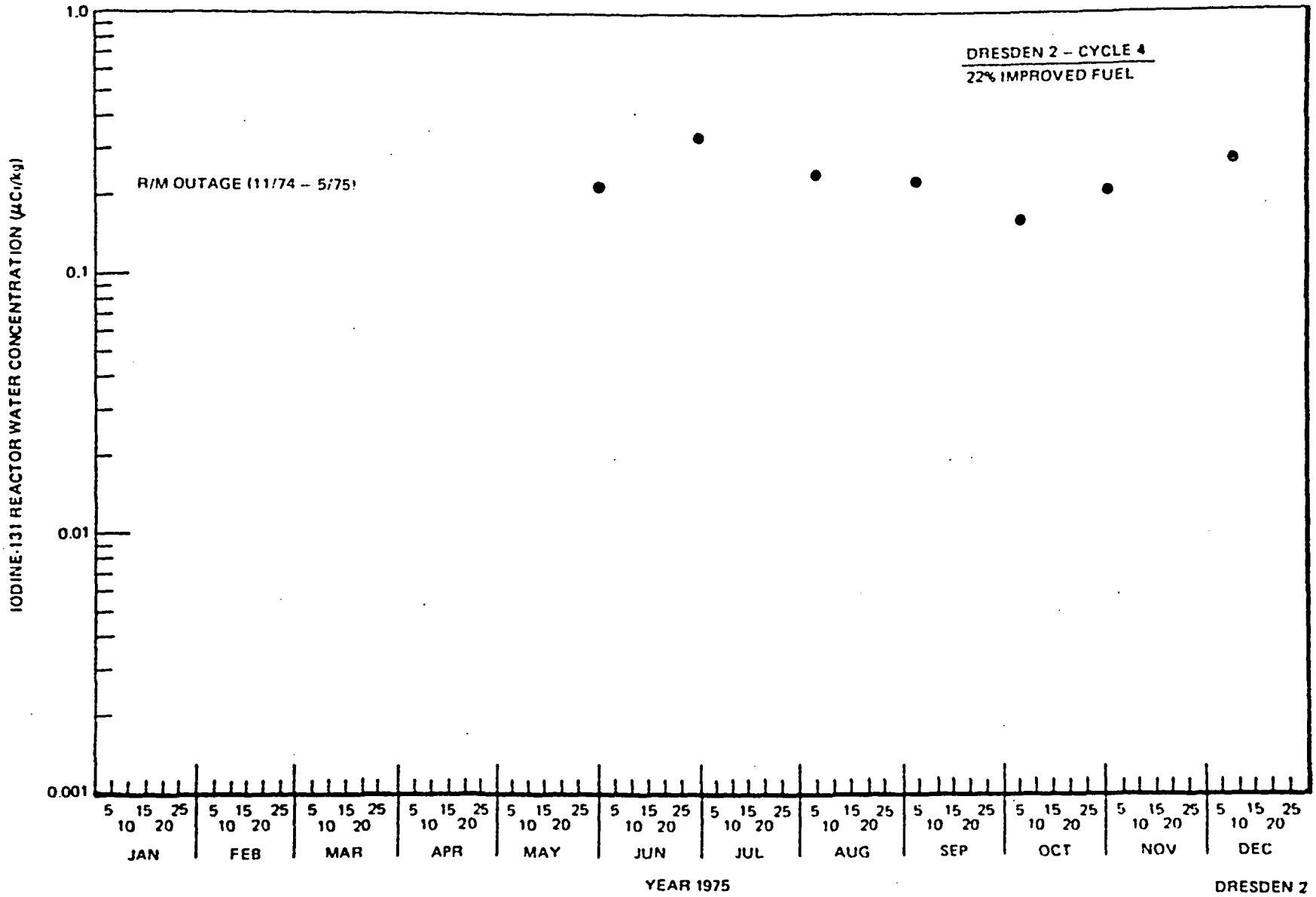
Figure 6-8. Iodine-131 Reactor Water Concentration at Dresden 2, 1975
