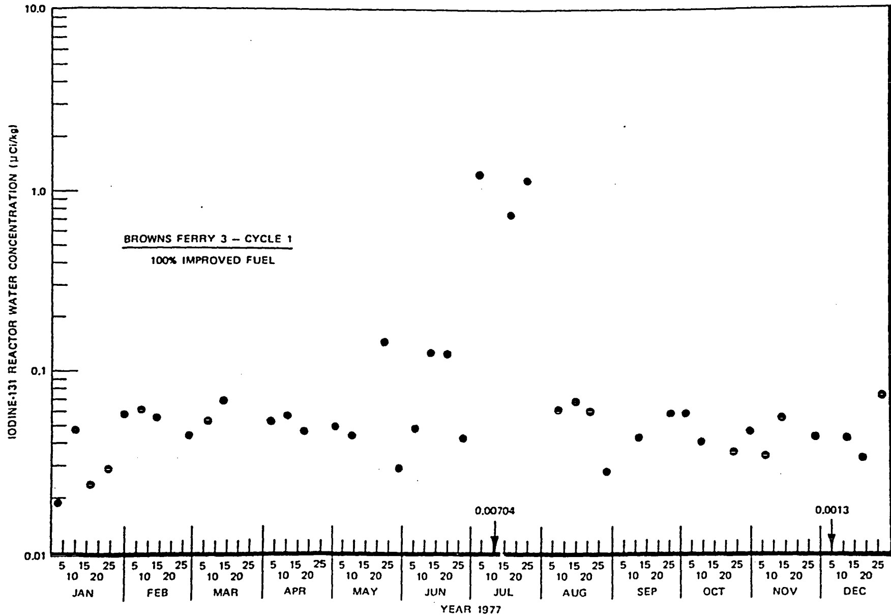
Figure 6-4. Iodine-131 Reactor Water Concentration at Browns Ferry 3, 1977
