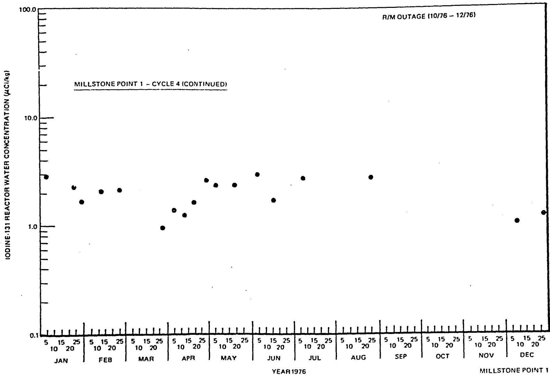
Figure 6-14. Iodine-131 Reactor Water Concentration at Millstone Point 1, 1976
