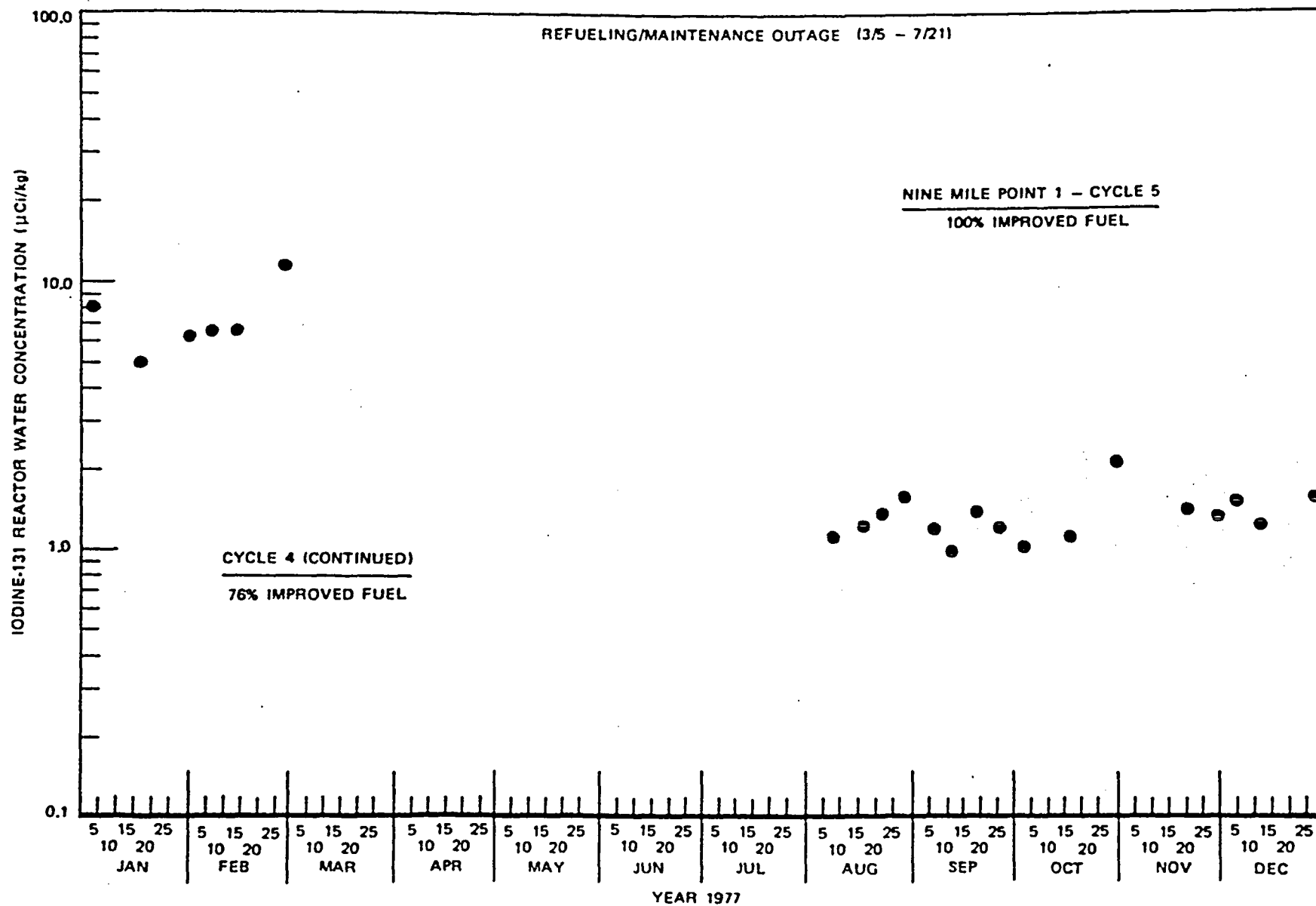
Figure 6-19a. Iodine-131 Reactor Water Concentration at Nine Mile Point 1, 1977
