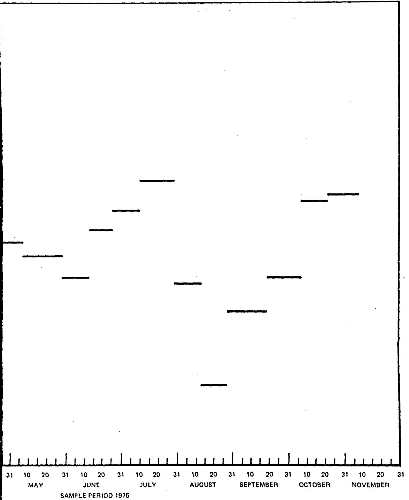
Figure 6-44. Normalized I-131 Release Rates, Radwaste Building Ventilation Exhaust at Vermont Yankee (1974 and 1975)
