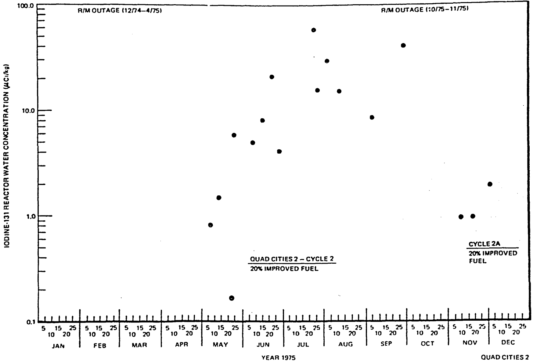
Figure 6-30. Iodine-131 Reactor Water Concentration at Quad Cities 2, 1975
