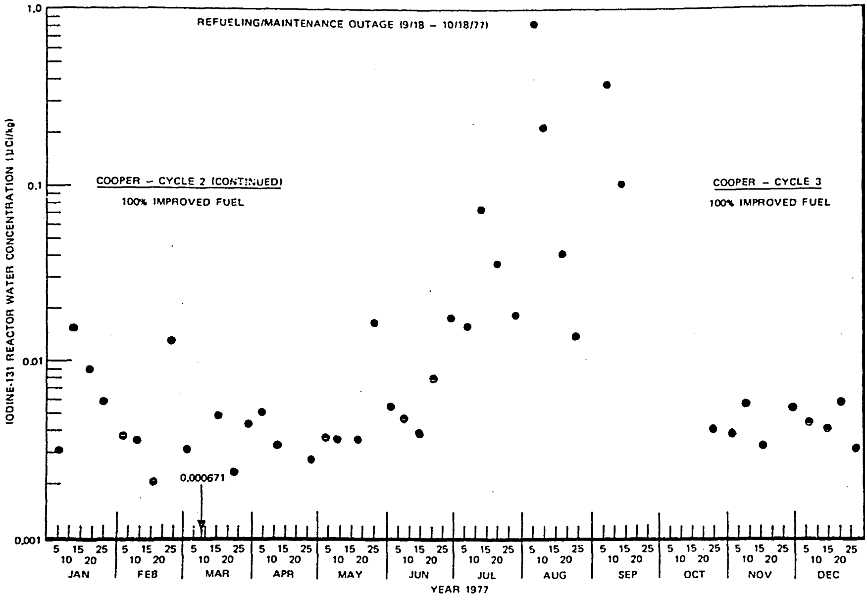
Figure 6-7b. Iodine-131 Reactor Water Concentration at Cooper, 1977
