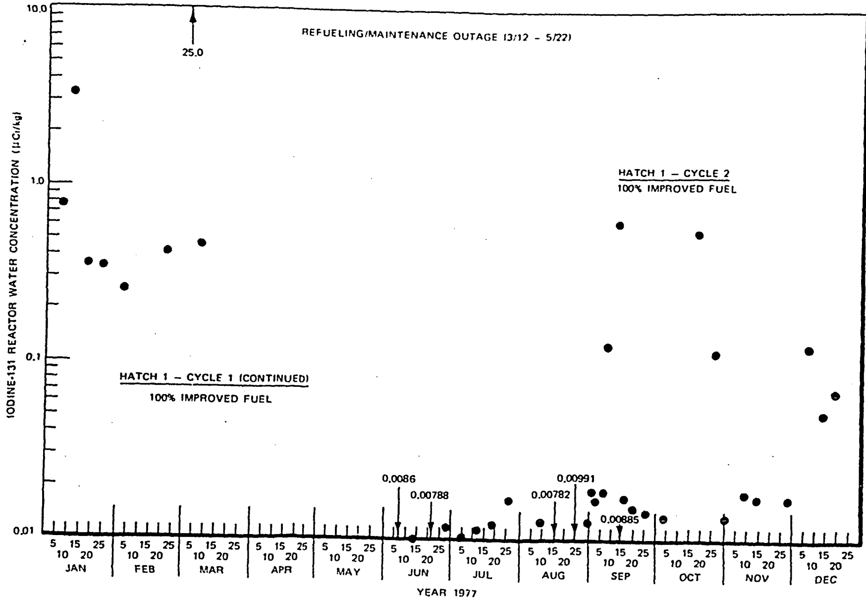
Figure 6-12b. Iodine-131 Reactor Water Concentration at Hatch 1, 1977
