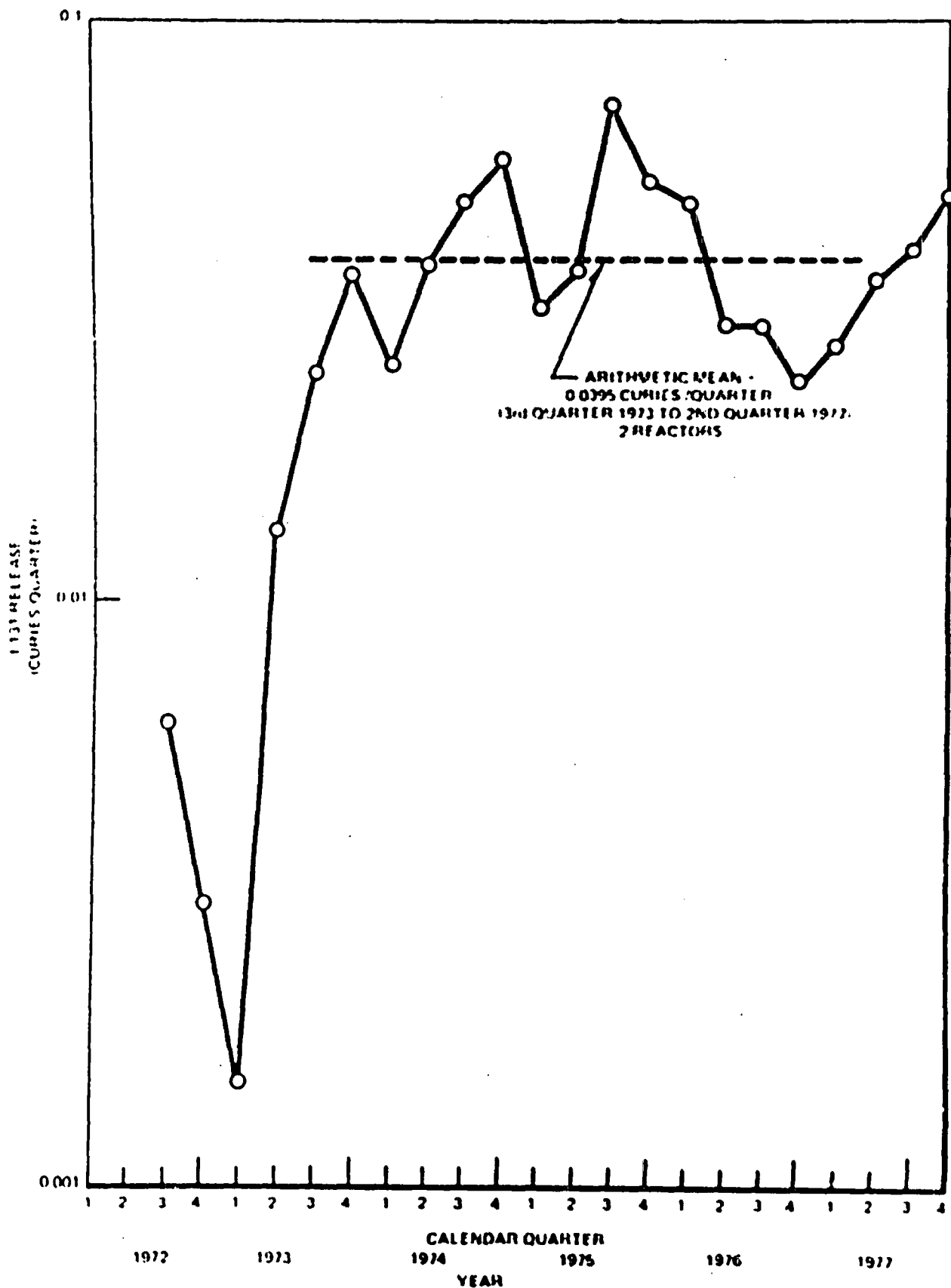
Figure 35 Calendar Quarter Reactor Building Ventilation Release of I-131 versus Time, Quad Cities 1 2
