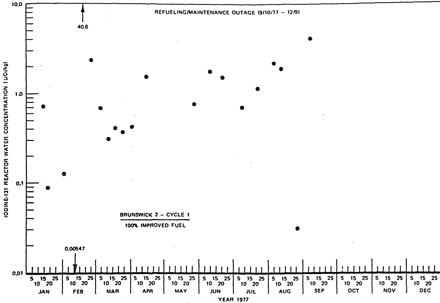
Figure 6-6. Iodine-131 Reactor Water Concentration at Brunswick 2, 1977
