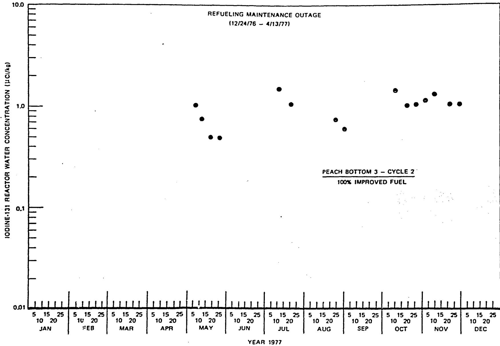
Figure 6-25a. Iodine-131 Reactor Water Concentration at Peach Bottom 3, 1977
