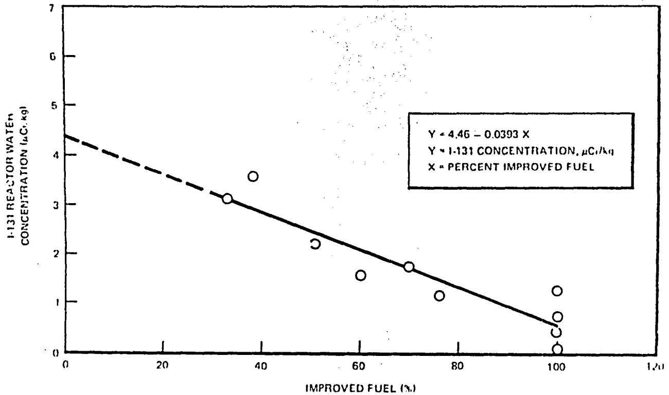
Figure 7-1. Correlation of I-131 Concentration in Reactor Water with Amount of Improved Fuel
