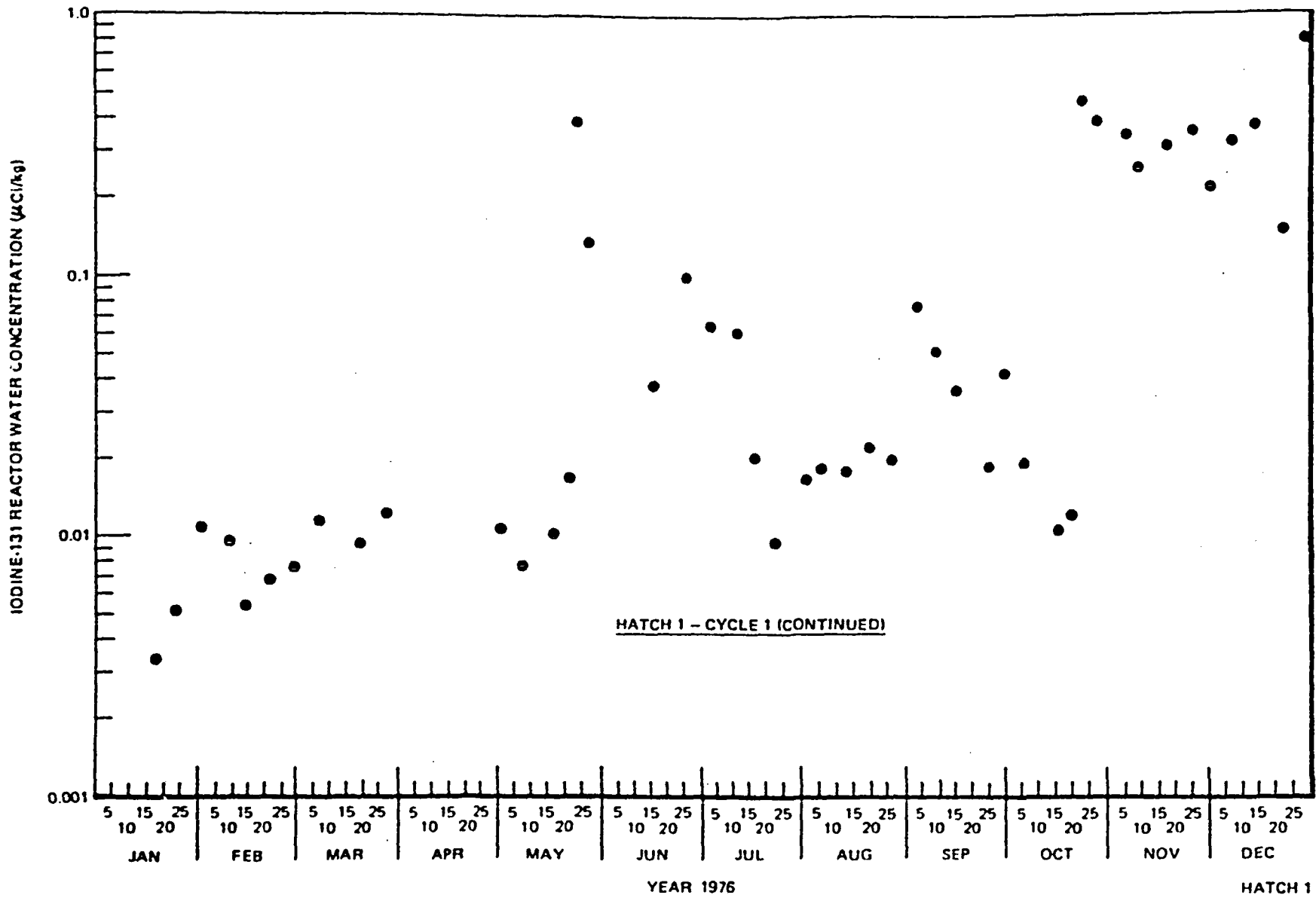
Figure 6-12a. Iodine-131 Reactor Water Concentration at Hatch 1, 1976
