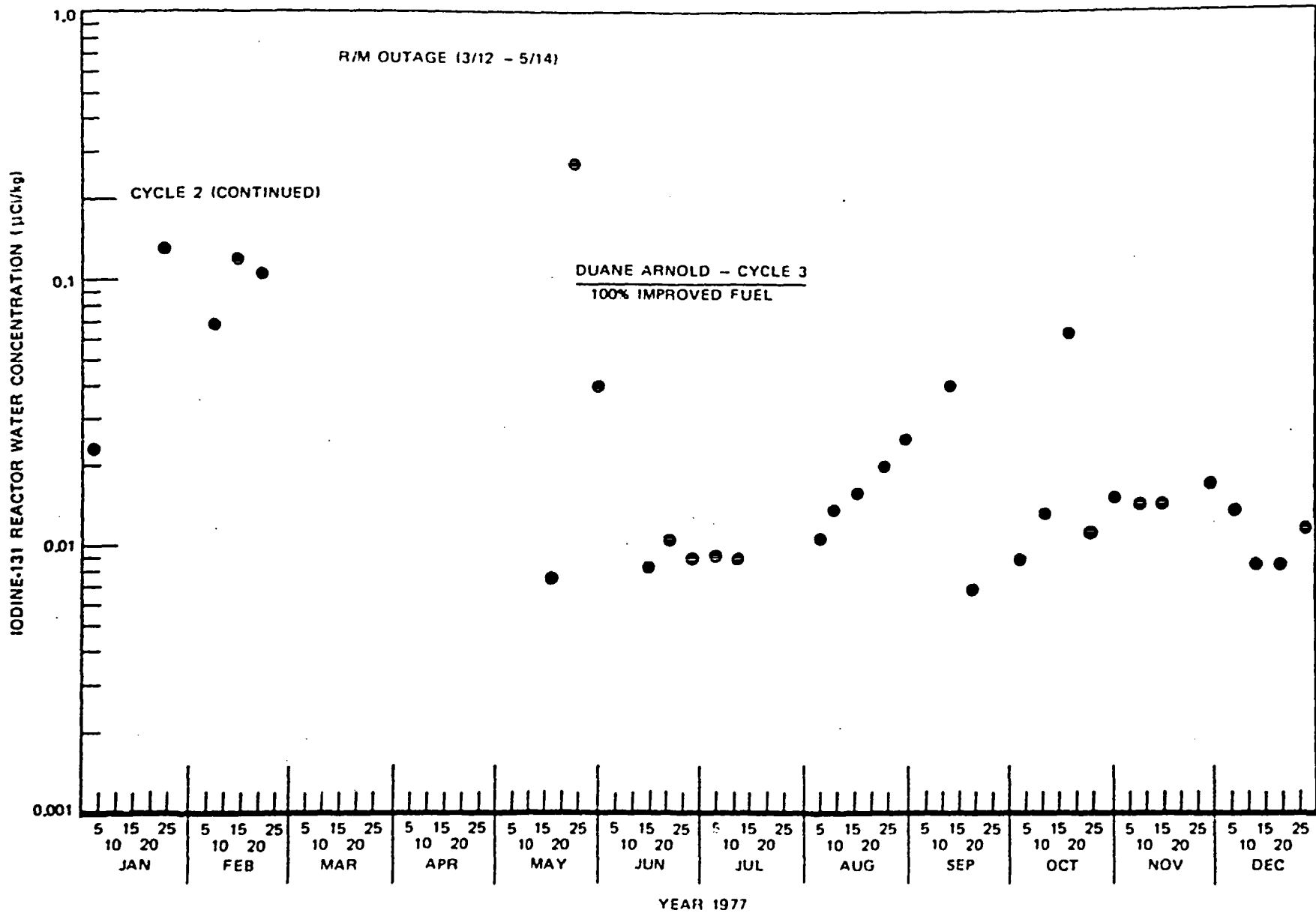
Figure 6-10b. Iodine-131 Reactor Water Concentration at Duane Arnold, 1977
