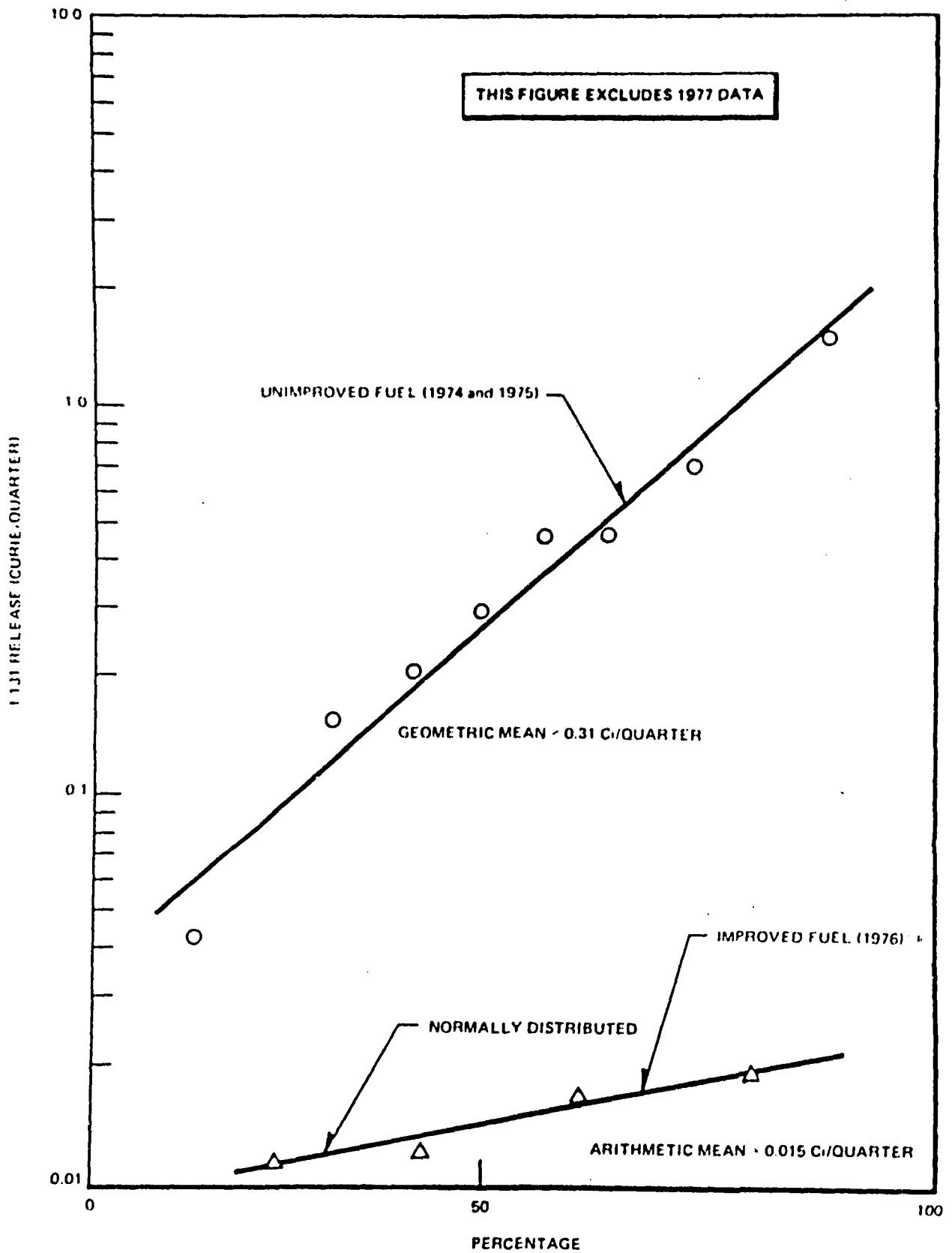
Figure 3-8. Accumulative Lognormal Probability Distribution of Calendar Quarter 1-131 Total Plant Ventilation Releases, Monticello (Reactor, Turbine and Radwaste Buildings, January 1974 to December 1976)
