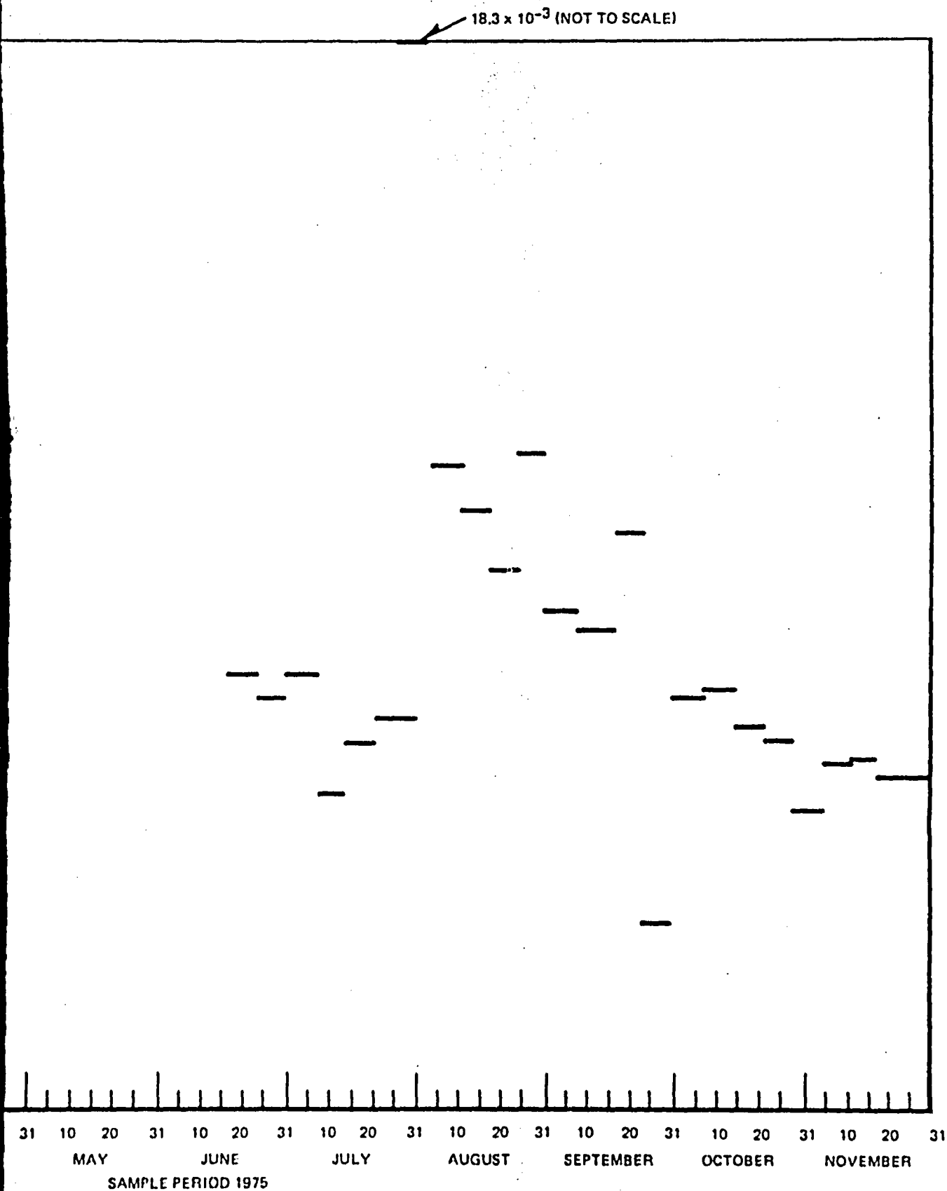
Figure 6-40. Normalized I-131 Release Rates, Reactor Building Ventilation Exhaust at Oyster Creek (1975 and 1976)
