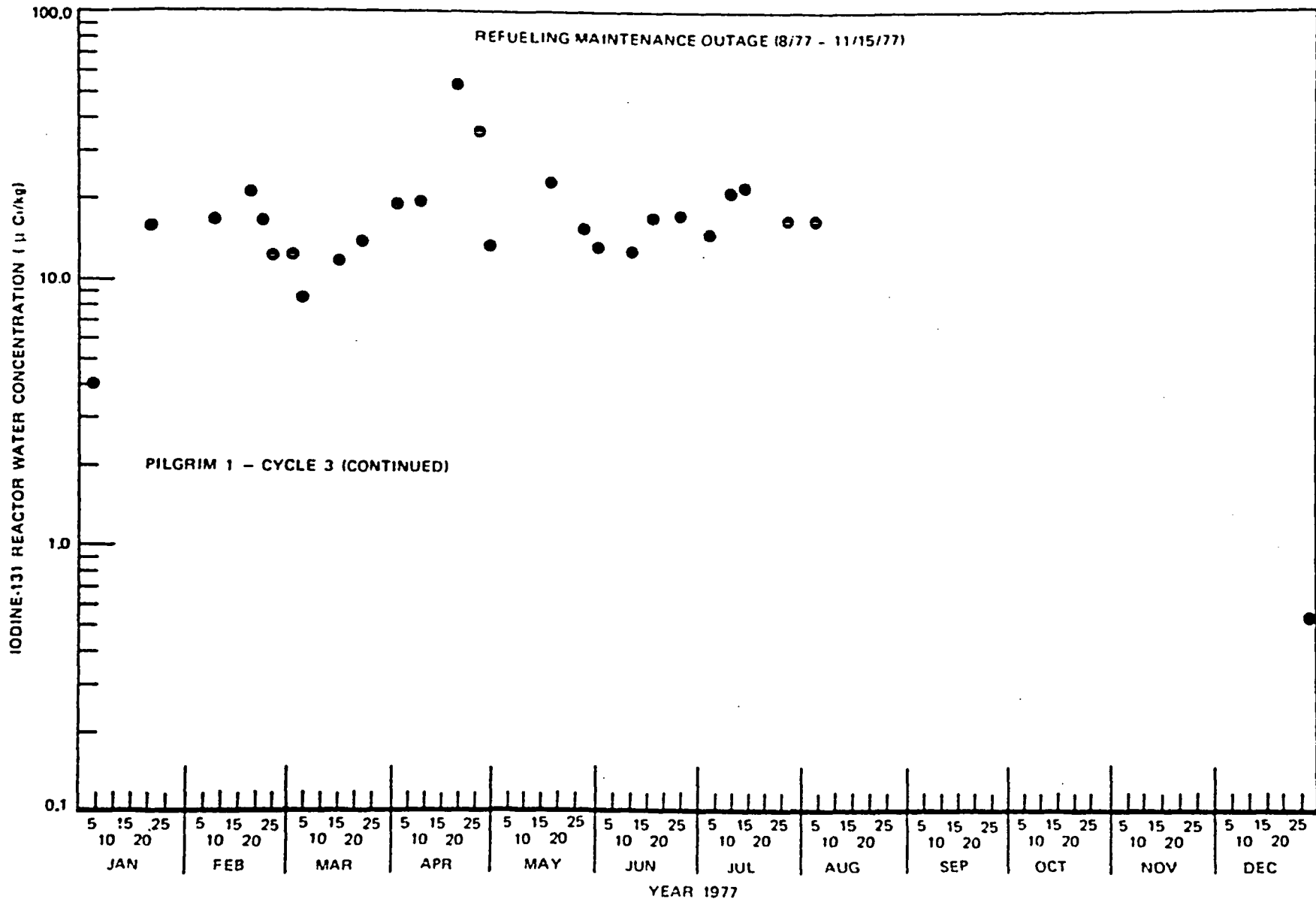
Figure 6-27a. Iodine-131 Reactor Water Concentration at Pilgrim 1, 1977
