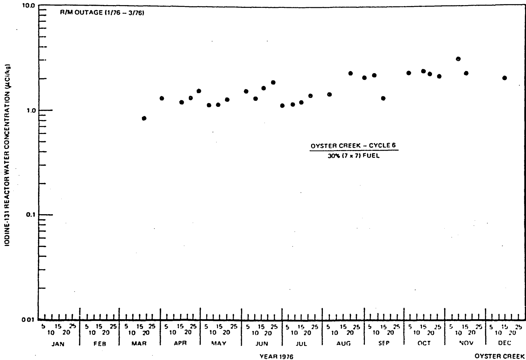
Figure 6-21. Iodine-131 Reactor Water Concentration at Oyster Creek, 1976
