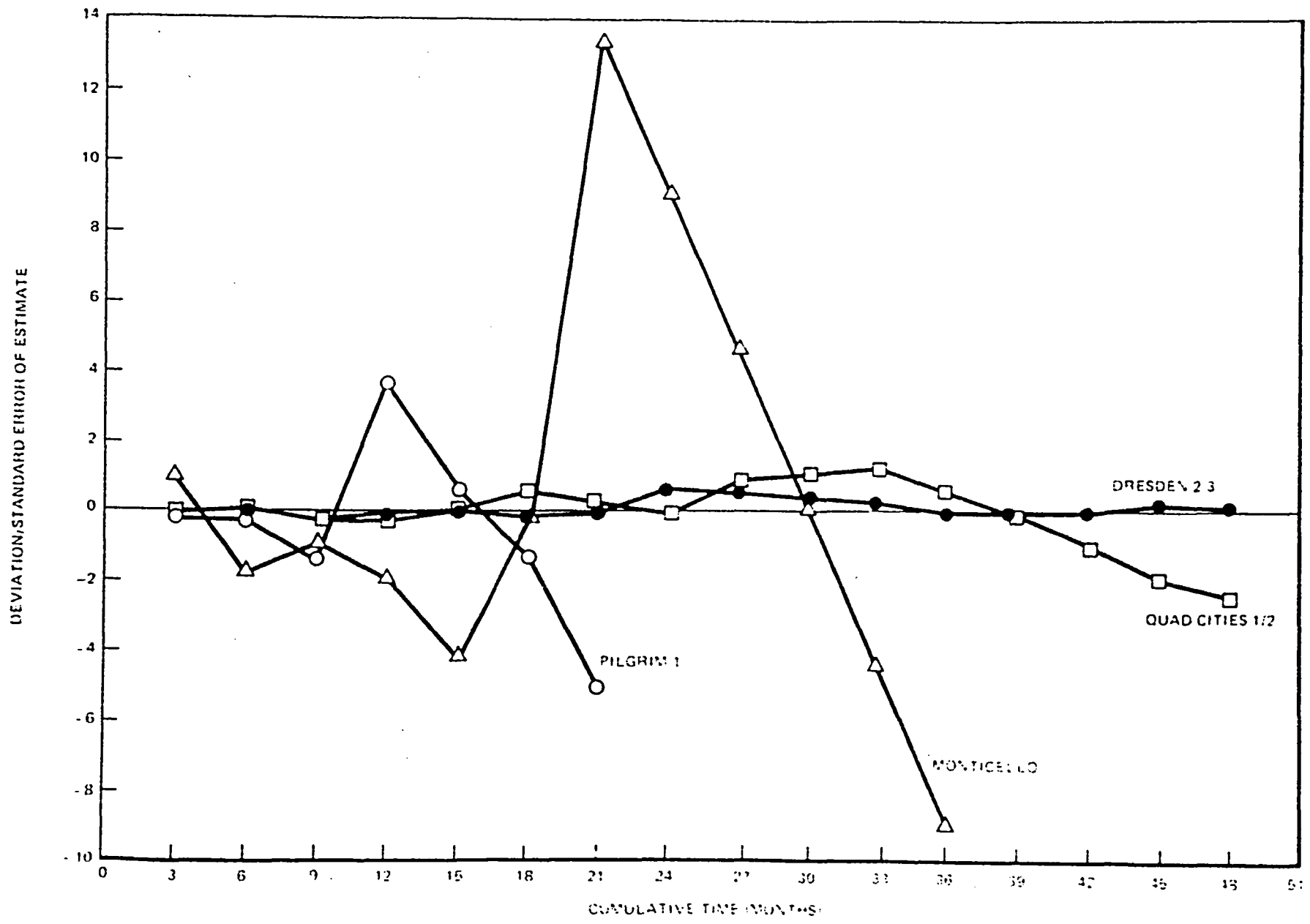
Figure 2-1. Long-Term Trend Analysis of Cumulative Iodine 131 Airborne Releases from BWR Ventilation Exhausts
