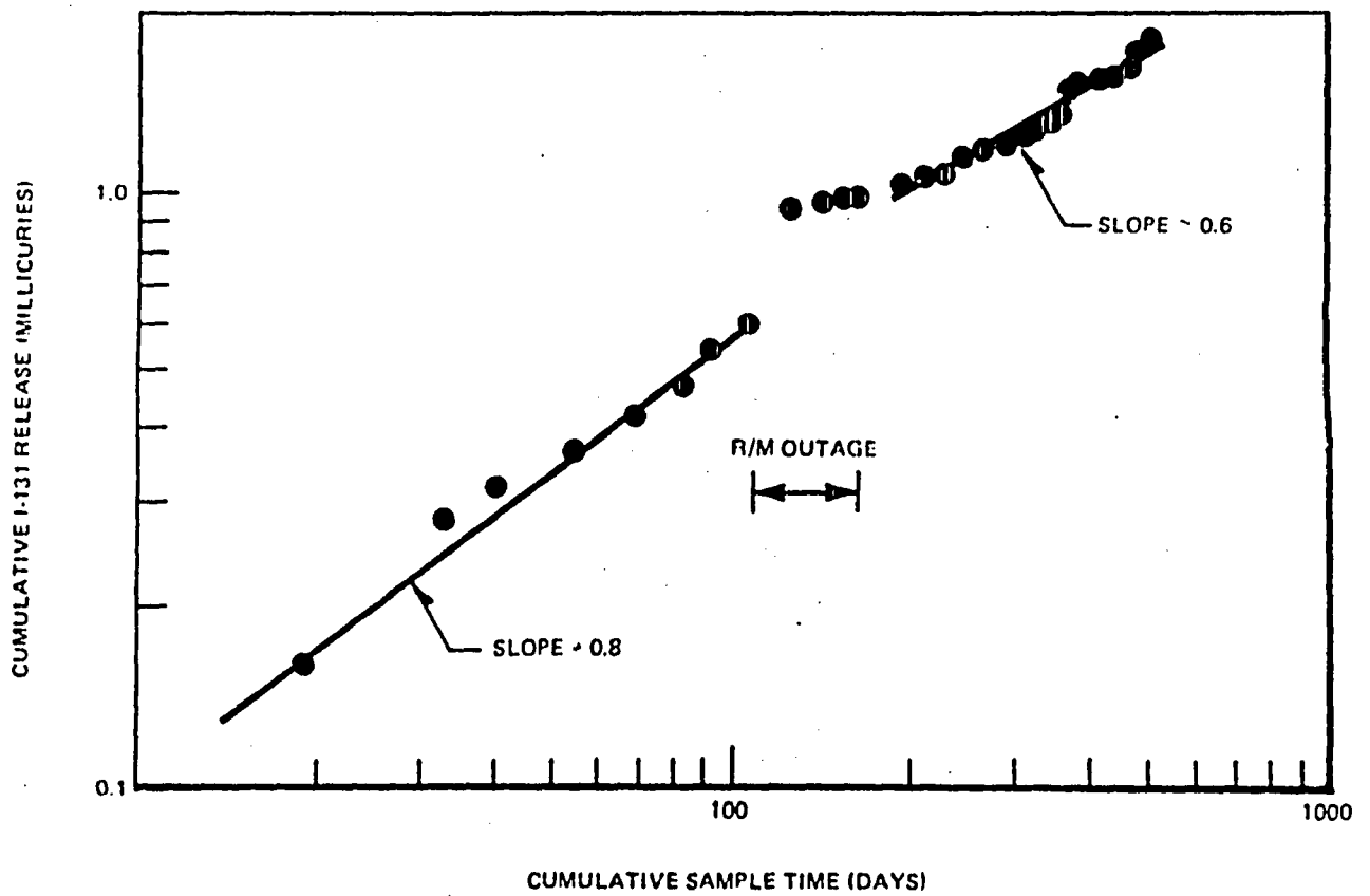
Figure 6-57. Cumulative Normalized I-131 Radwaste Building Airborne Release at Vermont Yankee
