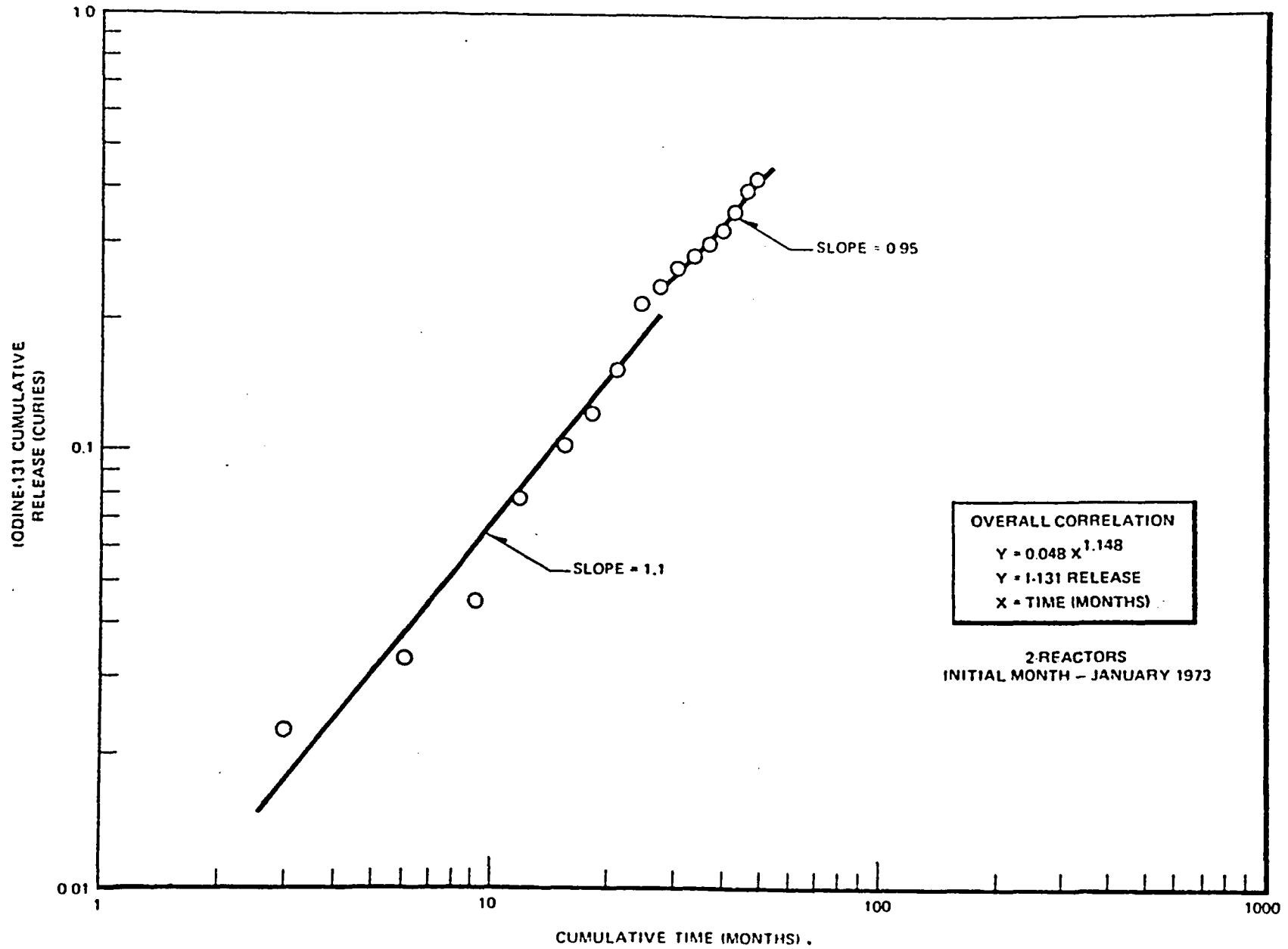
Figure 6-67. Trend Analysis of Dresden 2/3 Iodine-131 Airborne Releases from Reactor Building Ventilation Exhaust
