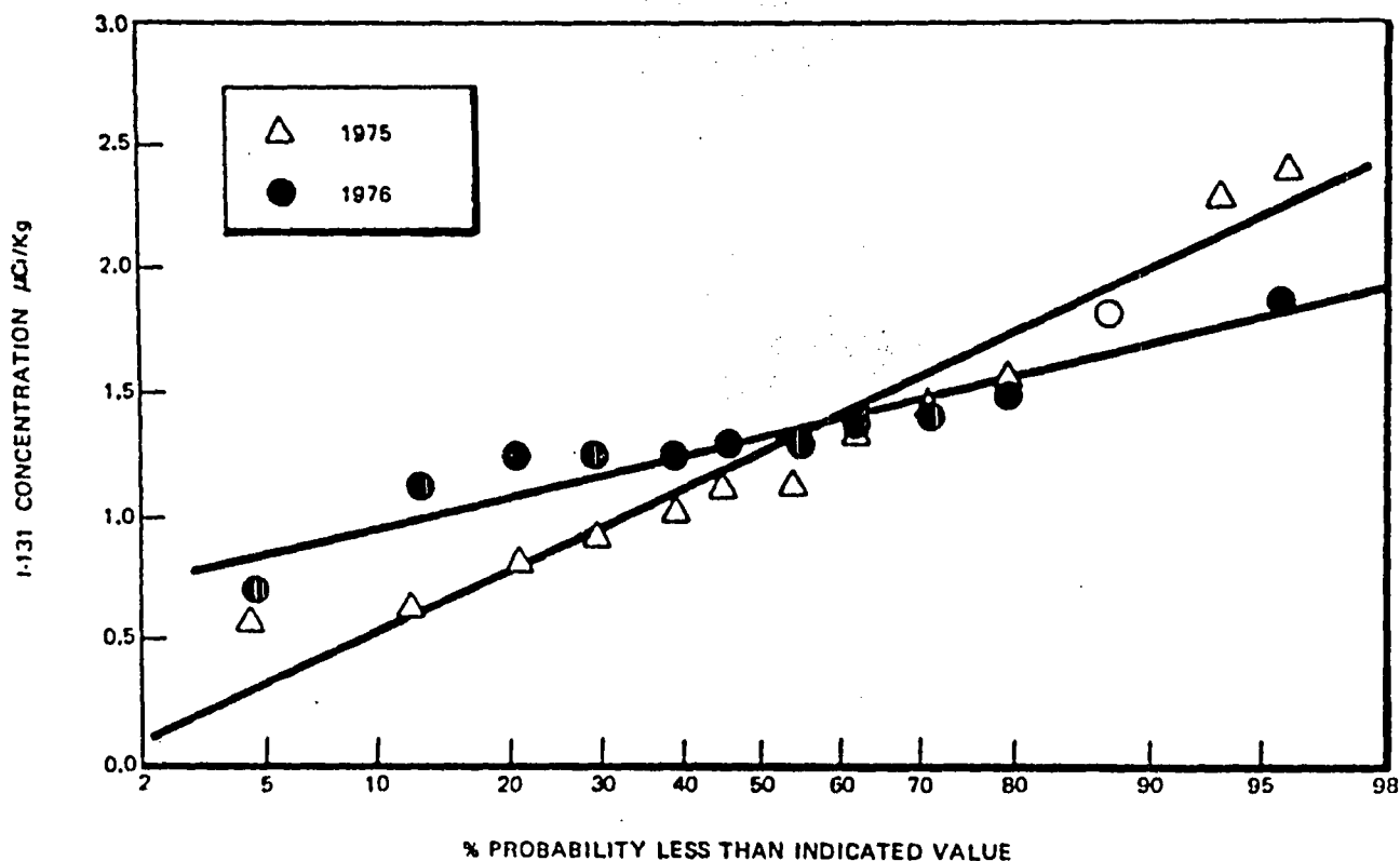
Figure 6-35. Normal Probability Distribution of Medians of Maximum Monthly I-131 Reactor Water Concentrations During 1975 and 1976 for 15 Domestic BWR's
