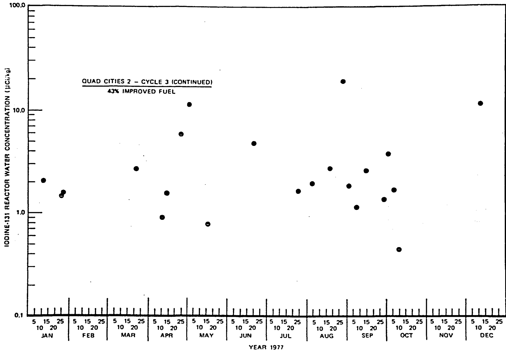
Figure 6-31a. Iodine-131 Reactor Water Concentration at Quad Cities 2, 1977
