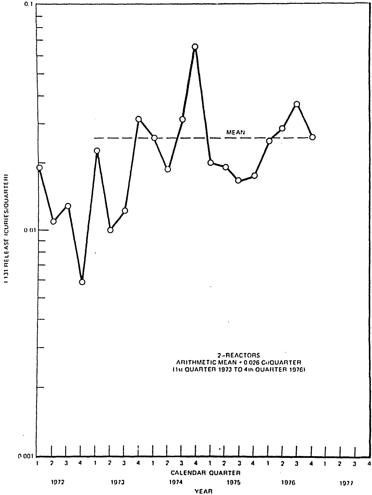
Figure 3-3. Calendar Quarter Reactor Building Ventilation Release of I-131 Versus Time, Dresden 2/3
