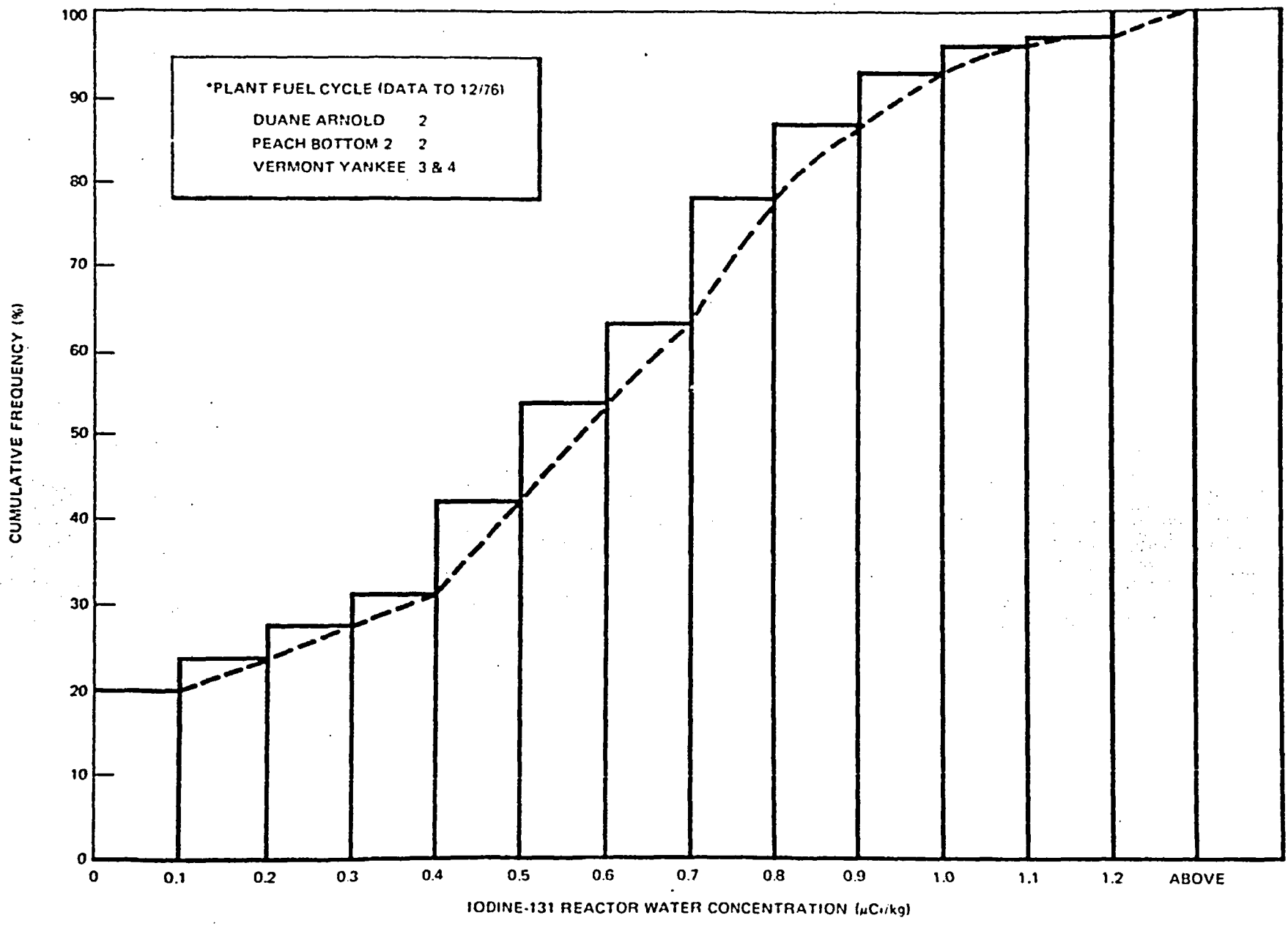
Figure 7-3. Cumulative Frequency Polygon and Ogive Curve of I-131 Reactor Water Concentrations in BWR's with 100% Improved Fuel*
