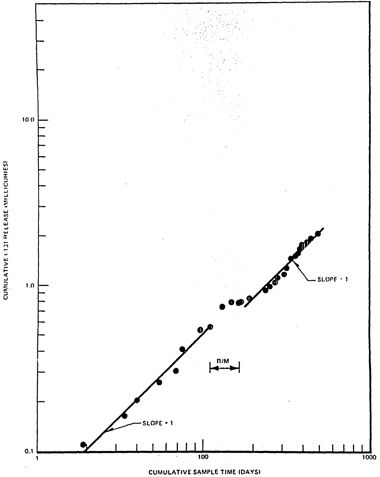
Figure 6-56. Cumulative Normalized I-131 Turbine Building Airborne Release at Vermont Yankee
