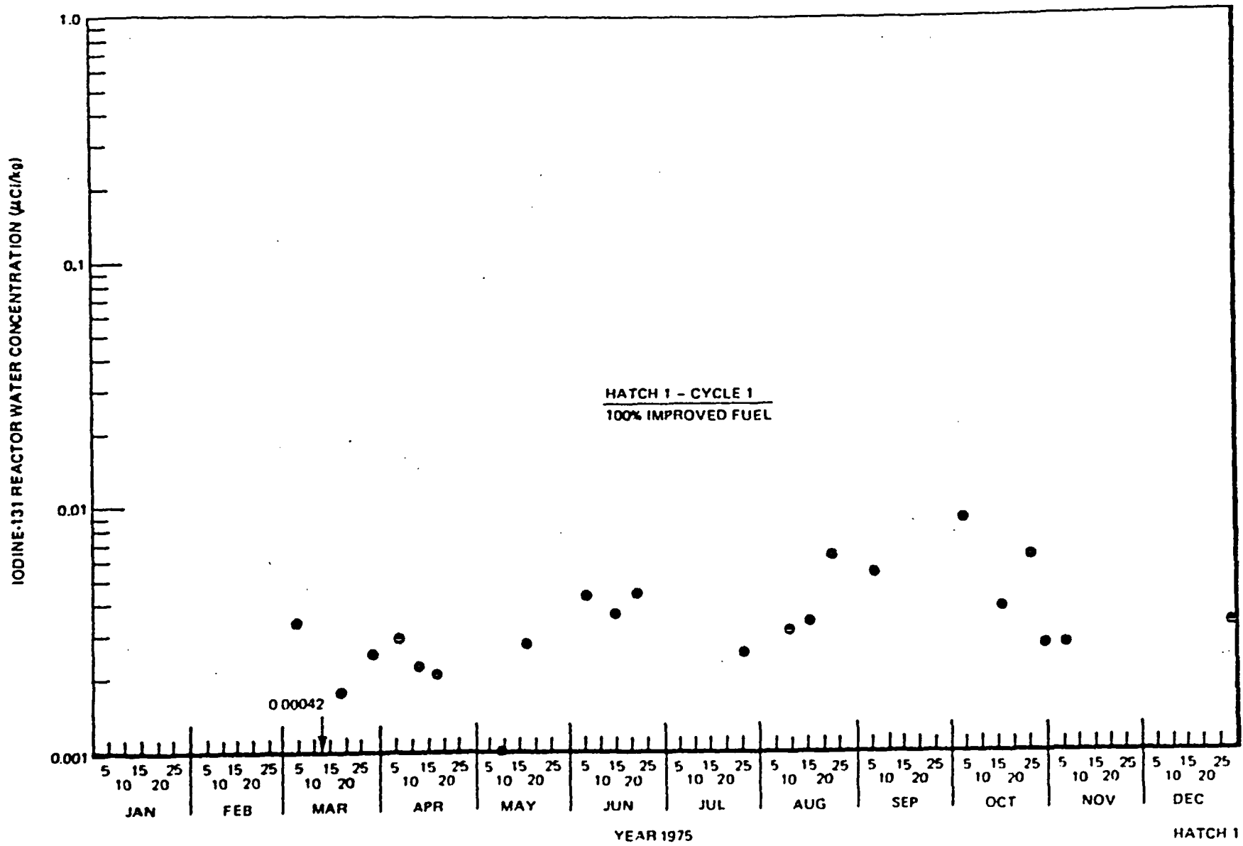
Figure 6-12. Iodine-131 Reactor Water Concentration at Hatch 1, 1975
