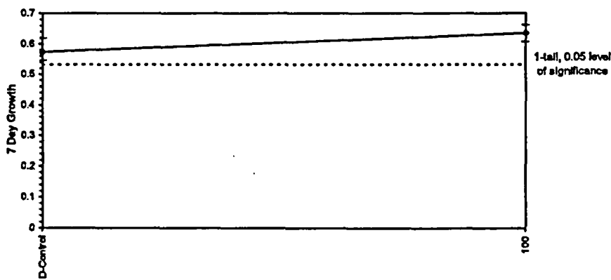
Dose-Response Plot
