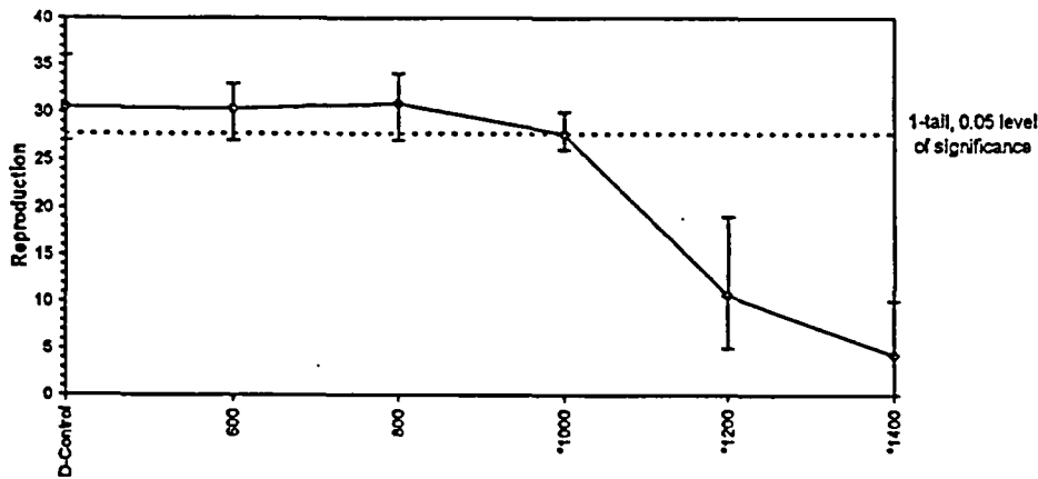
Dose-Response Plot
