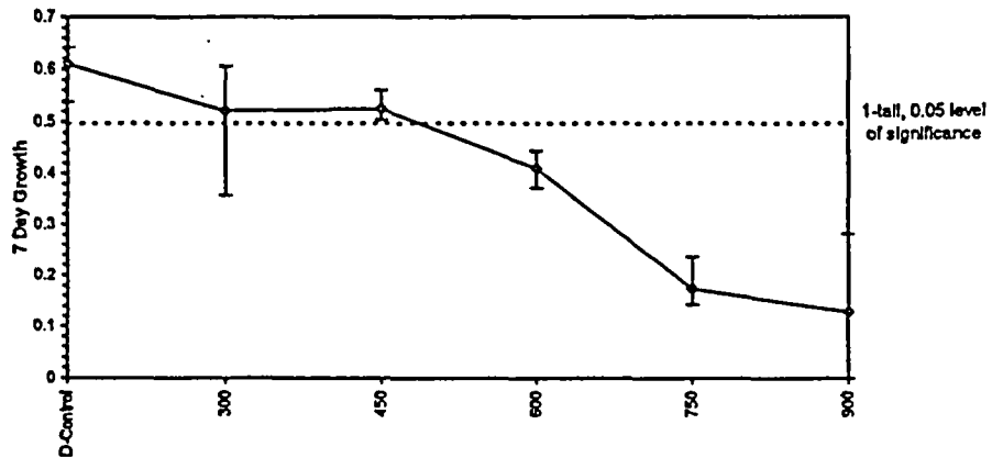
Dose-Response Plot
