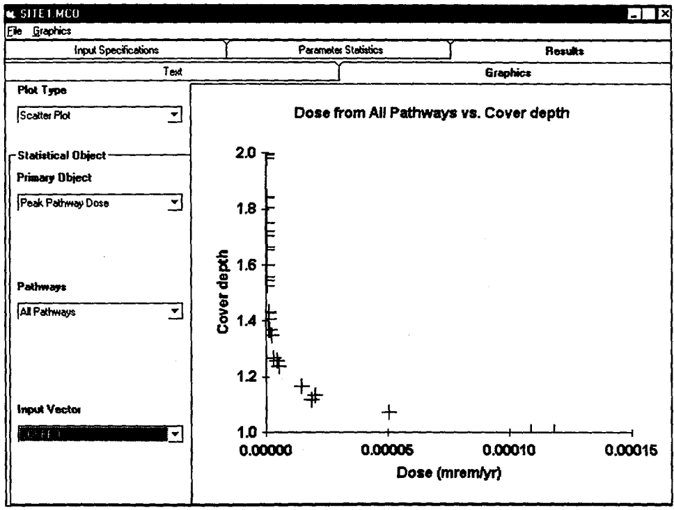
Figure 13 Scatter Plot
