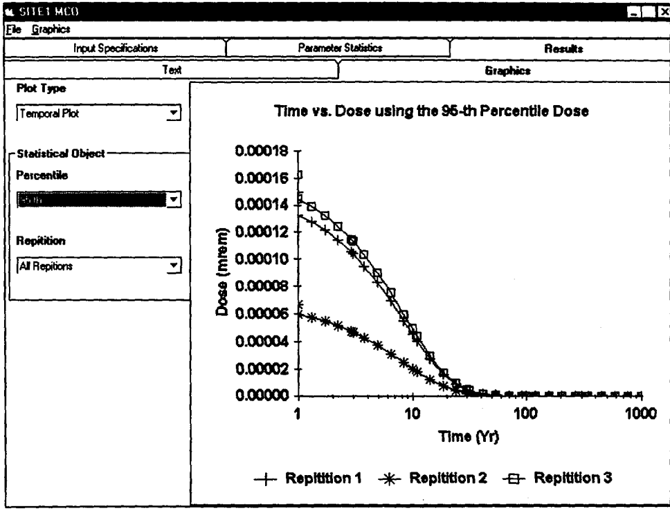
Figure 14 Temporal Plot
