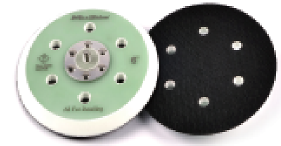
3013150 6" (150mm) Max OPM: 12000 Thread: 5/16"-24 Hole: 6
