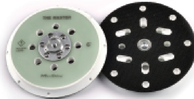
3011150 6" (150mm) Max OPM: 12000 Thread: 5/16"-24 Hole: 8
