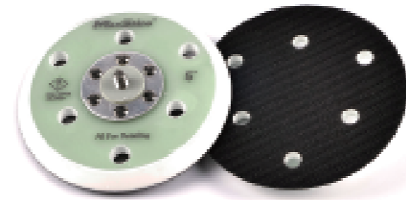
3013125 5" (125mm) Max OPM: 12000 Thread: 5/16"-24 Hole: 6
