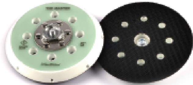
3011125 5" (125mm) Max OPM: 12000 Thread: 5/16"-24 Hole: 8
