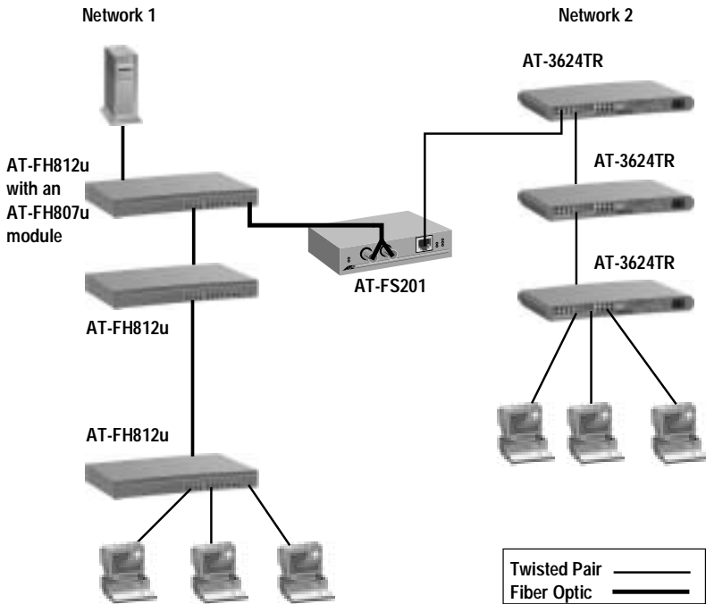
Figure 4 Network Topology
