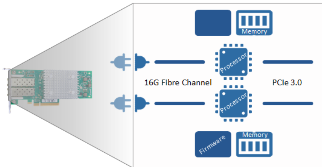
Figure 2. QLogic Enhanced Gen 5 Fibre Channel Adapter Port Isolation Architecture
