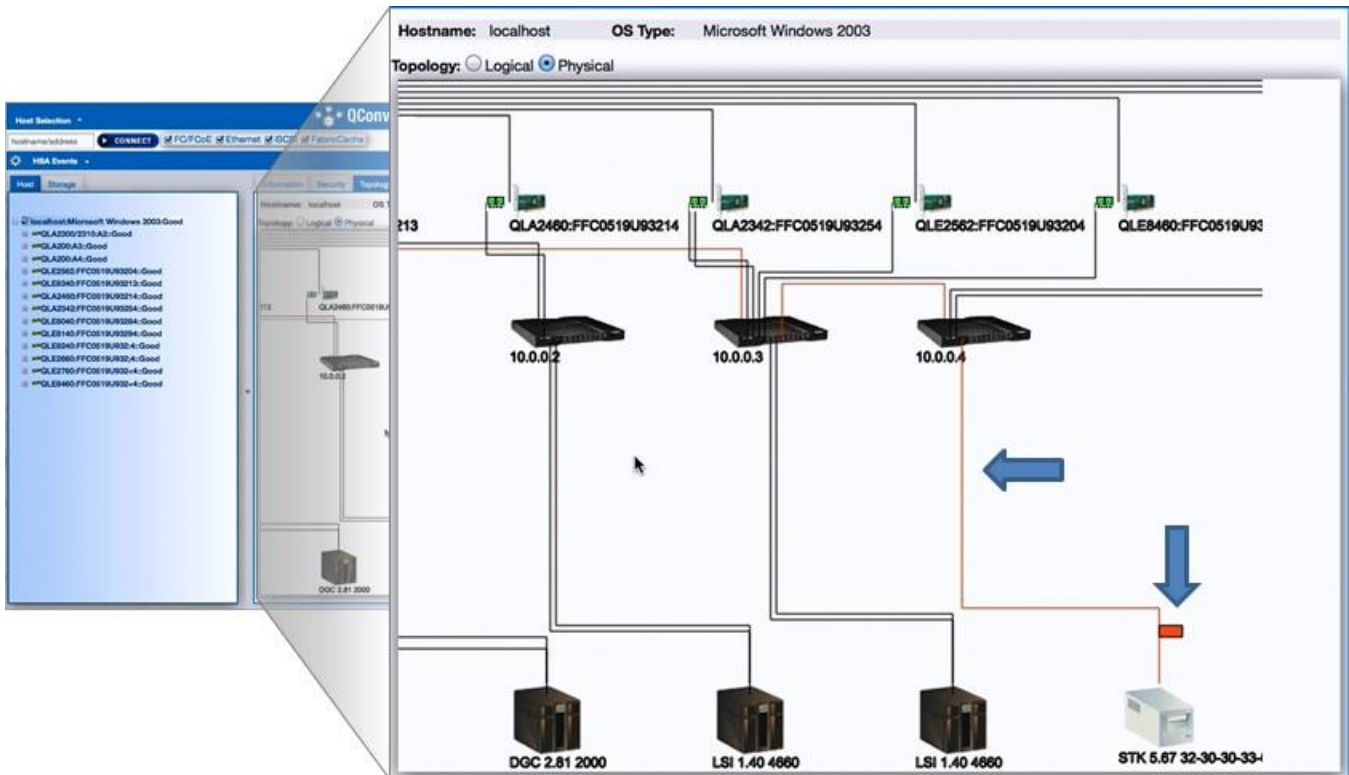
Figure 12. FC Traceroute
