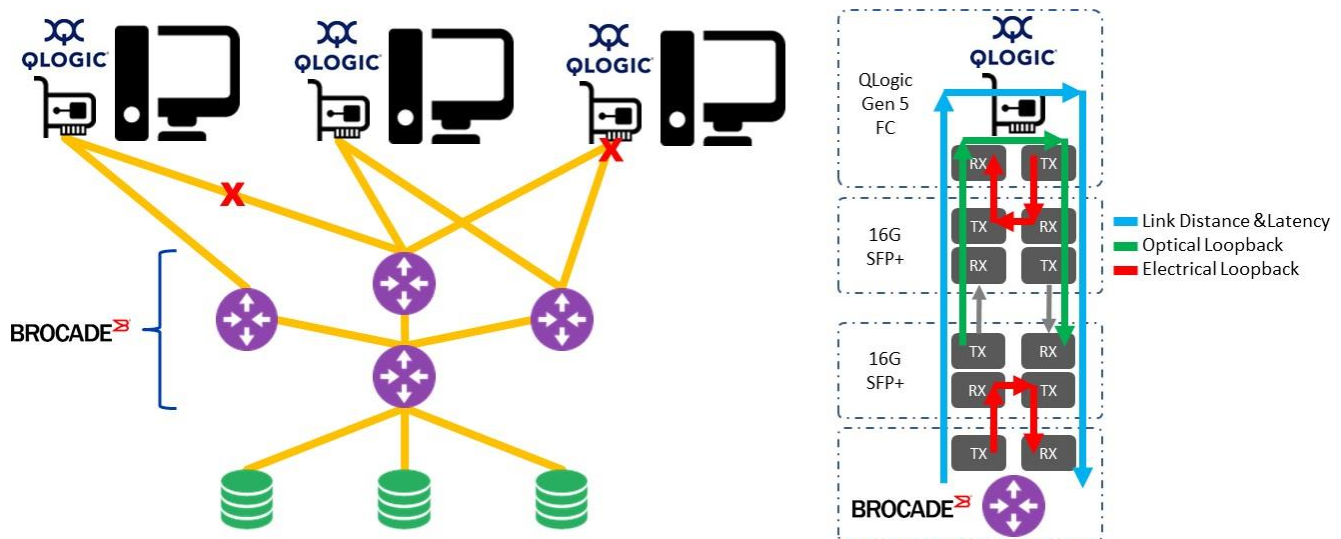
Figure 9. QLogic Enhanced Gen 5 FC with ClearLink Diagnostics (D_Port)
