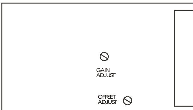
Figure 5.2 Showing the Potentiometers for Gain & Offset Adjustment
