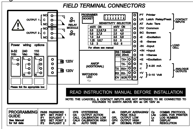
Figure 2.1 The LCA15F Field Connection Terminals
