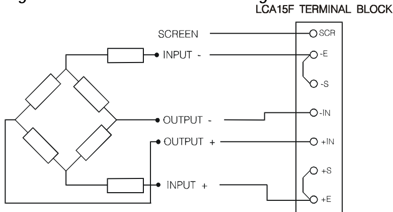
Figure 2.2 The 4 Wire Strain Gauge
