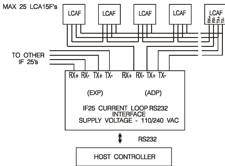
Figure 7.2 Connecting Multiple LCA15Fs
