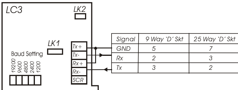
Figure 7.5 RS232 Mode Connection to PC
