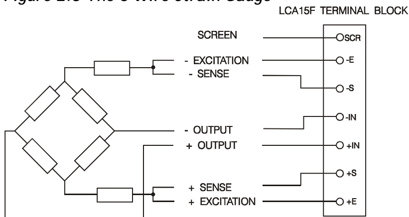
Figure 2.3 The 6 Wire Strain Gauge
