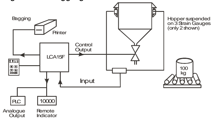
Figure 1.1 Bagging
