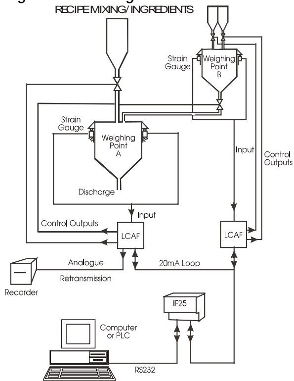
Figure 1.3 Mixing Control
