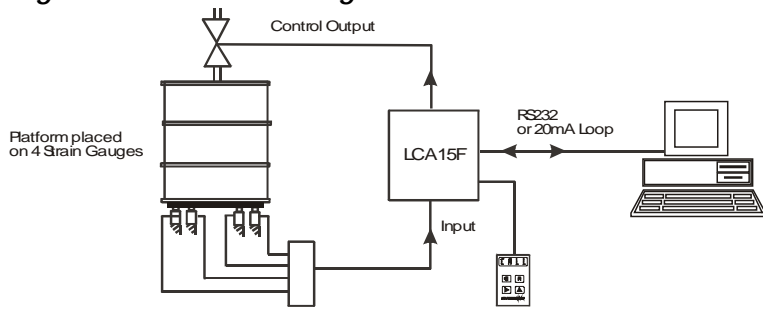
Figure 1.2 Drum Filling
