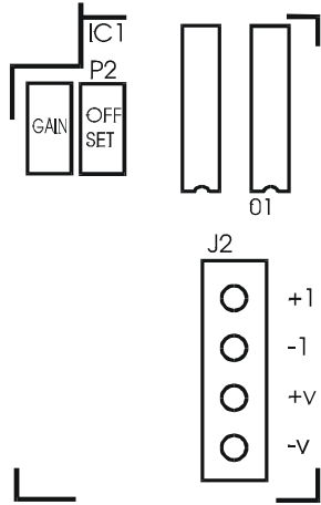
Figure 5.3 - UAFAO Connections
