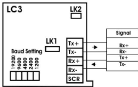
Figure 7.3 The LC3 Isolated RS232/485 - RS485 Mode Connections
