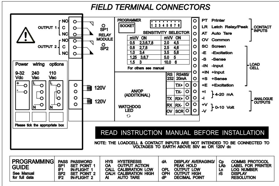
Figure 2.1 The LCA15 Field Connection Terminals
