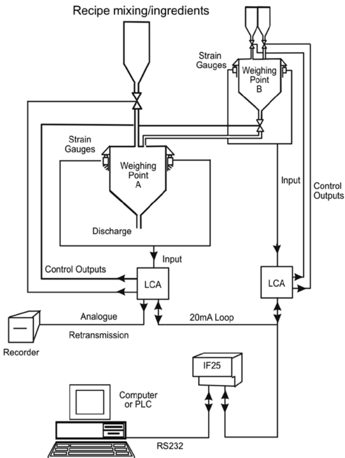
Figure 1.3 Mixing Control
