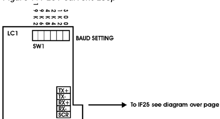
Figure 7.1 LC1 Current Loop
