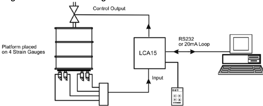
Figure 1.2 Drum Filling
