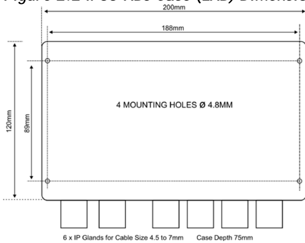
Figure 2.2 IP65-ABS Case (LAB) Dimensions & Mounting Points
