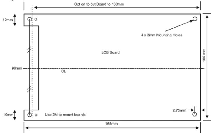
Figure 2.5 LCB Board
