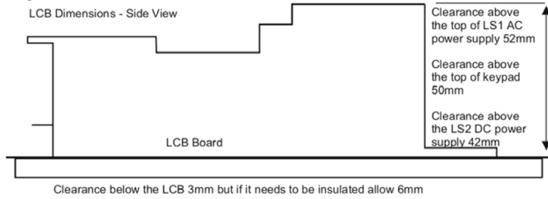
Figure 2.4 LCB Dimensions - Side View
