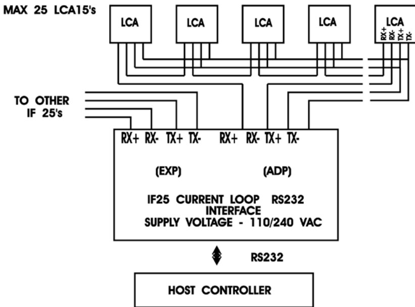
Figure 7.2 Connecting Multiple LCA15s
