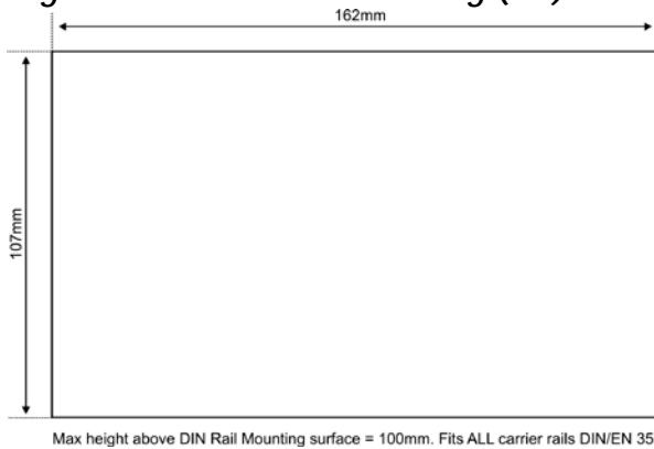
Figure 2.3 DIN Rail Mounting (D2) Dimensions
