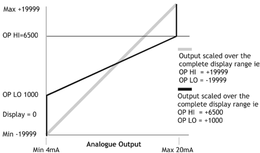
Figure 5.1 Analogue Output
