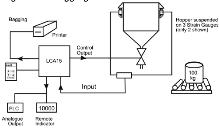
Figure 1.1 Bagging
