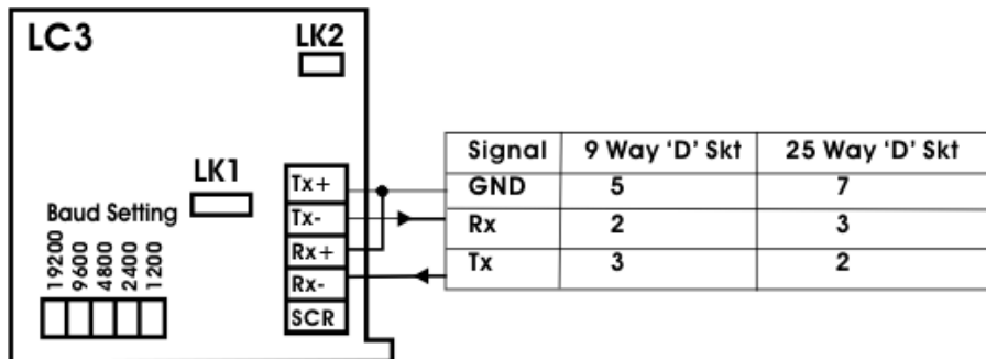
Figure 7.5 RS232 Mode Connection to PC
