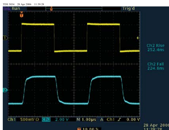
Figure 4.2: Response of the SIM983 to a 1.0 V peak-peak step, G = +4.00 , V_{ofs} = 0.000 V.
