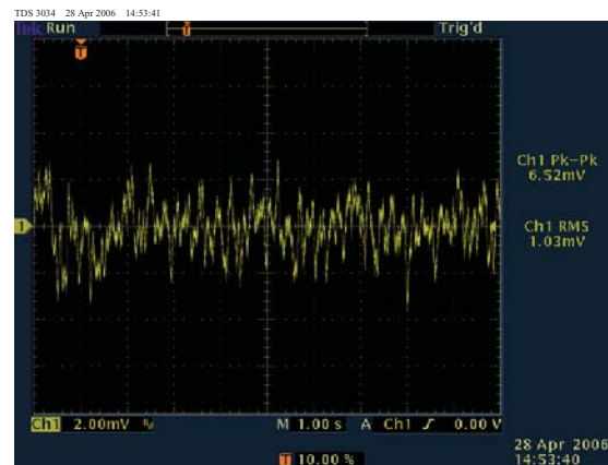
Figure 4.9: 0.1 Hz to 10 Hz noise of the SIM983, G = +19.99 , additional gain of 50.
