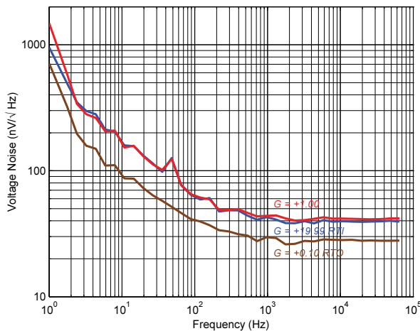
Figure 4.8: Noise of the SIM983, referenced to the input for |G| \geq 1 .
