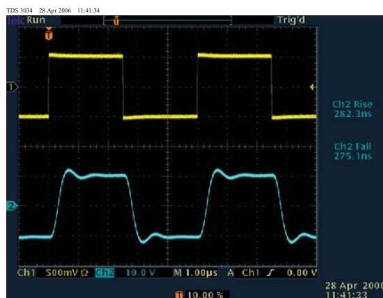
Figure 4.4: Response of the SIM983 to a 1.0 V peak-peak step, G = +19.99 , V_{ofs} = 0.000 V.
