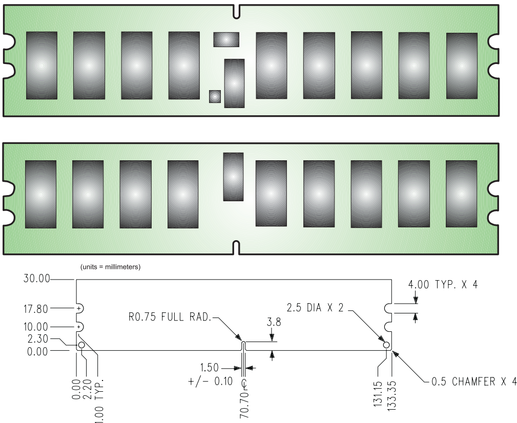
Figure 1: KVR667D2S4P5/2G 240-Pin DIMM
