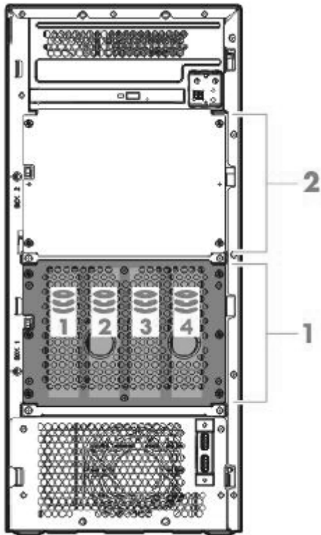
1-4 4 x LFF SATA/SAS/SSD Hot Pluggable Hard Drives Bays
