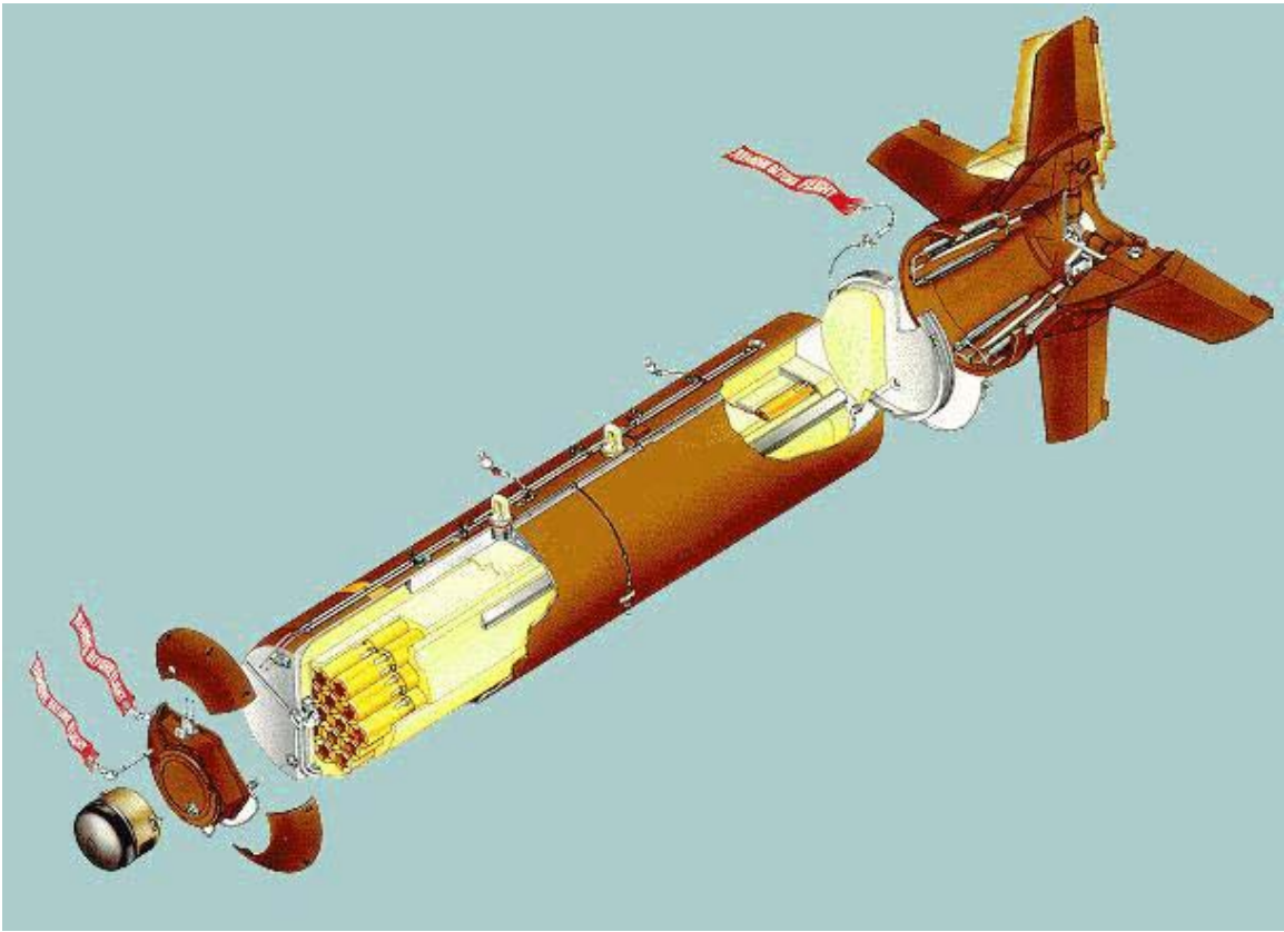
Diagram of a CBU-87 with cluster bomblets (BLU-97s) packed inside. Courtesy of Global Security.
