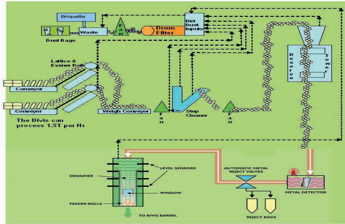
Block Diagram of the Bivis Dry End
