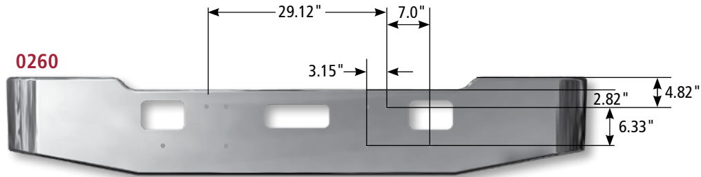
Freightliner® FLC-112
