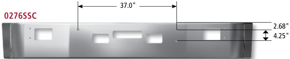
Freightliner® FLD 120
