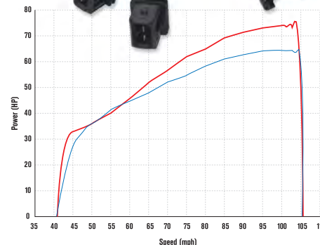
COBRA: Max Torque = 80.2 Max Power = 74.53 STOCK: Max Torque = 73.1 Max Power = 64.37
