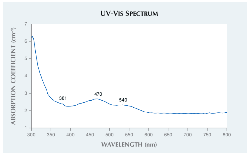
Figure 11. UV-Vis spectrum of this orangy pink euclase. The 470 and 540 nm absorption peaks probably originated from \text{Mn}^{3+} and the 381 nm peak from \text{Fe}^{3+} .
