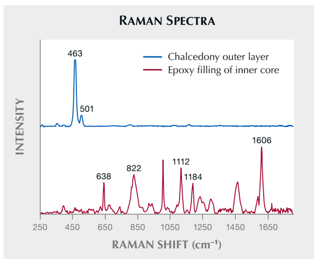
Figure 15. The Raman spectra of the outer layer and the inner core of the beads matched those expected for chalcedony (K.J. Kingma and R.J. Hemley, “Raman spectroscopic study of microcrystalline silica,” American Mineralogist , Vol. 79, 1994, pp. 269–273) and epoxy resin (K.E. Chike et al., “Raman and near-infrared studies of an epoxy resin,” Applied Spectroscopy , Vol. 47, No. 10, 1993, pp. 1631–1635). The stacked spectra are baseline-corrected and normalized.
