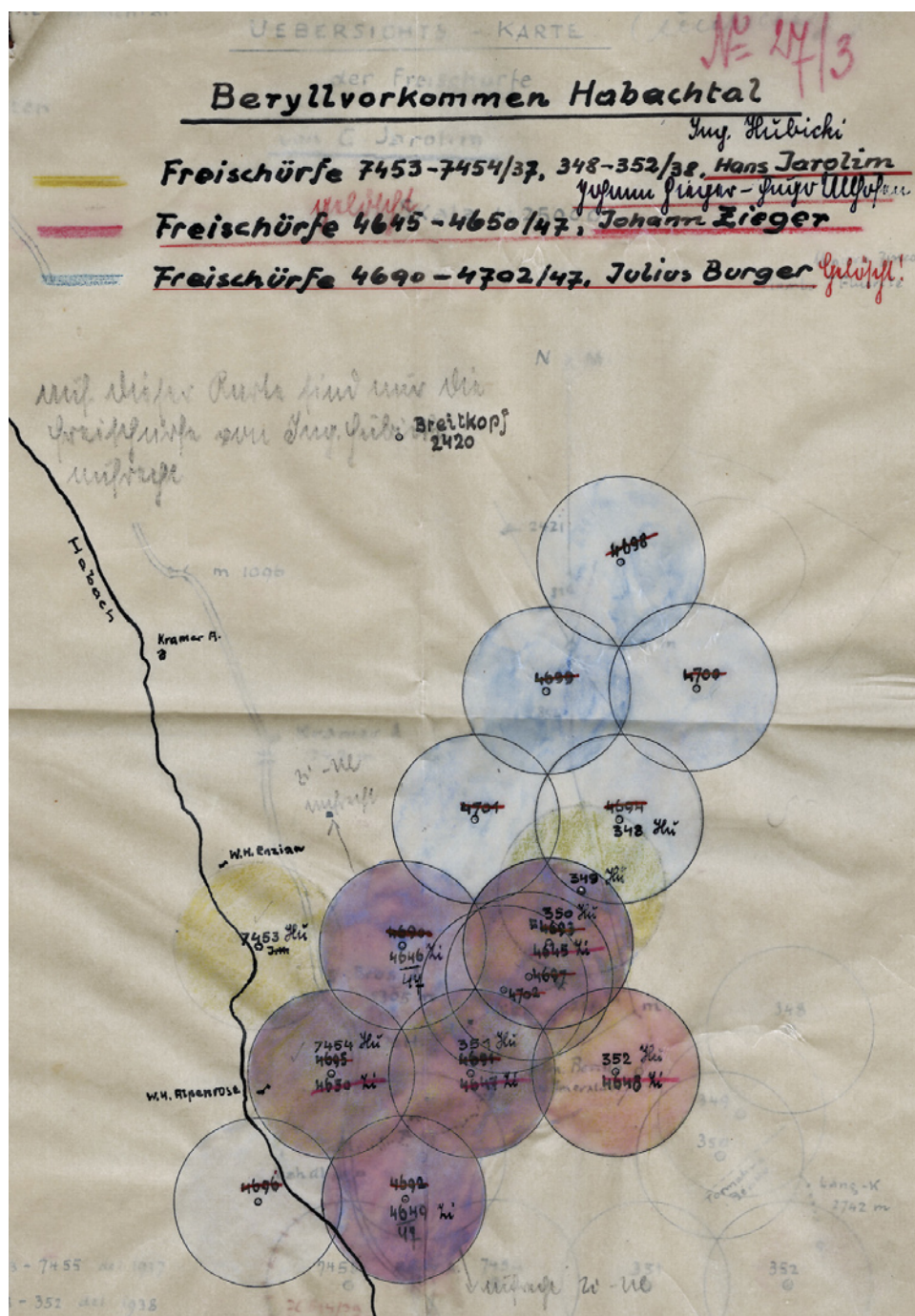
Figure 10. Under Austrian law, overlapping exploration permits could be granted to multiple parties, as seen in this map for the area of the Habachtal emerald mine from the 1940s and 1950s. Three different individuals—Hans Jarolim (greenish yellow), Johann Zieger (purple), and Julius Burger (blue)—had each been authorized to perform activities over several circles with a radius of 425 m each. File Beryl Bramberg, Collection of W. Günther, Archive of the Bergbau- und Gotikmuseum Leogang.
