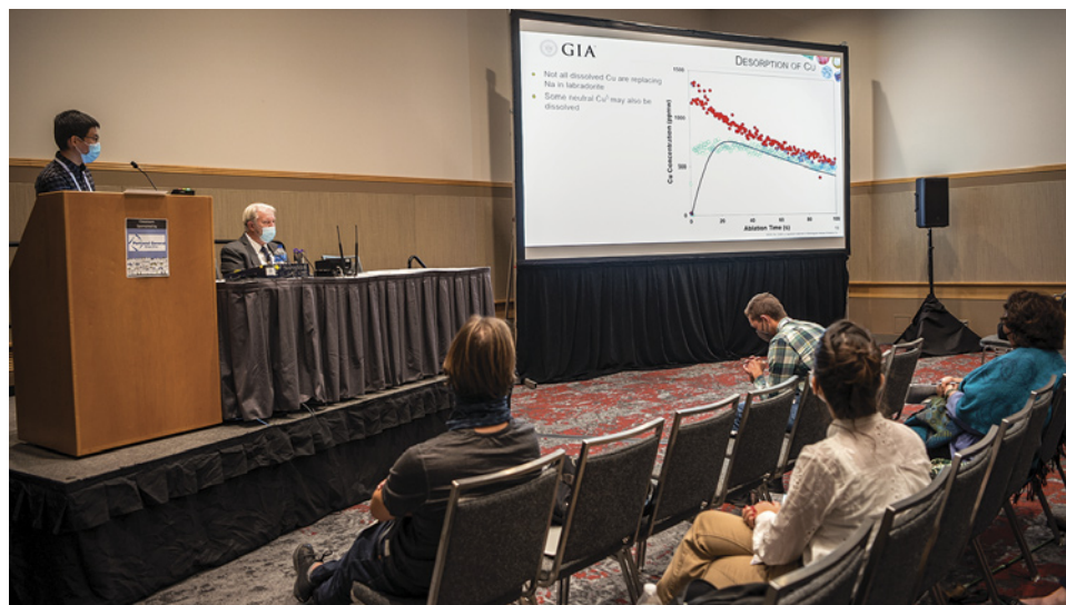
Figure 21. Speaking at the GSA annual meeting, Shiyun Jin of GIA presents his research on the rapid diffusion of copper in Oregon sunstones. Photo by Robert Weldon.
