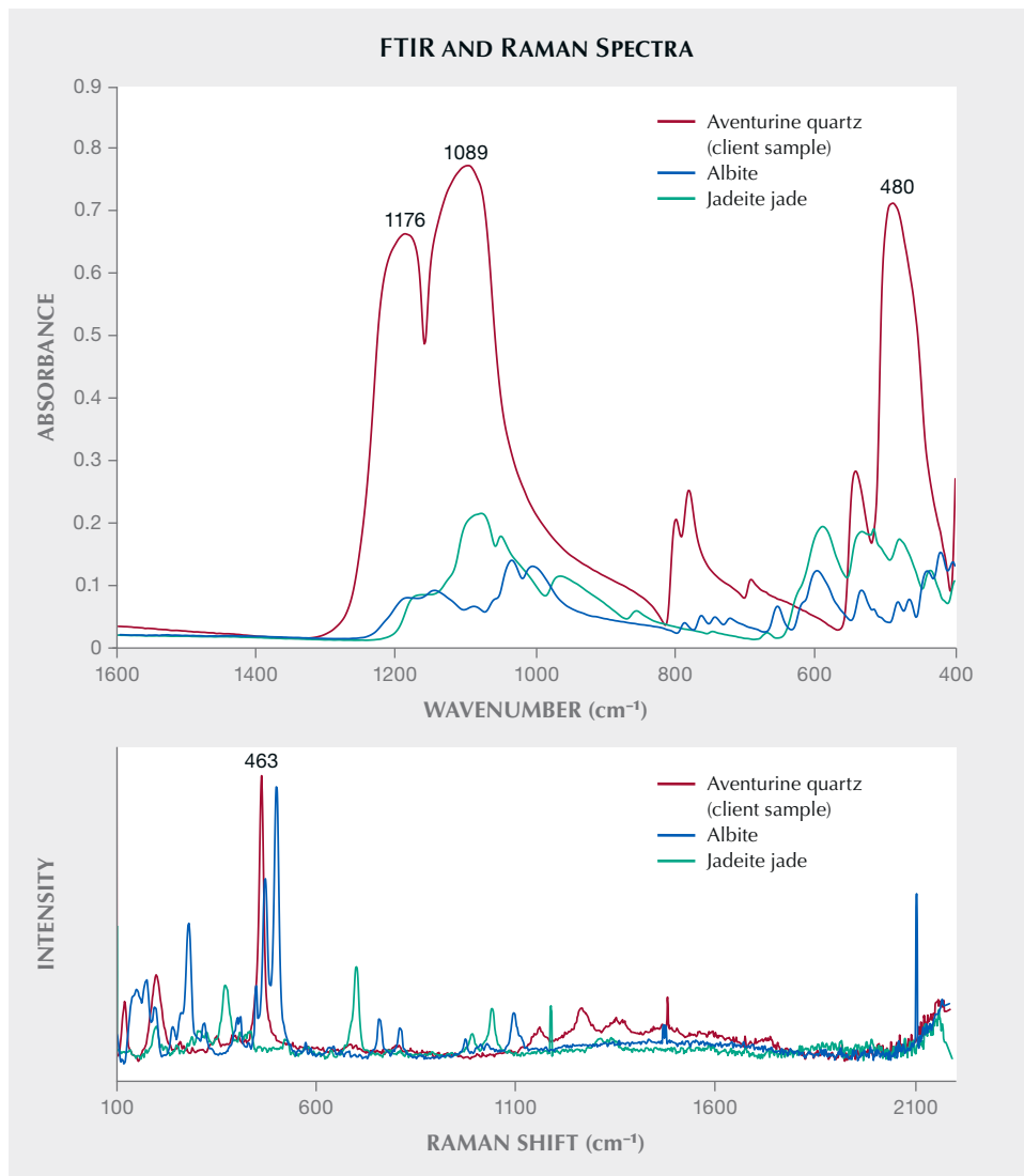
Figure 19. FTIR (top) and Raman (bottom) spectroscopy confirmed the client's bangle was fashioned from aventurine quartz. Peaks observed in the FTIR spectra (main peaks at 1176, 1089, and 480 \text{cm}^{-1} ) and Raman spectra (main peak at 463 \text{cm}^{-1} ) did not match those expected for albite or jadeite jade. FTIR and Raman spectra of aventurine quartz were collected from the client's sample; spectra of albite and jadeite jade were from the author's database.
