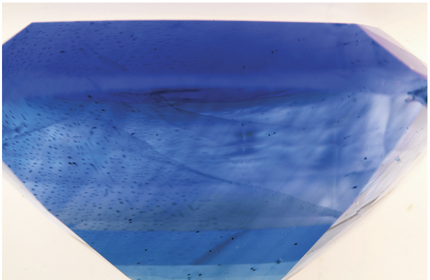
Figure 21. When immersed in mineral oil, curved color banding is visible along with a natural-looking flux fingerprint and large gas bubbles. Field of view 7.19 mm.
