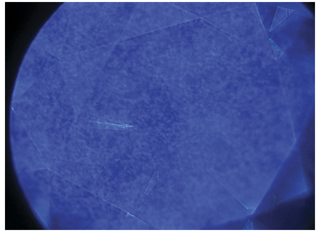
Figure 10. This diamond's blue fluorescence provides strong contrast to the inert radiation stains, as shown by the DiamondView. Image by Michaela Stephan; field of view 8.265 mm.
