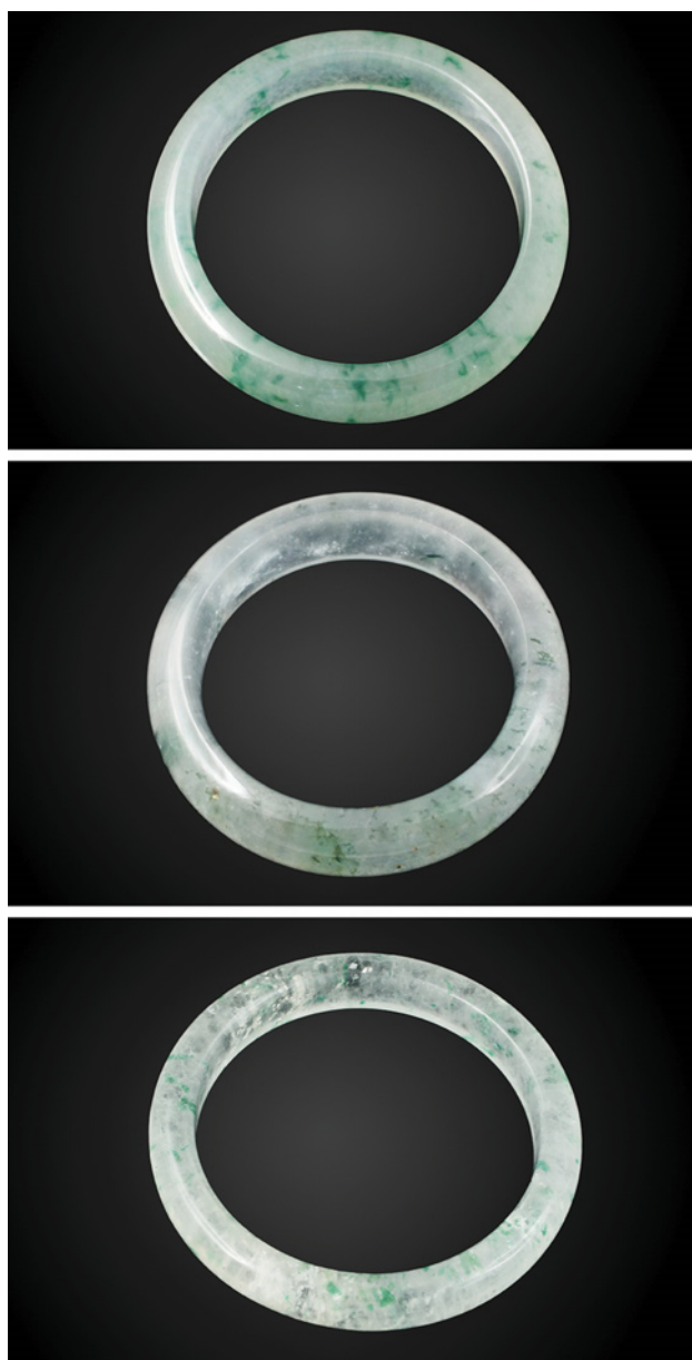
Figure 18. Bangles of similar appearance fashioned from different materials: jadeite jade (top), albite (middle), and aventurine quartz (bottom, client sample). All exhibit green “floating flower” inclusions. Photos by Lai Tai-An Gem Lab.
