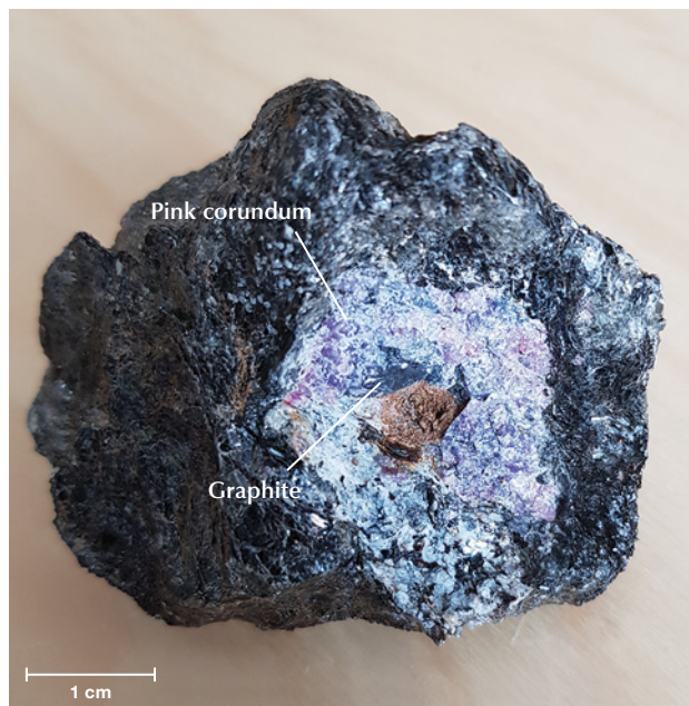
Figure 2. Pink corundum from the Maniitsoq locality containing a macroscopic inclusion of graphite. Photo by Kristoffer Szilas.
