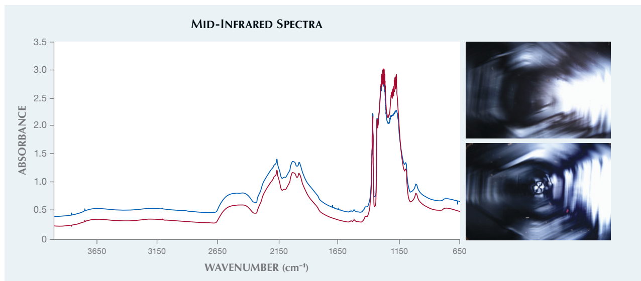
Figure 6. Left: Overlapping mid-infrared spectra of both lenses revealed them to be type Ia diamonds. Right: Two strain images, one of each lens, under cross-polarized light showing natural growth structure and internal stress during natural diamond formation. Field of view 19.27 mm.
