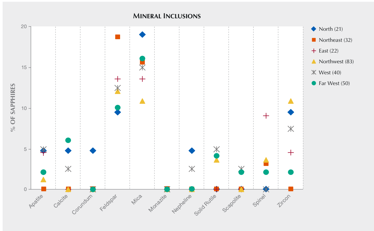
Figure 23. This graph shows the percentage of the samples that contained at least one conclusively identified crystal. The most common crystals in Mogok sapphire are feldspar and mica. The numbers in parentheses represent the number of samples from each area.
