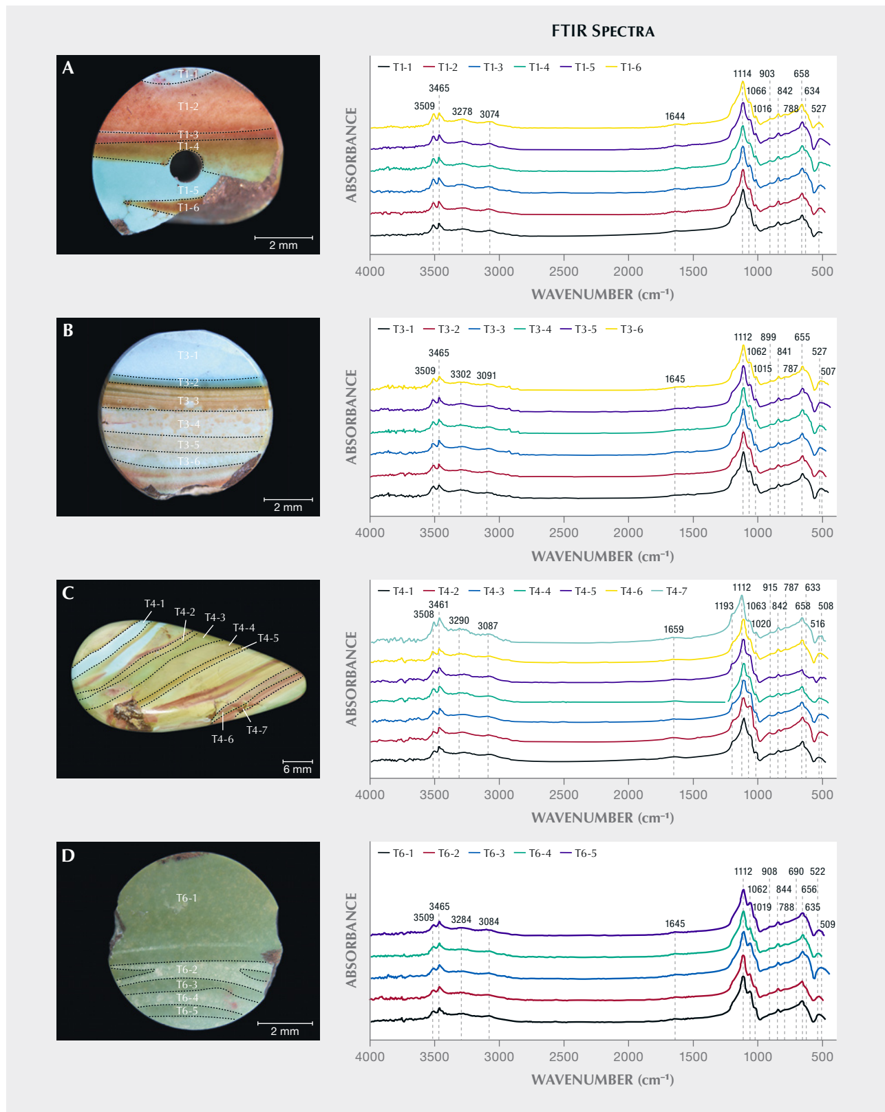
Figure 8. Division of bands and FTIR spectra of specimens T1, T3, T4, and T6, which were sliced open. A: T1-1 through T1-6, six bands. B: T3-1 through T3-6, six bands. C: T4-1 through T4-7, seven bands. D: T6-1 through T6-5, five bands. Photos by Tianting Lei.
