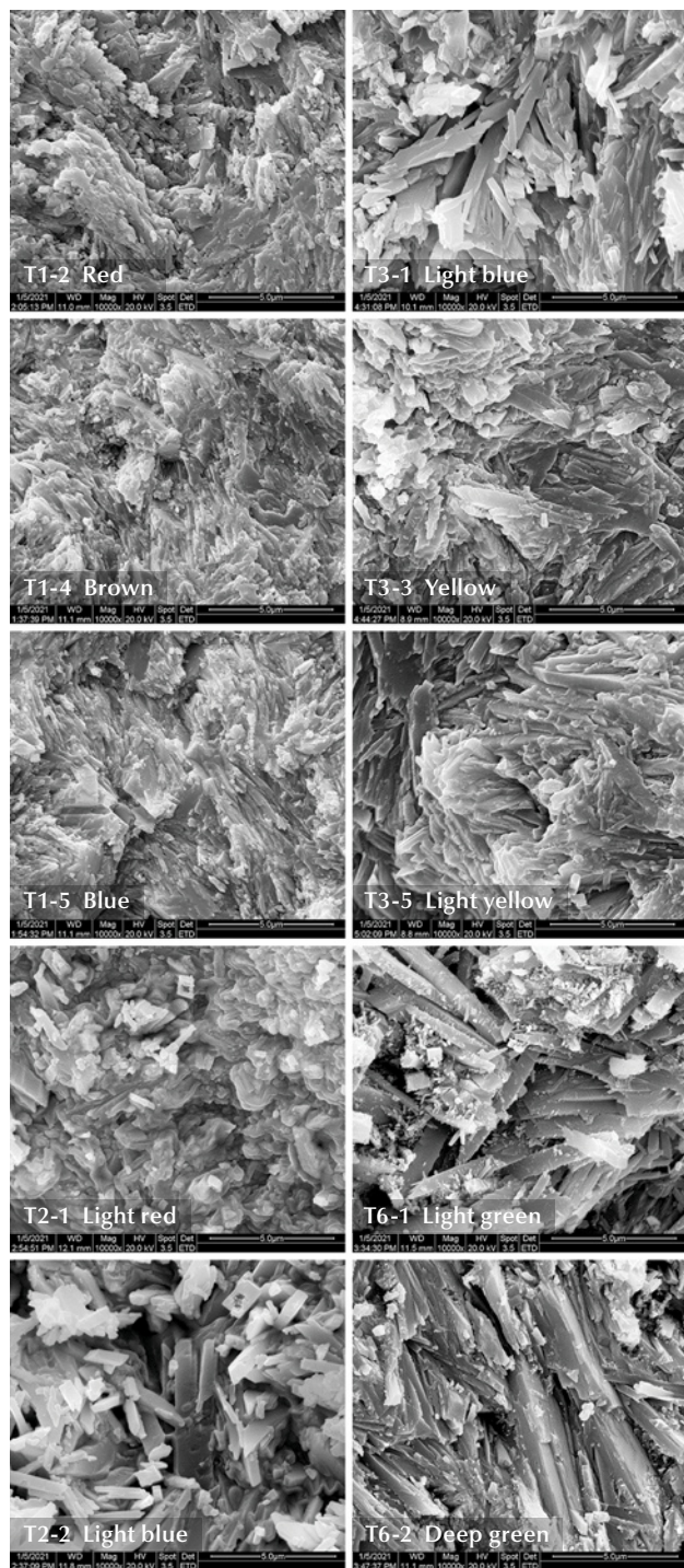
Figure 9. SEM microtopography of different bands in samples T1, T2, T3, and T6. Images by Tianting Lei; field of view 13.5 µm.
