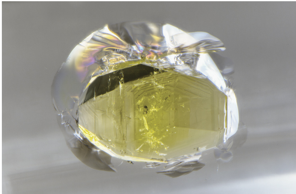
Figure 13. The transparent yellow monazite (?) inclusion in the rock crystal quartz and the stress cracks immediately surrounding it are both clearly visible in this image. Photomicrograph by Nathan Renfro; field of view 4.86 mm.
