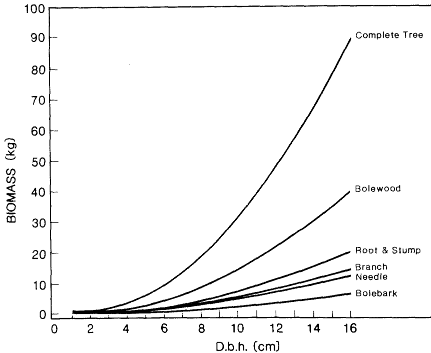
Figure 2.—Relationship of black spruce component biomass and d.b.h. as predicted by regression equations.
