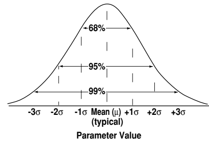
Figure 24. Normal Distribution.
