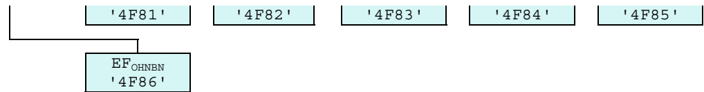
Figure 4.2: File identifiers and directory structures of USIM
