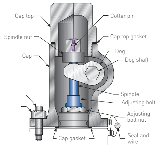
Packed lifting lever Type D
