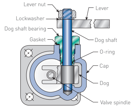
Packed lifting lever Type D (top view)
