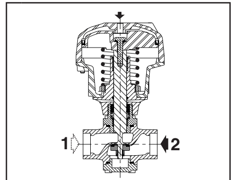
NC function
