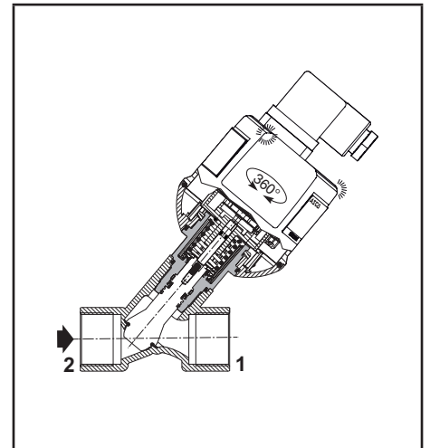
DC construction
