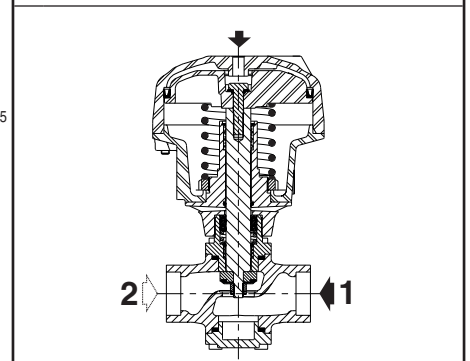
NC function
