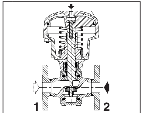
NC function
