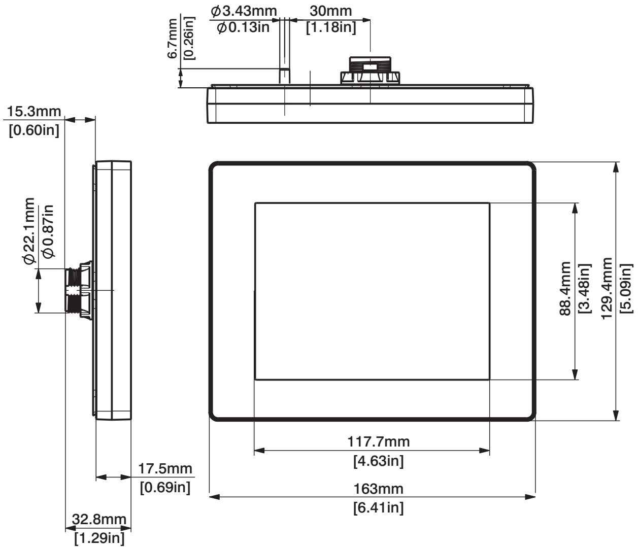
Figure 10.4: MDLN Dimensions
