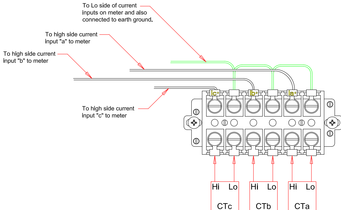
Figure 4.4: EI SB-6TC Shorting Block Wiring Diagram
