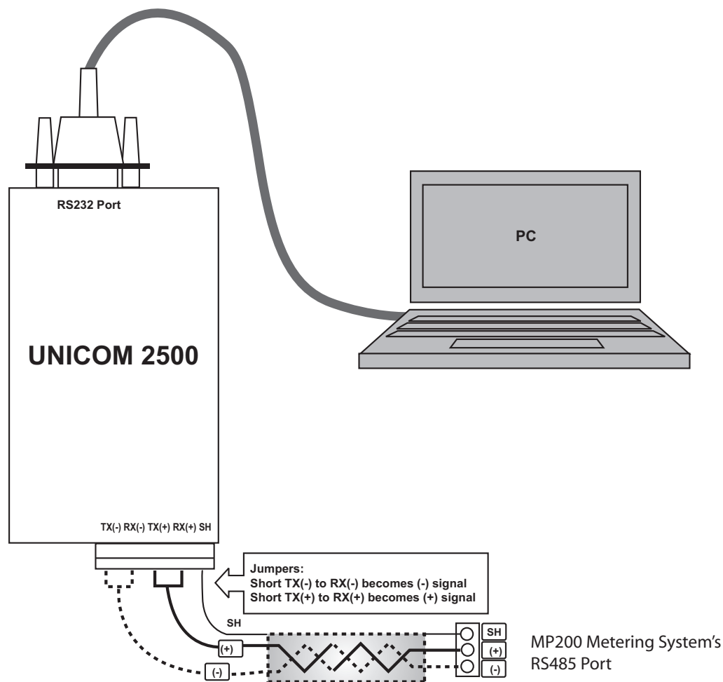
Figure 5.6: Unicom 2500 with Connections
