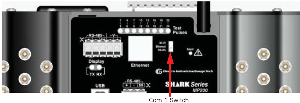
Figure 10.12: Com 1 Switch Set to Ethernet/WiFi
