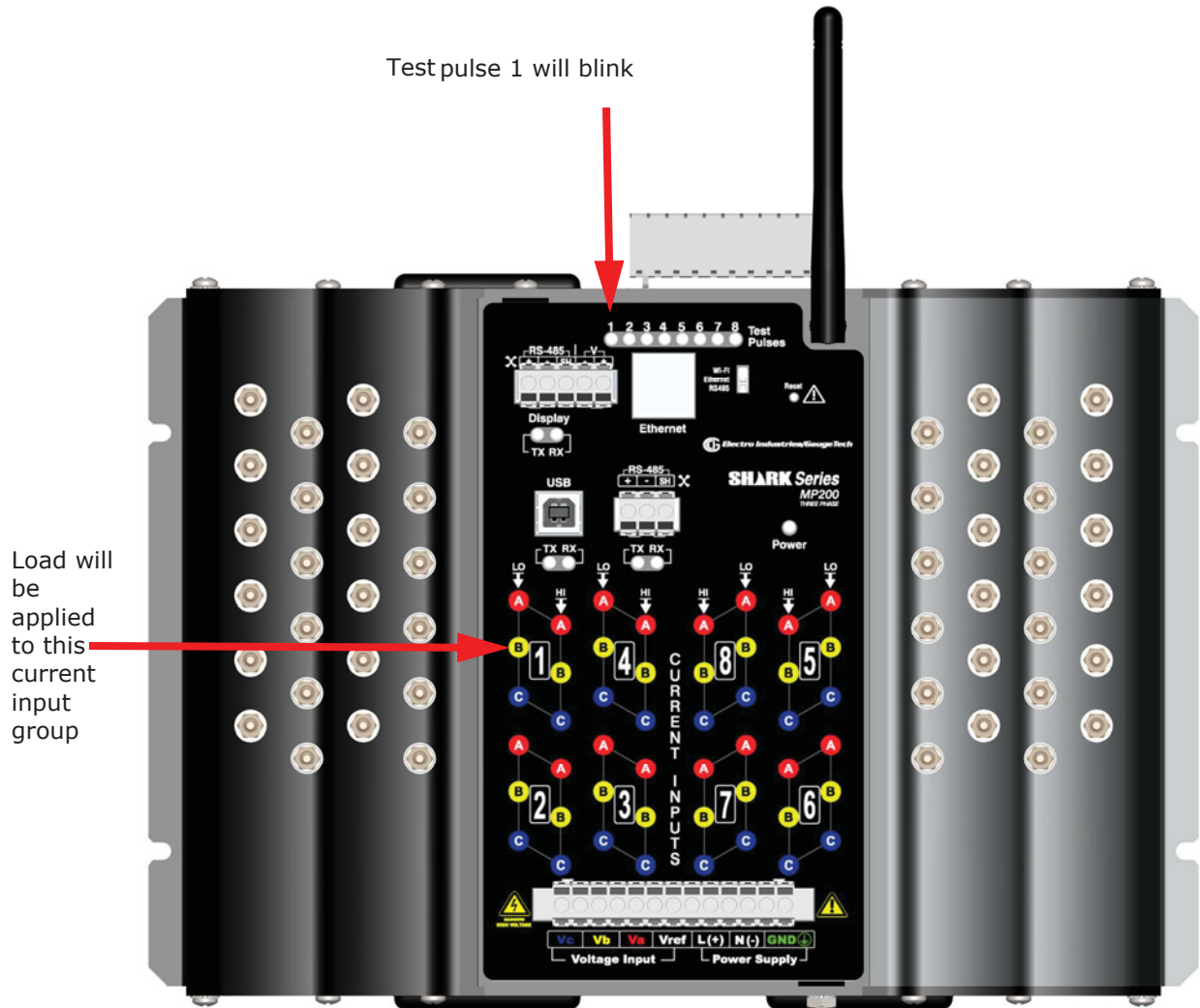
Figure 6.1: Meter 1 and Test Pulse 1 for MP200-Y Unit
