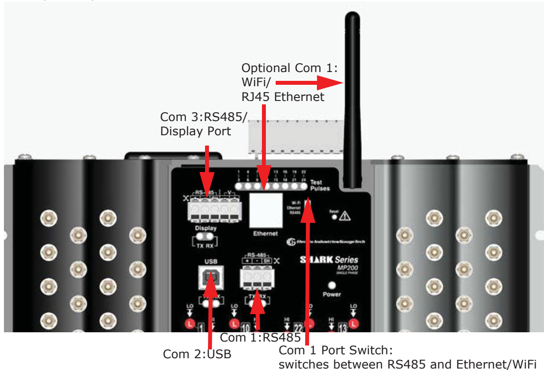
Figure 5.1: MP200 Unit Communication Ports
