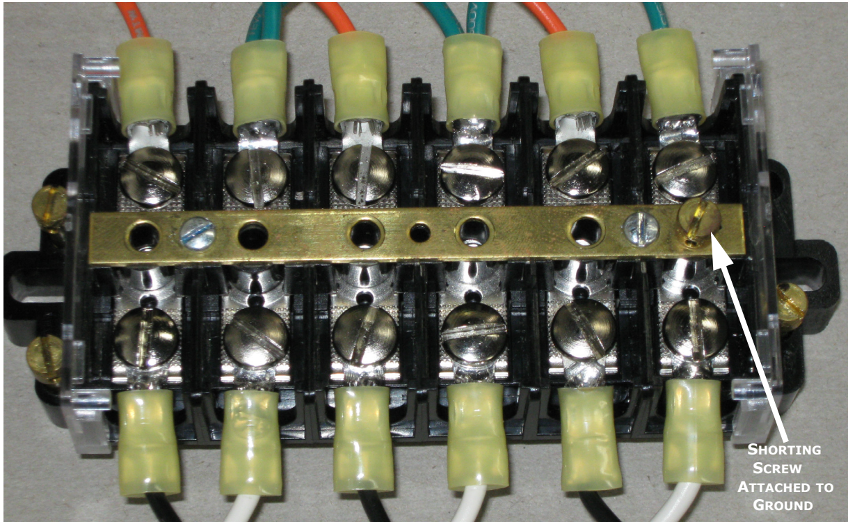
Figure 4.6: EI SB-6TC with Shorting Screw Attached to Ground Terminal
