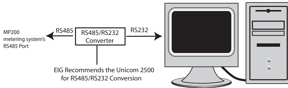
Figure 5.2: MP200 Unit Connected to a PC via RS485 bus
