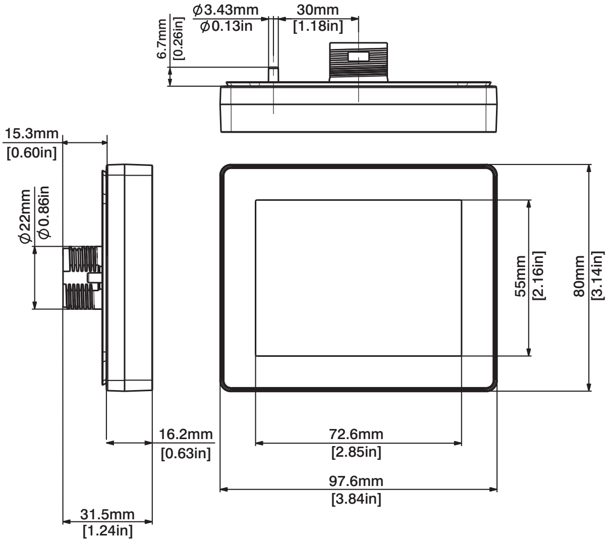
Figure 10.3: MDSN Dimensions
