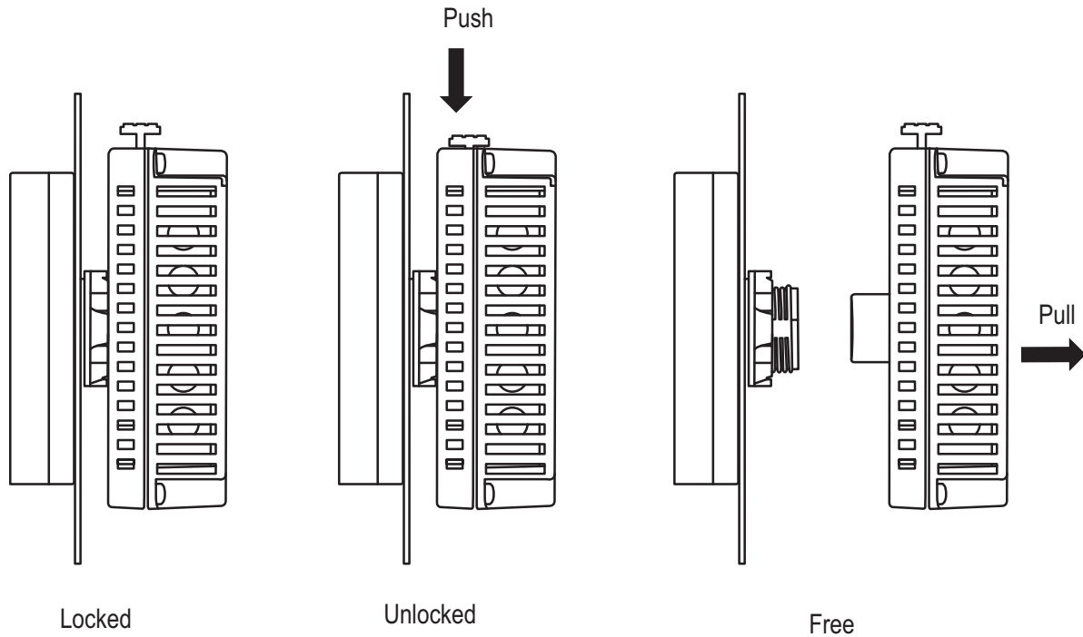
Figure 10.11: Removing the Rear Module from the Display Module
