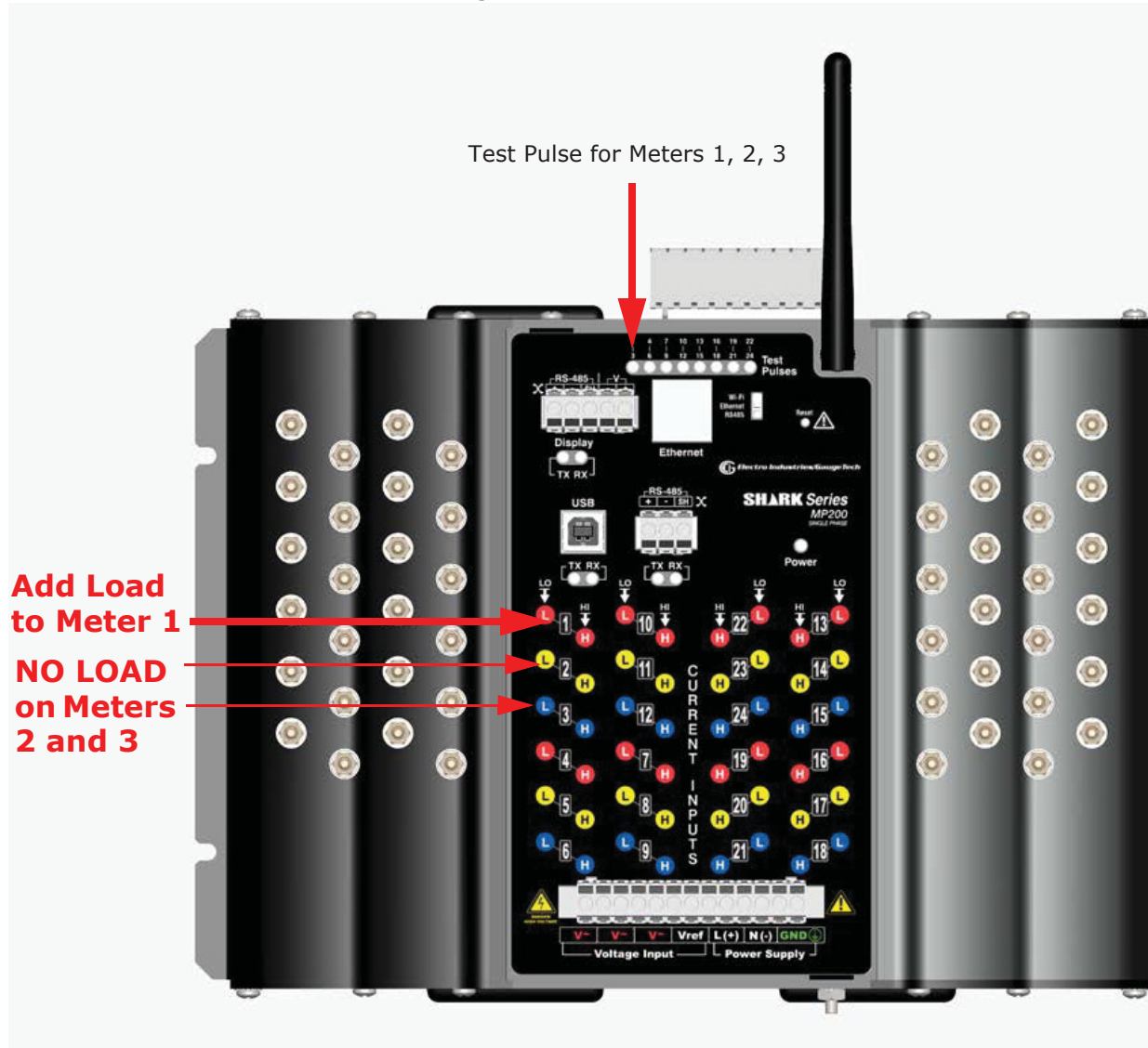
Figure 6.2: Meter 1 and Test Pulse 1 for MP200-S Unit: NO LOAD on Meters 2 and 3
