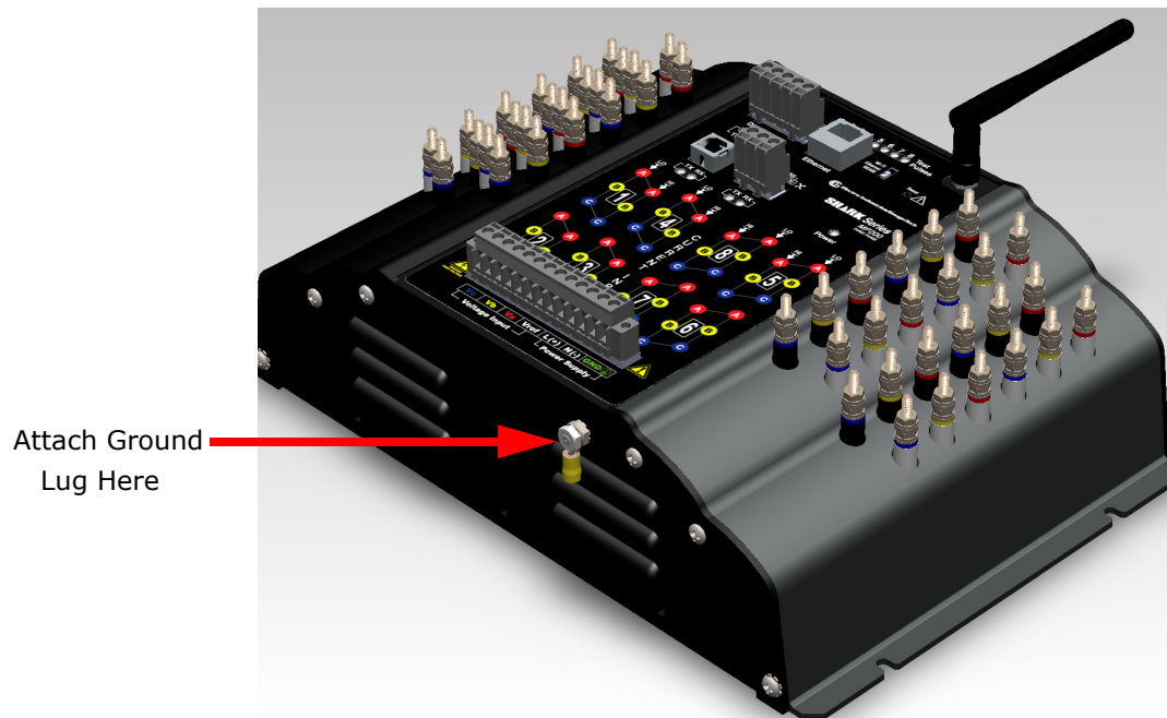
Figure 4.1: Ground Lug Connection
