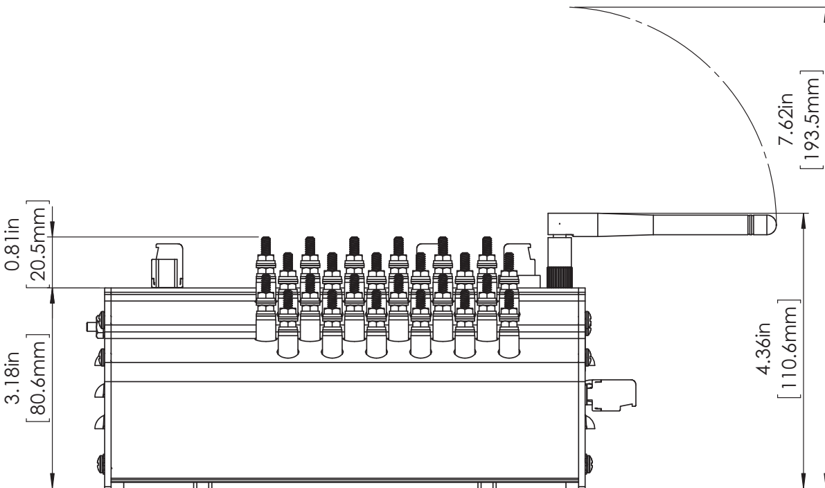
Figure 3.2: MP200 Unit Side Dimensions
