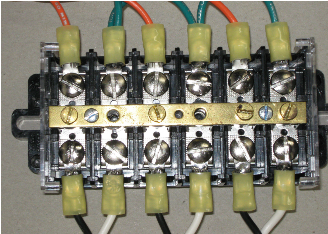
Figure 4.7: EI SB-6TC with All CTs Shorted Properly
