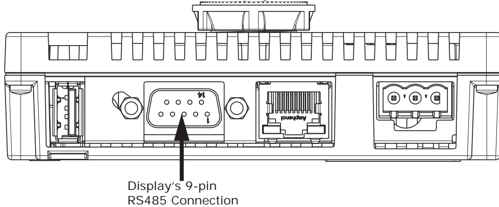
Figure 10.11: Display's RS485 Connection
