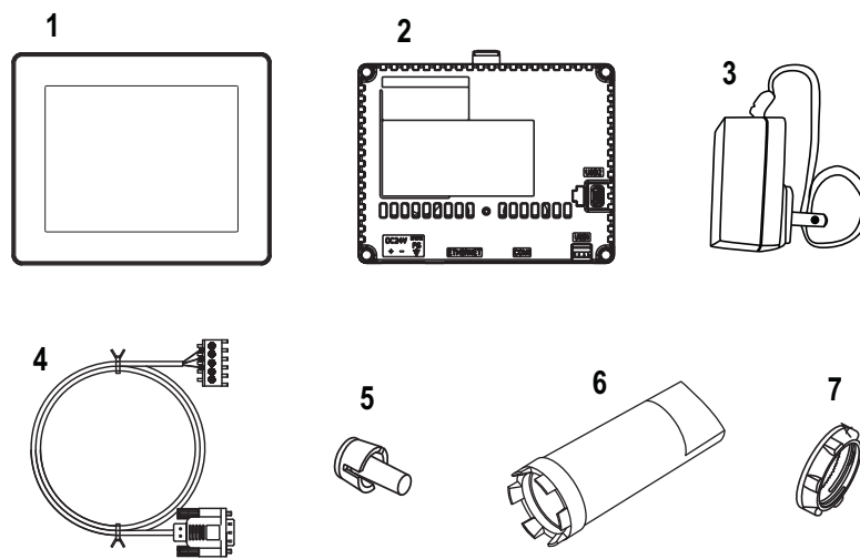
Figure 10.2: Display Kit Contents
