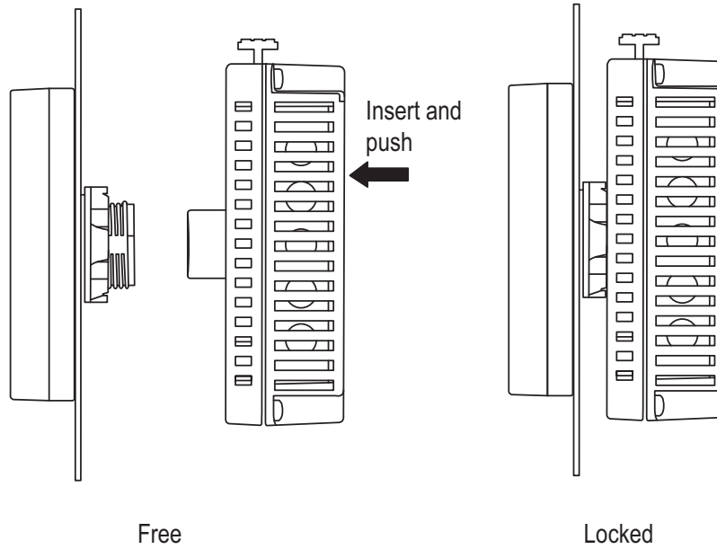
Figure 10.10: Connecting the Rear Module to the Display Module
