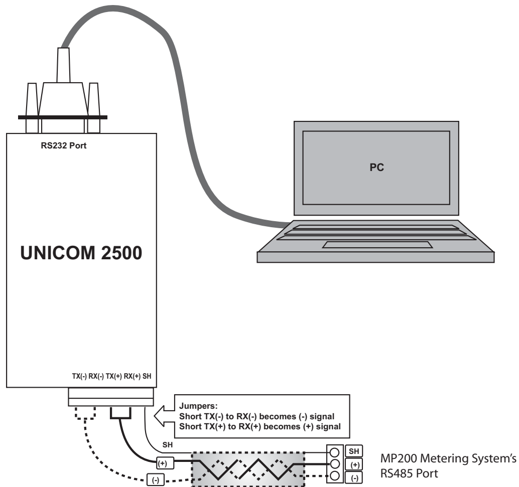
Figure 5.6: Unicom 2500 with Connections
