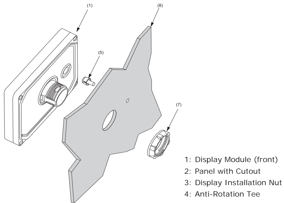
Figure 10.8: Installation Components
