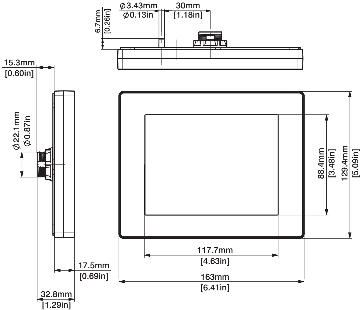
Figure 10.4: MDLN Dimensions
