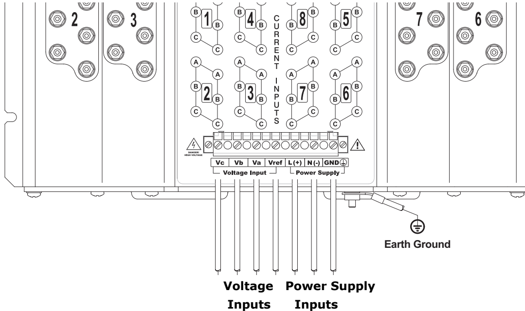
Figure 4.2: MP200 Unit Connections
