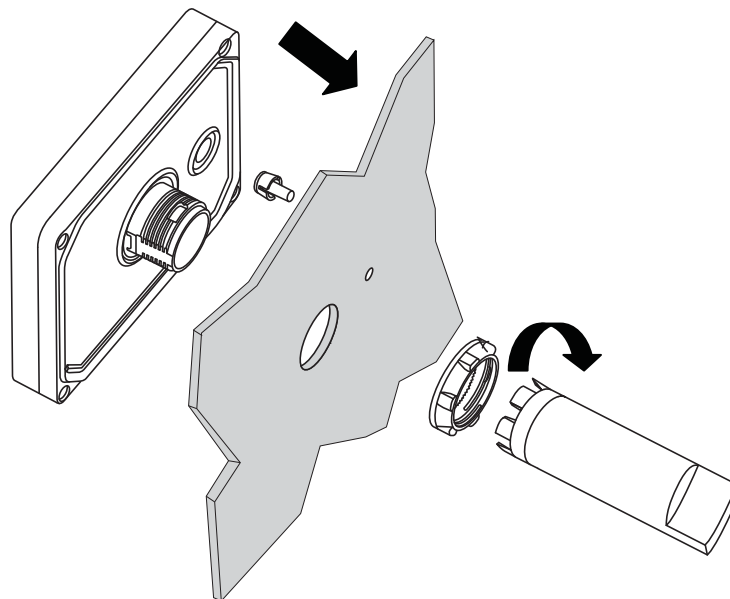
Figure 10.9: Attaching the Nut Using the Socket Wrench
