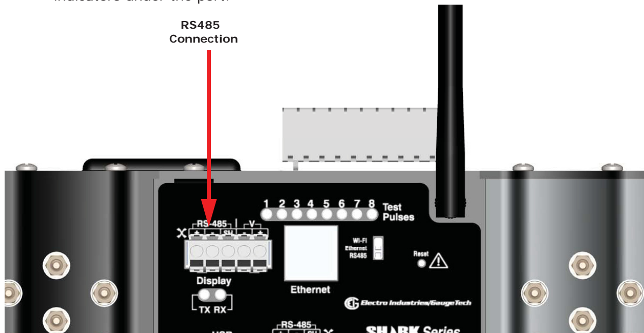
Figure 5.9: Com 3 RS485/Display Port
