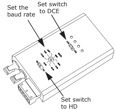
Figure 5.7: Unicom 2500 Settings
