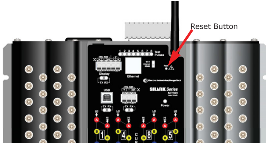
Figure 8.3: Location of Reset Button
