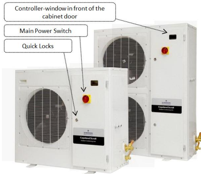
Figure 2: ZX unit housing
