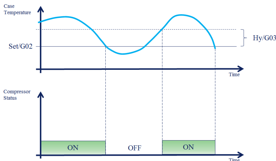
Figure 9: External temperature sensor – Functionality
