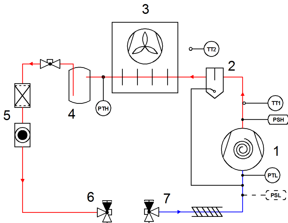
Figure 5: P&I diagram for ZXDE units
