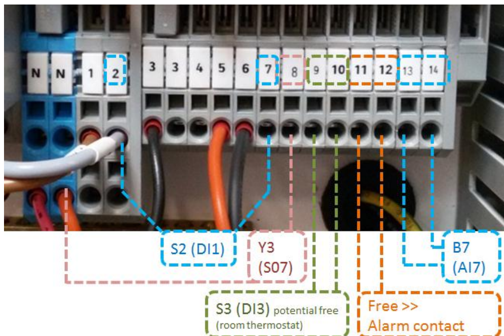
Figure 8: Prearranged additional connections
