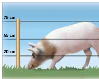
Electric fences for pigs are 0.55 to 0.75 m high with 2 to 3 wires. Outer fences for domestic pigs should have a second fence to protect against wild animals.
