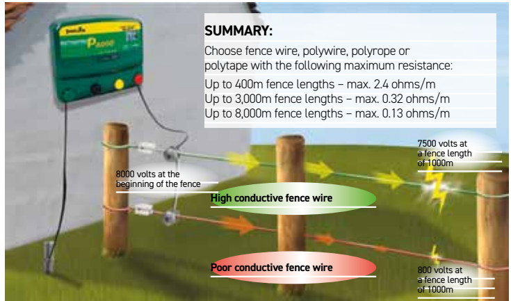
In longer fence lengths, only high conductivity fence wires ensure maximum performance to the end of the fence.
