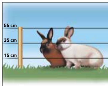
Electric fences for protecting against rabbits are approx. 0.55 m high with 3 wires. With rabbits, in order to prevent them digging under the fence, it may be necessary to lay an earthed wire directly on the ground. The fence should be slightly canted towards the animals.
