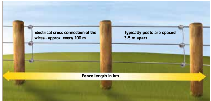
No vegetation - no contact between the vegetation and the fence wire
