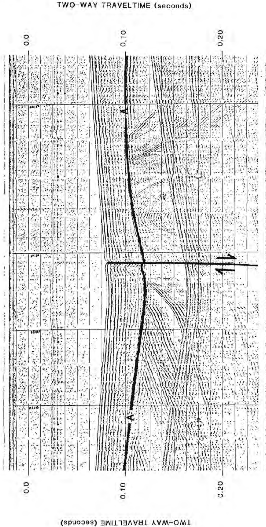
Figure 7-1 University of Washington seismic profile 10-14.
