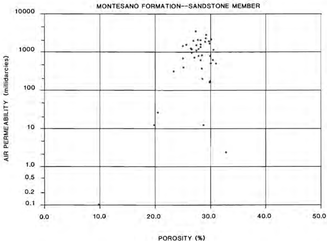
Figure 4-5 Plot of porosity vs. permeability for the sandstone member of the Montesano Formation.
