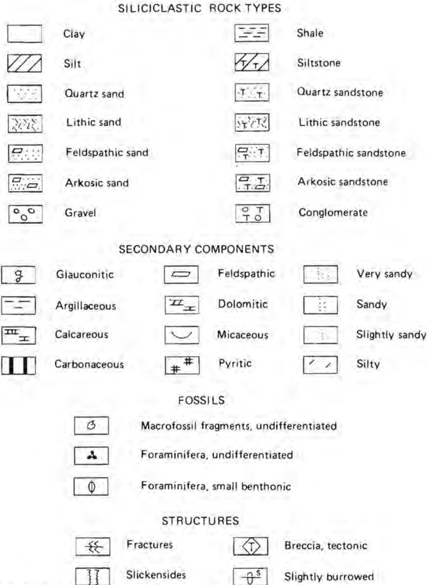
Figure 3-2 Symbols used on lithologic columns (from Swanson, 1981).
