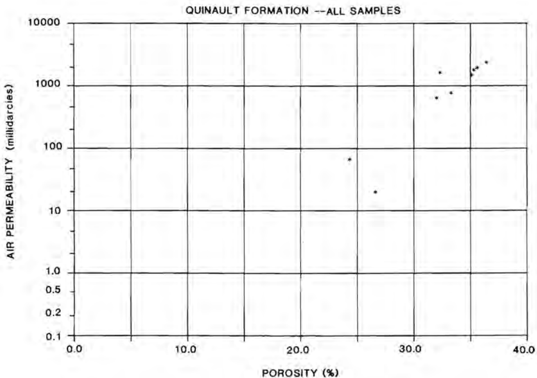
Figure 4-7 Plot of porosity vs. permeability for the Quinault Formation.
