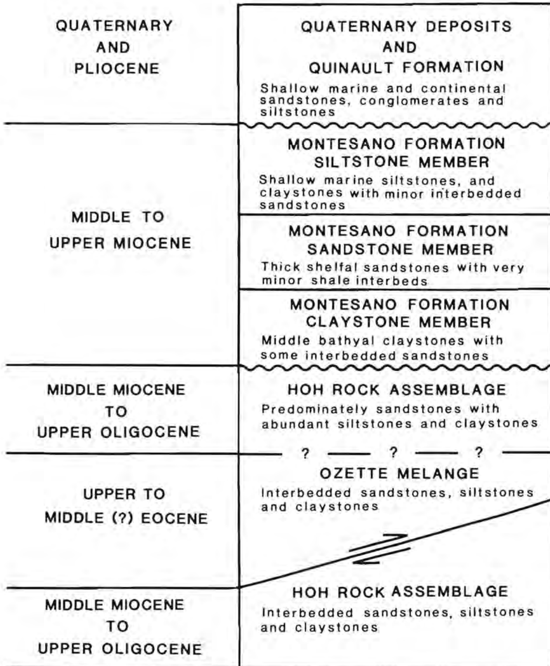
Figure 6-1 Generalized lithostratigraphic penetrated in Ocean City wells.
