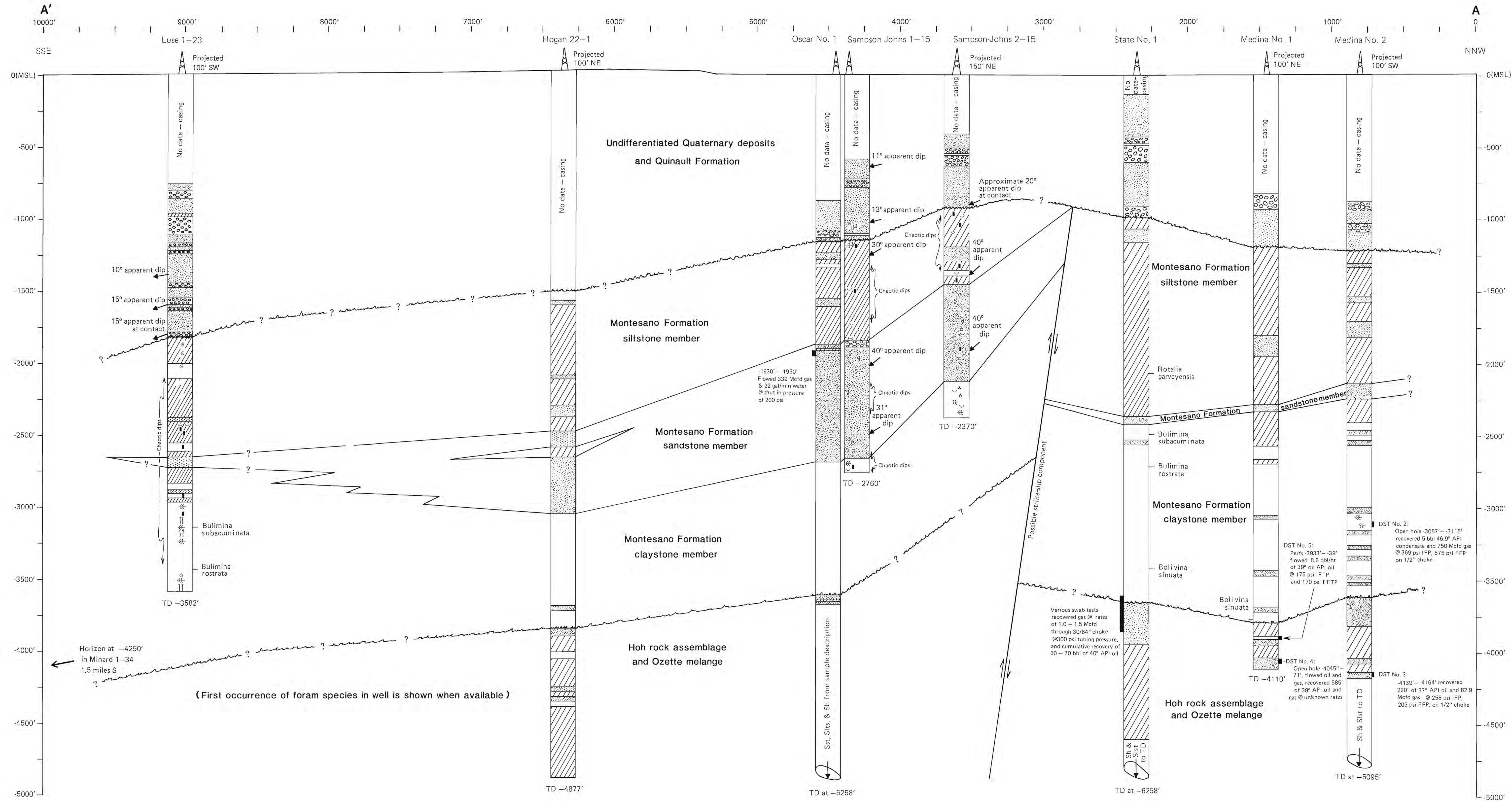
PLATE 6 CROSS SECTION OF OCEAN CITY AREA WELLS
