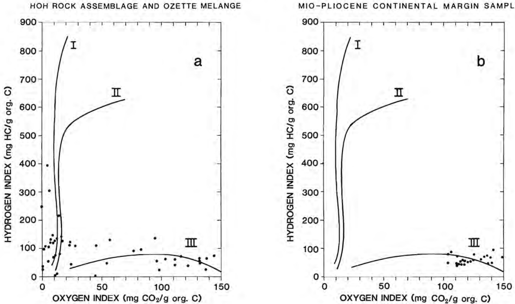
Figure 5-2 Van Krevelen diagrams for the Hoh and Ozette and for the Montesano and Quinalt sequences. Some data provided by EXLOG, Inc., 1989.
