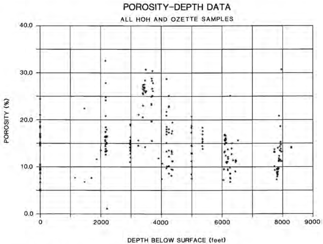
Figure 4-2 Plot of porosity vs. depth for Hoh and Ozette rocks.
