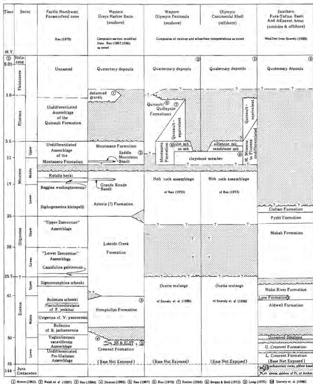
Figure 2-2 Stratigraphic columns for the Olympic Peninsula, Grays Harbor Basin, coastal Washington, and the Washington continental shelf.
