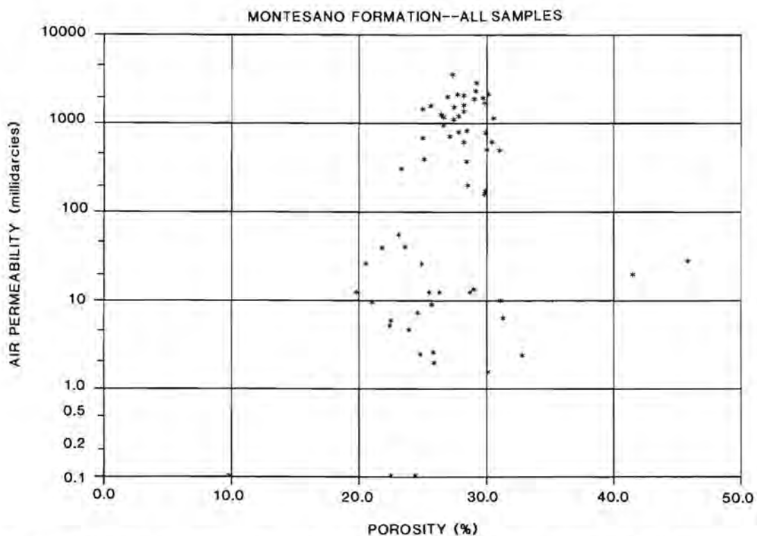
Figure 4-4 Plot of porosity vs. permeability for samples of all samples of the Montesano Formation.
