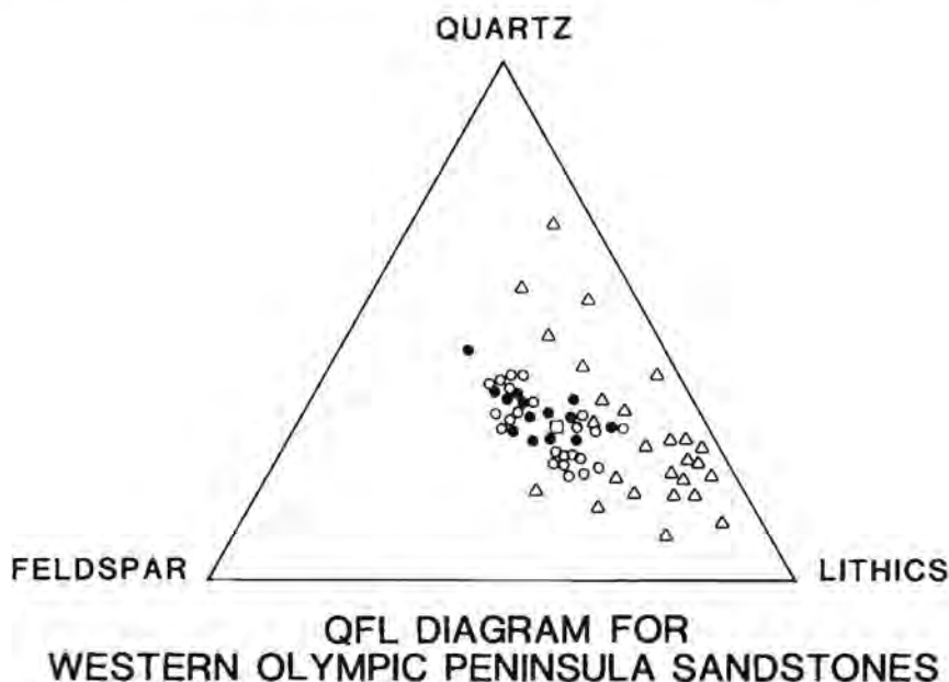
Figure 3-1 QFL plot for various sandstones from the western Olympic Peninsula. Ozette, square; Hoh, dots (Grady, 1985); Montesano, circles (Bigelow, 1987); Quinault, triangles (Horn, 1969).
