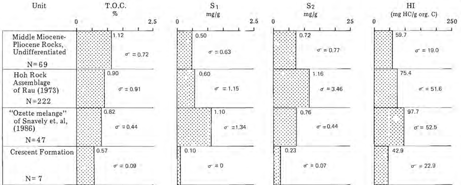
Figure 5-1 Histograms showing some geochemical characteristics of Washington continental margin strata. Some data provided by EXLOG, Inc., 1989.
