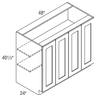
B4840FH Vertical divider
