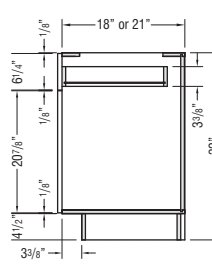
32" HIGH VANITY CABINET
