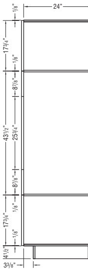
SINGLE OVEN CABINET
