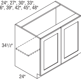
B24FH-B36FH Butt doors B39FH-B48FHCS Center mullion
