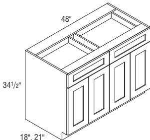
VB4834 - Vertical divider
