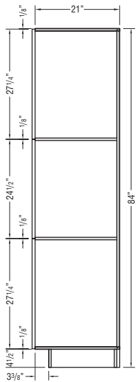
VANITY UTILITY CABINET
