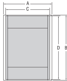
Appliance Trim Panel Max Cut-out (Shaded)
