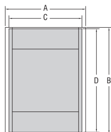
Appliance Trim Panel Max Cut-out (Shaded)
