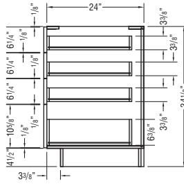
FOUR-DRAWER BASE CABINET
