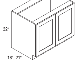
V3932 _ -V4832 _ CS Center mullion
