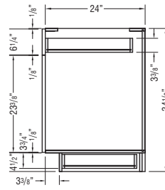
BASE CABINET with TOEKICK DRAWER
