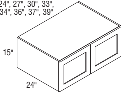
W241524-W371524 Butt doors W391524 Center mullion
