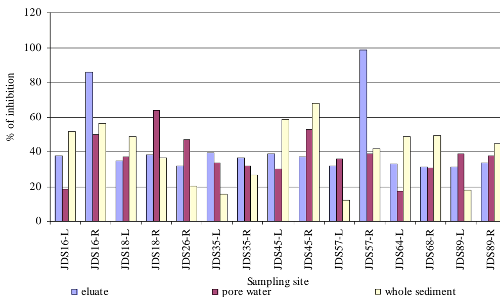
Figure 38: Inhibition of light emission of dry sediment fraction eluate (30 minute exposition) versus pore water (30 minute exposition) and whole sediment (5 minute exposition)
