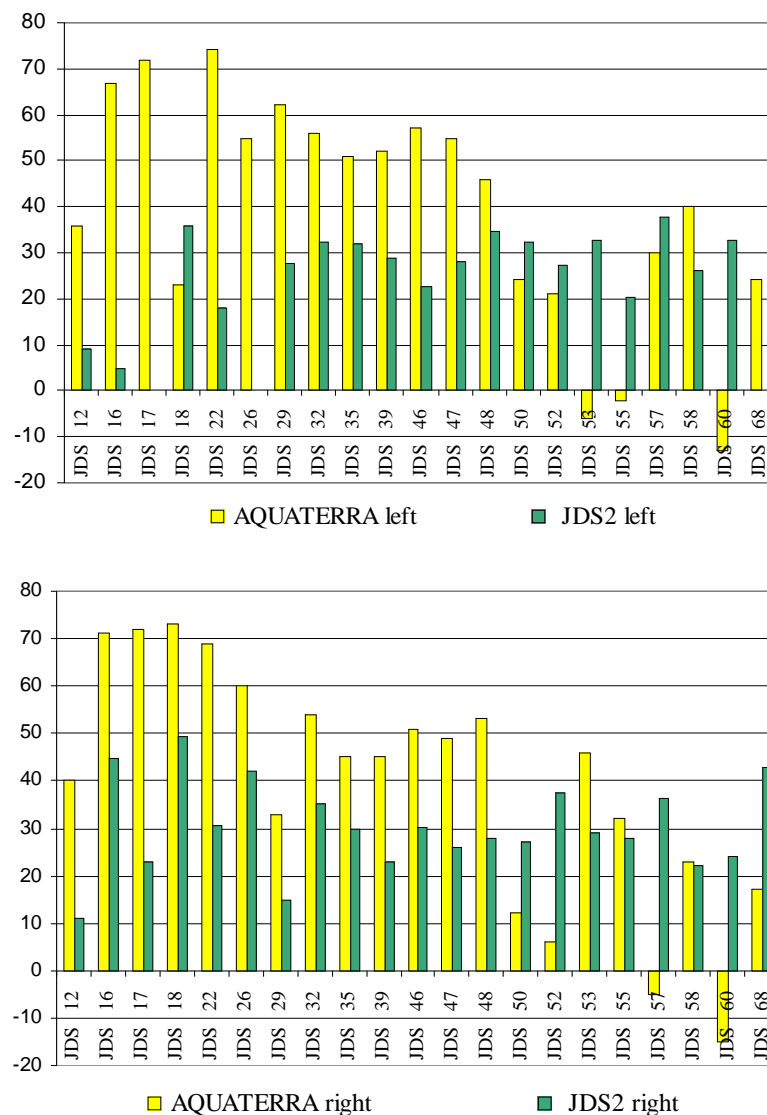
Figure 37: Toxic effect of pore water to Vibrio fischeri in longitudinal profiles of the Danube
