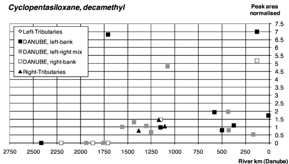
Figure 93: Occurrence profile of decamethylcyclopentasiloxane (D5) in the JDS2 sediment samples
