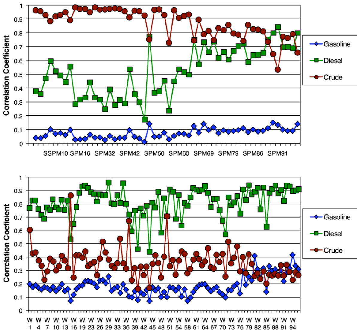
Figure 66: Characterisation of hydrocarbon contamination by correlating fluorescence spectra of water (W) and SPM sample extracts with the arbitrary standards
