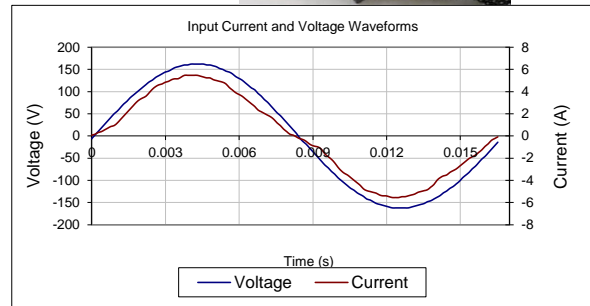
Input AC Current Waveform (ITHD = 9.21%, 50% Load)
