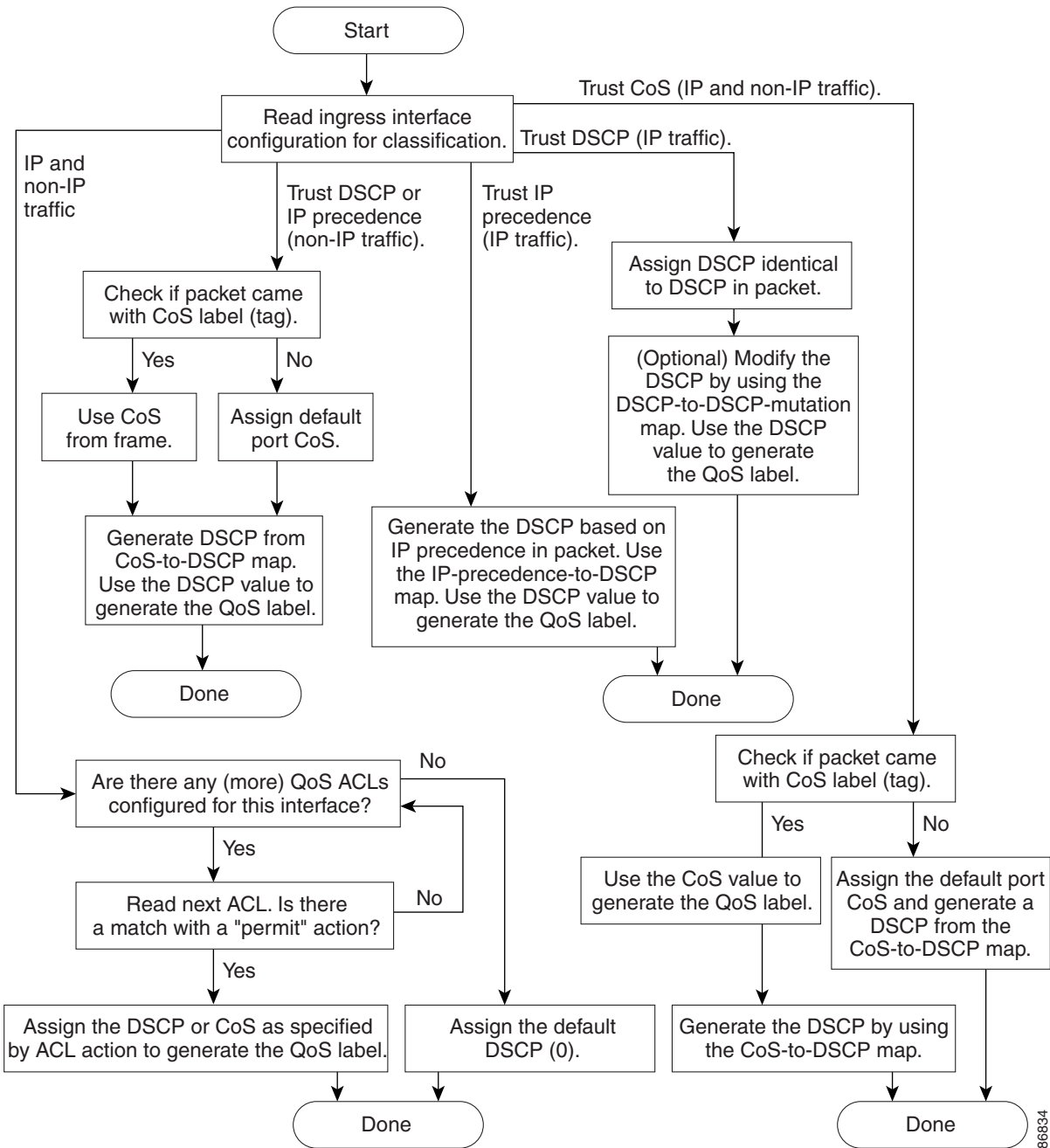
Figure 36-3 Classification Flowchart
