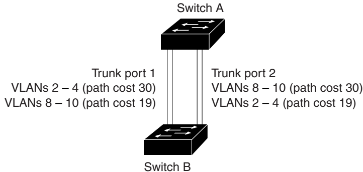
Figure 13-5 Load-Sharing Trunks with Traffic Distributed by Path Cost
