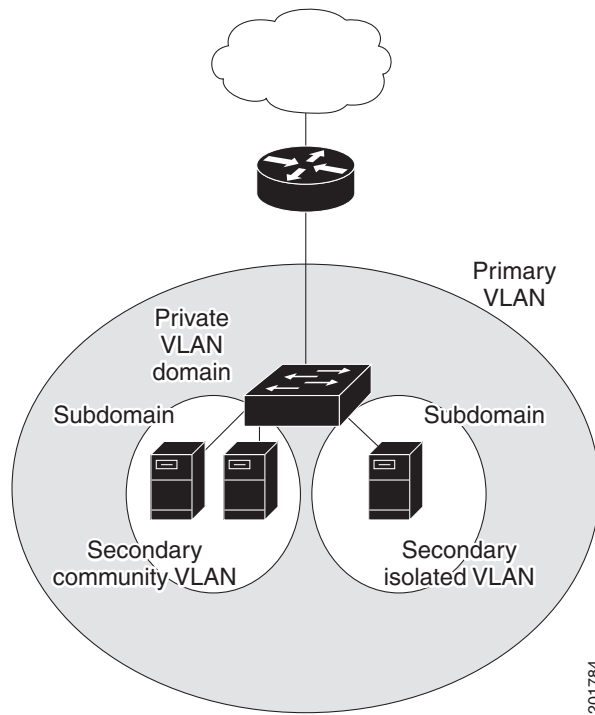
Figure 16-1 Private-VLAN Domain
