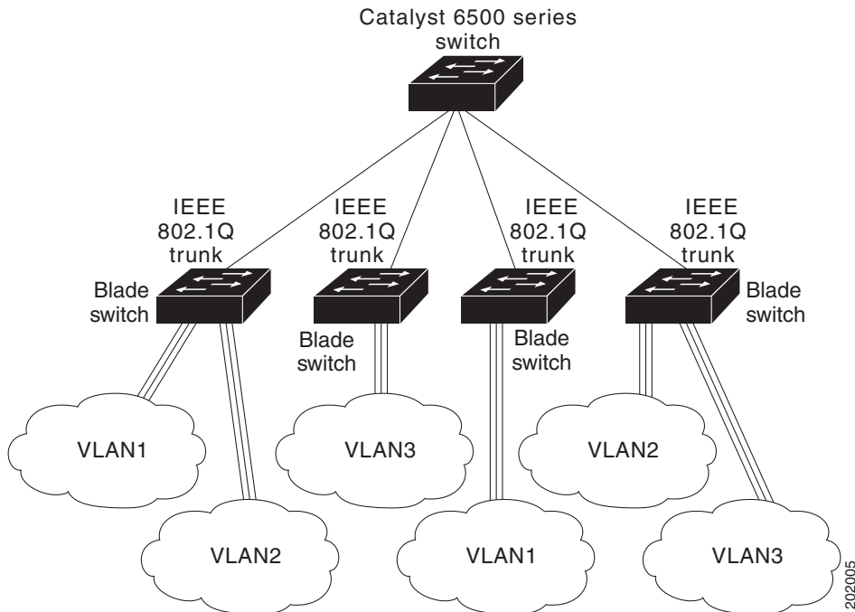
Figure 13-3 Switches in an IEEE 802.1Q Trunking Environment
