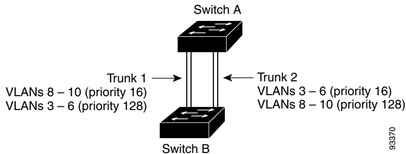
Figure 13-4 Load Sharing by Using STP Port Priorities
