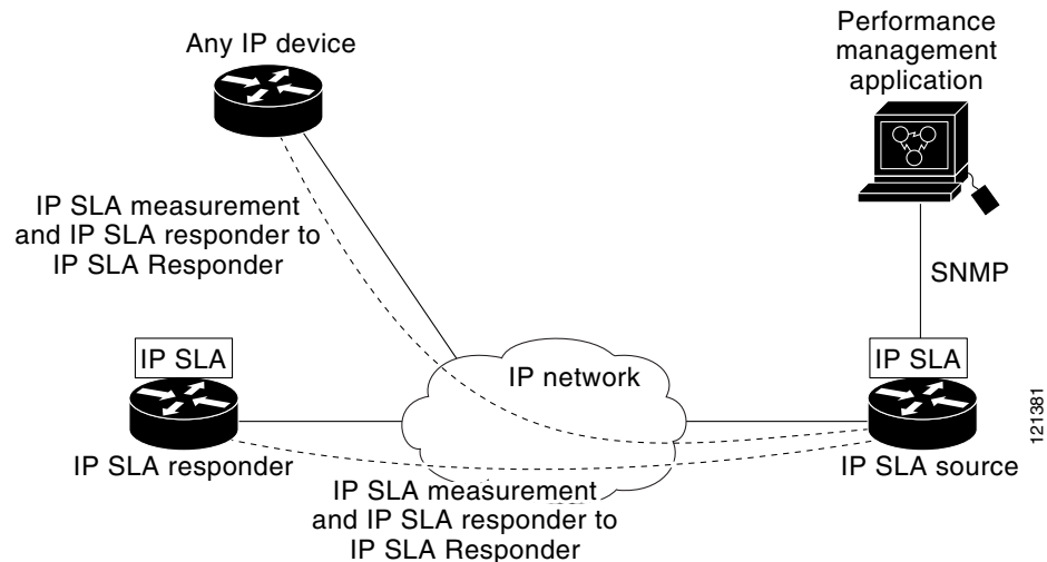
Figure 41-1 Cisco IOS IP SLAs Operation
