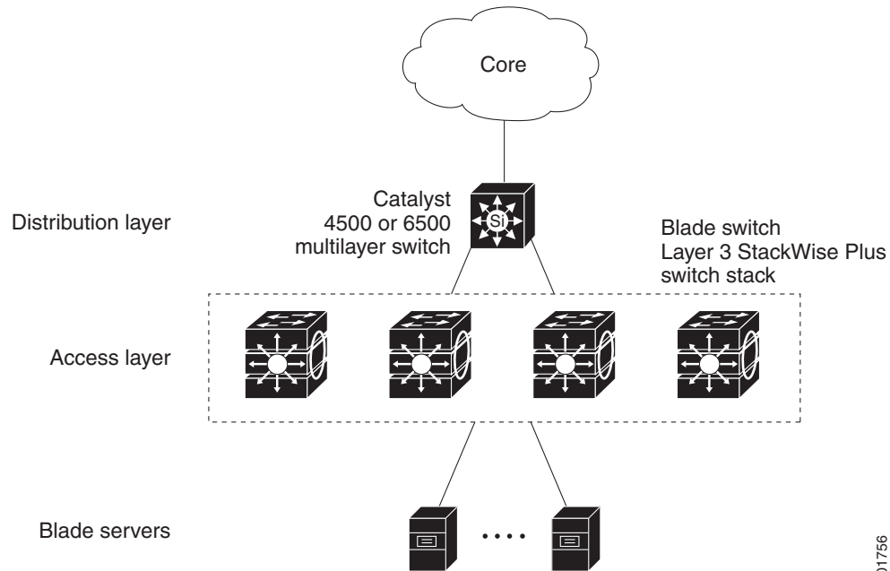
Figure 1-1 Data Center
