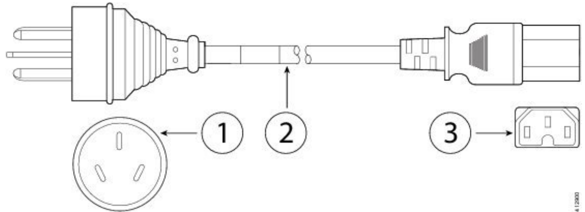
Figure 2: CAB-9K10A-AU (Australia)
