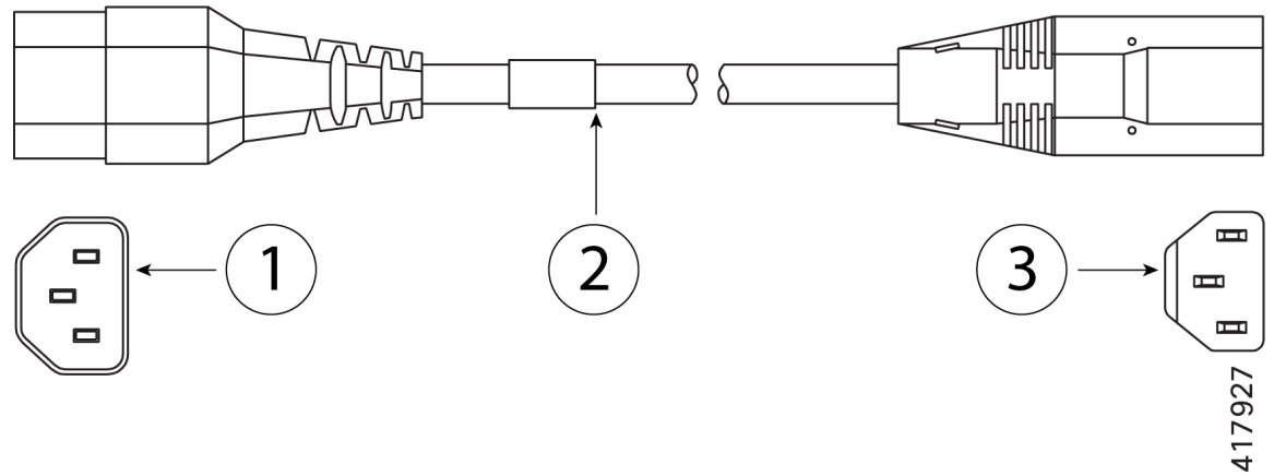
Figure 16: CAB-C13-CBN (2.2-foot C13-C14 Cabinet Jumper Power Cord)
