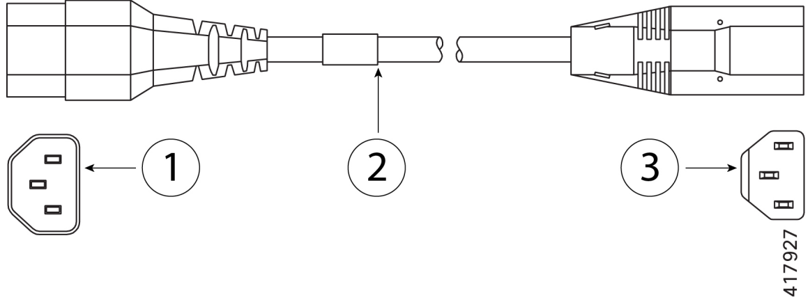
Figure 17: CAB-C13-C14-2M (6.6-foot C13-C14 Cabinet Jumper Power Cord)
