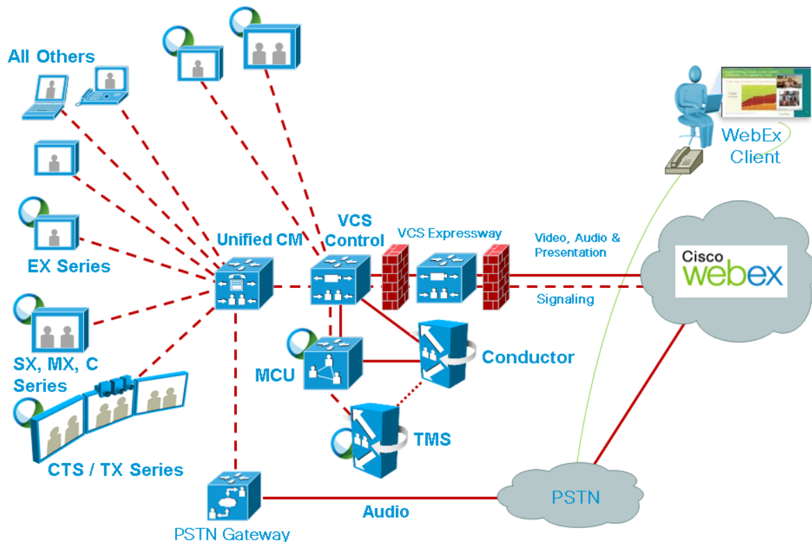
Figure 6: Network Topology - SIP Video and Presentation with PSTN Audio Using Unified CM
