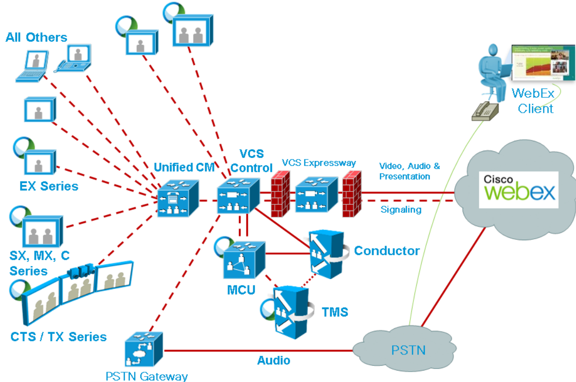
Figure 7: Network Topology - SIP Video and Presentation with PSTN Audio Using Cisco VCS Control
