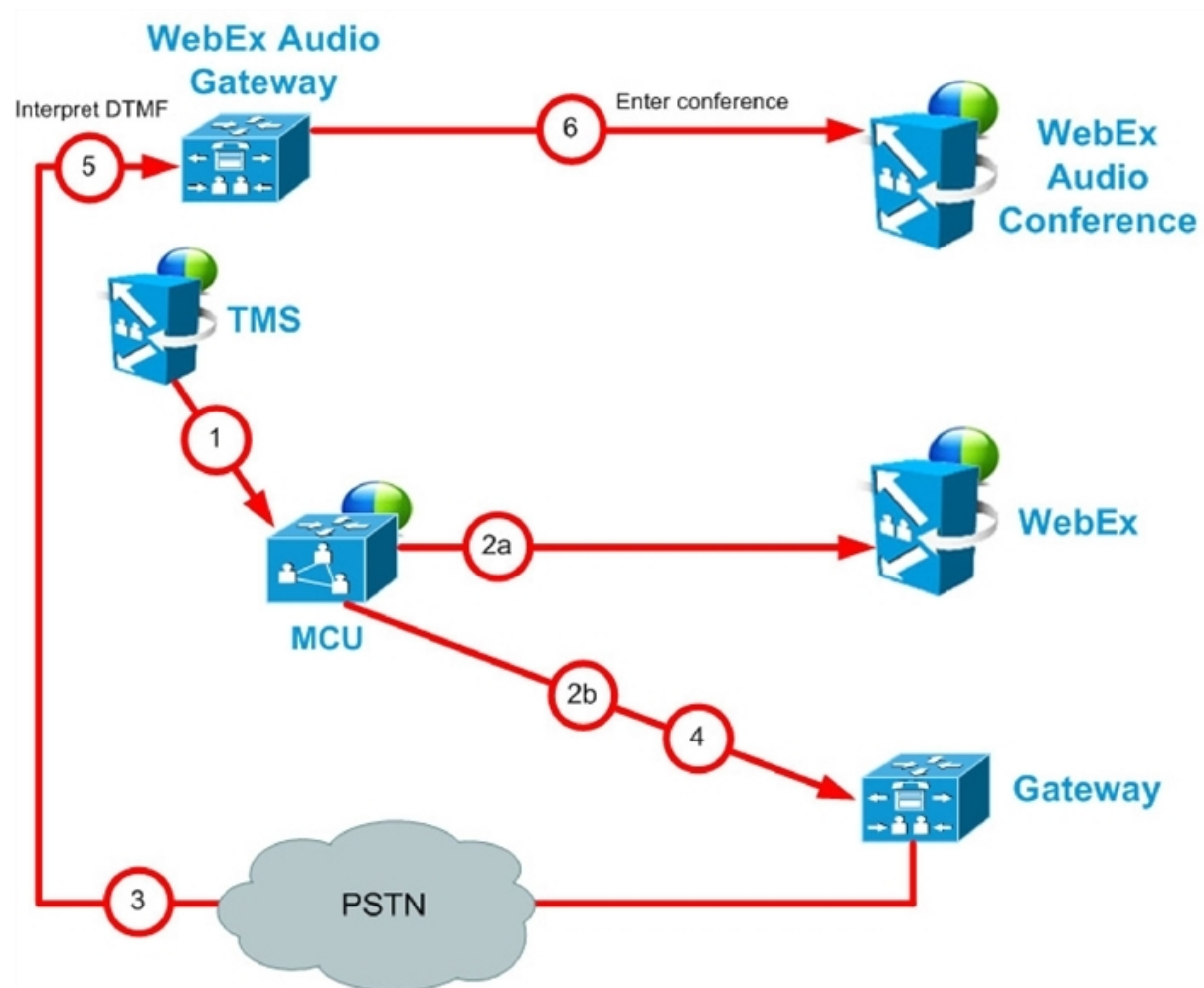
Figure 14: WebEx Audio (PSTN) Call Flow
