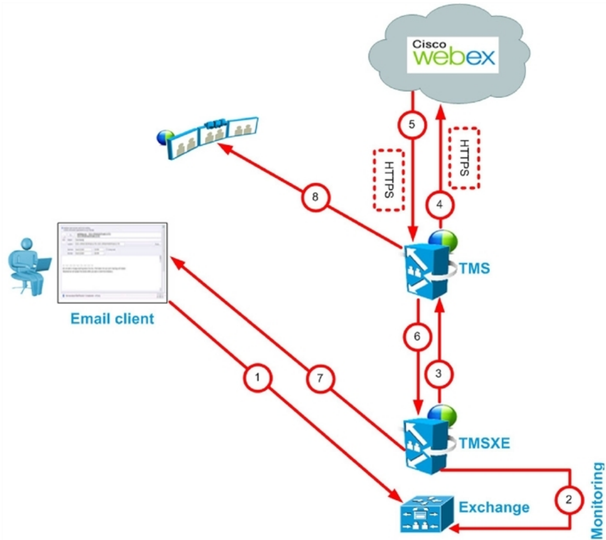
Figure 10: Cisco WebEx Scheduling Mailbox Scheduling Flow
