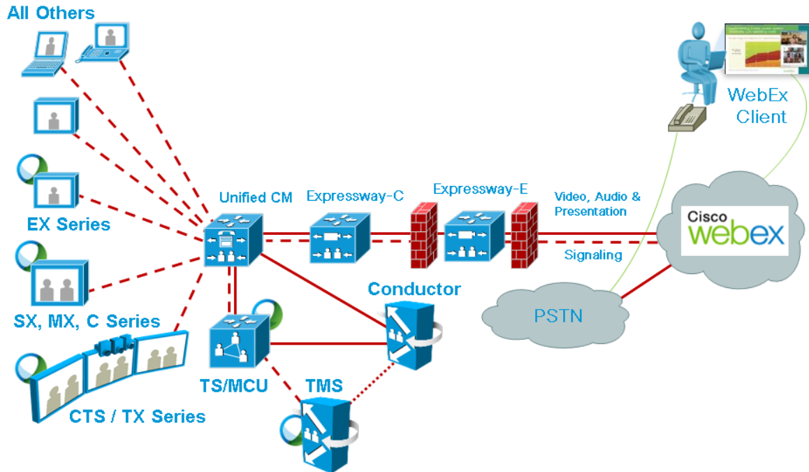
Figure 2: Network Topology - SIP Video, Audio and Presentation
