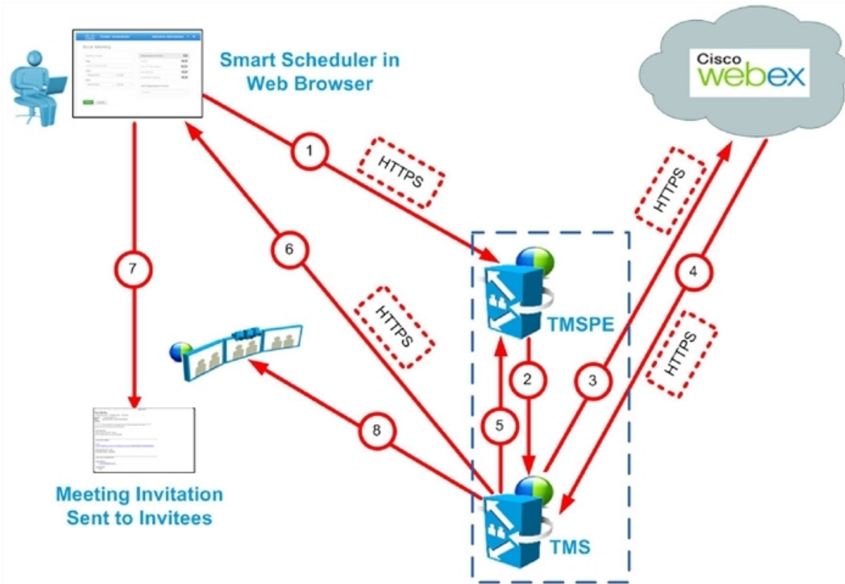
Figure 9: Cisco WebEx Smart Scheduler Scheduling Flow
