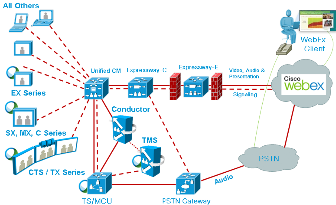
Figure 4: Network Topology - SIP Video and Presentation with PSTN Audio Using Cisco Expressway-C
