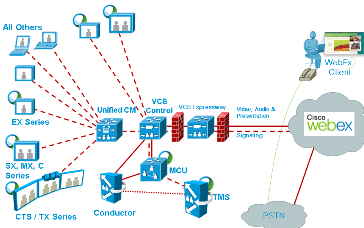
Figure 5: Network Topology - SIP Video, Audio and Presentation
