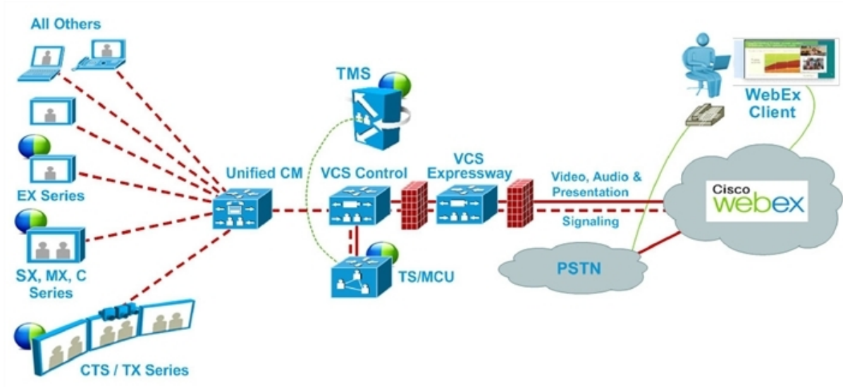
Figure 25: SIP Audio Deployment with Endpoints Registered to Unified CM
