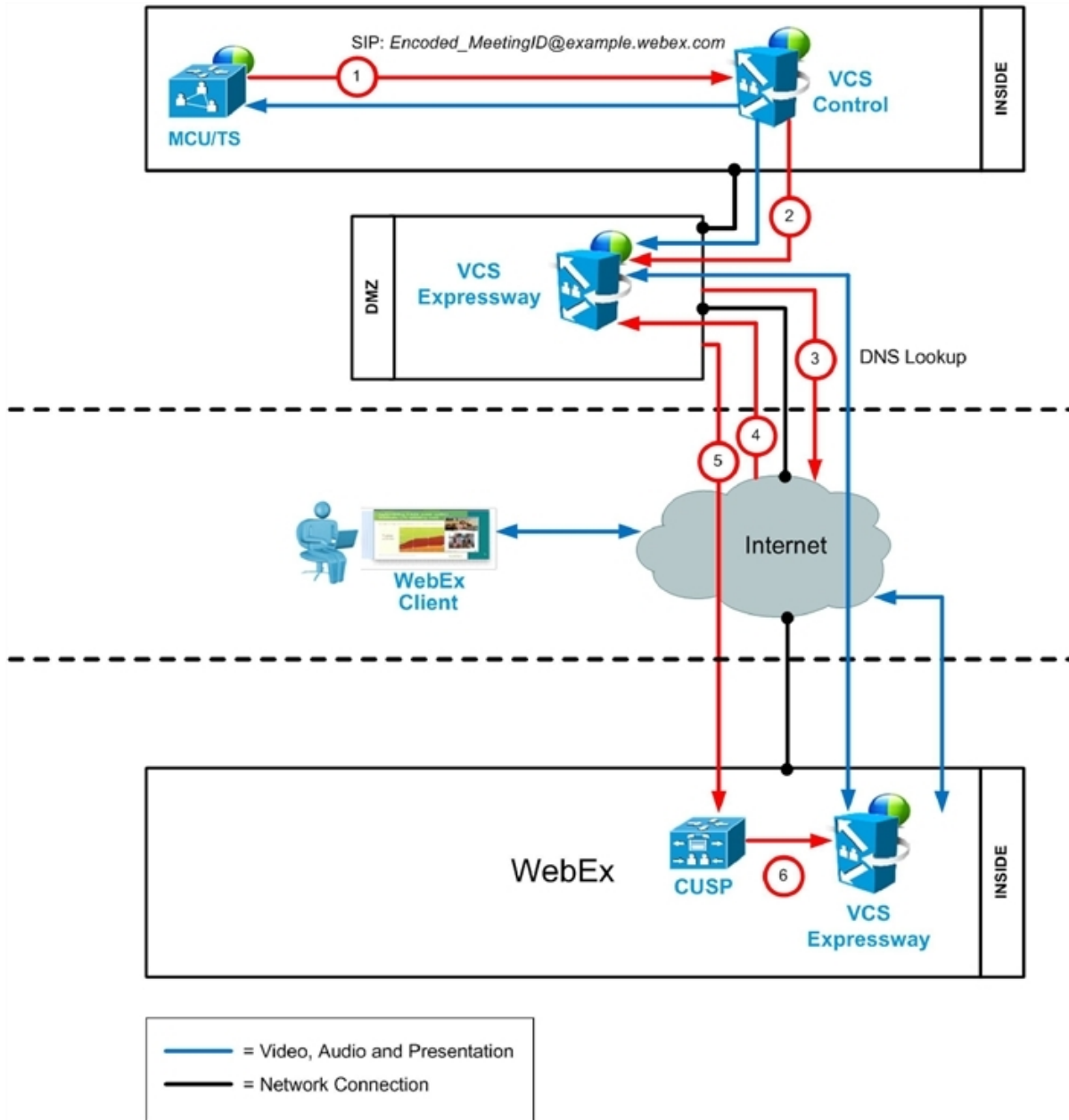
Figure 11: SIP Audio Call Flow
