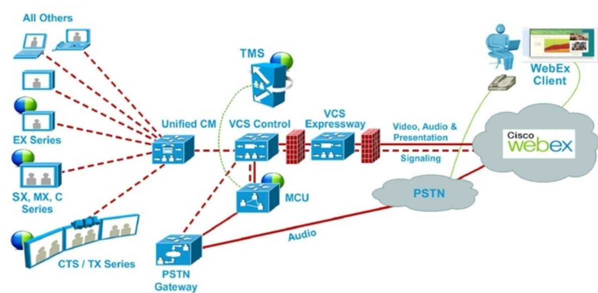
Figure 26: PSTN Audio Deployment with Gateway Registered to VCS and Endpoints Registered to Unified CM
