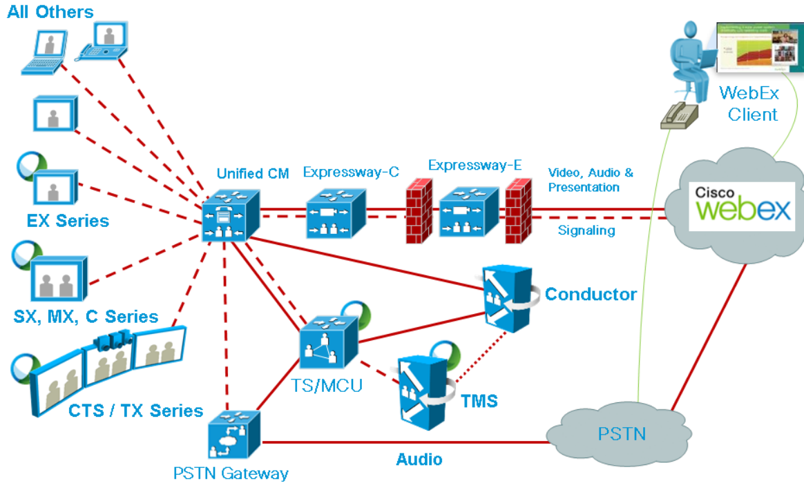
Figure 3: Network Topology - SIP Video and Presentation with PSTN Audio Using Unified CM
