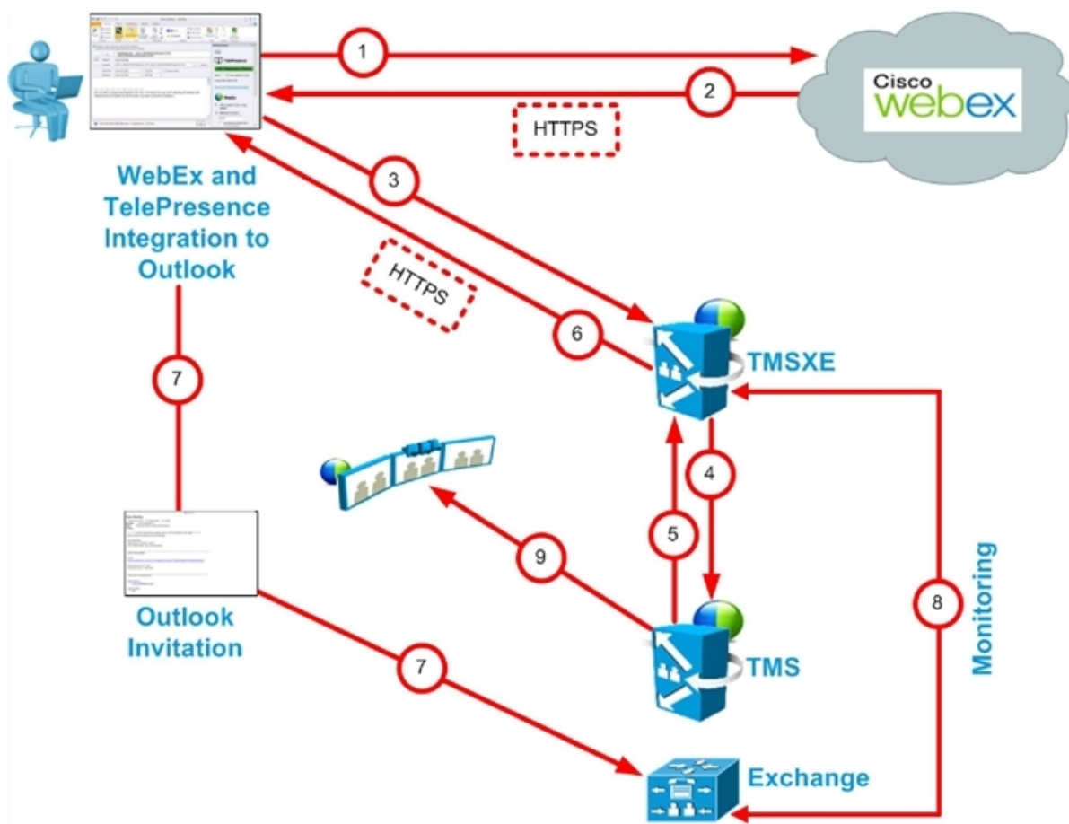
Figure 8: Cisco WebEx and TelePresence Integration to Outlook Scheduling Flow
