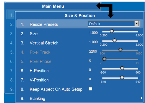
Figure B-7 View Previous Menu
