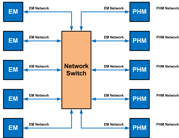
Figure 3-20 Projectors in an EM Network
