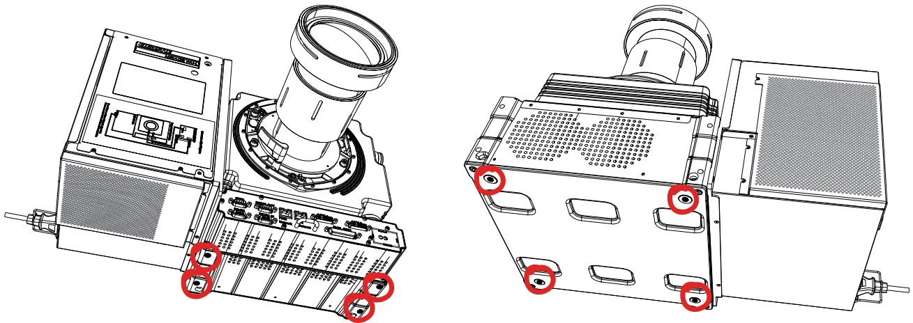
Figure 2-1 Mounting Holes
