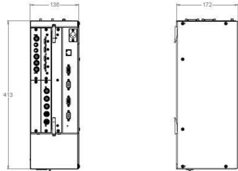
Figure 7-3 Electronic Module Dimensions
