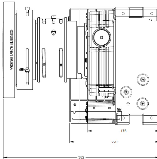
Figure 7-5 Mirage WU-L Side Dimensions with 0.75:1 Lens
