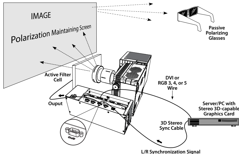
Figure 3-25 Mirage WU-L: Typical Stereo 3D Configuration: With Passive Glasses
