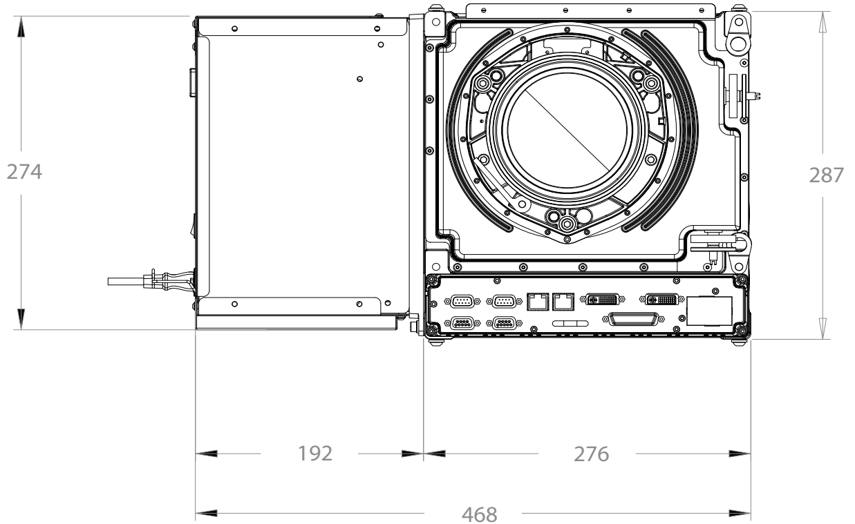
Figure 7-1 Mirage WU-L Front Dimensions
