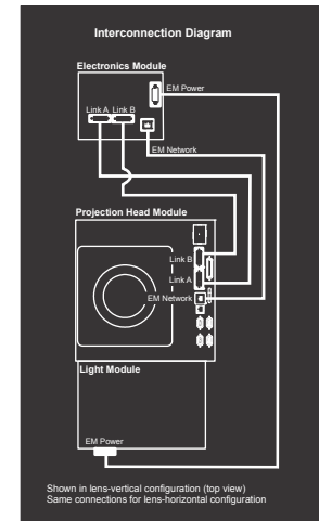
Figure 2-2 Module Interconnections
