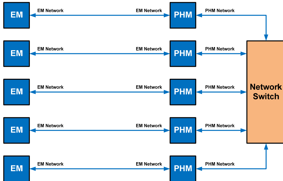
Figure 3-21 Projectors in a PHM Network
