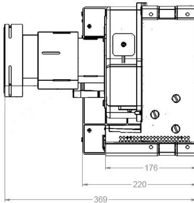
Figure 7-2 Mirage WU-L Side Dimensions with 1.2 - 1.6:1 Lens
