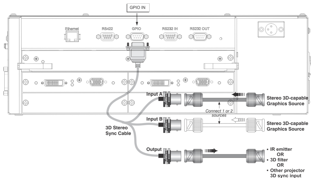
Figure 3-23 Mirage GPIO 3D Stereo Sync Cable
