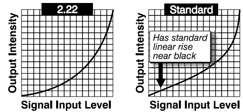
Figure 3-12 Gamma Curve
