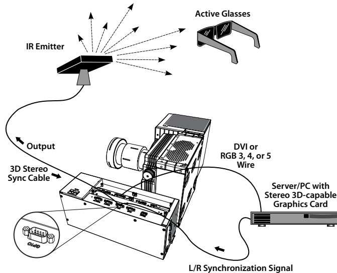
Figure 3-24 Mirage WU-L: Typical Stereo 3D Configuration: With Active Glasses
