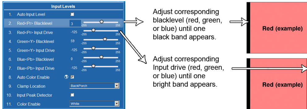
Figure 3-11 Adjusting Input Levels Using the Peak Detector
