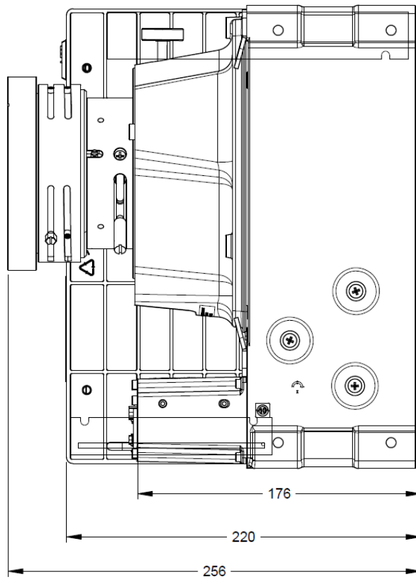
Figure 7-4 Mirage WU-L Side Dimensions with 0.64 Lens
