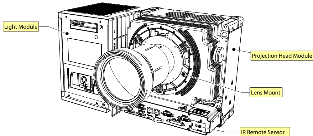
Figure 1-2 Mirage WU-L Projector
