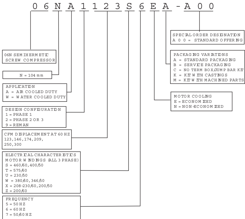
06N SCREW COMPRESSOR SIGNIFICANCE CHART
