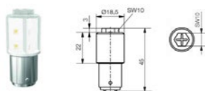
MRBD1508xx 8 chip-led
