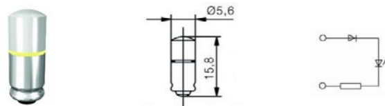
MWCG57xx Multi-Look®
