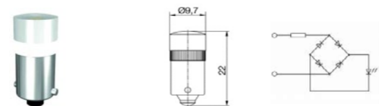
MWCB22xx9 Multi-Look®
