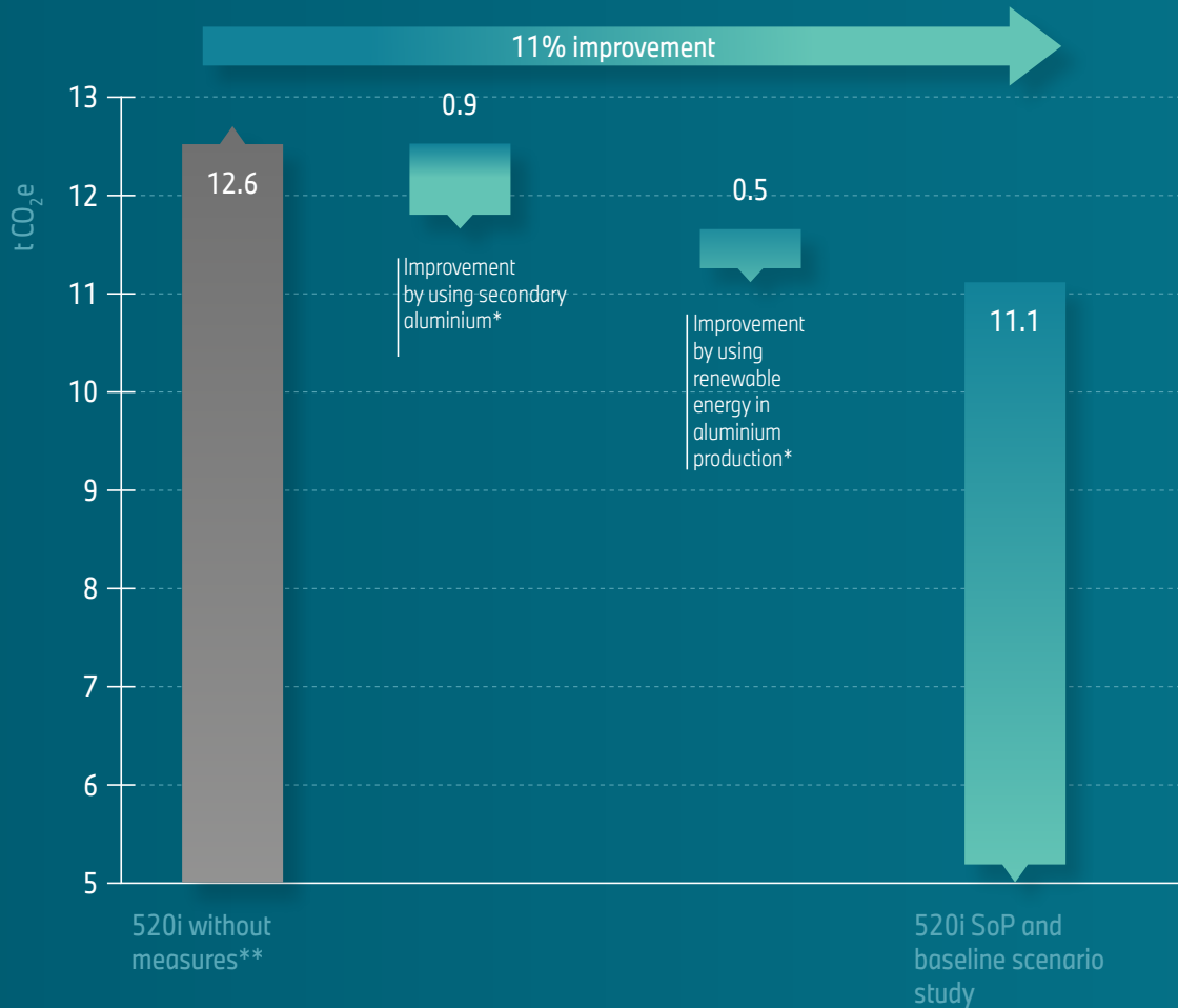
Fig. 5: Influence of development targets on the global warming potential in the manufacturing phase of the BMW 520i
