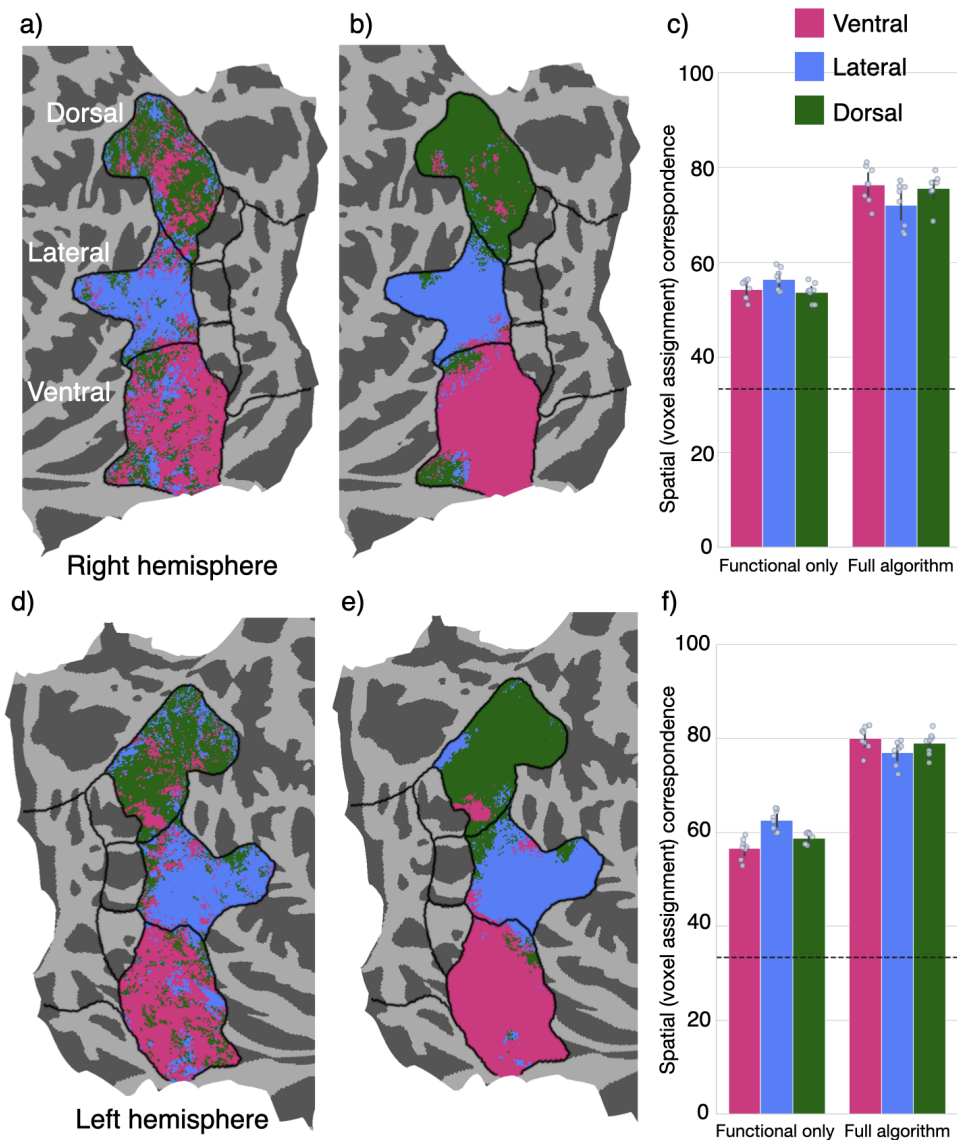
Figure S3. Validating the 1-to-1 mapping algorithm by testing how well it maps one brain onto another brain. (a) Right hemisphere voxels in Target (Subj. 2) brain colored by their assignment to streams in Source (Subj. 1) right hemisphere voxels using the algorithm [30] that matches each unit to a voxel solely based on functional similarity. Essentially, all spatial information was removed and voxels in the Target brain were assigned to voxels from the Source brain purely on the basis of how correlated they were in their responses to the shared stimuli across subjects. We refer to this mapping as functional only. (b) Right hemisphere voxels in Target (Subj. 2) brain colored by their assignment to Source (Subj. 1) right hemisphere voxels using the full algorithm that additionally incorporates a gentle smoothness constraint, which encourages neighboring voxels in the target space to "pick" neighboring voxels in the source space (algorithm used in main text). (c) Spatial correspondence between brains using the functional only or full algorithm. Bars: Comparison of right hemisphere voxel-to-voxel correspondence. Data show substantially higher correspondences when using the full algorithm in both the right (Ventral: t(7) = 41.3, p = 1.3 \times 10^{-9} , Lateral: t(7) = 15.6, p = 1.1 \times 10^{-6} , Dorsal: t(7) = 27.0, p = 2.5 \times 10^{-8} ) and left hemisphere (panel f; Ventral: t(7) = 18.2, p = 3.7 \times 10^{-7} , Lateral: t(7) = 18.1, p = 4.0 \times 10^{-7} , Dorsal: t(7) = 21.8, p = 1.1 \times 10^{-7} ). Data plotted for high-level ROIs across three streams, averaged across source subjects for each target subject. Color represents stream (pink: Ventral, blue: Lateral, and green: Dorsal). Dotted line: chance level (33%). Error bar: 95% CI, each dot is a subject. Data show that the full algorithm achieves a better brain-to-brain mapping. (d), (e), and (f), same for left hemisphere.
