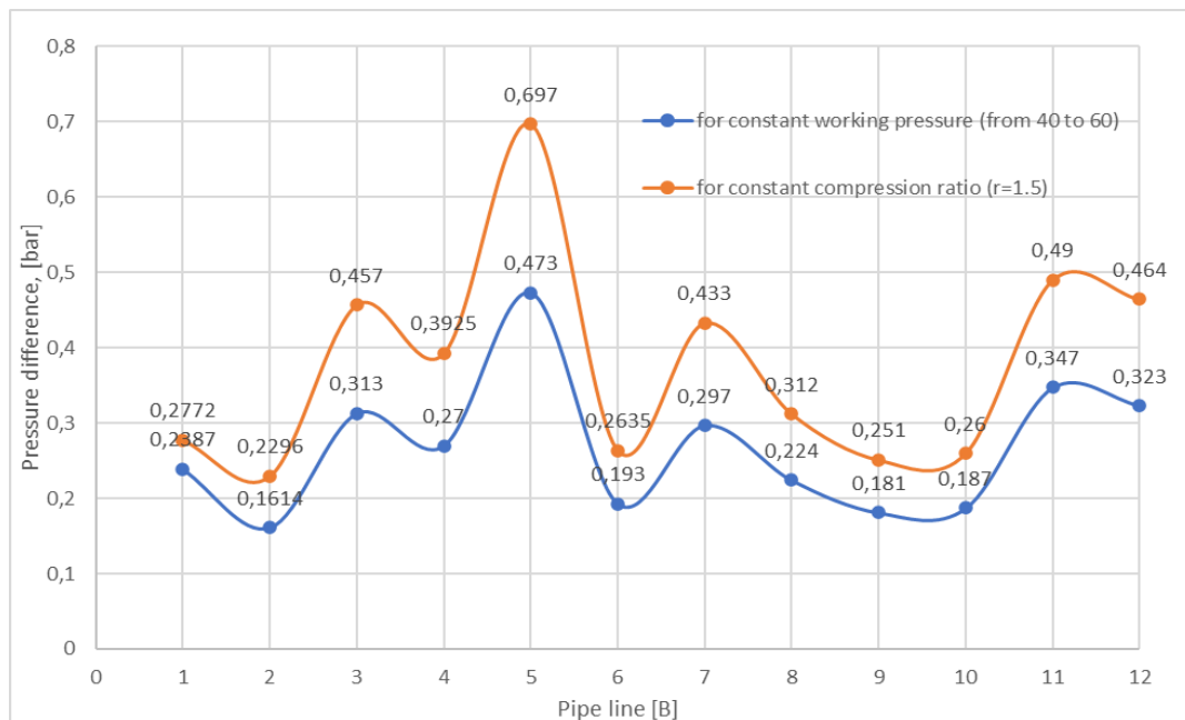
Figure 34. Pressure Loss Changes for Compressor Station
