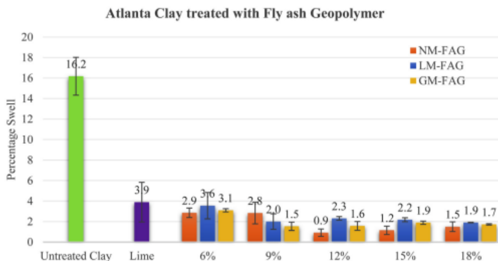
Figure 4. Metakaolin geopolymer reinforced Atlanta clay (Khadka et.al, 2020)
