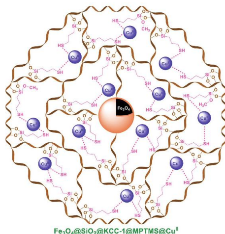
Figure 7. Fe_3O_4@SiO_2@KCC-1@MPTMS@Cu^{II} magnetic nanocatalyst
