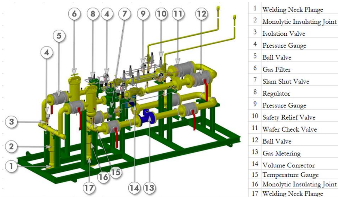
Figure 18. Pressure Reducing and Measuring Station Collector ( (Penawaran, 2023)
