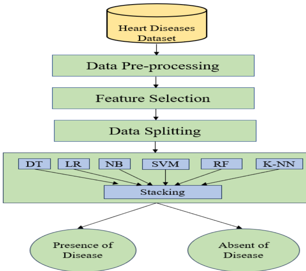
Figure 35: The flow diagram of the suggested model for heart disease prediction
