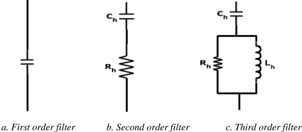
Figure 6. Passive filters
