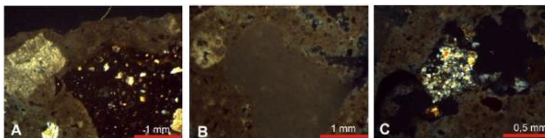
Figure 17. General view of the thin section of sample 1 under a polarizing microscope. A. Brick fragment and limestone fragment (double nicol) found in sample 1. B. Lime lump (double nicol) found in sample 1. C. Sandstone fragment (double nicol) found in sample 1
