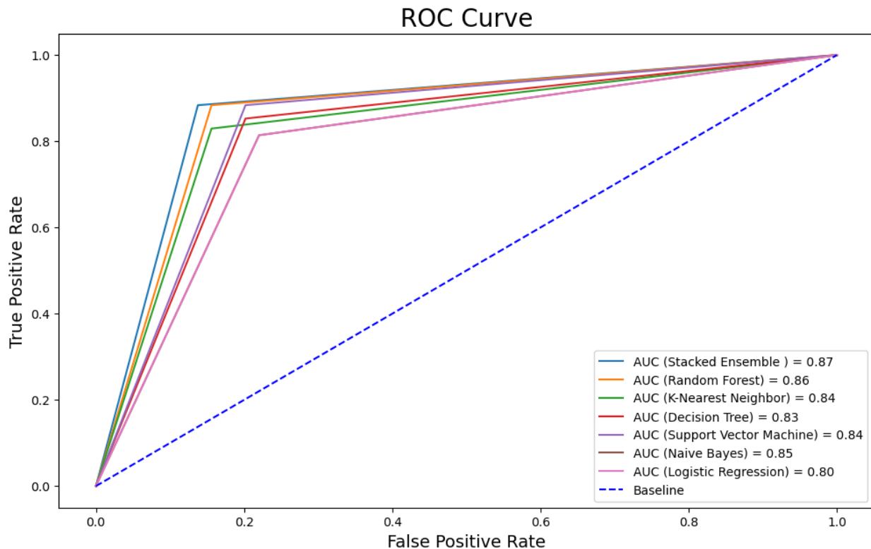
Figure 39: The AUC-ROC Curve of each ML algorithm
