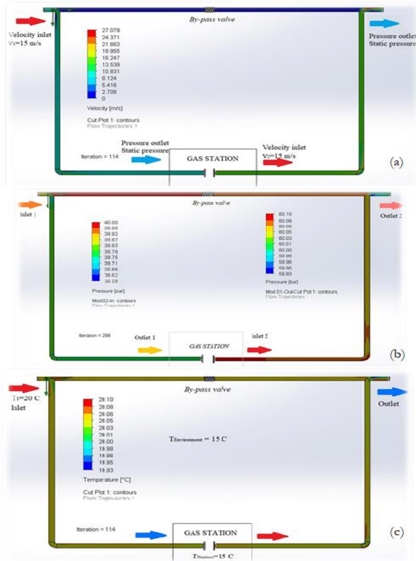
Figure 26. Contours of a) speed b) pressure and) temperature for standart collector
