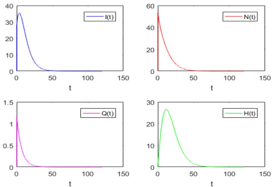
Figure 4. Dynamics of the Effect of Quarantine on the Spread of COVID-19 for d(\alpha) = \Gamma(1 + 2\alpha/7) .
