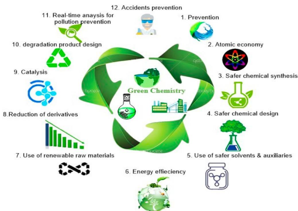
Scheme 1. Green Chemistry
