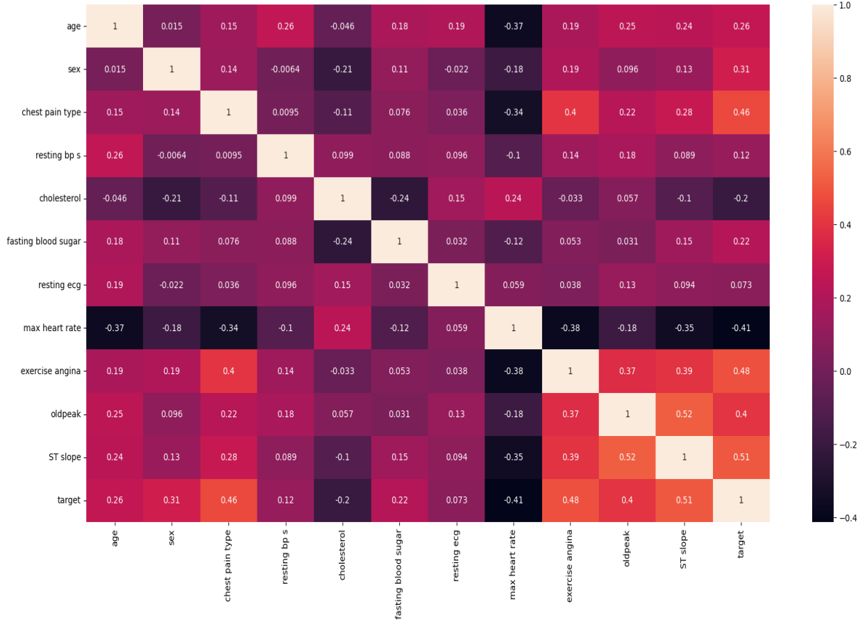
Figure 37: Correlation heatmap
