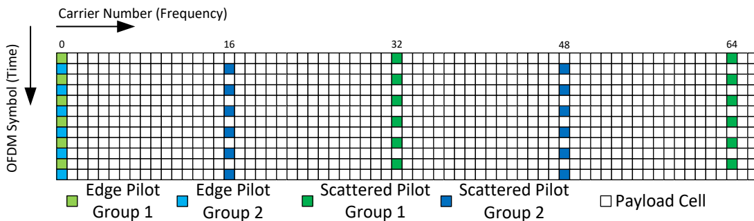
Figure L.9.11 MIMO pilot scheme MP16_2 for Walsh-Hadamard pilot encoding.
