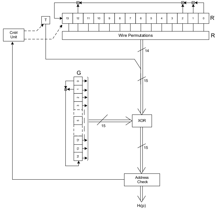
Figure 7.29 FI address generation scheme for the 32K FFT size.
