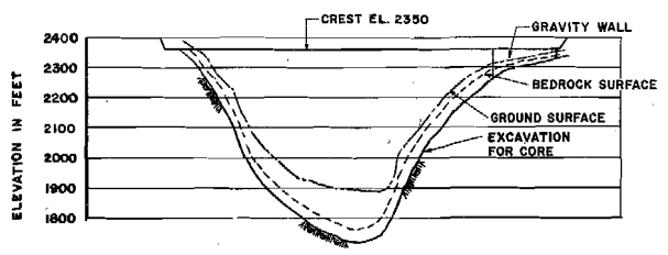
LONGITUDINAL SECTION THRU C OF MAIN DAM SCALE B
