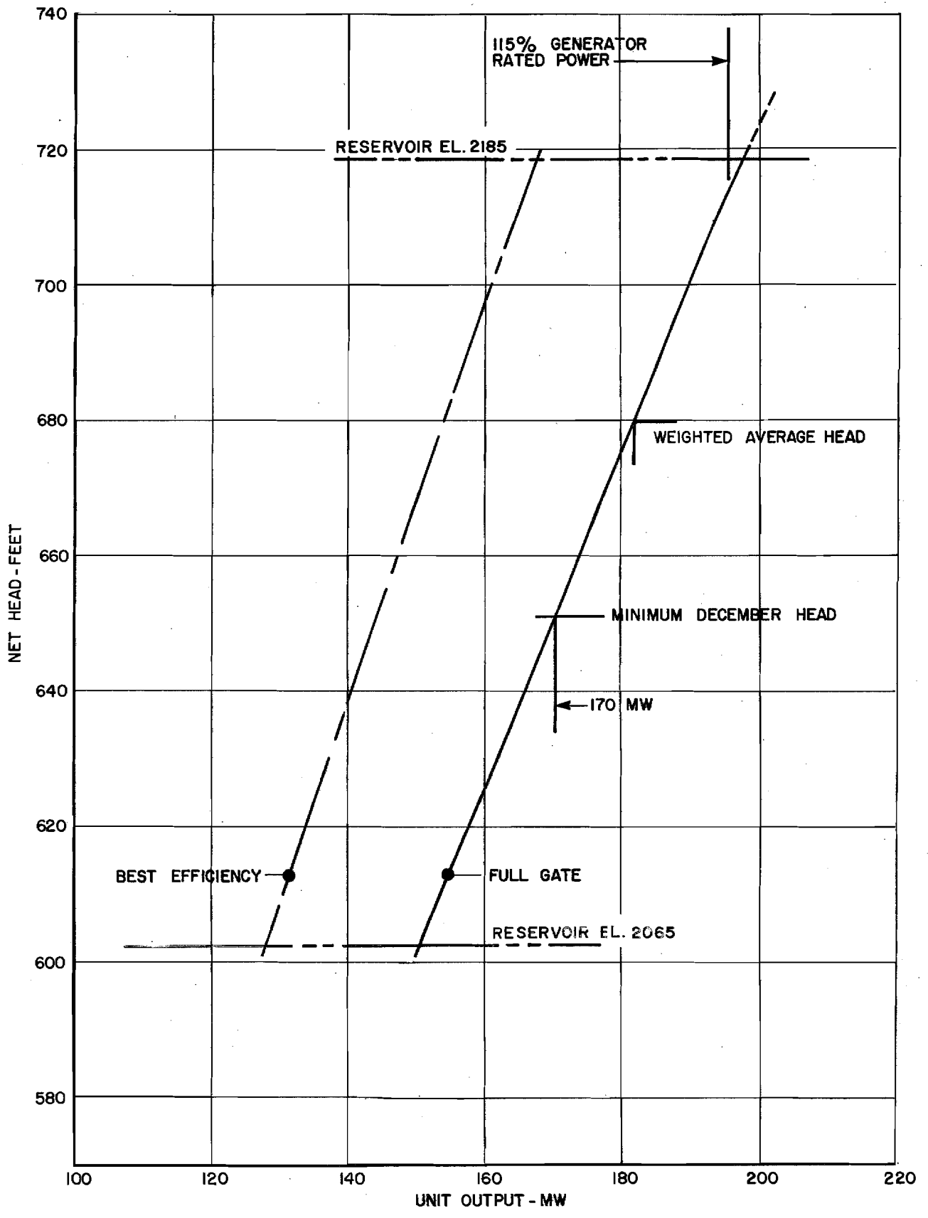
WATANA - UNIT OUTPUT
