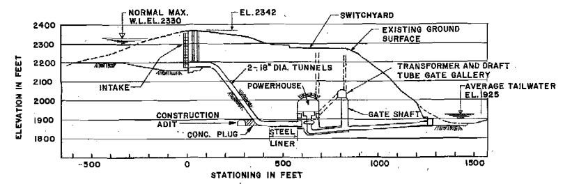
POWER FACILITIES PROFILE SCALE B
