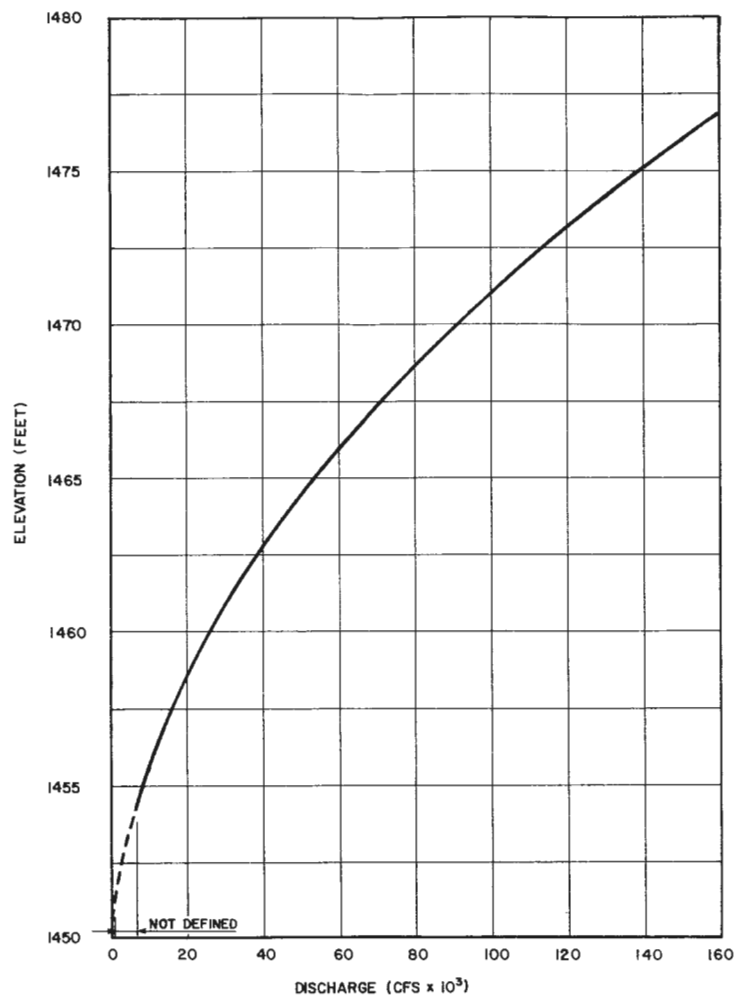
TAILWATER RATING
