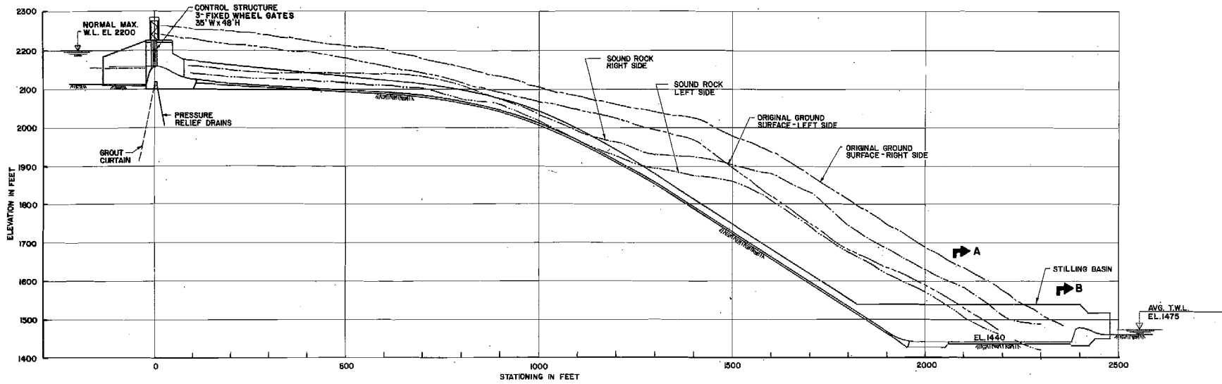
SPILLWAY PROFILE
