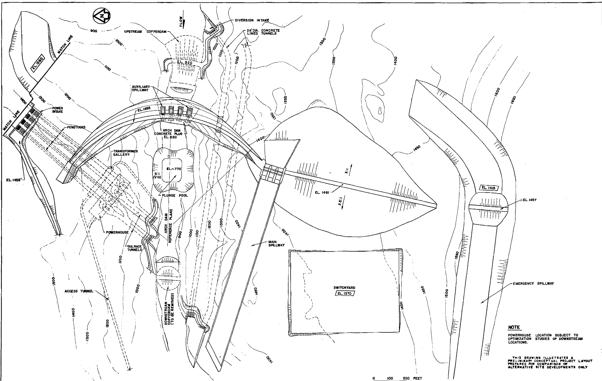
GENERAL ARRANGEMENT
