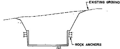
SECTION A-A SCALE C
