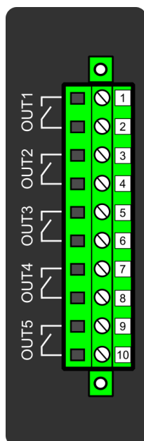
Figure. 8.6 - 247. Digital output module (DO5) with five add-on digital outputs.
