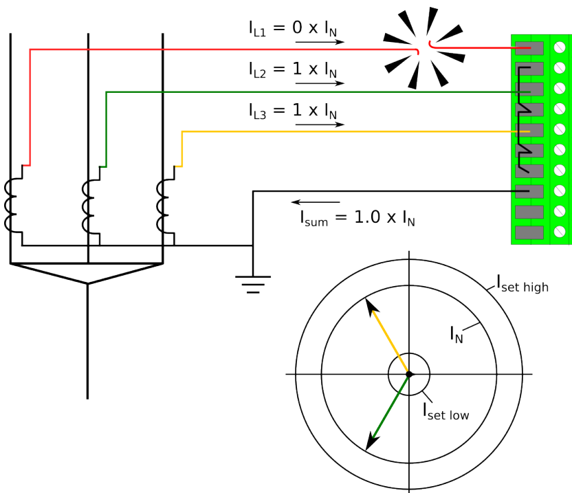
Figure. 5.5.1 - 212. Secondary circuit fault in phase L1 wiring.
