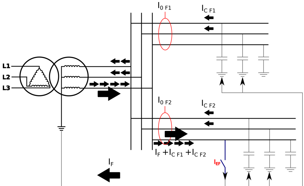
Figure. 5.3.5 - 95. Angle tracking of I_{0dir} function (directly earthed or small impedance network).
