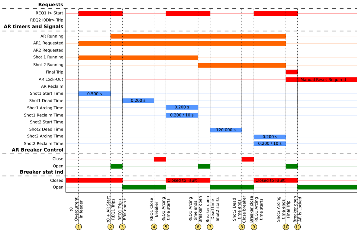
Figure. 5.4.4 - 185. Signal status graph of the permanent overcurrent auto-recloser cycle.
