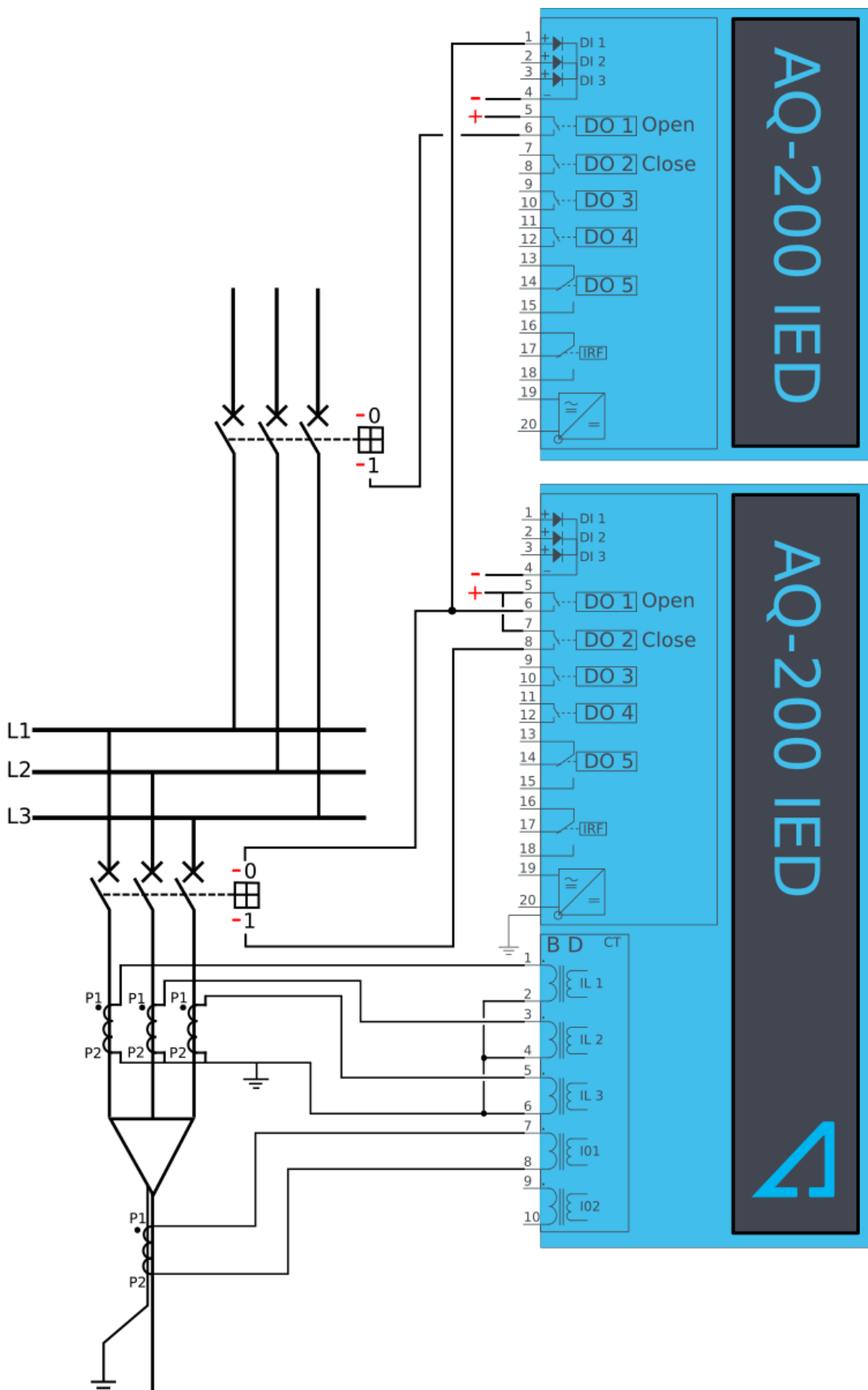
Figure. 5.3.8 - 110. Wiring diagram when the device is configured as a dedicated CBFP unit.
