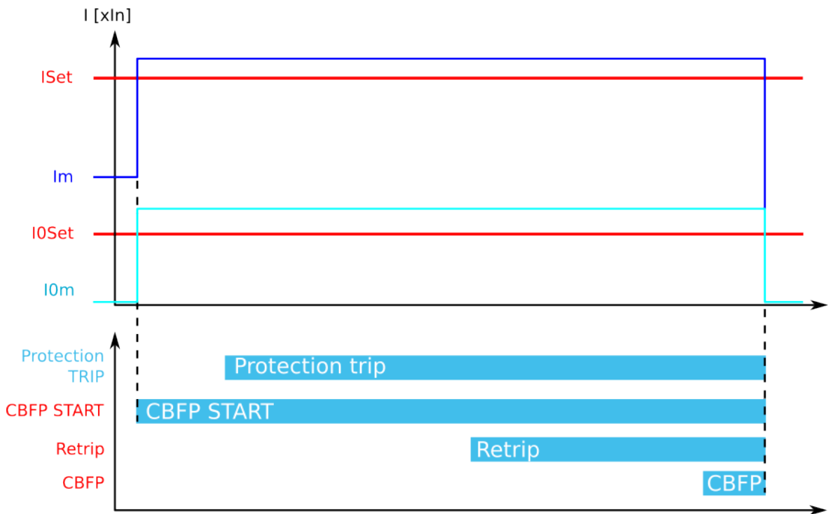
Figure. 5.3.8 - 103. Retrip and CBFP when "Current" is the selected criterion.
