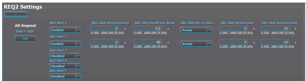
Figure. 5.4.4 - 180. Settings for I0dir> with two shots.
