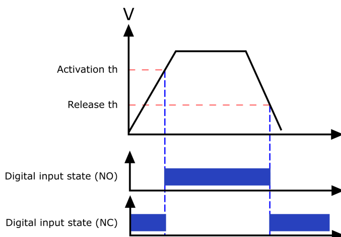
Figure. 8.5 - 246. Digital input state when energizing and de-energizing the digital input channels.
