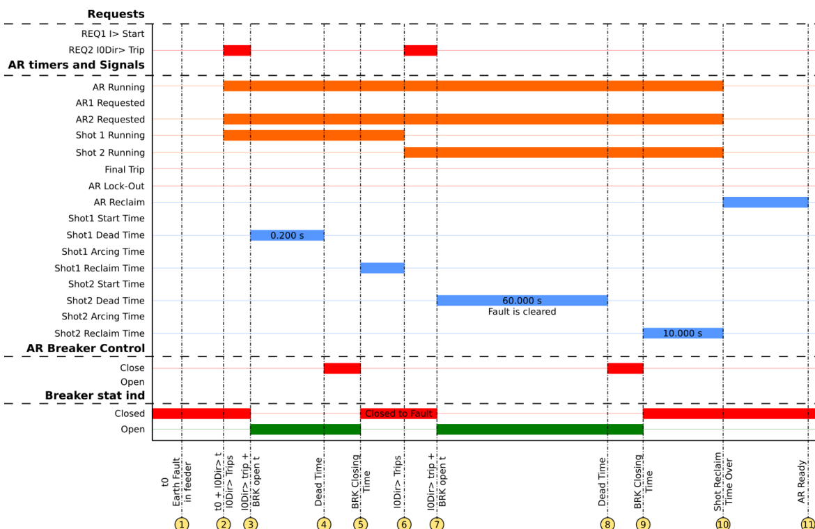
Figure. 5.4.4 - 181. Signal status graph of the semi-permanent earth fault auto-recloser cycle.
