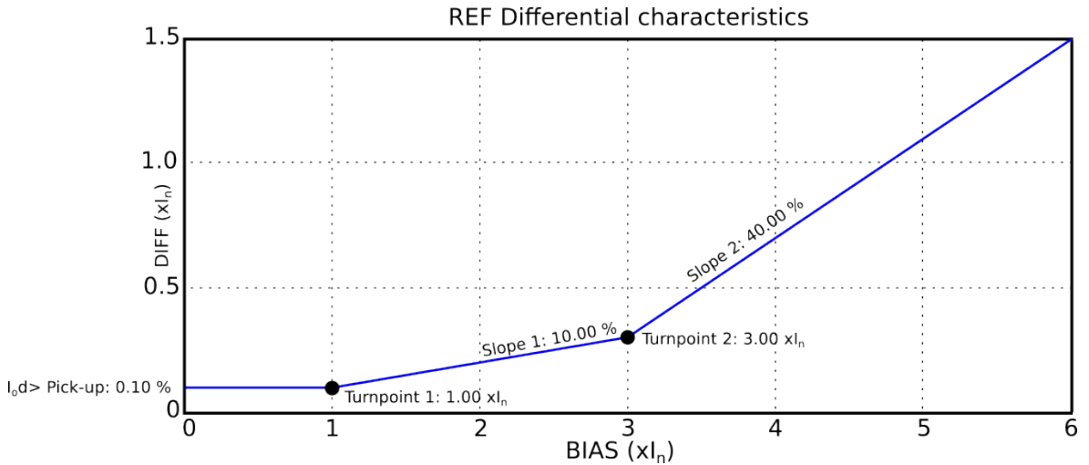
Figure. 5.3.9 - 113. Differential characteristics for the I0d> function with default settings.
