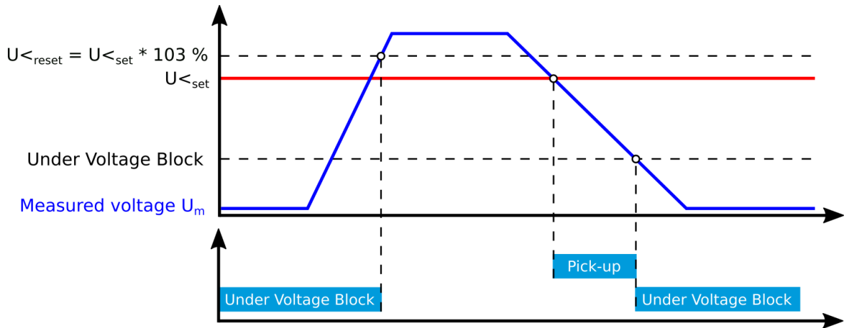
Figure. 5.3.11 - 123. Example of the block setting operation.
