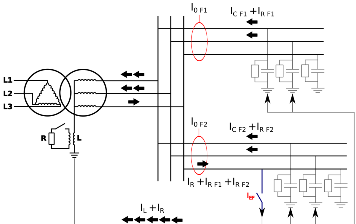
Figure. 5.3.5 - 94. Angle tracking of I_{0dir} function (Petersen coil earthed network model).
