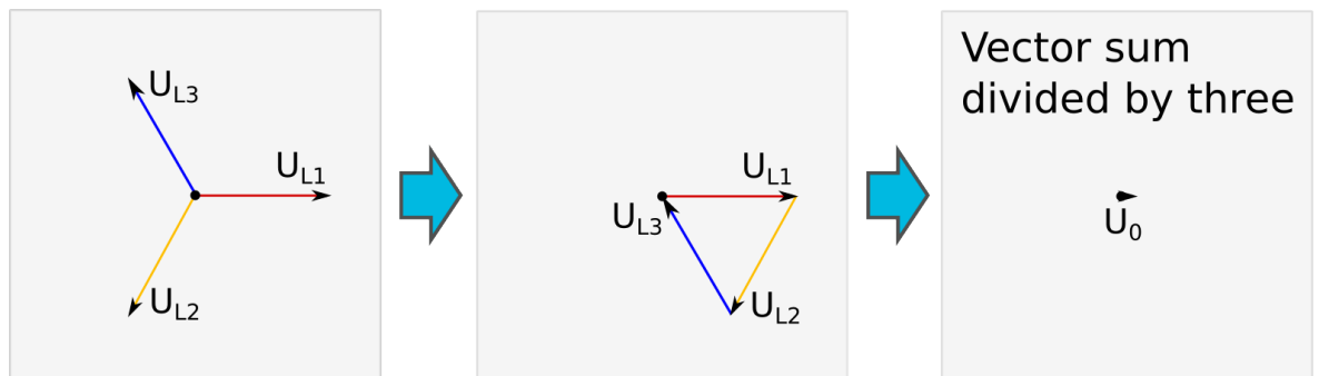
Figure. 5.3.12 - 125. Earth fault in isolated network.
