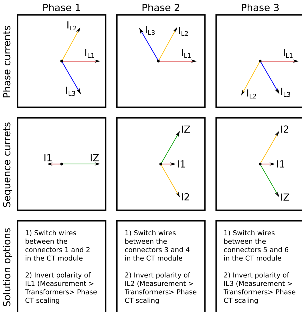
Figure. 5.2.1 - 63. Common phase polarity problems.
