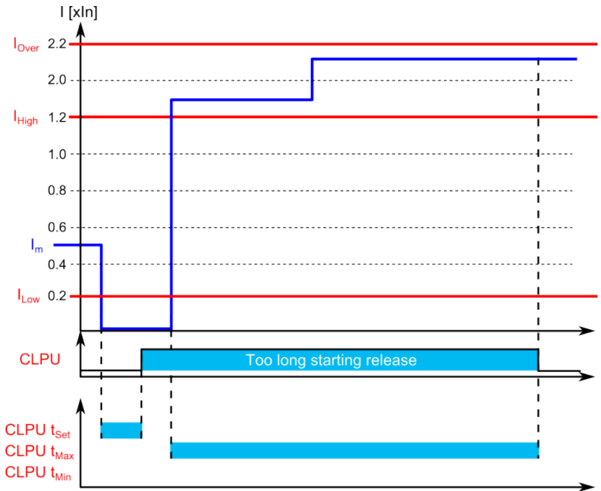
Figure. 5.4.5 - 197. Example of timers and pick-up parameters (activated pick-up and instant release due to too long starting).
