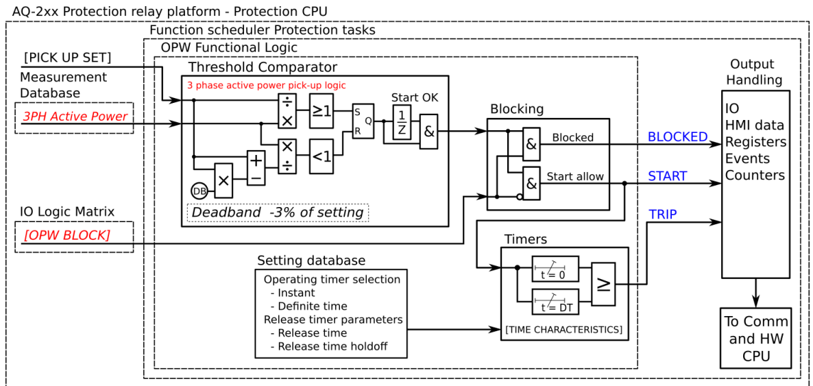
Figure. 5.3.16 - 141. Simplified function block diagram of the P> function.
