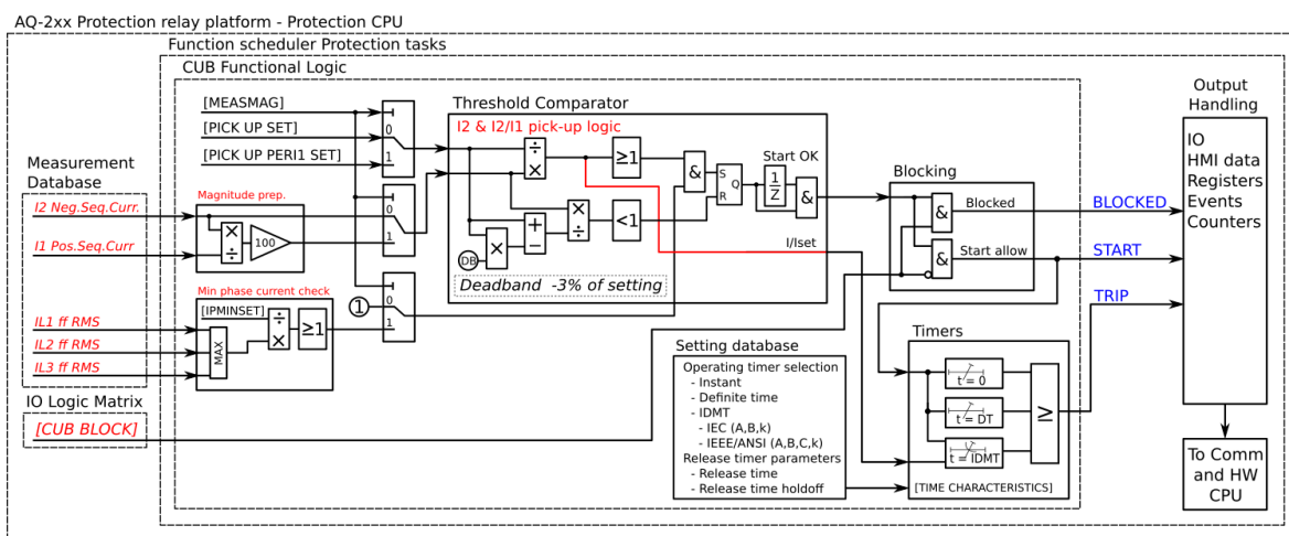
Figure. 5.3.6 - 98. Simplified function block diagram of the I2> function.
