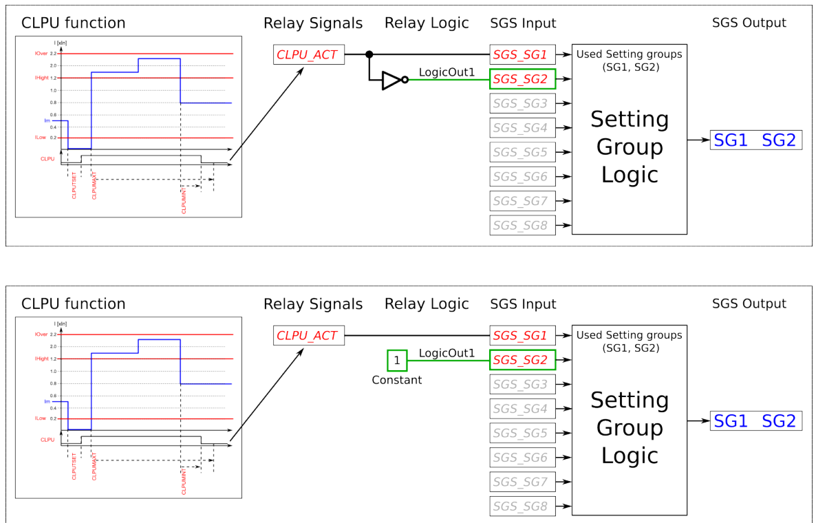
Figure. 5.4.1 - 172. Entirely application-controlled setting group change with the cold load pick-up function.
