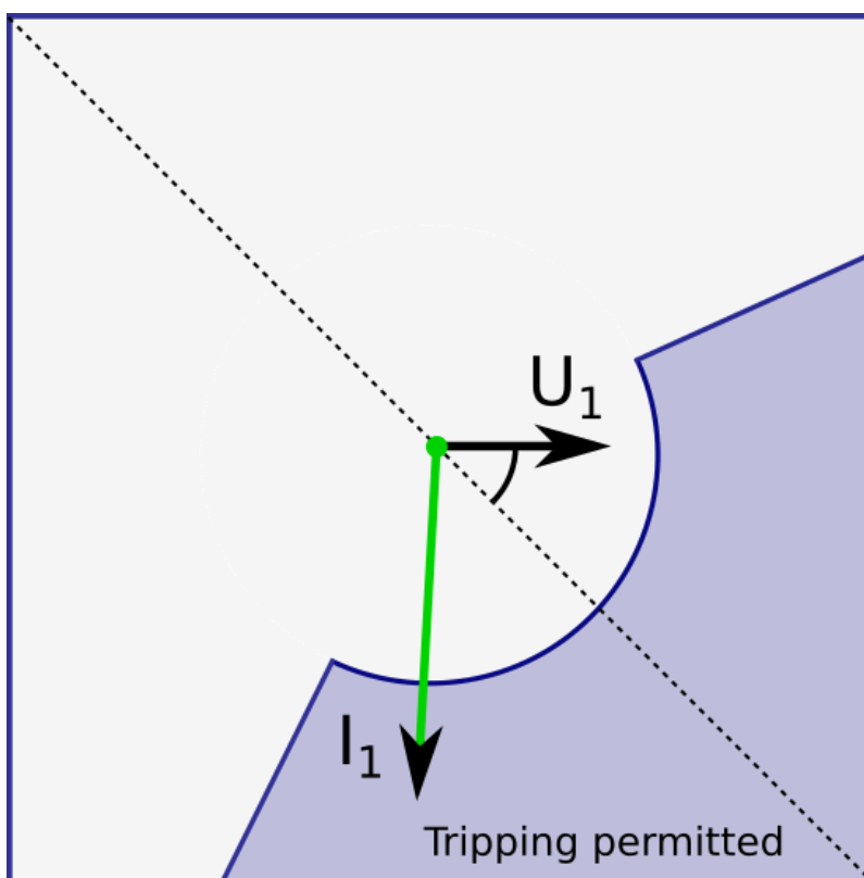
Figure. 5.3.4 - 90. Operation sector area when the sector center has been set to -45 degrees.
