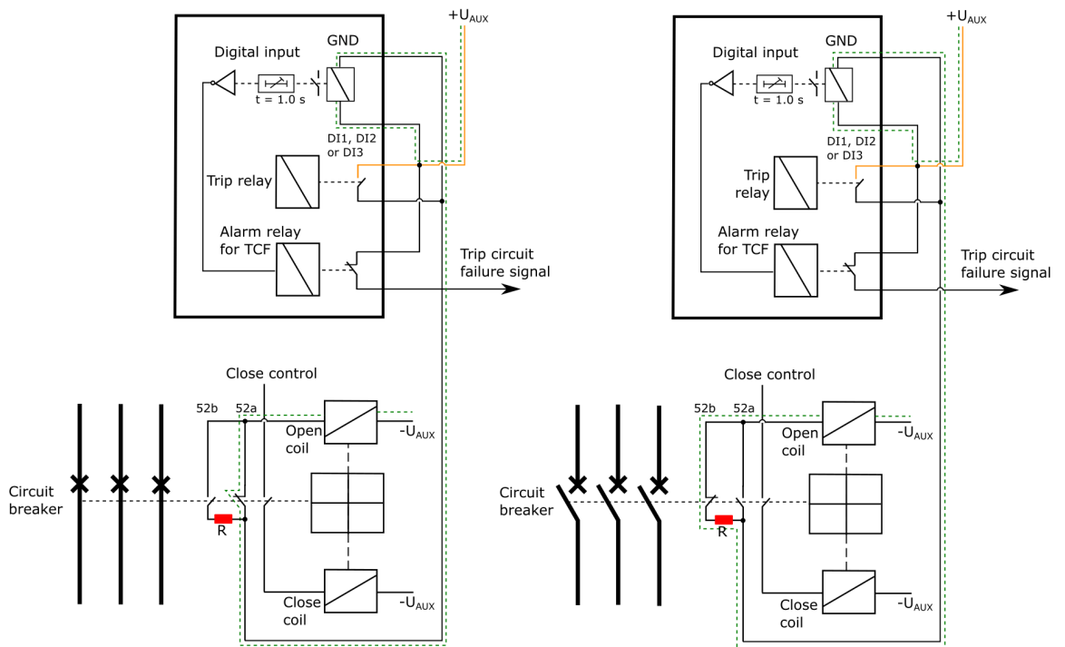
Figure. 7.4 - 235. Trip circuit supervision with one DI and one non-latched trip output.
