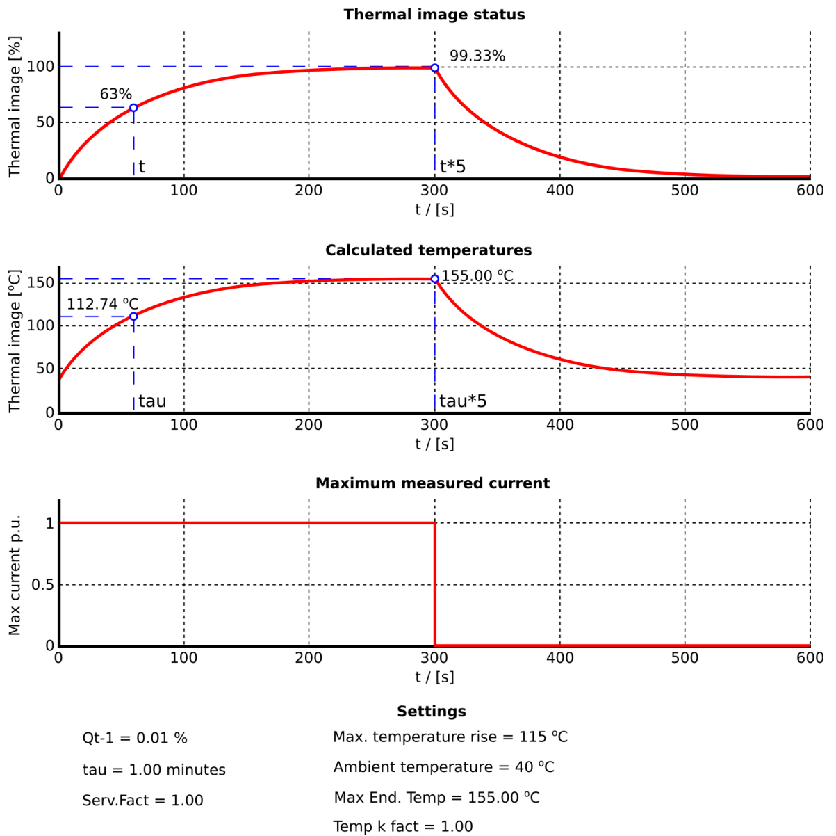
Figure. 5.3.19 - 147. Example of thermal image calculation with nominal conditions.
