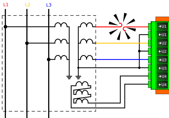
Figure. 5.5.2 - 220. Secondary circuit fault in phase L1 wiring.
