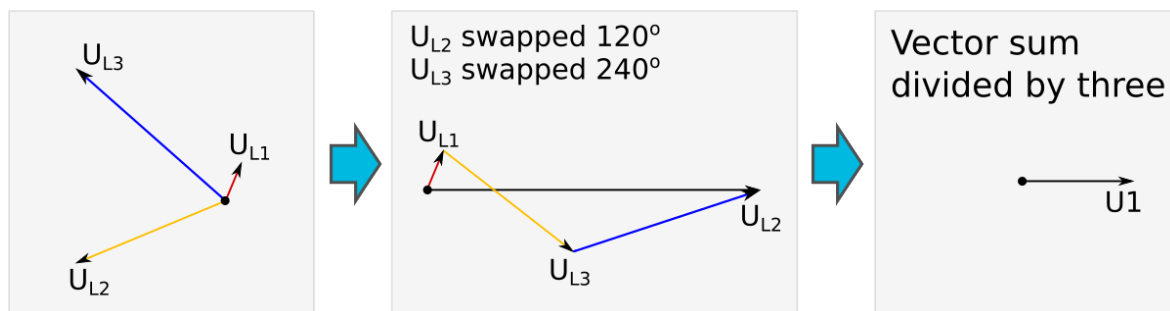
Figure. 5.3.13 - 130. Close-distance short-circuit between phases 1 and 3.
