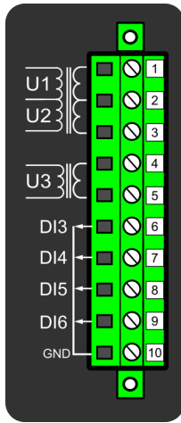
Figure. 8.4 - 244. Voltage measurement module.
