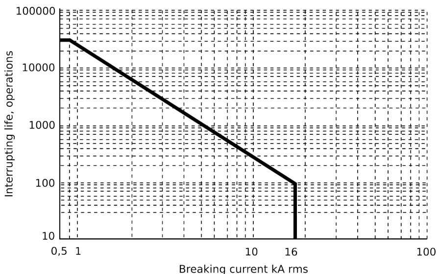
Figure. 5.5.3 - 222. Example of the circuit breaker interrupting life operations.
