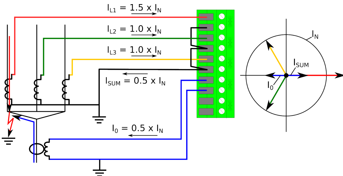
Figure. 5.3.9 - 118. Cable end differential when a fault occurs.
