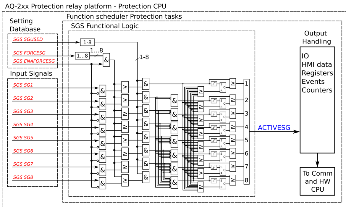
Figure. 5.4.1 - 167. Simplified function block diagram of the setting group selection function.
