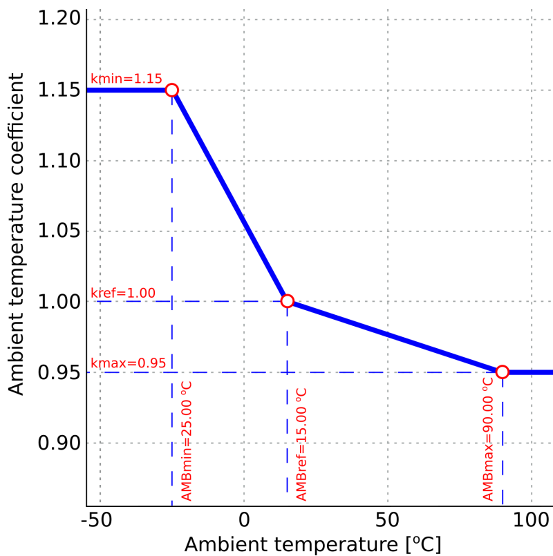
Figure. 5.3.19 - 148. Ambient temperature coefficient calculation (a three-point linear approximation and a settable correction curve).
