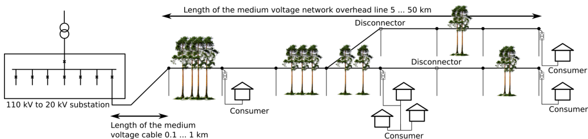
Figure. 5.4.4 - 175. Diagram of a typical radial medium-voltage network in rural areas.
