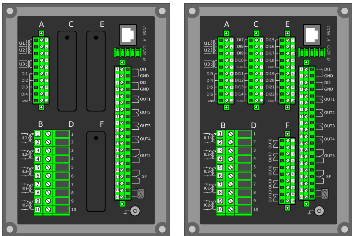
Figure. 8.1 - 240. Modular construction of AQ-X213.
