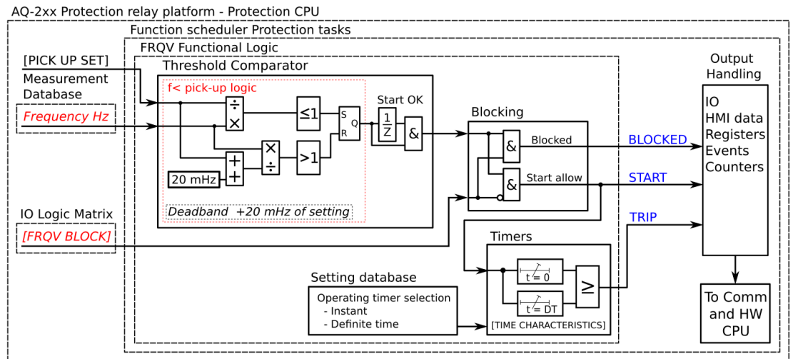
Figure. 5.3.14 - 137. Simplified function block diagram of the f< function.
