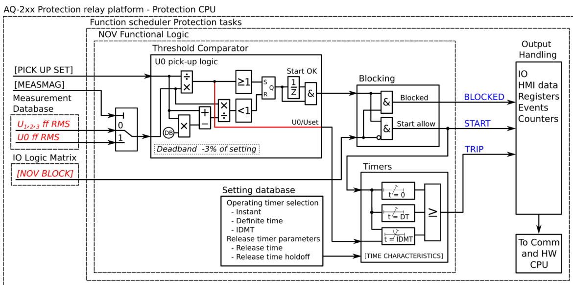
Figure. 5.3.12 - 127. Simplified function block diagram of the U0> function.
