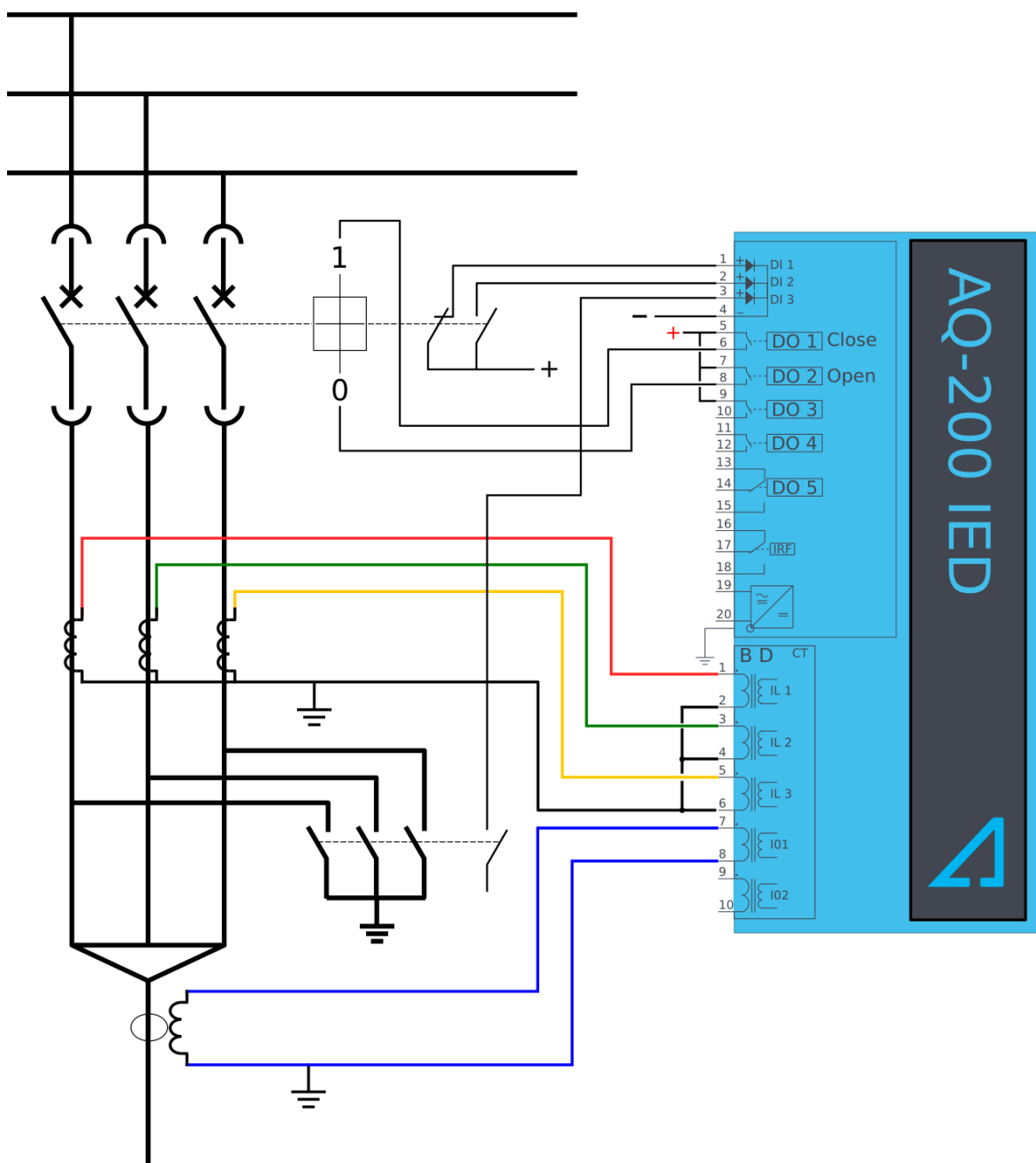
Figure. 5.4.2 - 174. Example of an interlock application.
