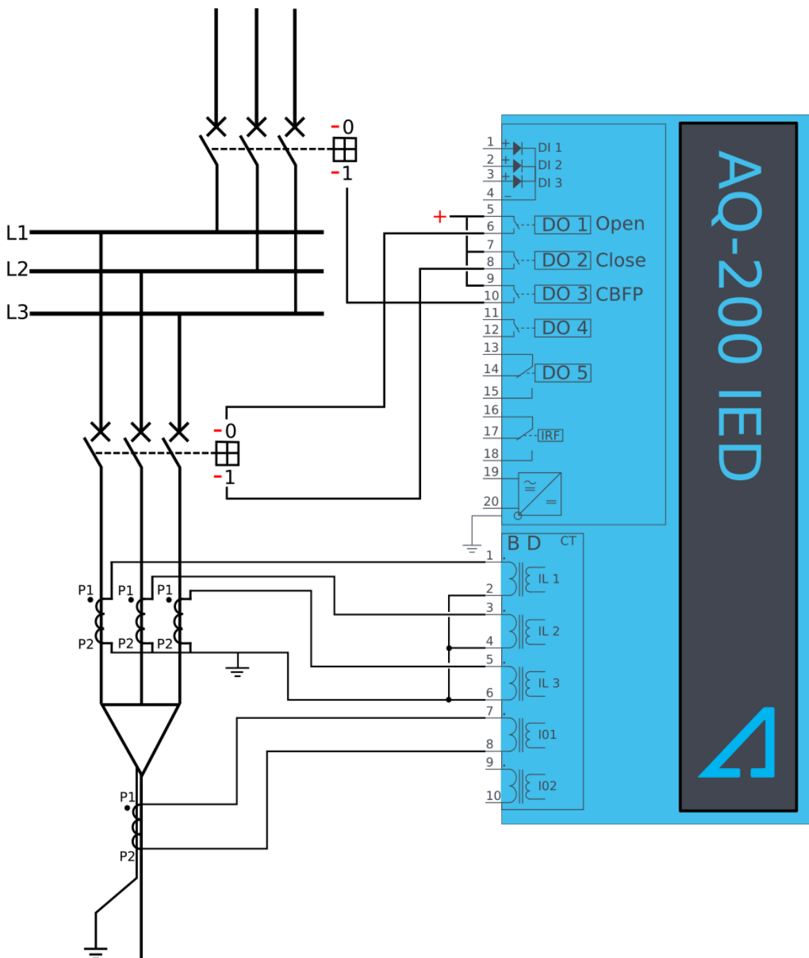
Figure. 5.3.8 - 106. Wiring diagram when Trip and CBFP are configured to the device.
