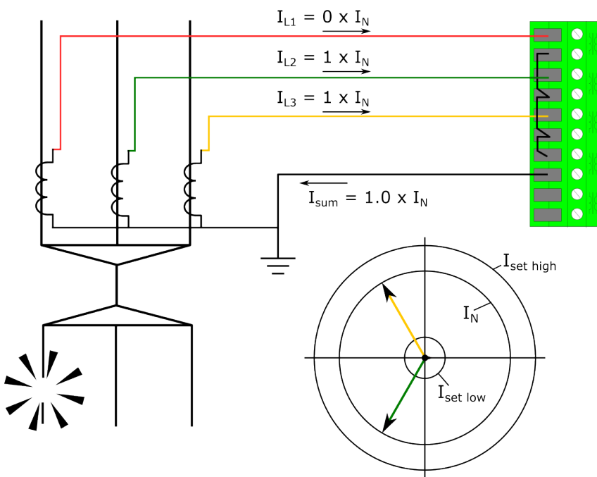
Figure. 5.5.1 - 213. Primary circuit fault in phase L1 wiring.
