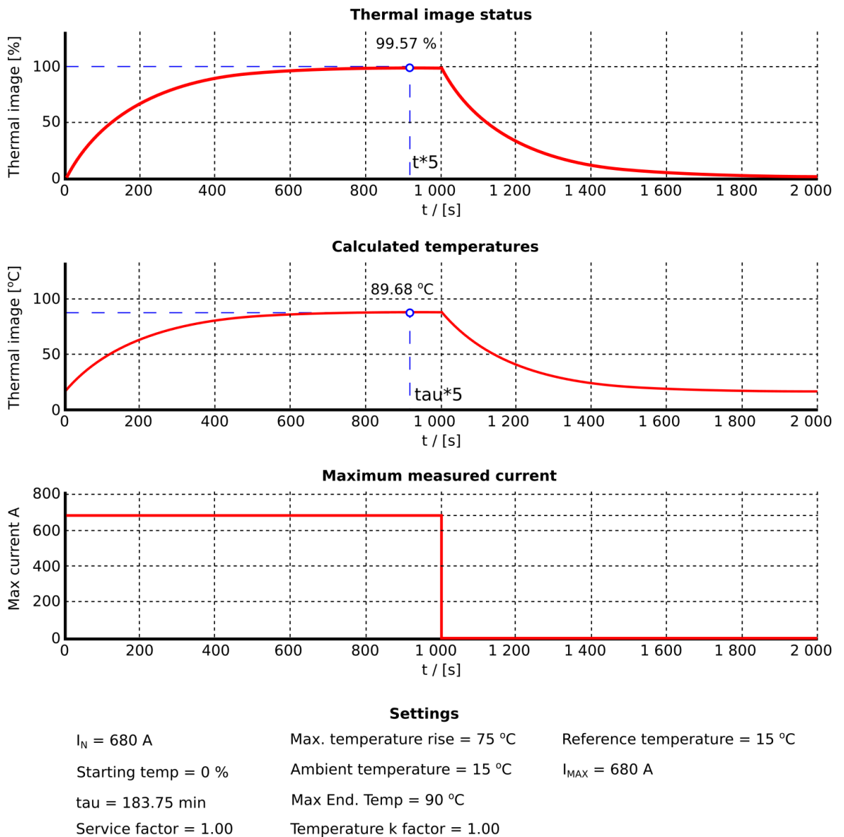
Figure. 5.3.19 - 156. Thermal image response with maximum load (installation according presumptions).
