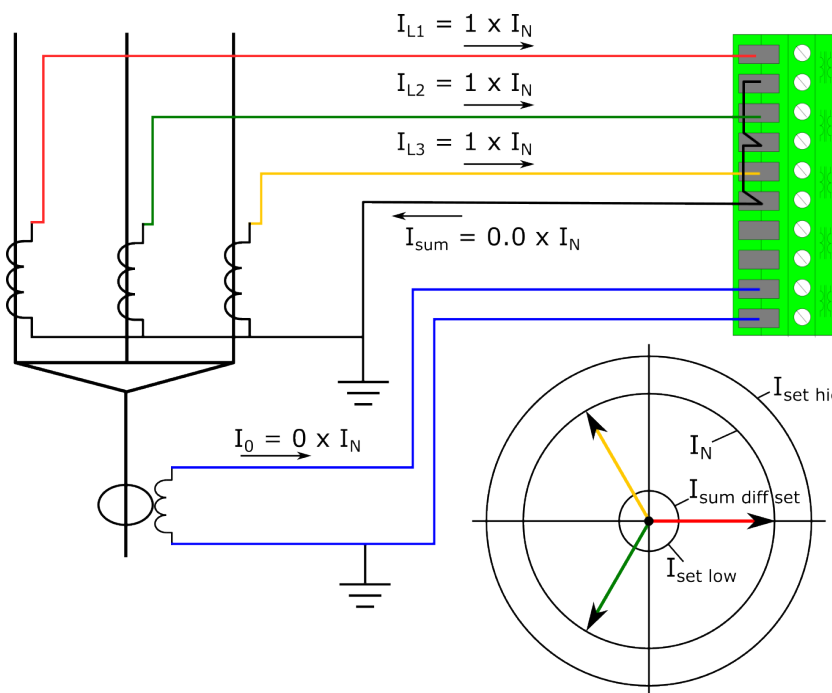
Figure. 5.5.1 - 216. Normal situation, residual current also measured.
