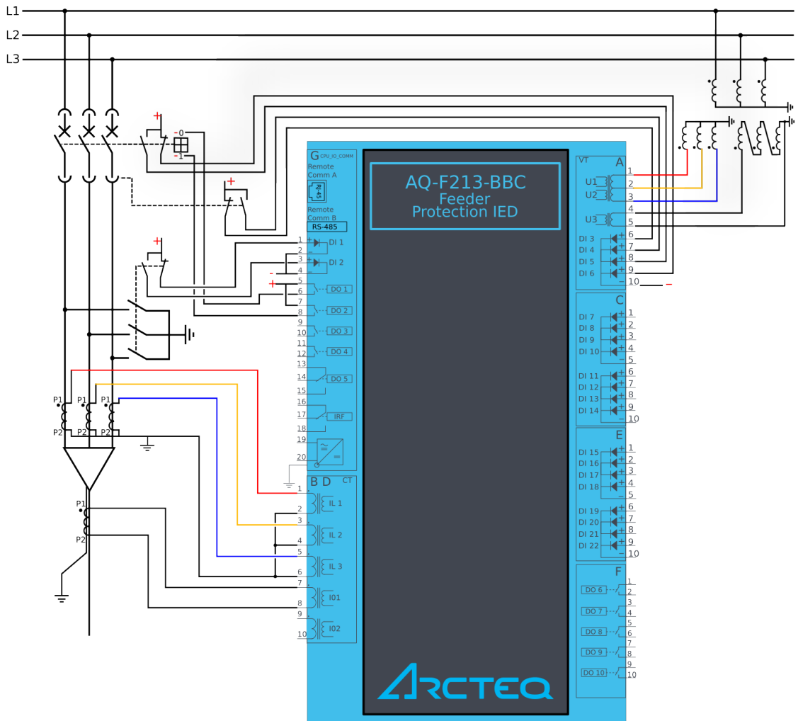
Figure. 7.2 - 233. Application example and its connections.
