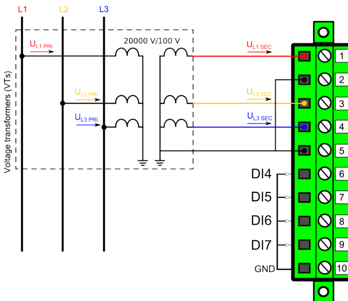
Figure. 5.2.2 - 70. Example connections for 2LL+U0 voltage measurement.
