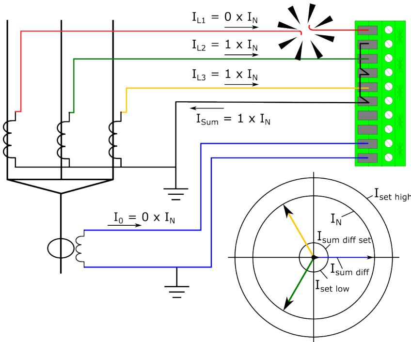
Figure. 5.5.1 - 217. Broken secondary phase current wiring.
