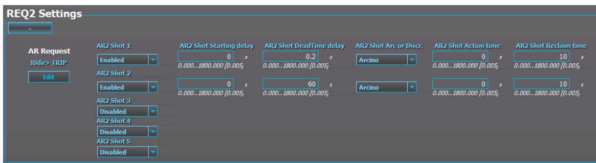
Figure. 5.4.4 - 182. Settings for I0dir> with two shots.
