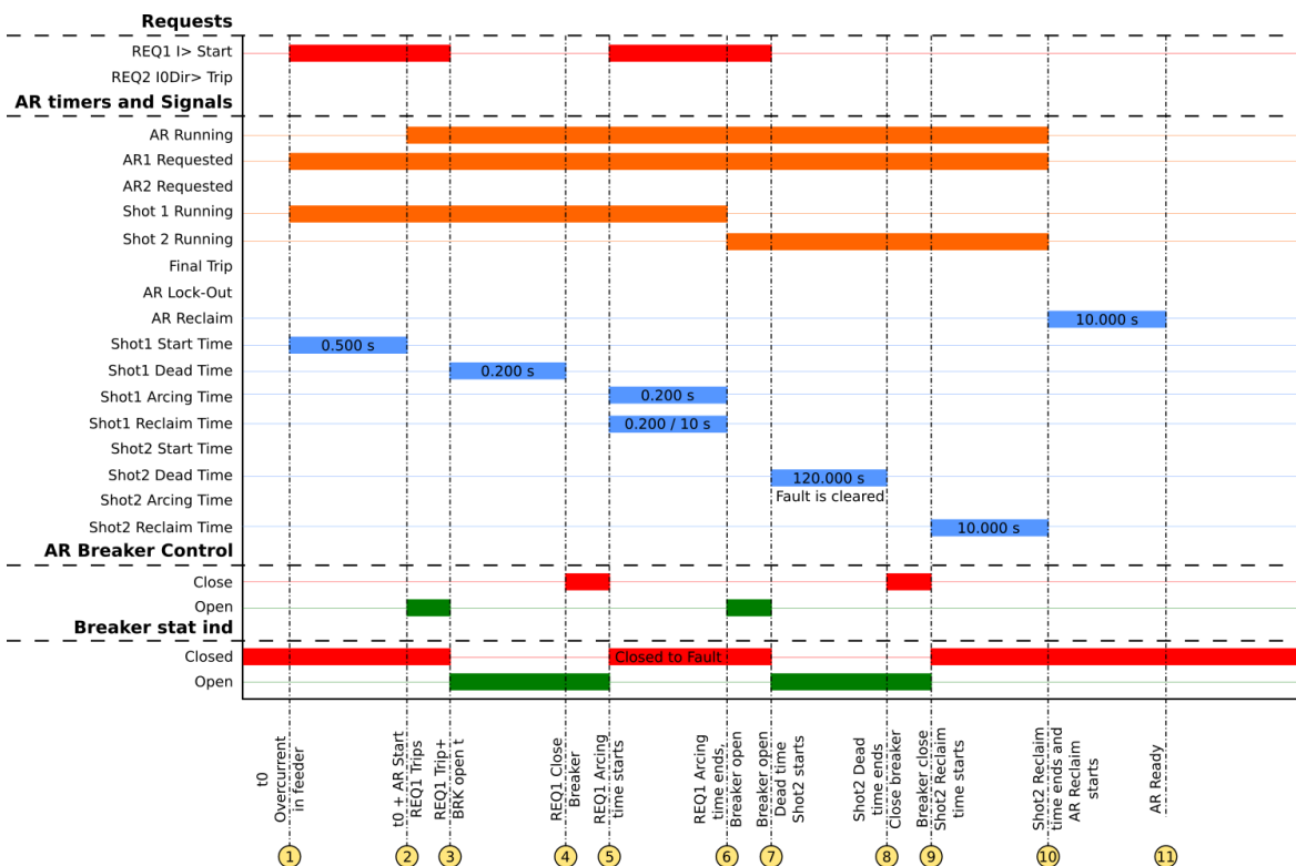
Figure. 5.4.4 - 187. Signal status graph of the semi-permanent overcurrent auto-recloser cycle.
