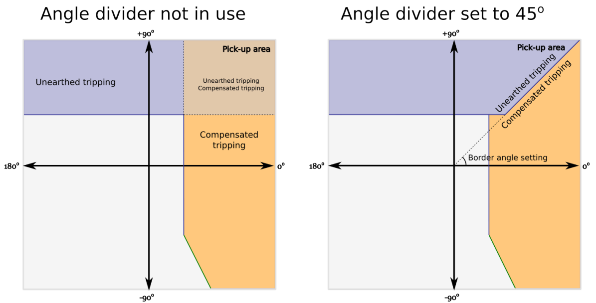
Figure. 5.3.5 - 97. Effect of angle divider when in use and when disabled.
