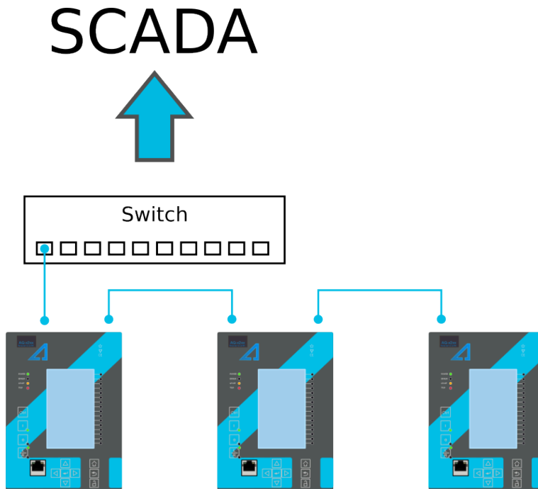
Figure. 8.11 - 255. Example of a multidrop configuration.
