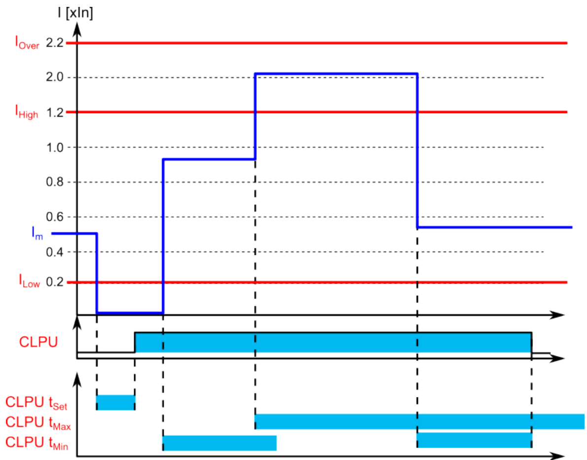
Figure. 5.4.5 - 199. Example of timers and pick-up parameters (an inrush current detected during T_{min} time).
