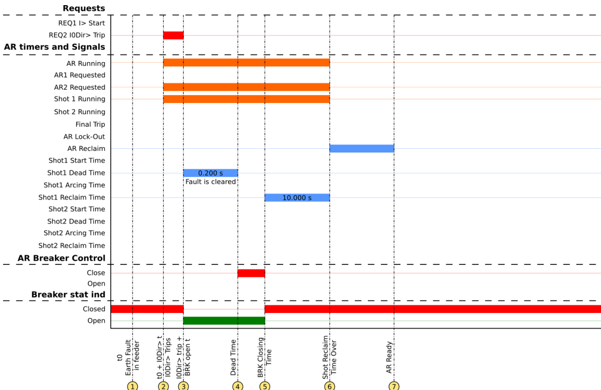
Figure. 5.4.4 - 183. Signal status graph of the transient earth fault auto-recloser cycle.
