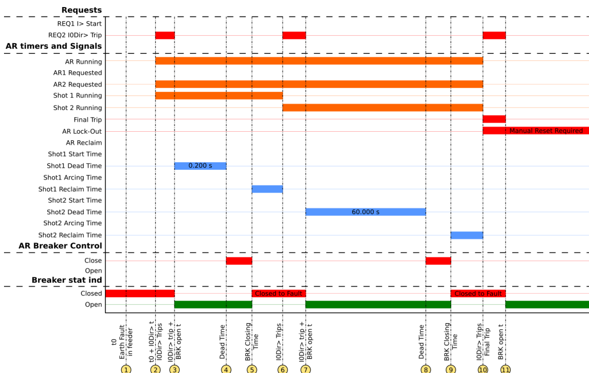
Figure. 5.4.4 - 179. Signal status graph of the permanent earth fault auto-recloser cycle.
