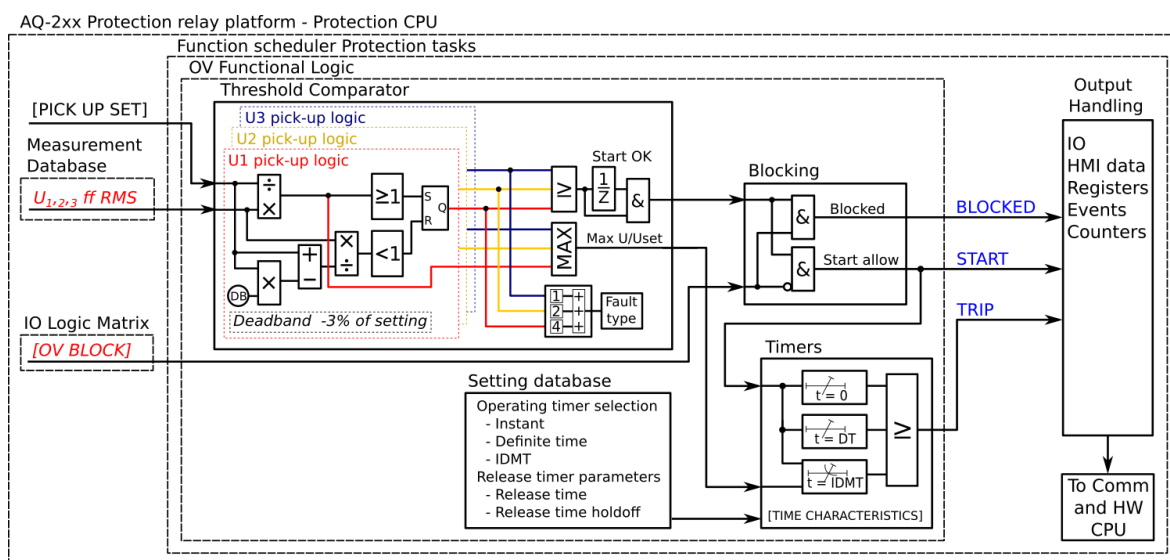
Figure. 5.3.10 - 121. Simplified function block diagram of the U> function.
