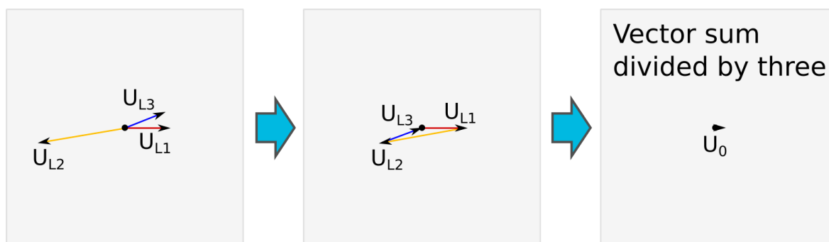
Figure. 5.3.12 - 126. Close-distance short-circuit between phases 1 and 3.
