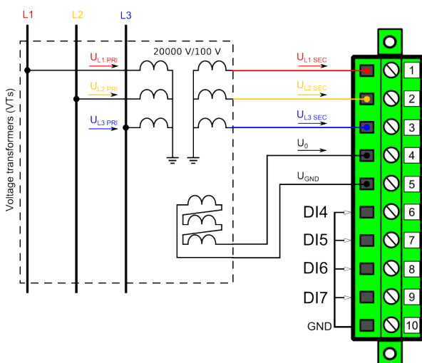
Figure. 5.2.2 - 66. Connections.
