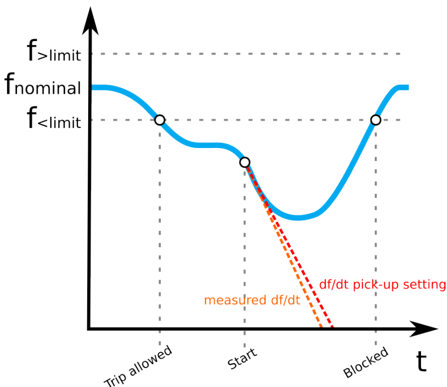
Figure. 5.3.15 - 138. Operation of the df/dt function when the frequency starts but doesn't trip.
