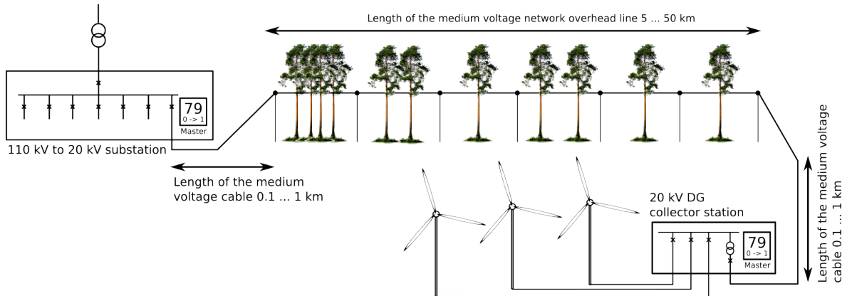
Figure. 5.4.4 - 190. Auto-reclosing with distributed generation in the line.
