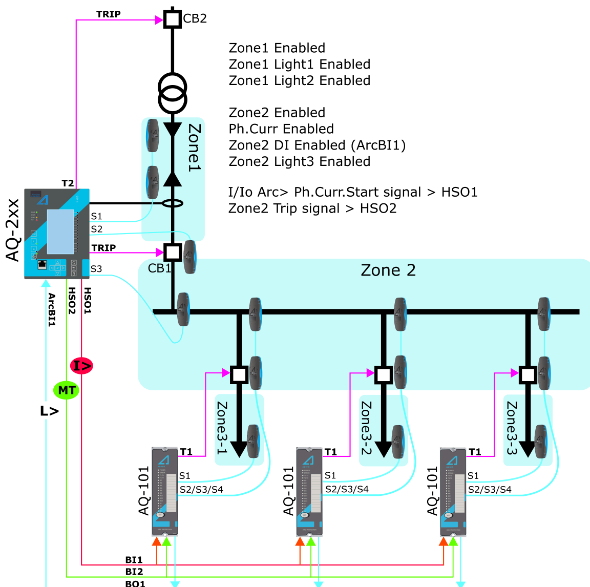
Figure. 5.3.21 - 162. Scheme IA1 (with AQ-101 arc protection relays).
