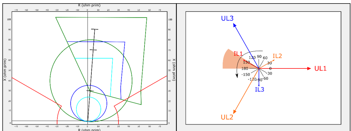
Figure. 5.3.23 - 164. Distance protection characteristics and directional overcurrent.
