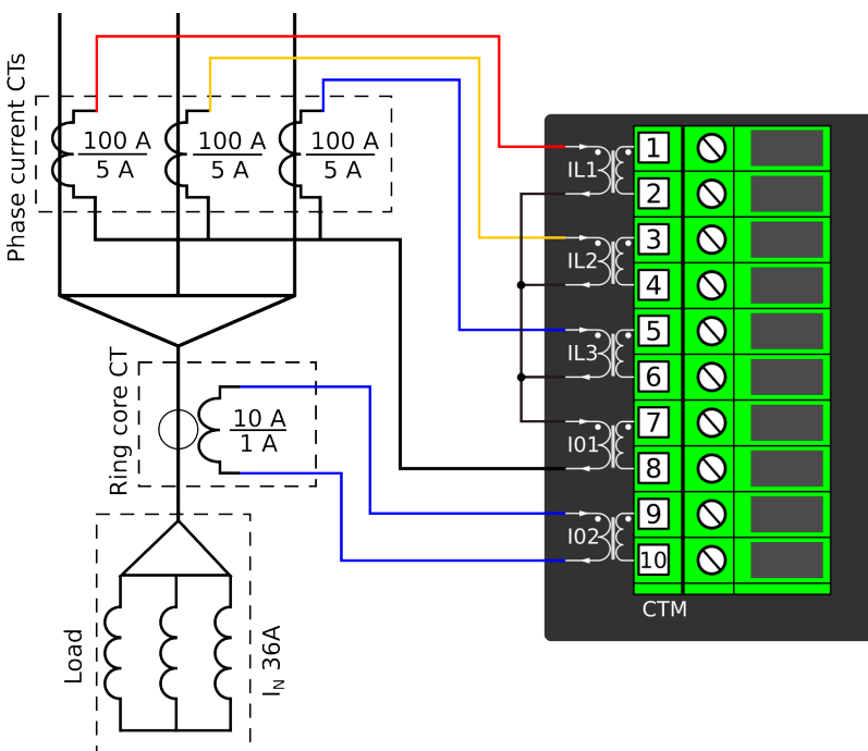
Figure. 5.2.1 - 55. Connections.
