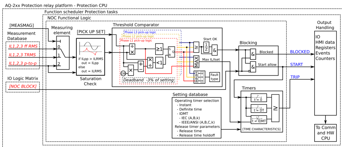
Figure. 5.3.2 - 86. Simplified function block diagram of the I> function.
