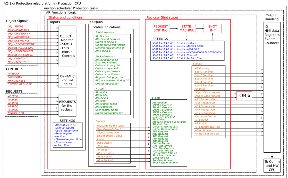
Figure. 5.4.4 - 191. Simplified function block diagram of the auto-recloser function.
