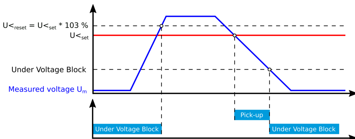
Figure. 5.3.13 - 135. Example of the block setting operation.
