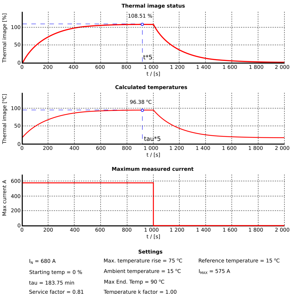
Figure. 5.3.19 - 157. Thermal image response with nominal currents and fine-tuned k_{\text{SF}} correction factor.
