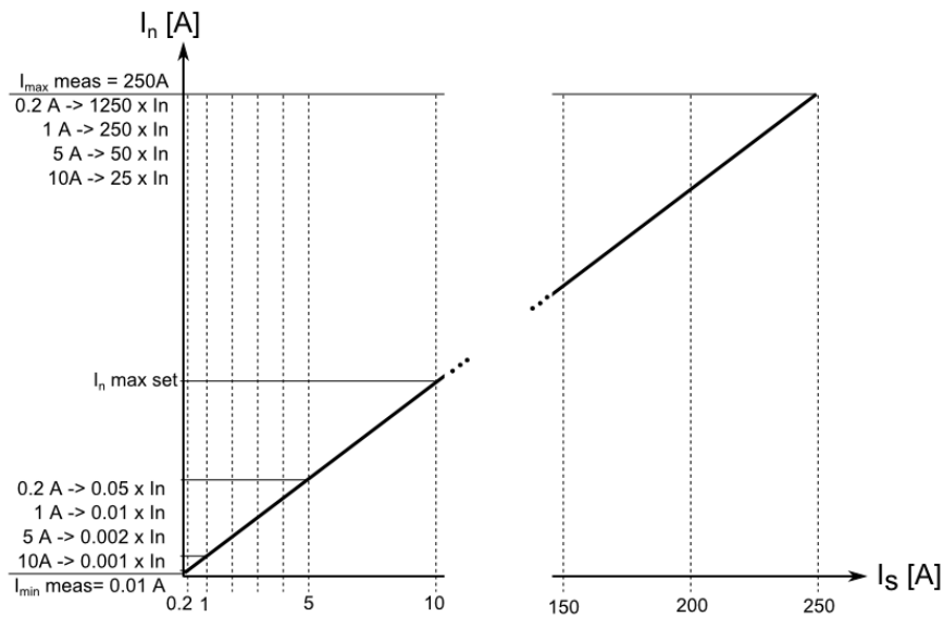
Figure. 5.3.1 - 79. Measurement range in relation to the nominal current.
