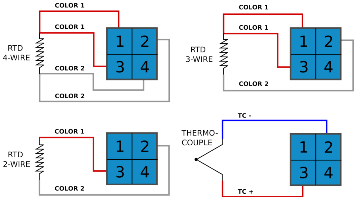
Figure. 8.8 - 250. Different sensor types and their connections.
