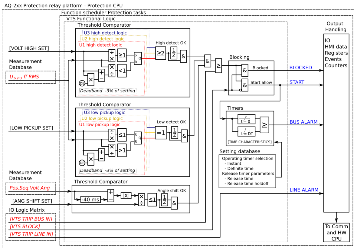
Figure. 5.5.2 - 221. Simplified function block diagram of the VTS function.
