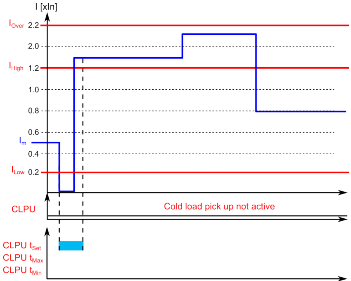
Figure. 5.4.5 - 195. Example of timers and pick-up parameters (no cold load pick-up, I_{low} too short).
