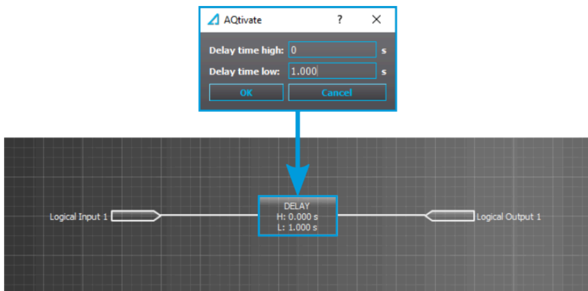
Figure. 5.4.12 - 208. Extending a logical input pulse.
