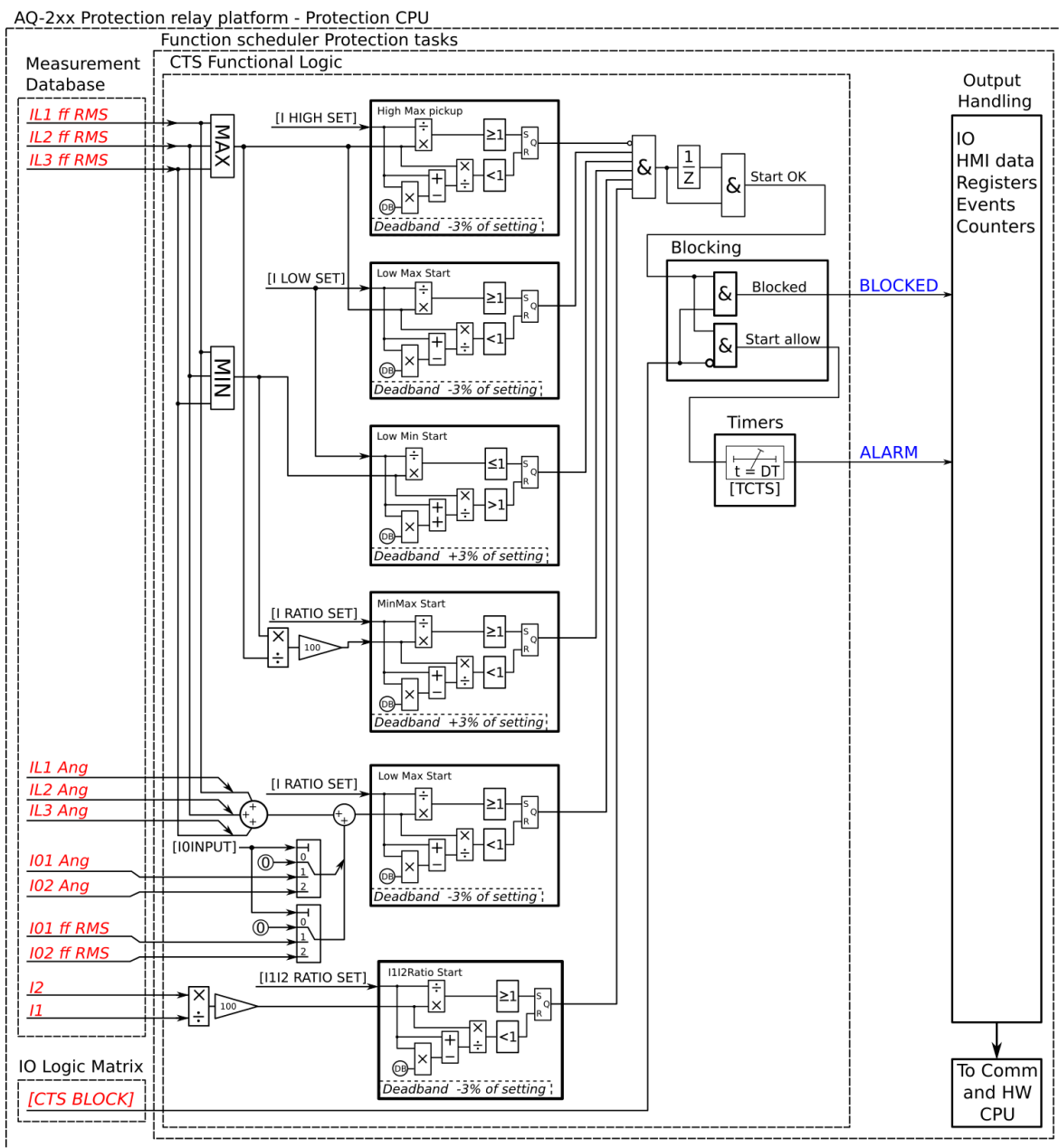
Figure. 5.5.1 - 210. Simplified function block diagram of the CTS function.
