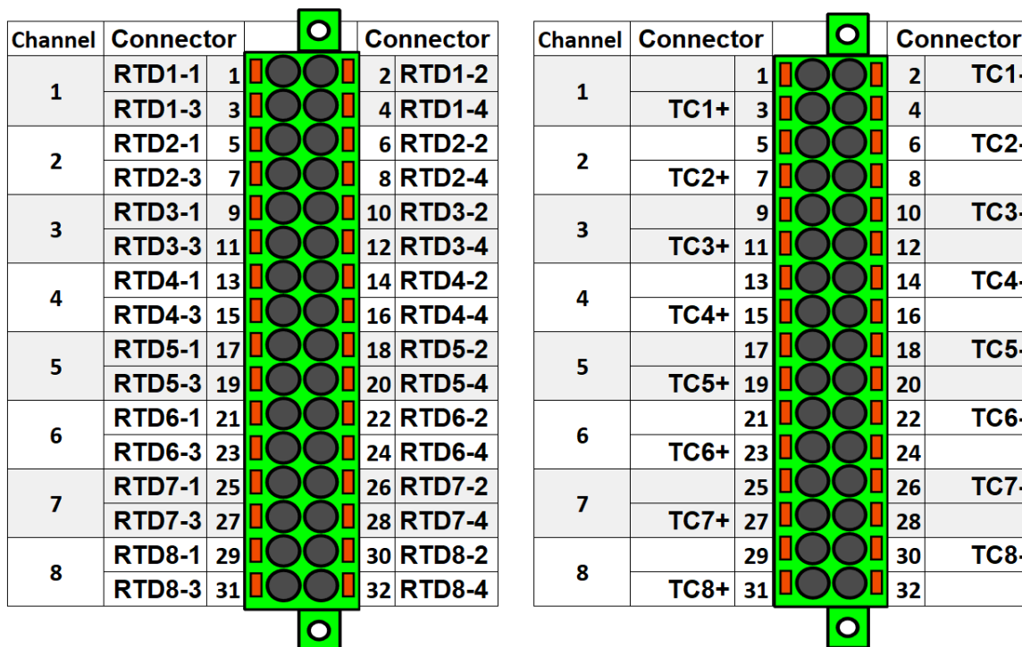
Figure. 8.8 - 249. RTD input module connectors.
