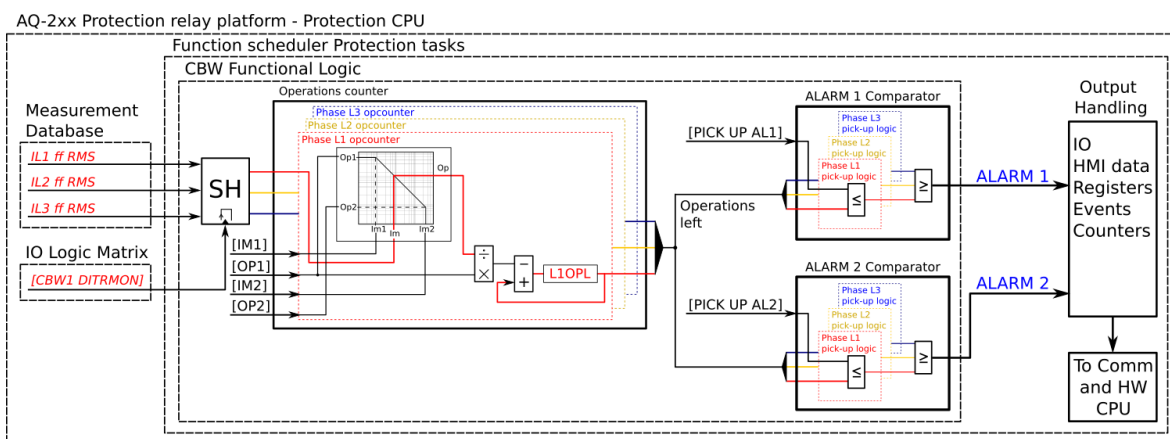
Figure. 5.5.3 - 223. Simplified function block diagram of the circuit breaker wear function.
