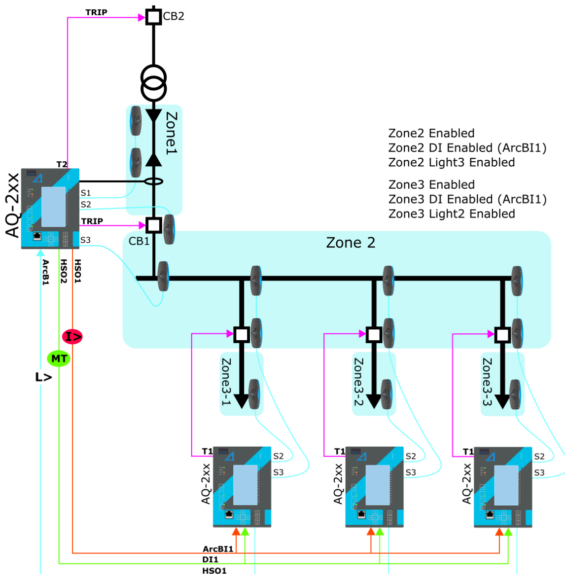
Figure. 5.3.21 - 163. Scheme IA1 (with AQ-200 protection relays).
