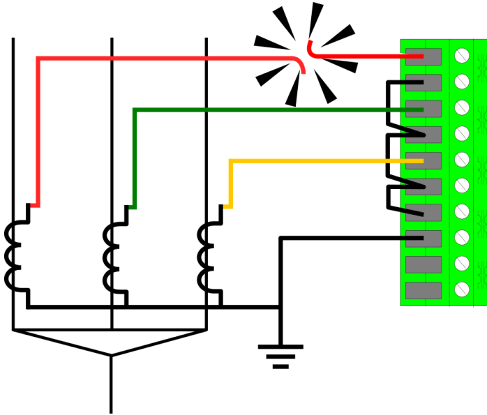
Figure. 5.5.1 - 209. Secondary circuit fault in phase L1 wiring.
