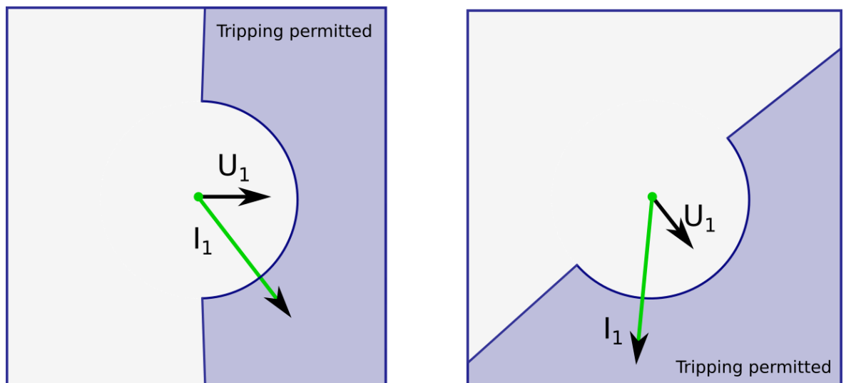
Figure. 5.3.4 - 89. Angle tracking of the I_{dir} > function (3LN/3LL + U_0 mode).
