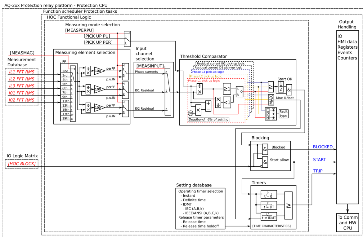
Figure. 5.3.7 - 100. Simplified function block diagram of the I h > function.
