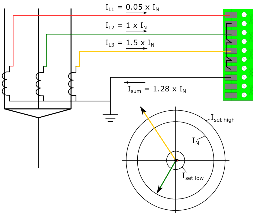
Figure. 5.5.1 - 214. No wiring fault but heavy unbalance.
