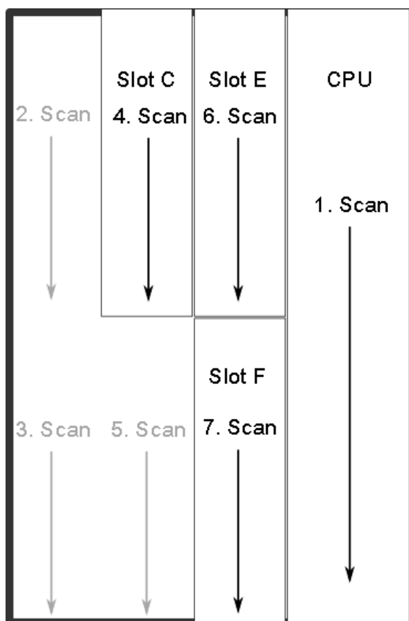
Figure. 8.1 - 241. AQ-X213 hardware scanning and I/O naming principles.
