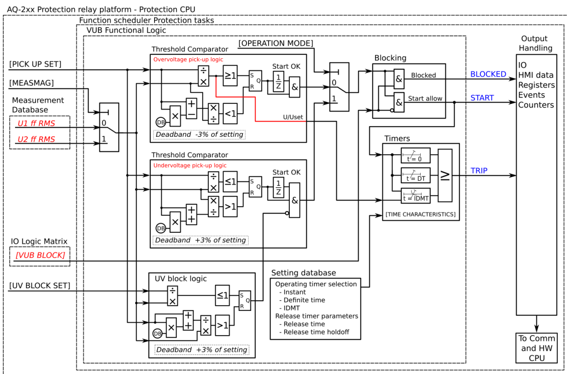
Figure. 5.3.13 - 134. Simplified function block diagram of the U1/U2>/< function.
