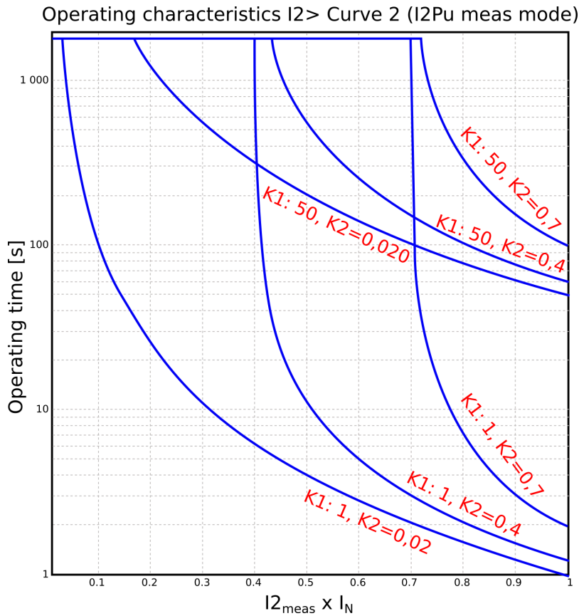
Figure. 5.3.6 - 99. Operation characteristics curve for I2> Curve2.
