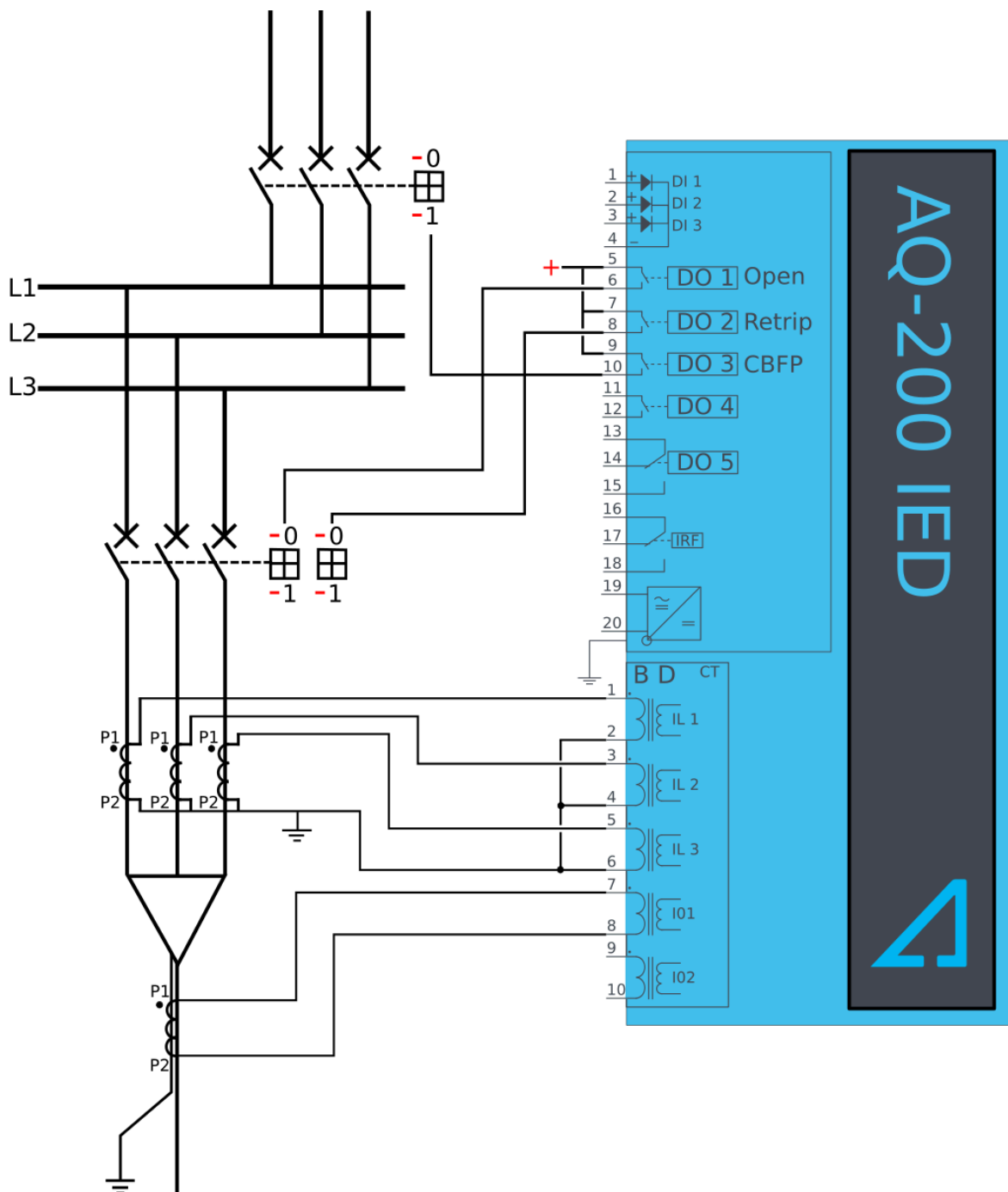
Figure. 5.3.8 - 102. Wiring diagram when Trip, Retrip and CBFP are configured to the device.
