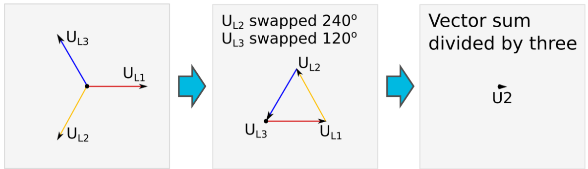
Figure. 5.3.13 - 132. Earth fault in isolated network.
