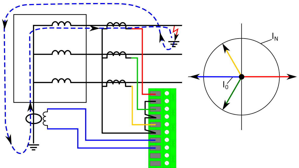
Figure. 5.3.9 - 119. Restricted earth fault outside a Y winding transformer.
