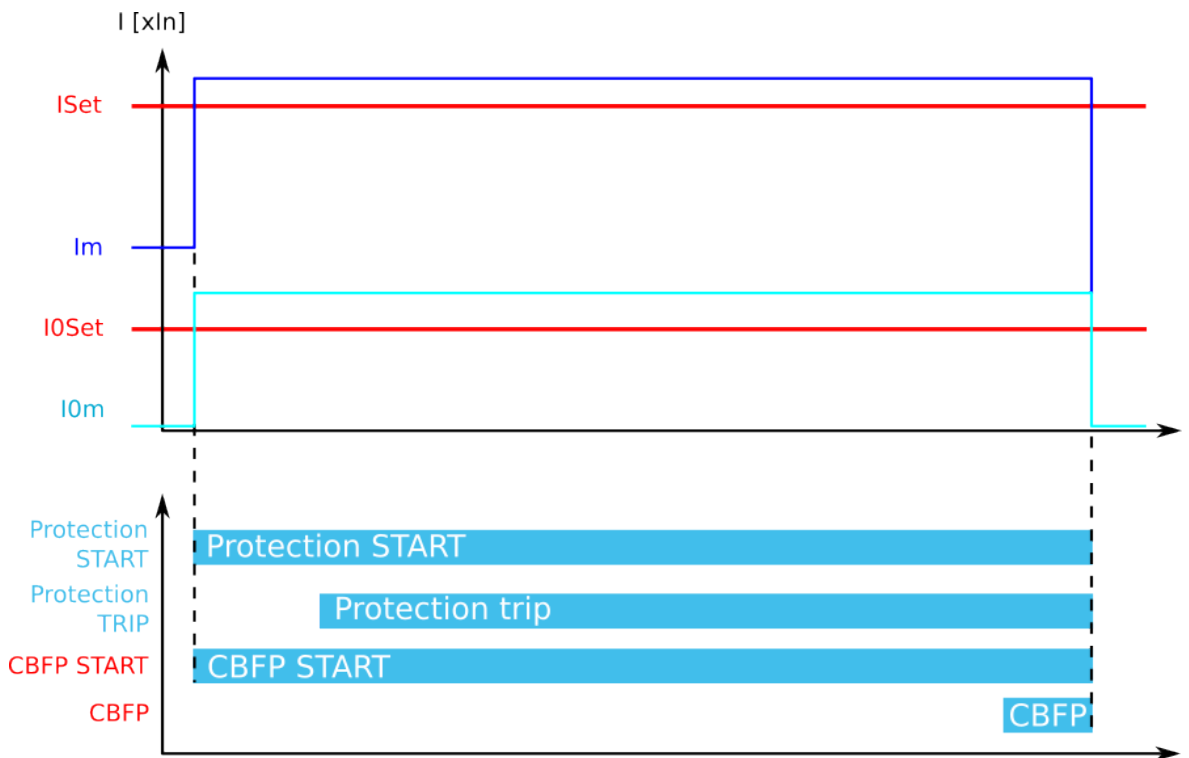
Figure. 5.3.8 - 107. CBFP when "Current" is the selected criterion.
