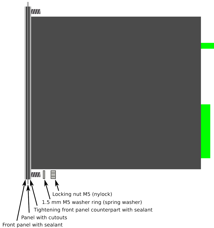
Figure. 8.14 - 261. Device installation.
