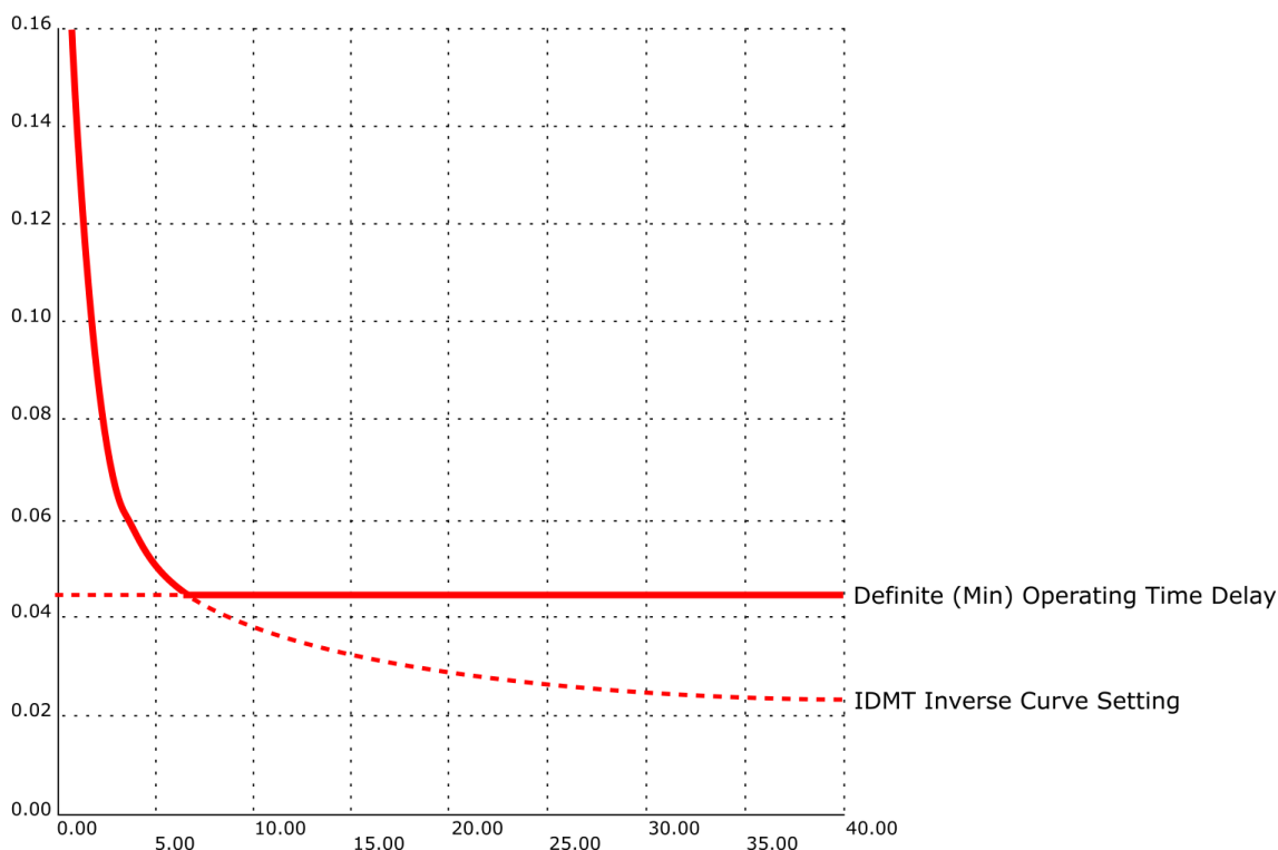
Figure. 5.3.1 - 80. Operating time delay: Definite (Min) and the minimum for tripping.
