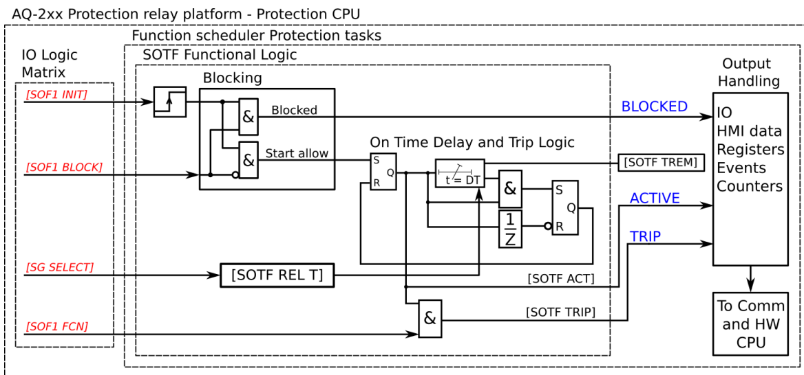
Figure. 5.4.6 - 200. Simplified function block diagram of the switch-on-to-fault function.
