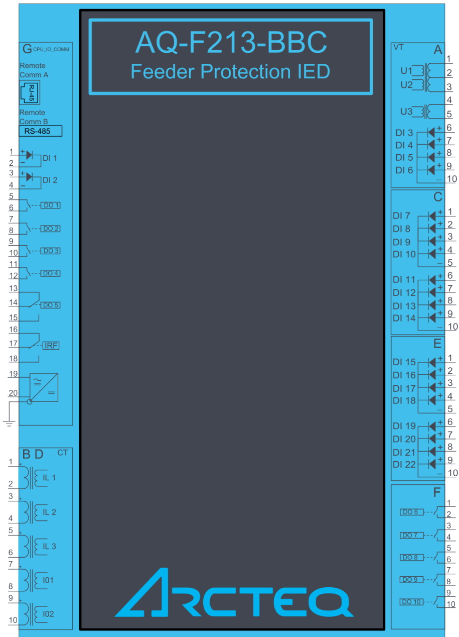
Figure. 7.1 - 231. AQ-F213 variant with digital input and output modules.
