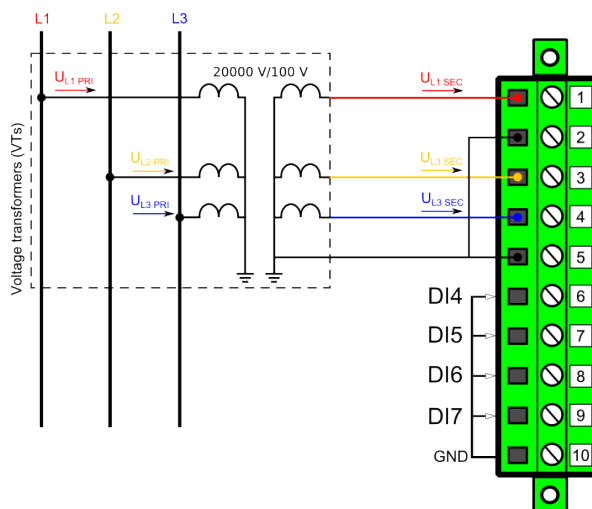
Figure. 5.2.2 - 65. Voltage measurement terminology
