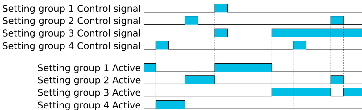
Figure. 5.4.1 - 168. Example sequences of group changing (control with pulse only, or with both pulses and static signals).
