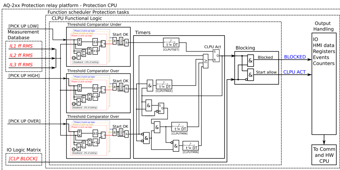
Figure. 5.4.5 - 193. Simplified function block diagram of the cold load pick-up function.
