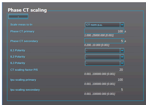
Figure. 5.2.1 - 56. Setting the phase current transformer scalings to CT nominal.
