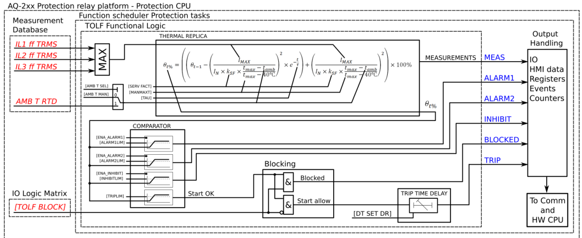
Figure. 5.3.19 - 159. Simplified function block diagram of the TF> function.
