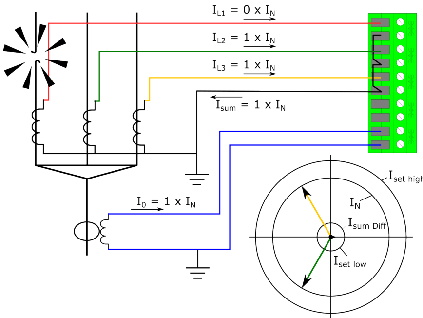
Figure. 5.5.1 - 218. Broken primary phase current wiring.
