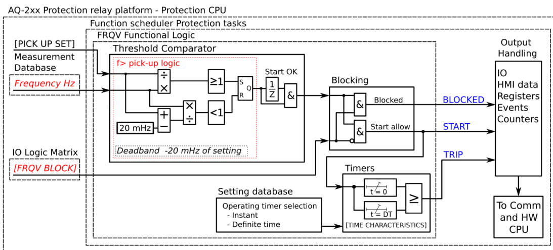
Figure. 5.3.14 - 136. Simplified function block diagram of the f> function.
