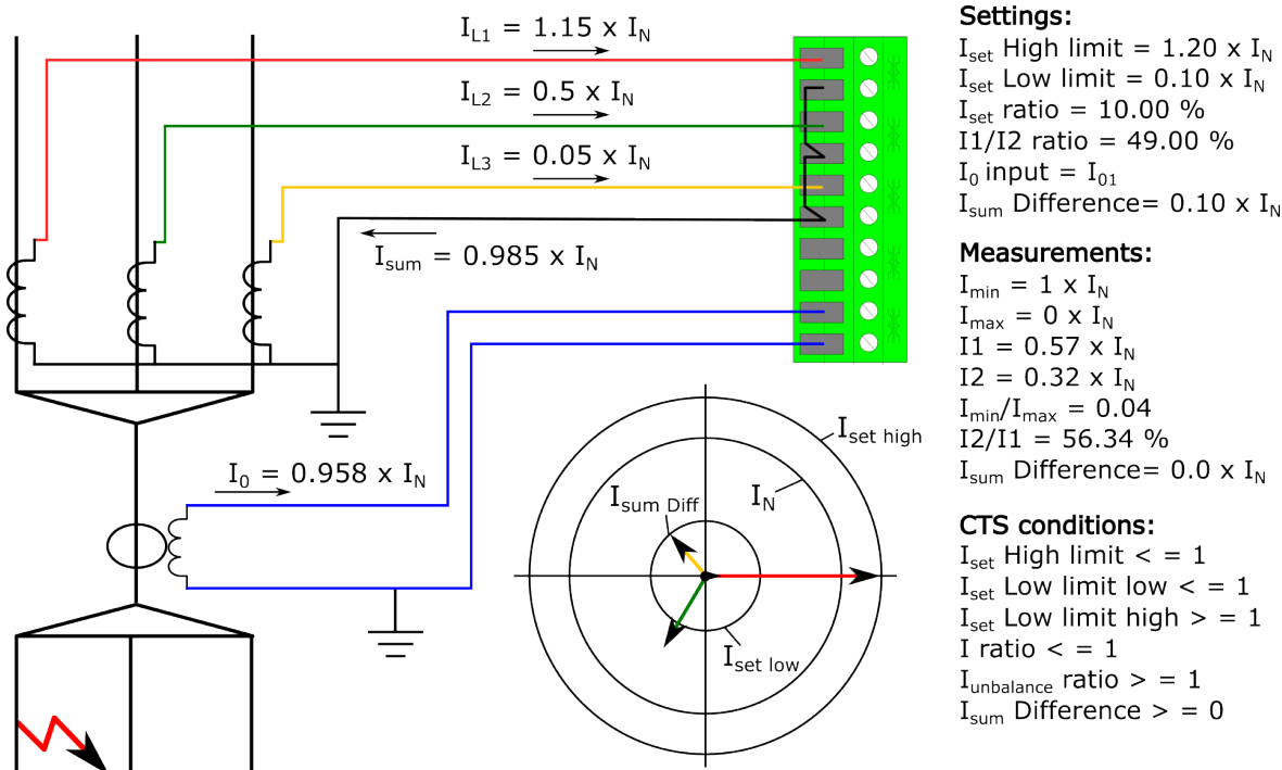
Figure. 5.5.1 - 219. Primary side high-impedance earth fault.
