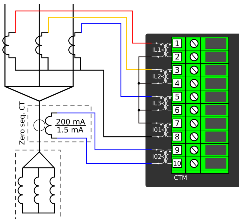
Figure. 5.2.1 - 62. Connections of ZCT scaling.
