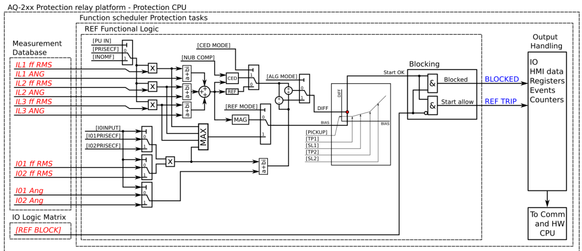
Figure. 5.3.9 - 112. Simplified function block diagram of the I0d> function.
