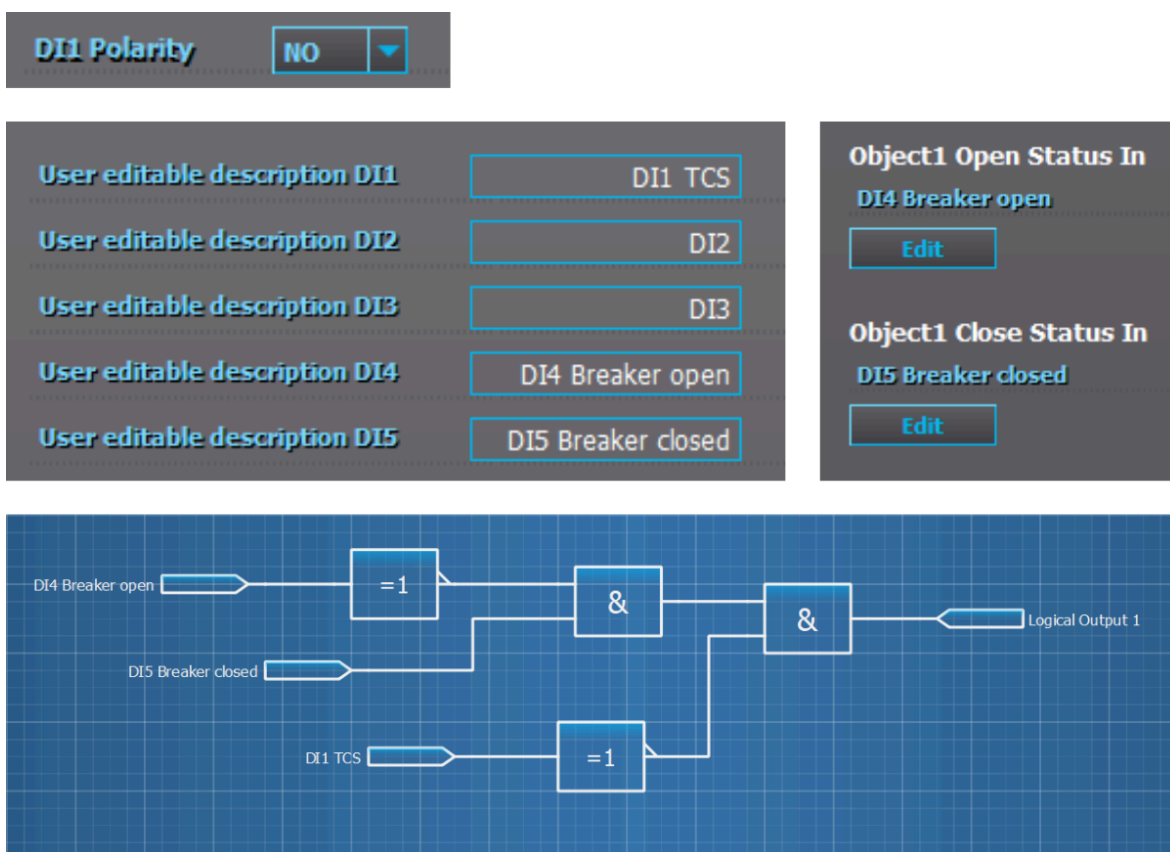
Figure. 7.4 - 239. Example block scheme.
