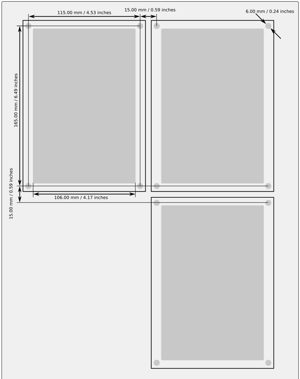
Figure. 8.14 - 262. Panel cutout dimensions and device spacing.
