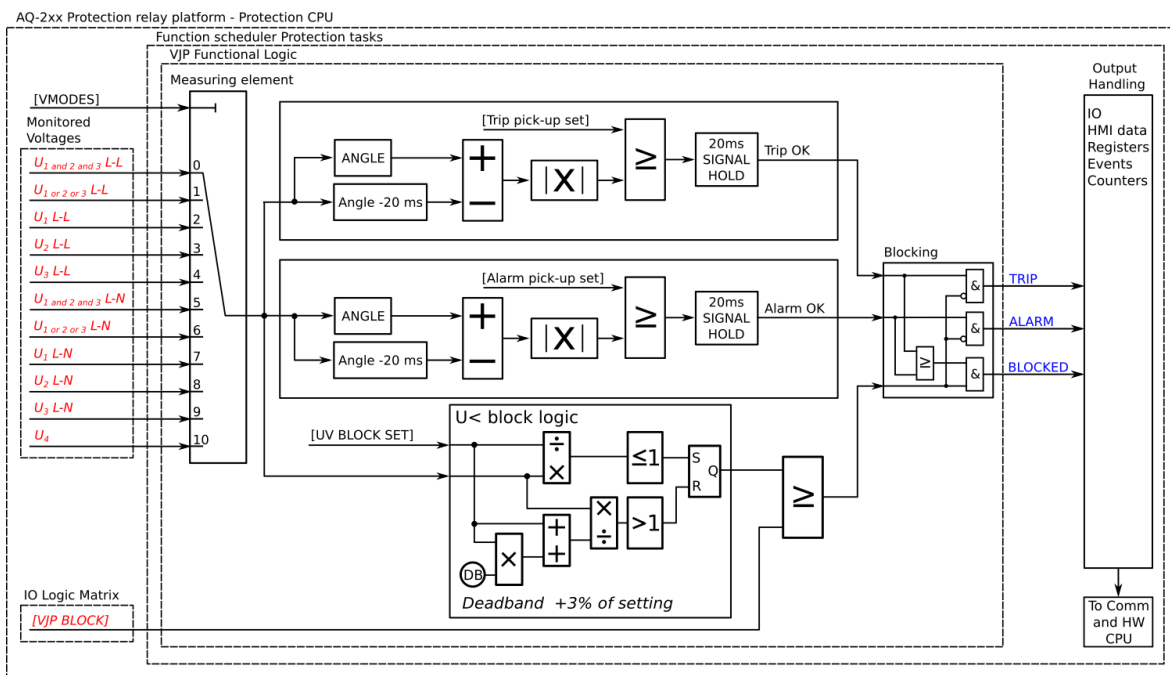
Figure. 5.4.8 - 203. Simplified function block diagram of the \Delta\phi function.
