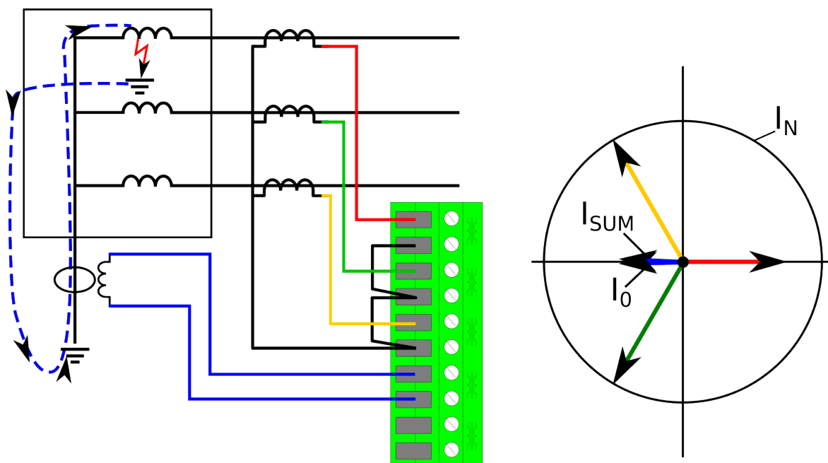
Figure. 5.3.9 - 120. Restricted earth fault inside a Y winding transformer.
