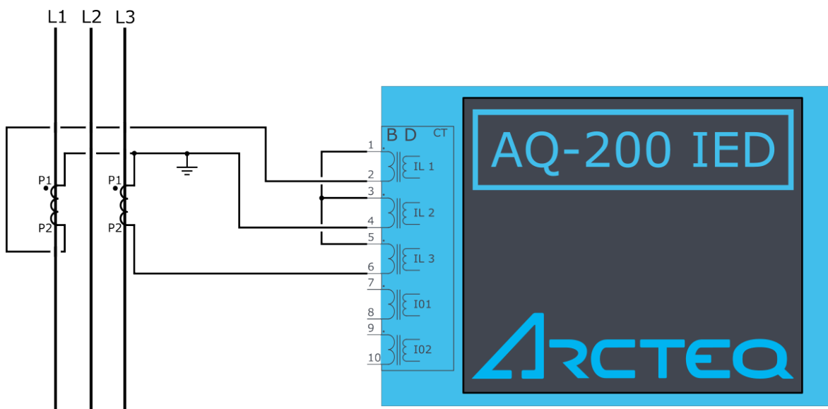
Figure. 7.3 - 234. ARON connection.
