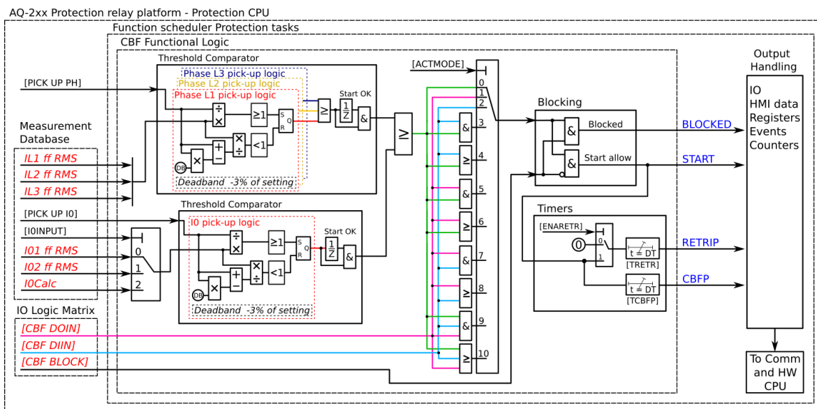
Figure. 5.3.8 - 101. Simplified function block diagram of the CBFP function.
