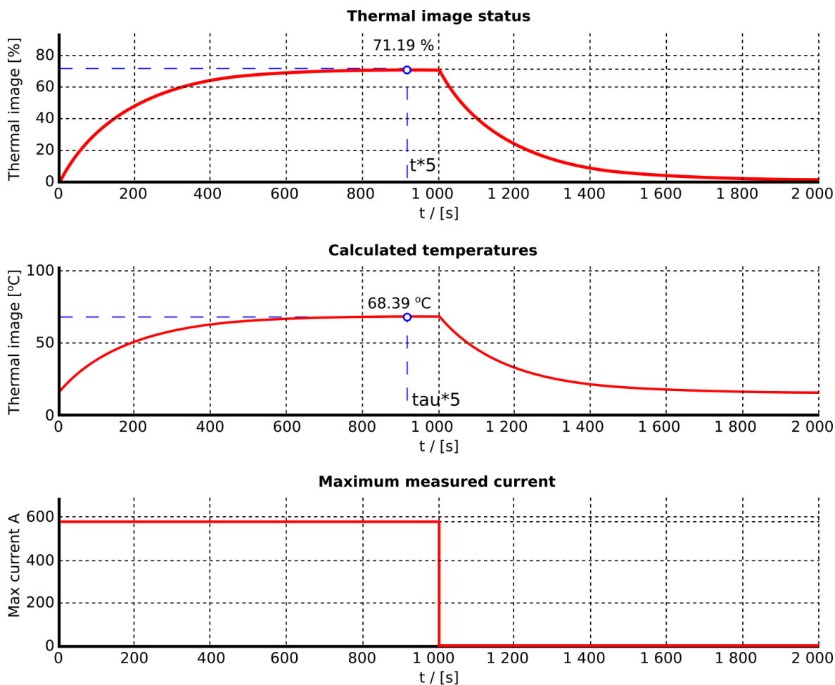
Figure. 5.3.19 - 155. Thermal image response with nominal load (installation according to presumptions).
