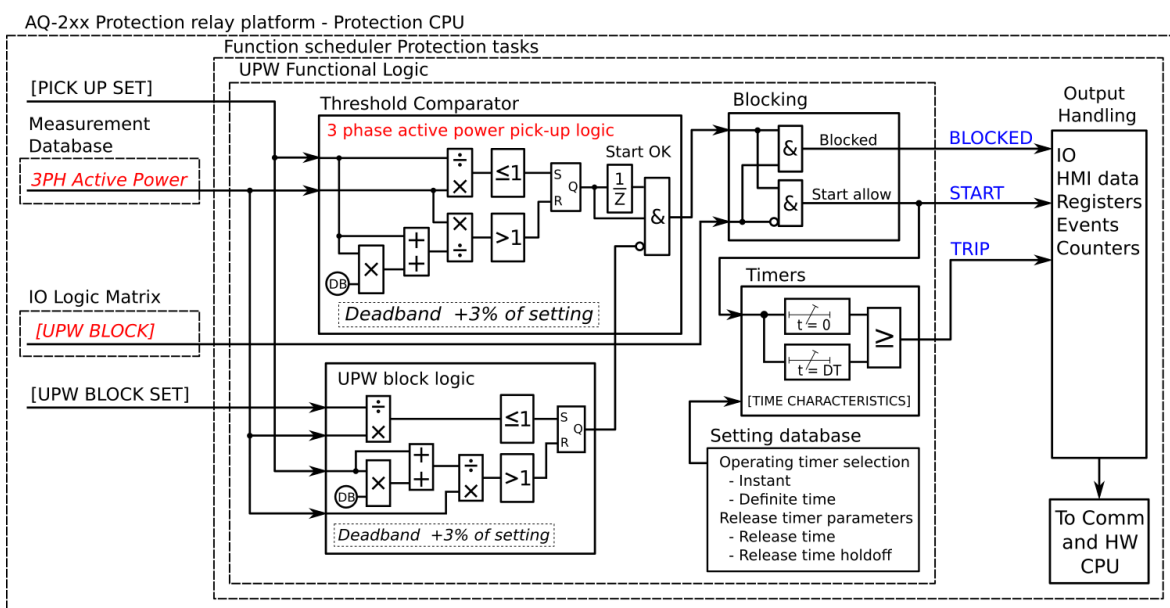
Figure. 5.3.17 - 143. Simplified function block diagram of the P< function.
