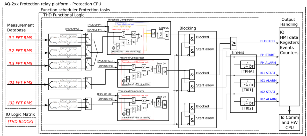
Figure. 5.5.5 - 225. Simplified function block diagram of the total harmonic distortion monitor function.
