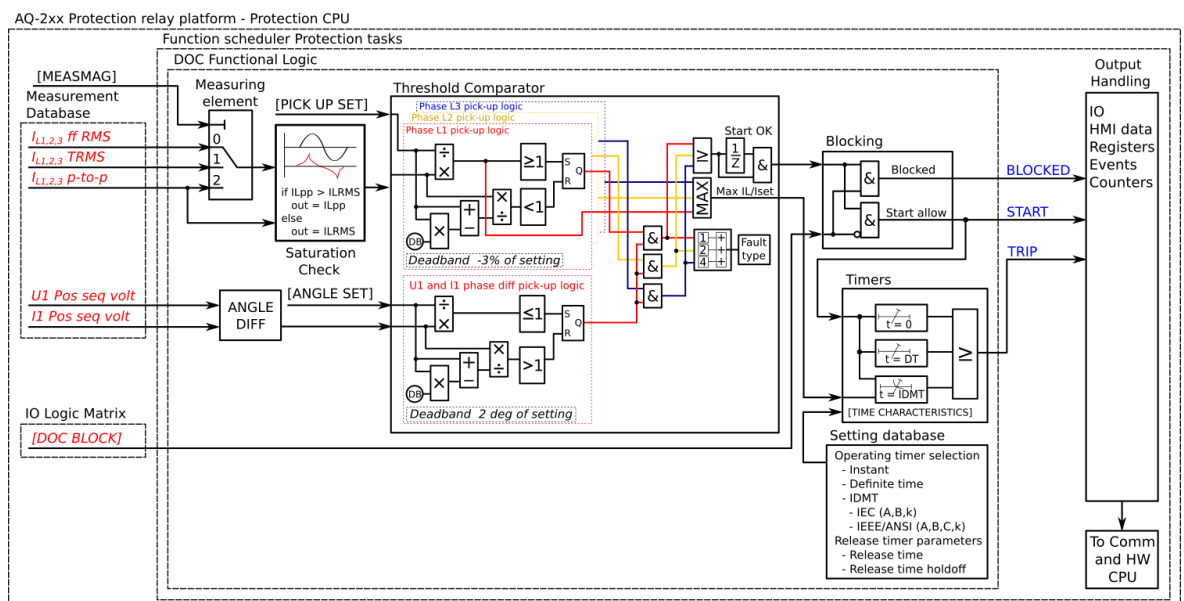
Figure. 5.3.4 - 88. Simplified function block diagram of the Idir> function.
