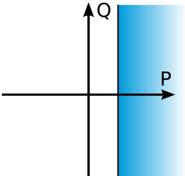
Figure. 5.3.16 - 140. Operating characteristics of overpower protection.
