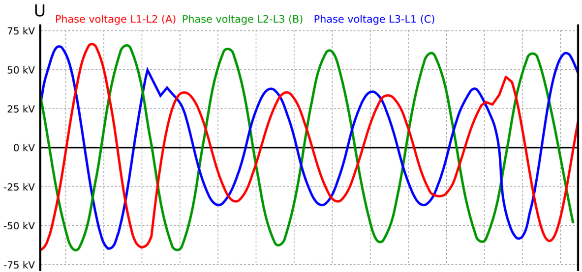
Figure. 5.4.8 - 204. Generator islanding.
