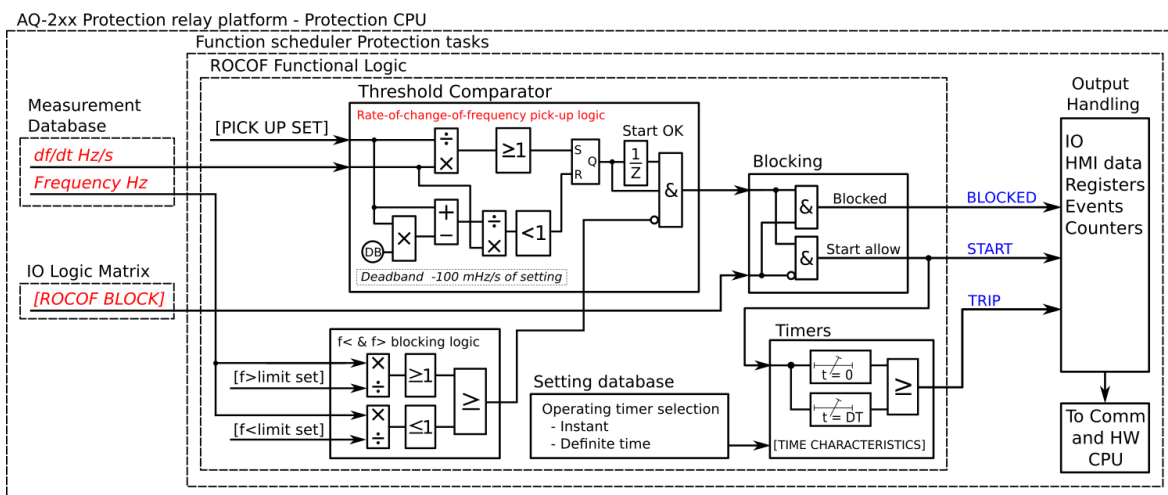
Figure. 5.3.15 - 139. Simplified function block diagram of the df/dt function.
