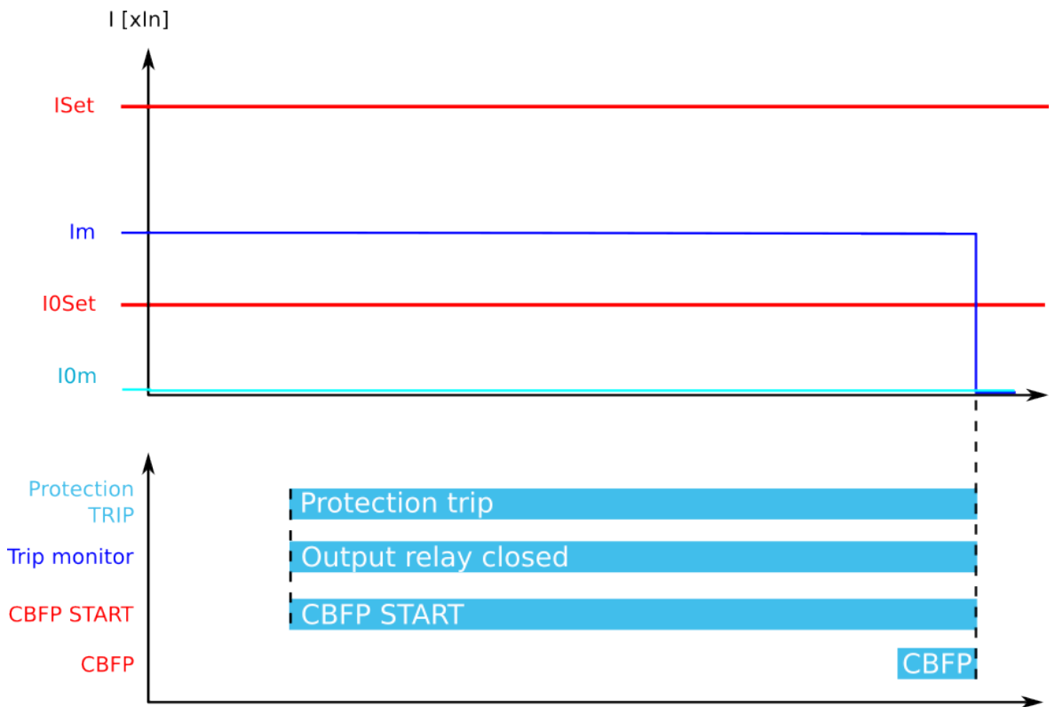
Figure. 5.3.8 - 109. CBFP when "Current or DO" is the selected criterion.
