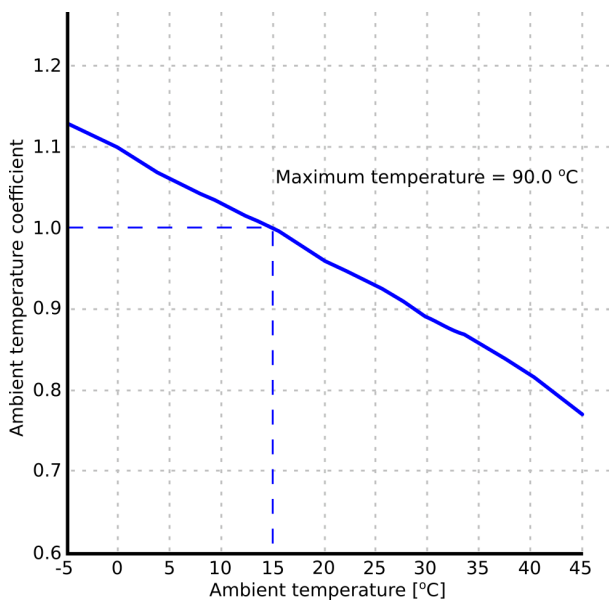
Figure. 5.3.19 - 151. Set correction curve for ambient temperature.
