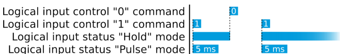
Figure. 5.4.12 - 207. Operation of logical input in "Hold" and "Pulse" modes.
