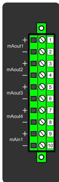
Figure. 8.13 - 259. Milliampere (mA) I/O module connections.
