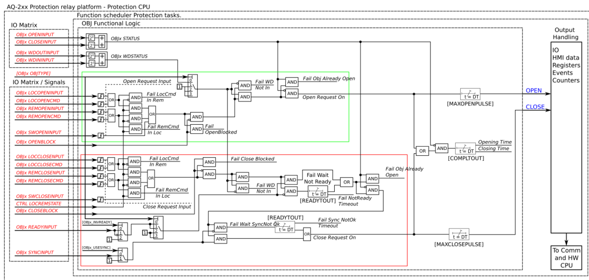
Figure. 5.4.2 - 173. Simplified function block diagram of the object control and monitoring function.
