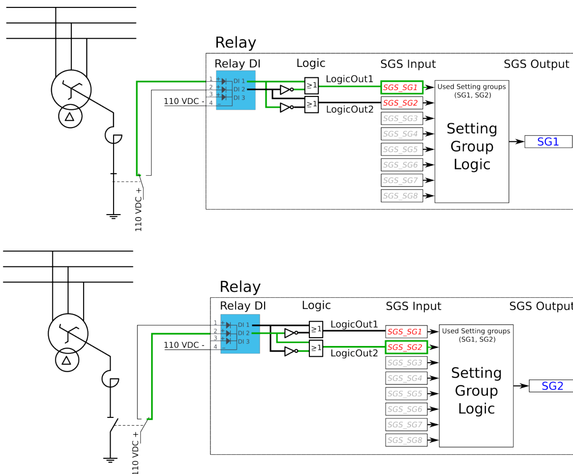
Figure. 5.4.1 - 171. Setting group control – two-wire connection from Petersen coil status with additional logic.
