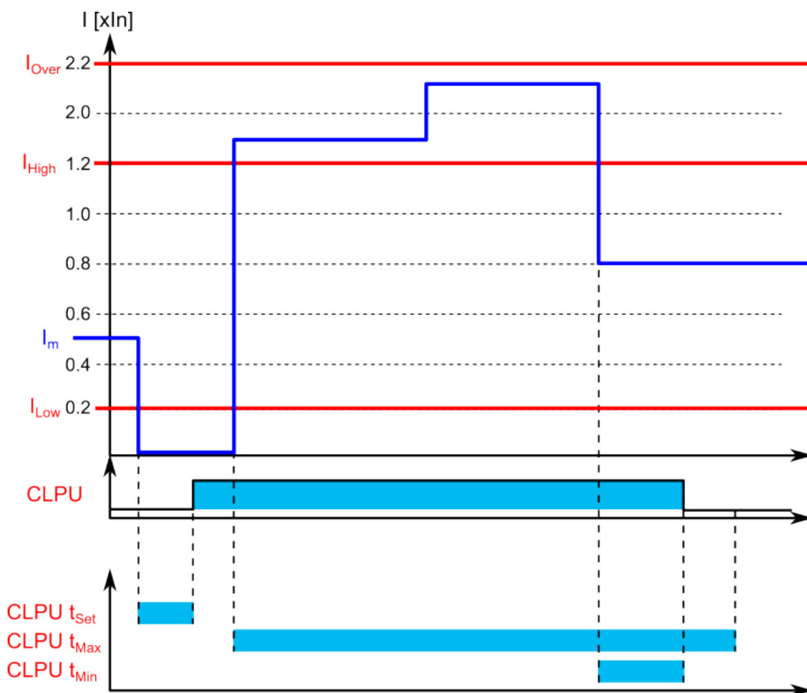
Figure. 5.4.5 - 194. Example of timers and pick-up parameters (normal CLPU situation).
