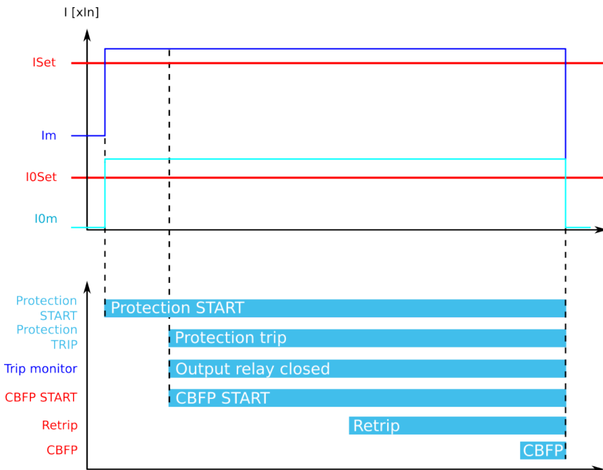
Figure. 5.3.8 - 104. Retrip and CBFP when "Current and DO" is the selected criterion.
