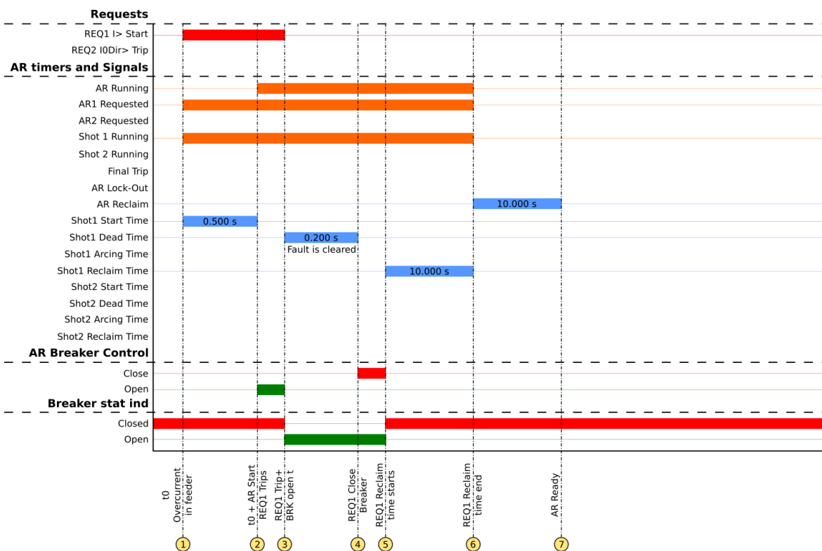
Figure. 5.4.4 - 189. Signal status graph of the transient overcurrent auto-recloser cycle.
