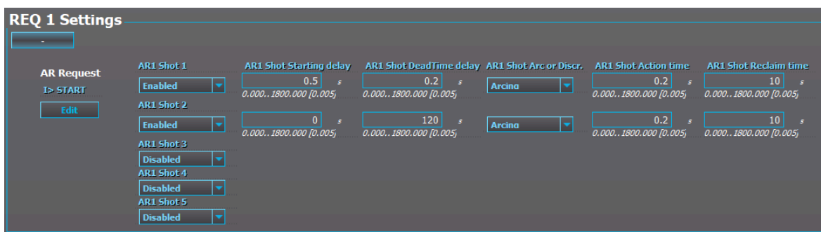
Figure. 5.4.4 - 186. Settings for I> with two shots.
