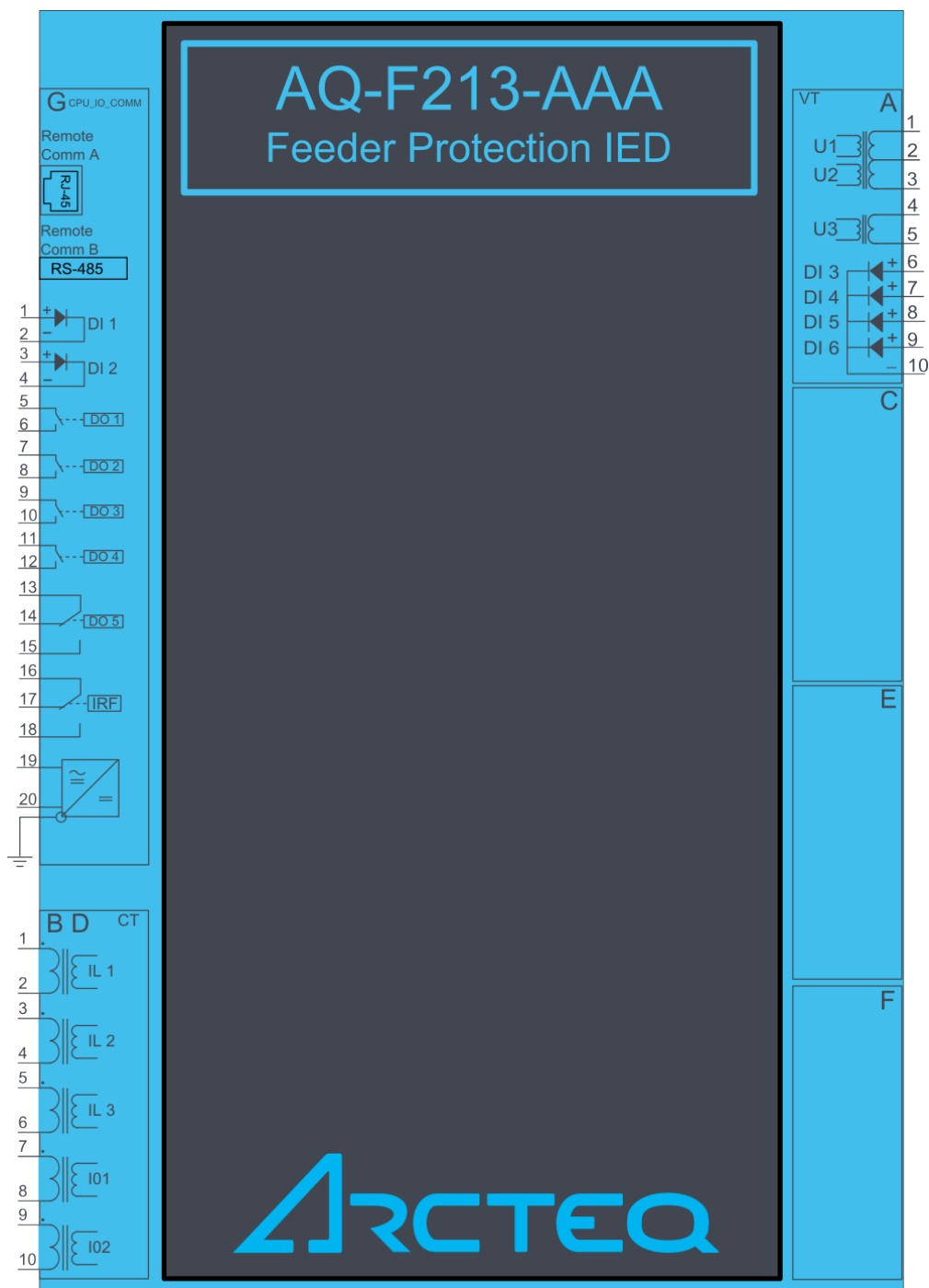
Figure. 7.1 - 230. AQ-F213 variant without add-on modules.
