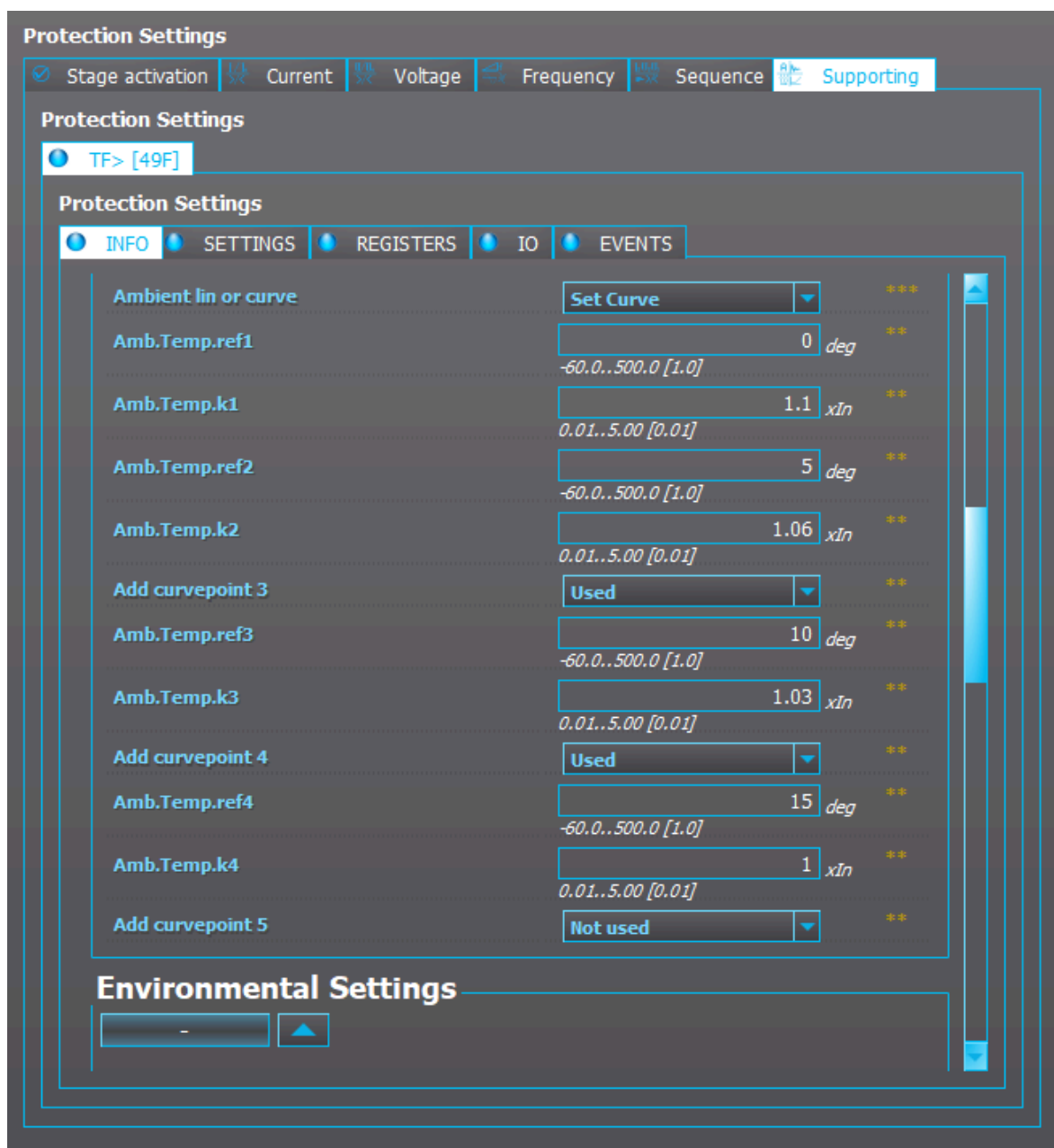
Figure. 5.3.19 - 150. Settings of the function's ambient temperature coefficient curve.
