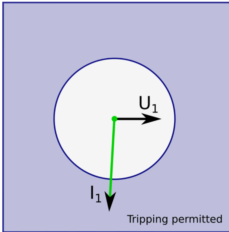
Figure. 5.3.4 - 91. When I_{dir} function has been set to "Non-directional" the function works basically just like a traditional non-directional overcurrent protection function.
