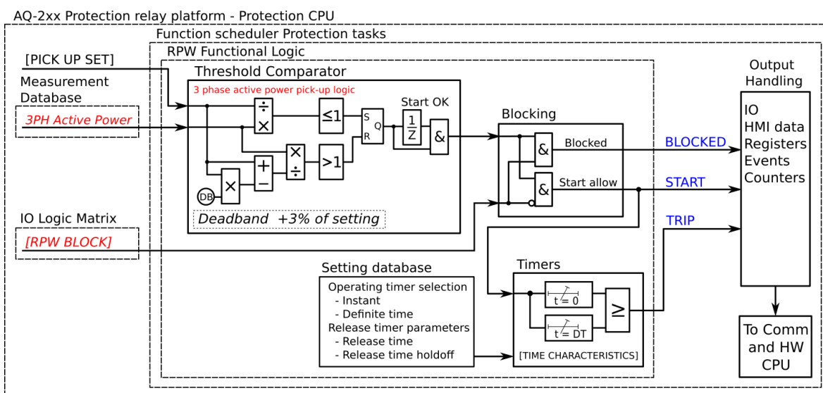
Figure. 5.3.18 - 146. Simplified function block diagram of the Pr function.
