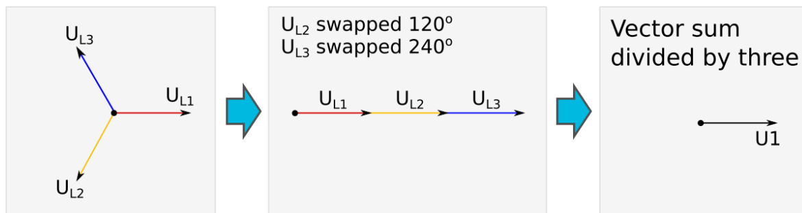
Figure. 5.3.13 - 129. Earth fault in an isolated network.
