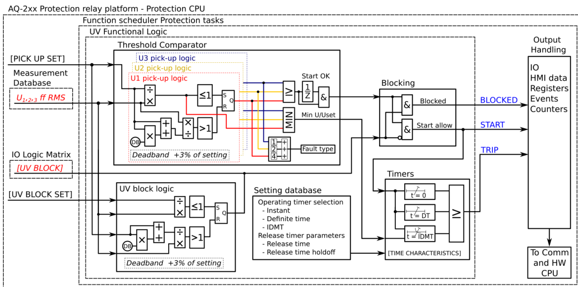
Figure. 5.3.11 - 122. Simplified function block diagram of the U < function.
