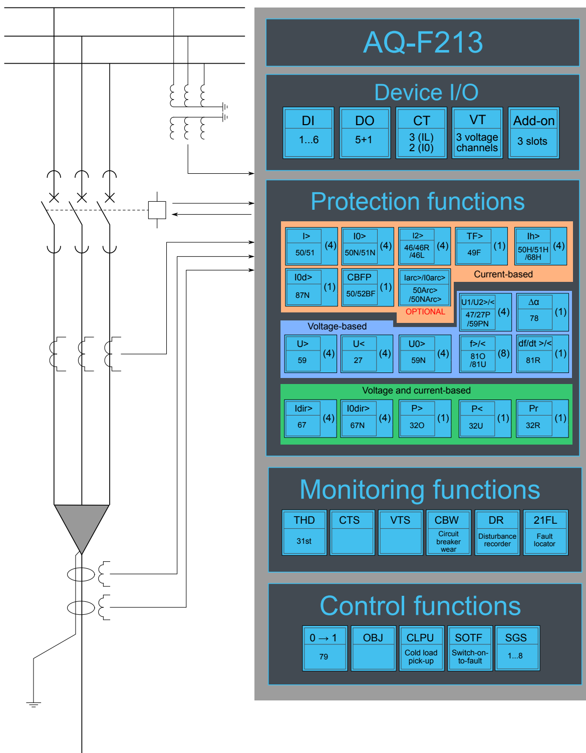
Figure. 7.1 - 232. AQ-F213 application example with function block diagram.
