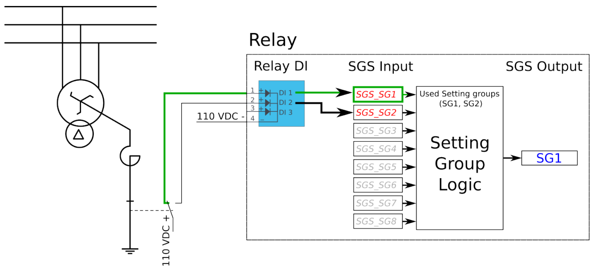
Figure. 5.4.1 - 170. Setting group control – two-wire connection from Petersen coil status.
