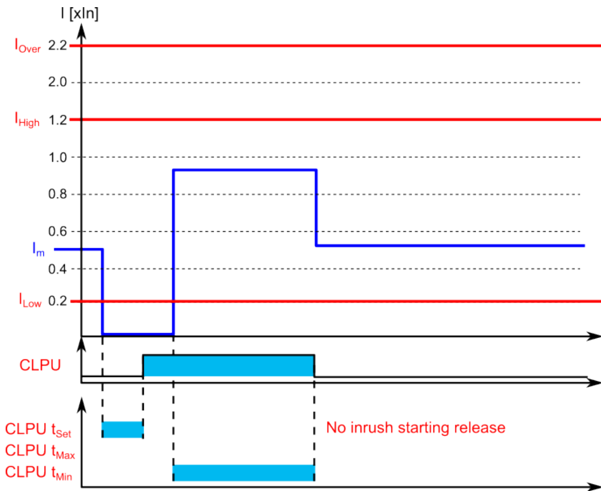
Figure. 5.4.5 - 198. Example of timers and pick-up parameters (no inrush current detected in the starting).
