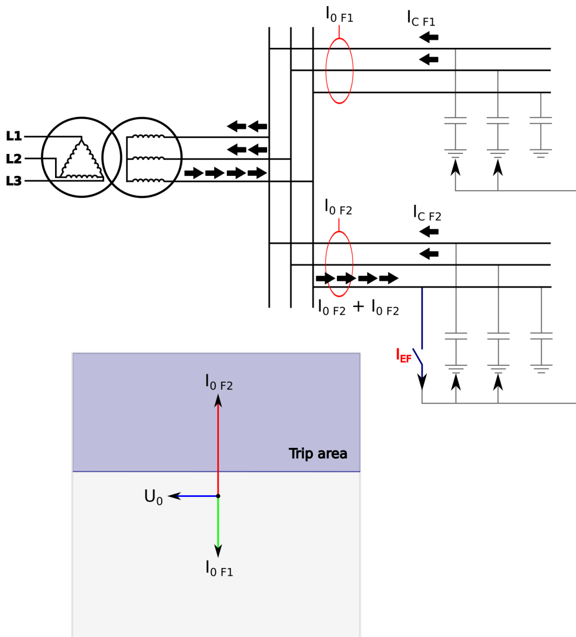
Figure. 5.3.5 - 93. Angle tracking of I_{0dir} function (unearthed network model) (32N)
