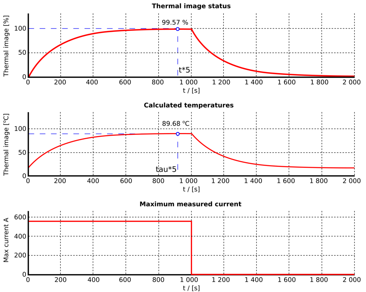
Figure. 5.3.19 - 158. Thermal response with k SF factor correctly set.
