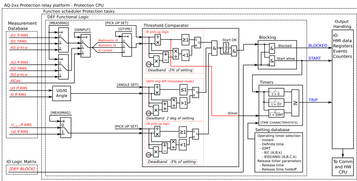
Figure. 5.3.5 - 92. Simplified function block diagram of the I0dir> function.
