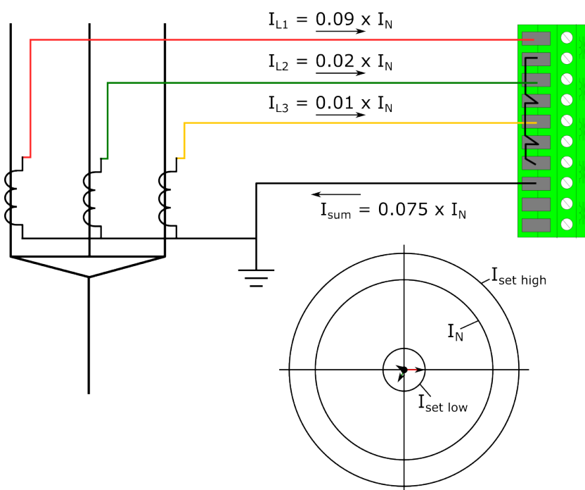
Figure. 5.5.1 - 215. Low current and heavy unbalance.
