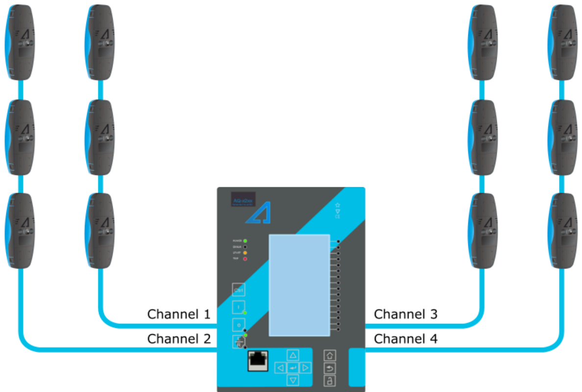
Figure. 5.3.21 - 161. IED equipped with arc protection.
