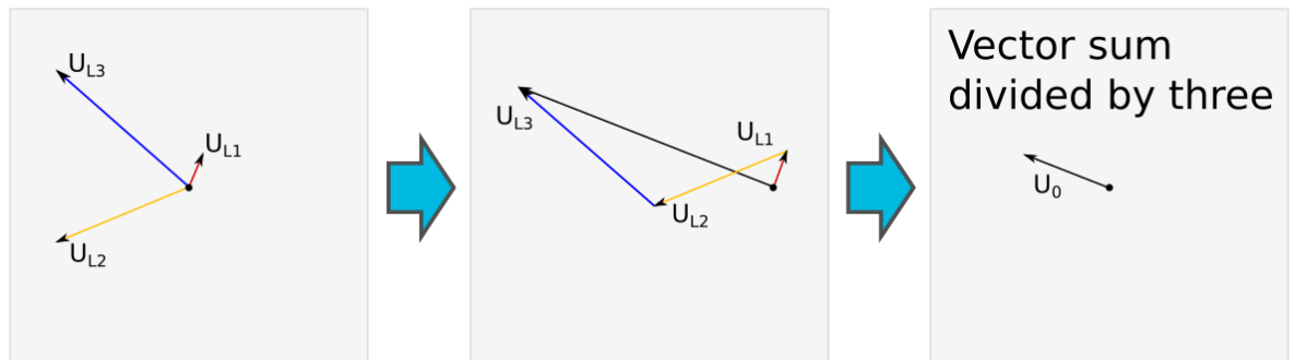
Figure. 5.3.12 - 125. Earth fault in isolated network.
