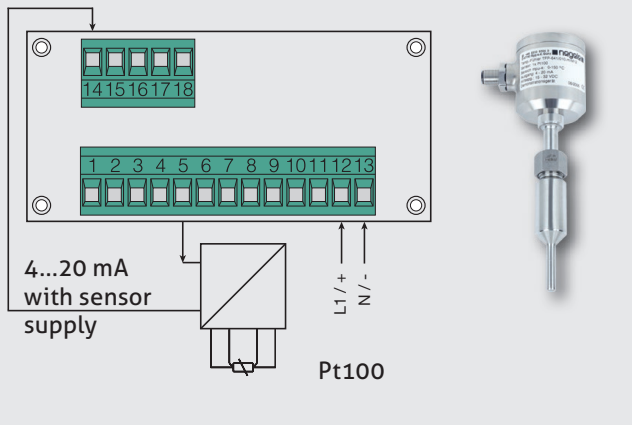
Fig. 1: Electrical connection | 2-wire transducer
