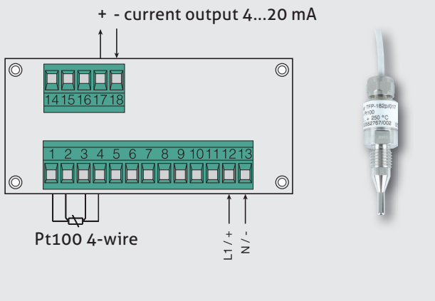
Fig. 3: Electrical connection | 0/4...20 mA
