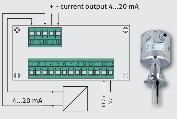
Fig. 3: Electrical connection | 0/4...20 mA
