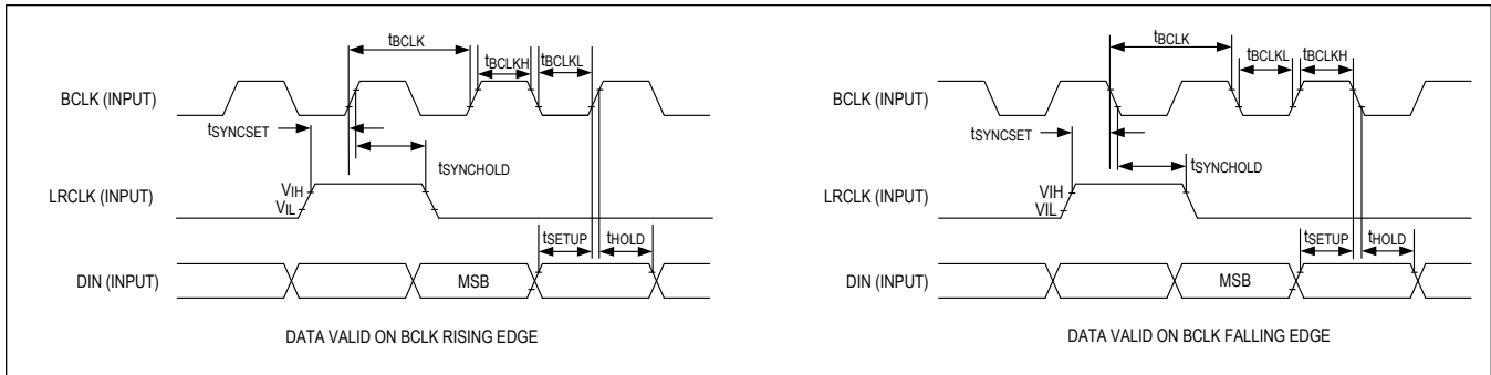
Figure 13. TDM Timing Diagrams—BCLK Rising Edge (MAX98361A/C) and BCLK Falling Edge (MAX98361B/D)
