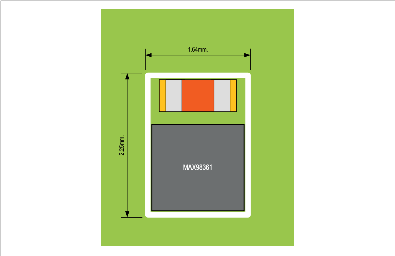
Figure 14. Solution Size
