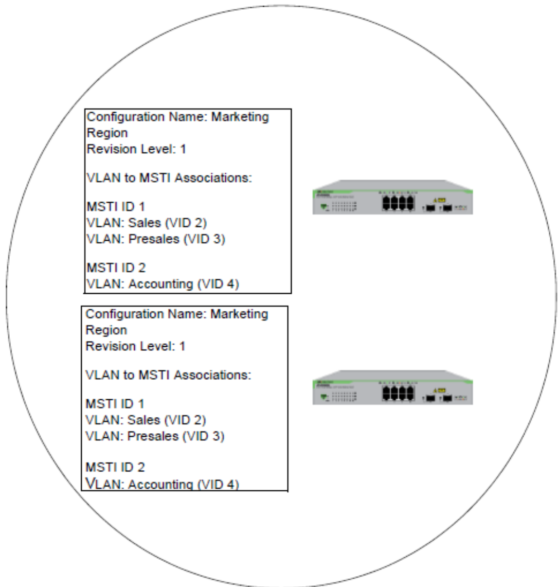
Figure 121. Multiple Spanning Tree Region
