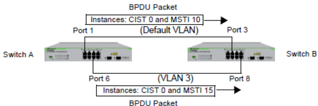
Figure 122. CIST and VLAN Guideline - Example 1
