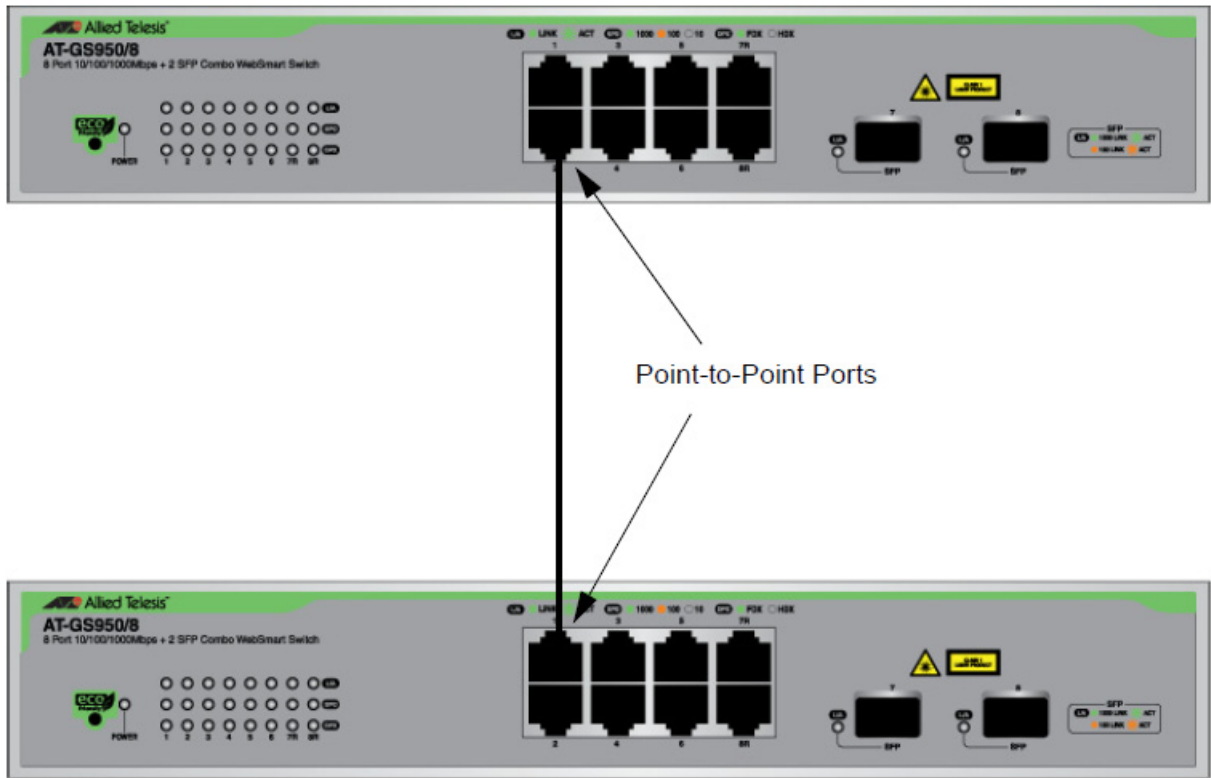
Figure 36. Point-to-Point Ports
