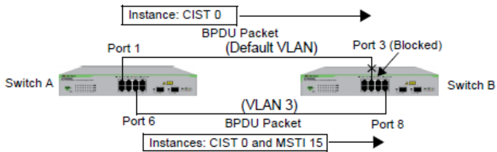
Figure 123. CIST and VLAN Guideline - Example 2
