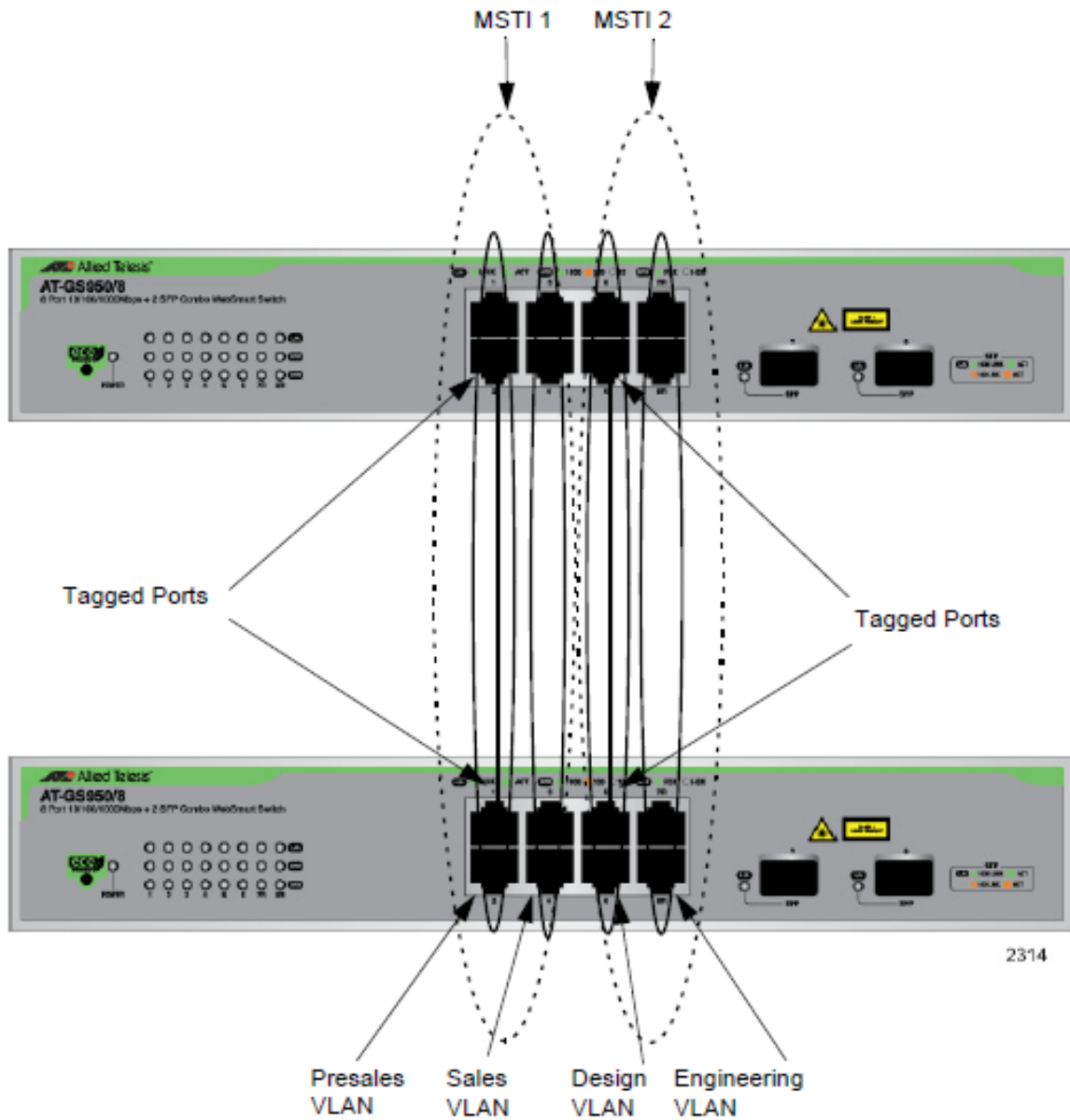
Figure 120. Multiple VLANs in a MSTI
