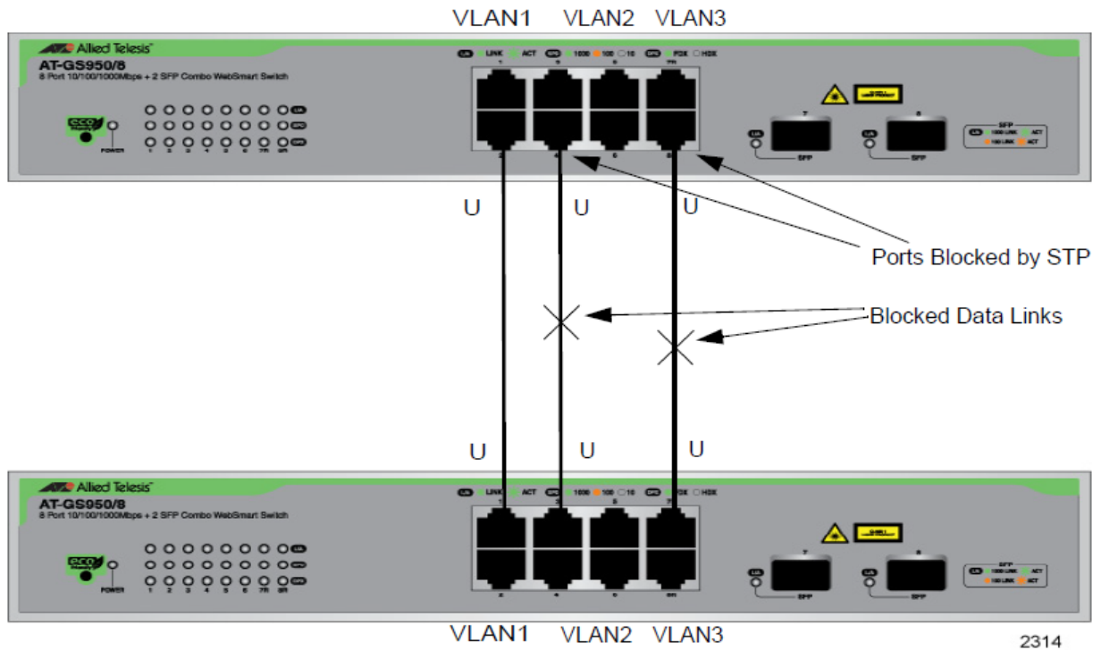
Figure 38. STP and VLAN Fragmentation with Untagged Ports
