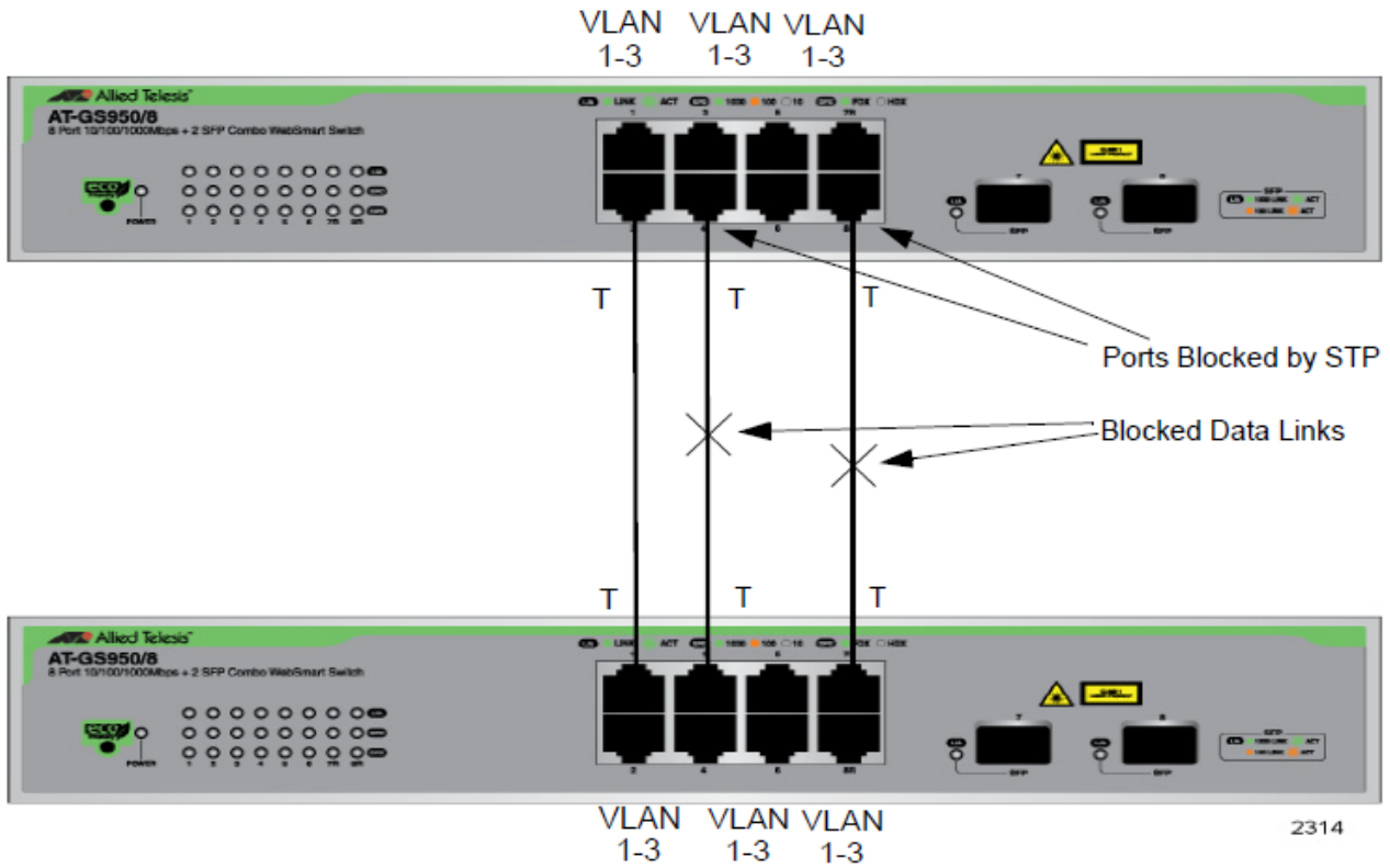
Figure 39. STP and VLAN Compatibility with Tagged Ports
