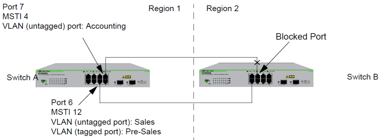
Figure 124. Spanning Regions - Example 1
