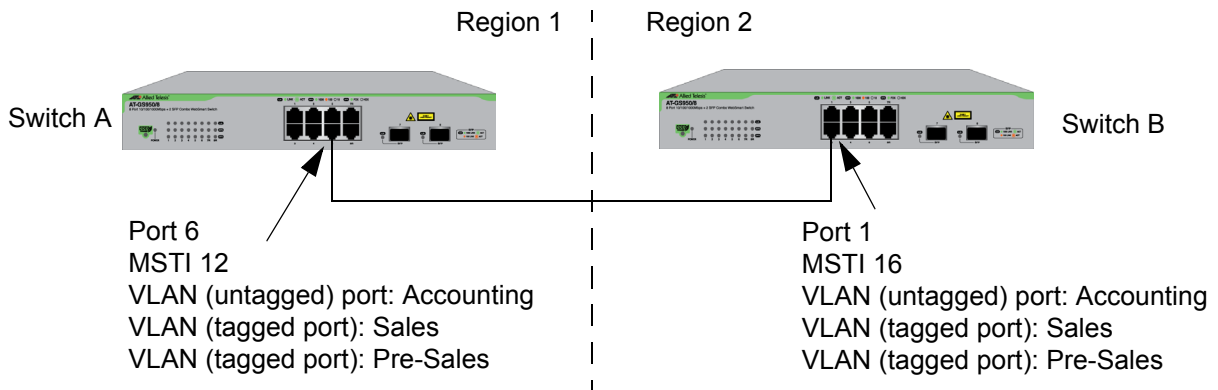
Figure 125. Spanning Regions without Blocking
