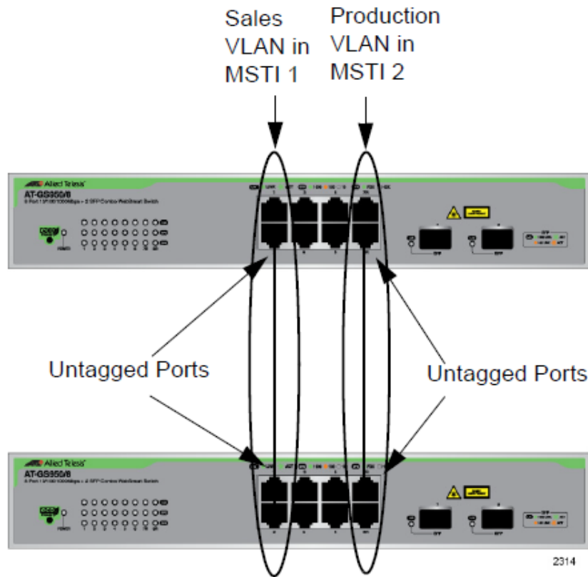
Figure 119. MSTP Example of Two Spanning Tree Instances
