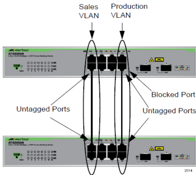
Figure 118. VLAN Fragmentation with STP or RSTP
