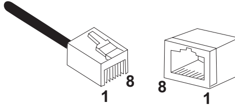
Figure 10 RJ-45 Connector and Port Pin Layout
