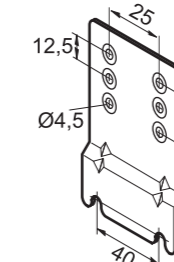
Mounting plate for units with hood Part No.: 803 801
