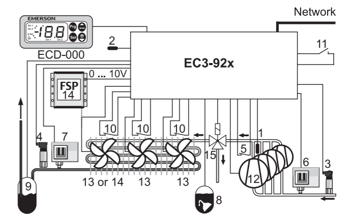
EC3-392 Rack and Condenser Controller (up to 4 compressors + condenser)
