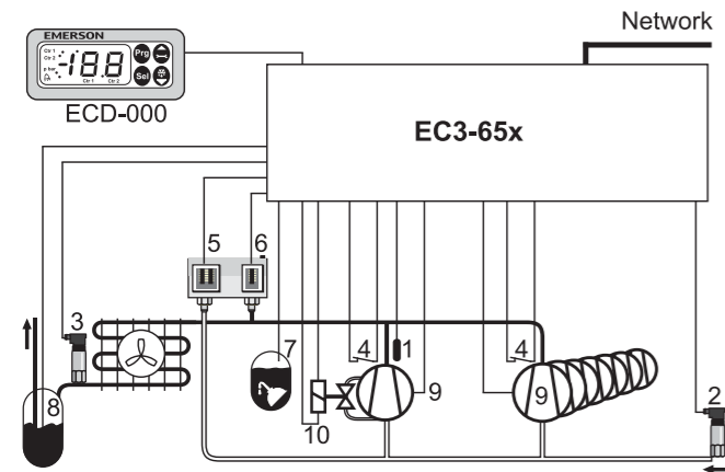
EC3-652 Rack Controller for 8 single-stage compressors or 7 single-stage Compressors and 1 Digital Scroll™
