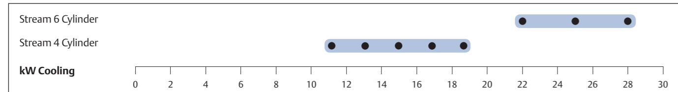
Conditions: EN12900 R404: Evaporating -35° C, Condensing 40° C, Suction Gas Temperature 20° C, Subcooling 0K
