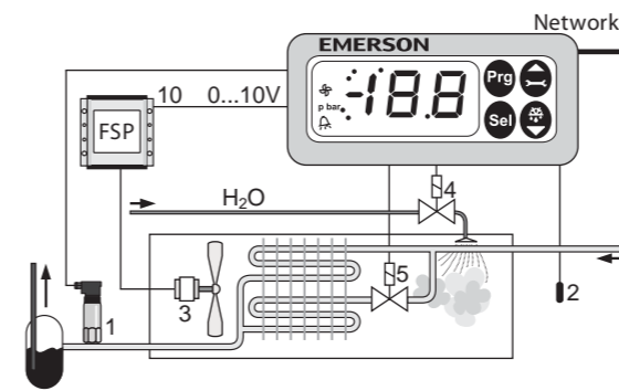
EC2-74x Condenser Controller with fan speed control
