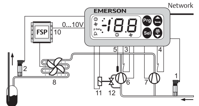
EC2-552 Condensing Unit Controller for 2 single stage compressors or 1 Digital Scroll™ and 1 single stage compressor
