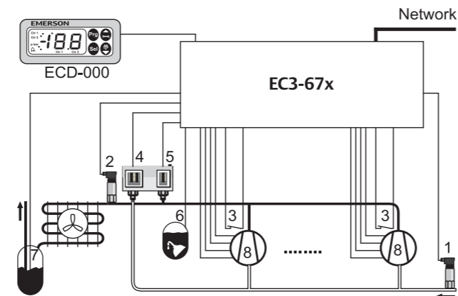
EC3-672 Rack Controller for Capacity Controlled Compressors
