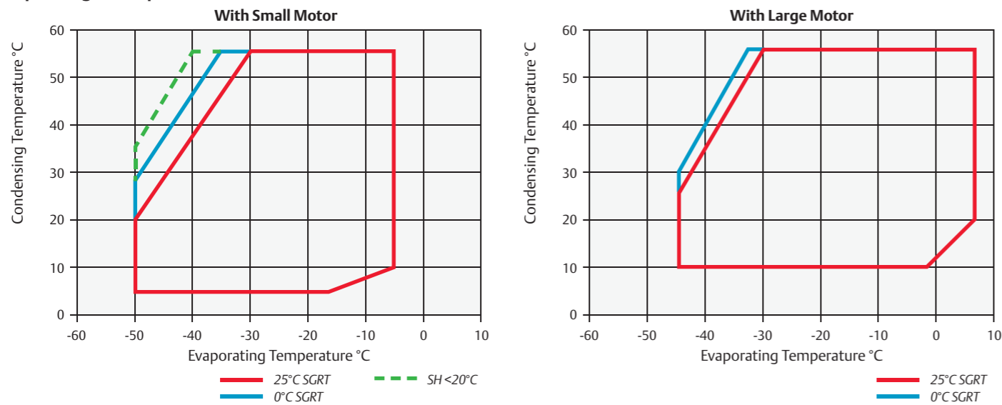
Conditions: EN12900 R404: Evaporating -35° C, Condensing 40° C, Suction Gas Temperature 20° C, Subcooling 0K
