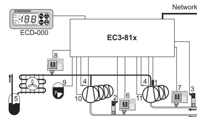
EC3-812 Dual Circuit Rack Controller (4 + 3 compressors)
