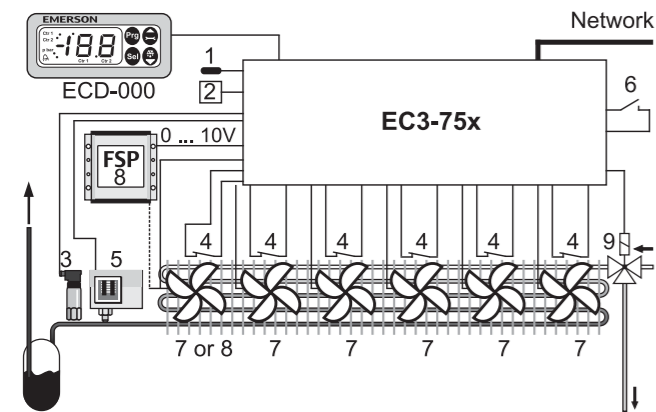
EC3-752 Condenser Controller
