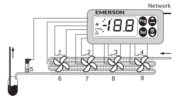
EC2-71x Condenser Controller for up to 4 fans
