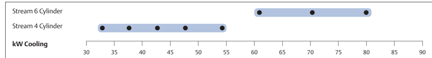
Conditions: EN12900 R404A: Evaporating -10° C, Condensing 45° C, Suction Gas Temperature 20° C, Subcooling 0K
